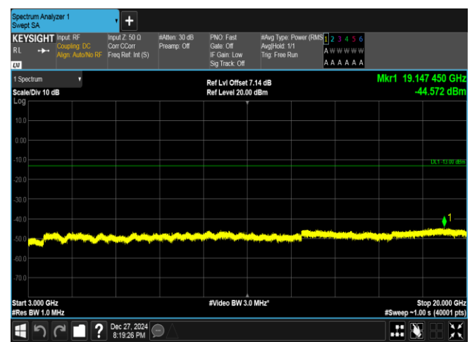
Band25-3MHz-QPSK-26055-1RB#14-3000~20000-PASS
