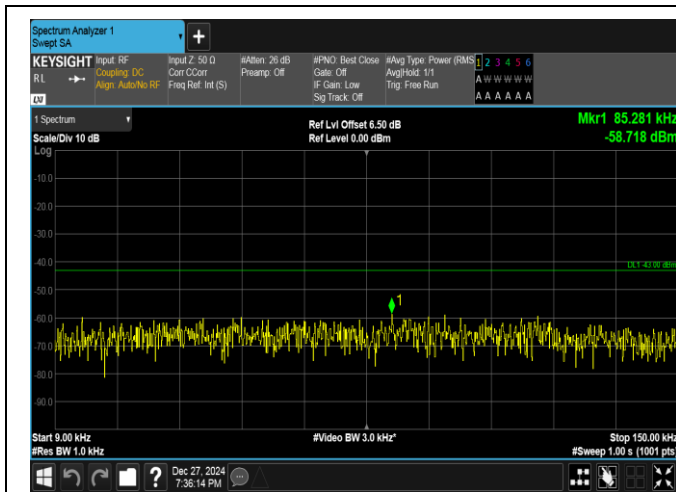
Band25-1.4MHz-16QAM-26365-1RB#0-0.009~0.15-PASS
