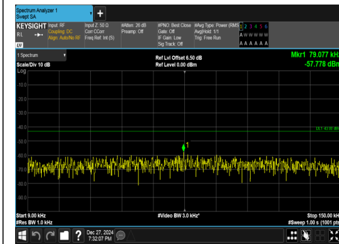
Band25-1.4MHz-16QAM-26047-1RB#5-0.009~0.15-PASS
