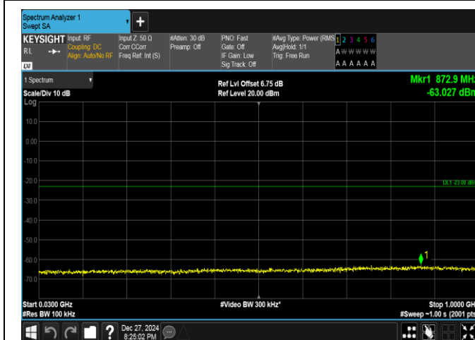
Band25-3MHz-QPSK-26365-1RB#14-30~1000-PASS
