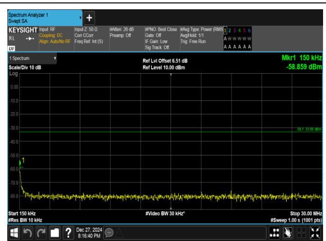
Band25-3MHz-QPSK-26055-1RB#0-0.15~30-PASS
