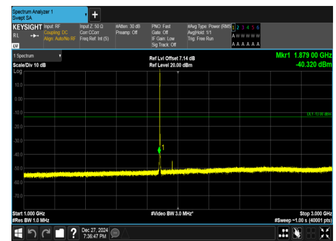
Band25-1.4MHz-16QAM-26365-1RB#0-1000~3000-PASS
