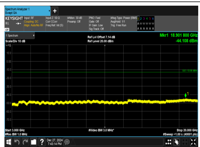
Band25-1.4MHz-16QAM-26683-1RB#0-3000~20000-PASS S
