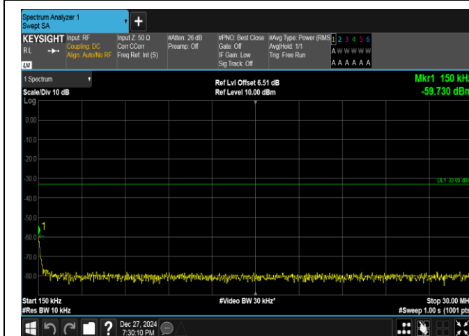
Band25-1.4MHz-16QAM-26047-1RB#0-0.15~30-PASS
