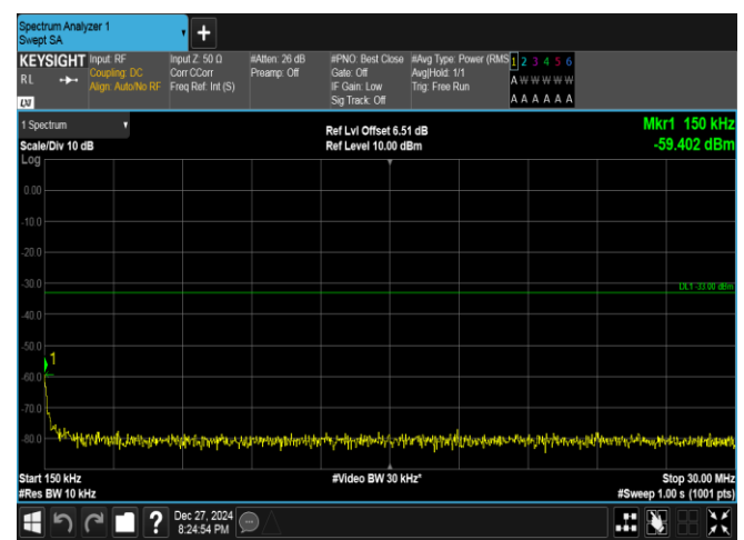
Band25-3MHz-QPSK-26365-1RB#14-0.15~30-PASS
