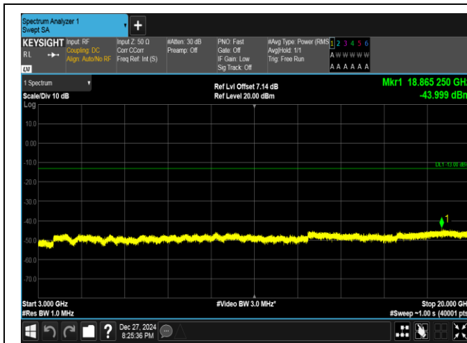
Band25-3MHz-QPSK-26365-1RB#14-3000~20000-PASS
