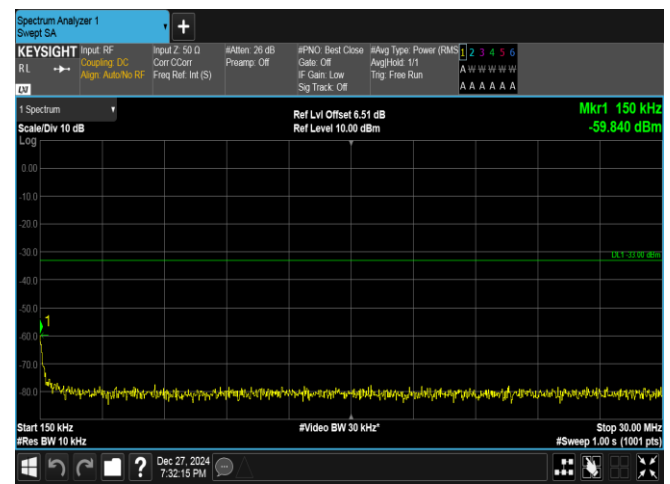
Band25-1.4MHz-16QAM-26047-1RB#5-0.15~30-PASS
