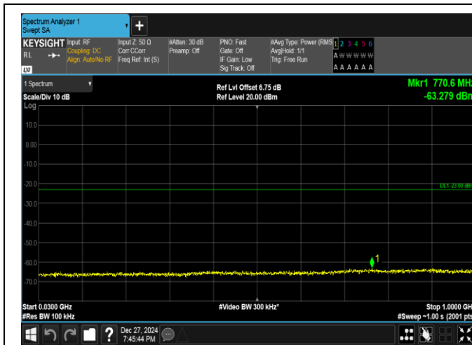
Band25-1.4MHz-QPSK-26683-6RB#0-30~1000-PASS
