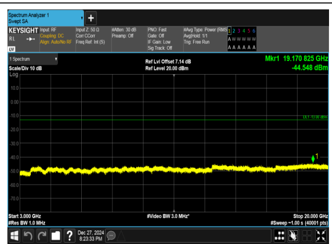
Band25-3MHz-QPSK-26365-1RB#0-3000~20000-PASS
