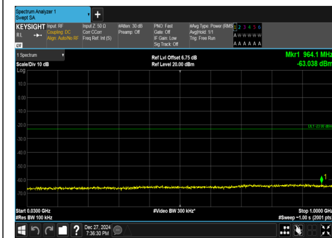
Band25-1.4MHz-16QAM-26365-1RB#0-30~1000-PASS
