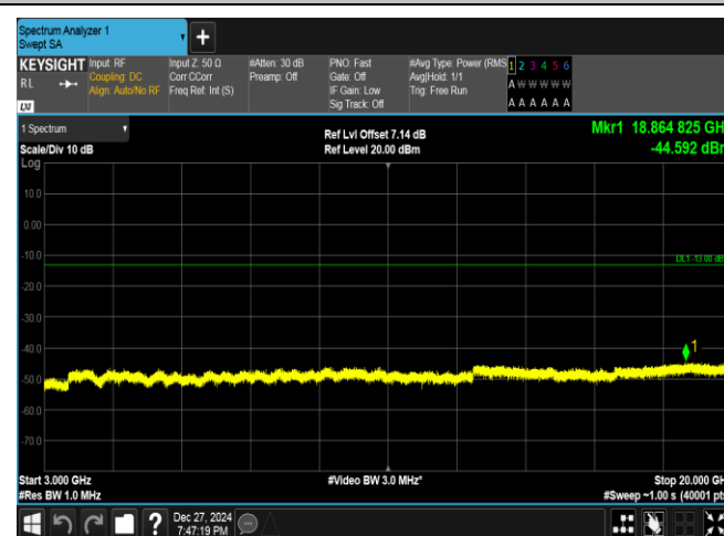
Band25-1.4MHz-16QAM-26683-6RB#0-3000~20000-PAS S
