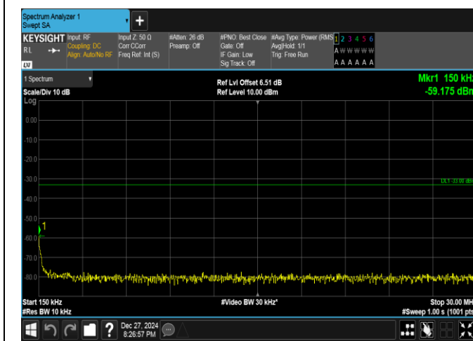
Band25-3MHz-QPSK-26365-15RB#0-0.15~30-PASS
