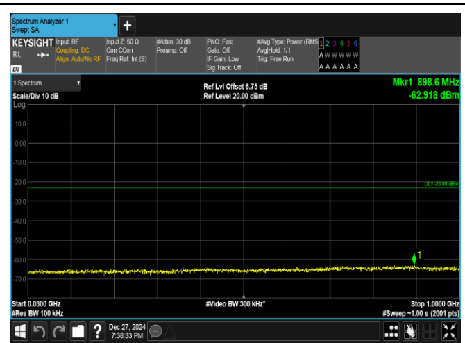
Band25-1.4MHz-16QAM-26365-1RB#5-30~1000-PASS
