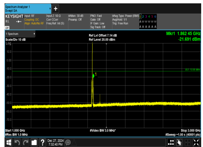
Band25-1.4MHz-16QAM-26047-1RB#5-1000~3000-PASS
