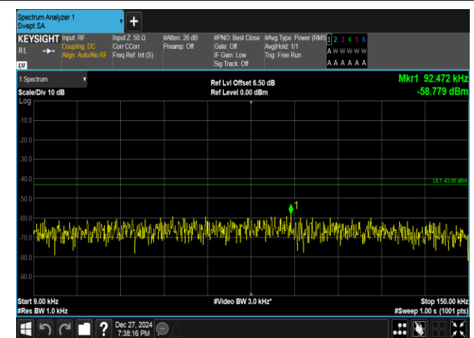
Band25-1.4MHz-16QAM-26365-1RB#5-0.009~0.15-PASS
