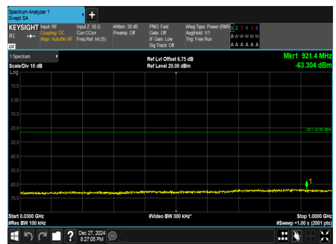
Band25-3MHz-QPSK-26365-15RB#0-30~1000-PASS
