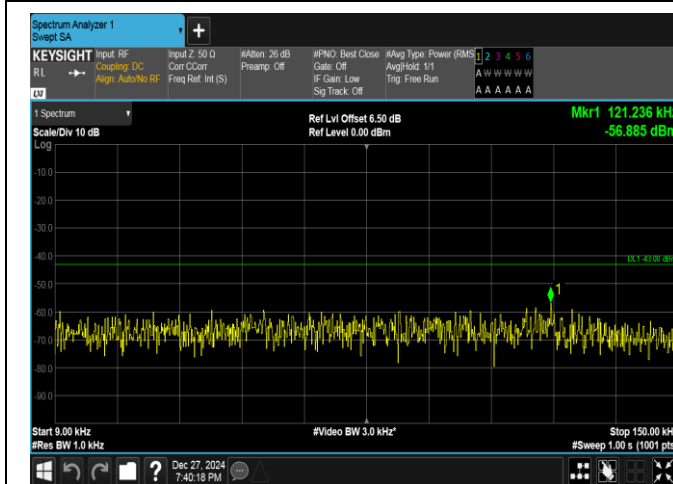
Band25-1.4MHz-16QAM-26365-6RB#0-0.009~0.15-PASS
