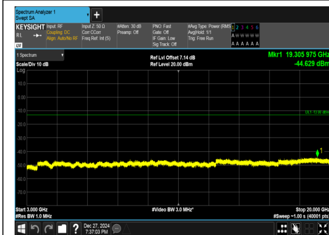
Band25-1.4MHz-16QAM-26365-1RB#0-3000~20000-PAS
