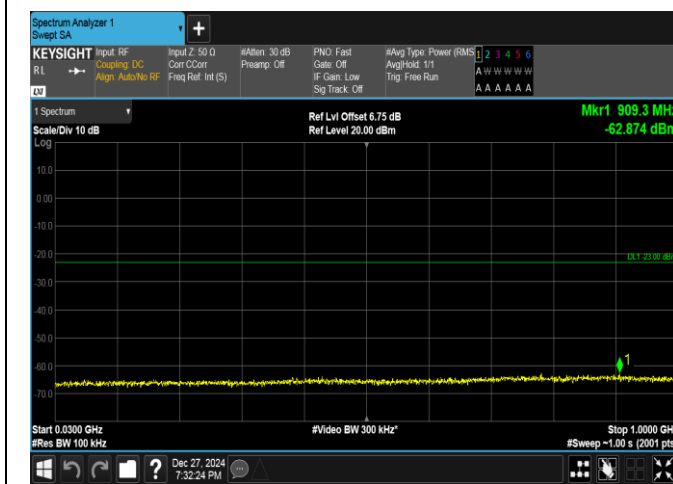
Band25-1.4MHz-16QAM-26047-1RB#5-30~1000-PASS
