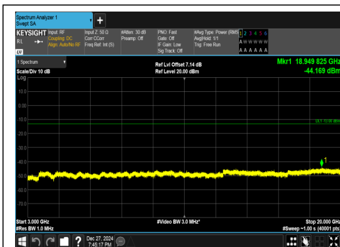
Band25-1.4MHz-16QAM-26683-1RB#5-3000~20000-PAS S
