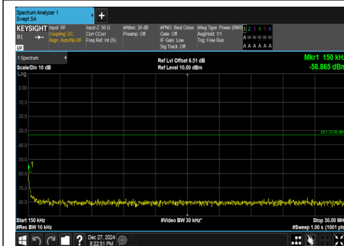
Band25-3MHz-QPSK-26365-1RB#0-0.15~30-PASS
