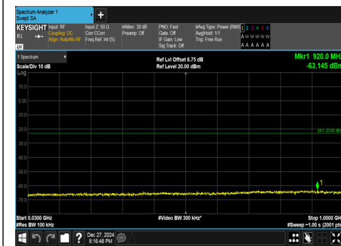
Band25-3MHz-QPSK-26055-1RB#0-30~1000-PASS
