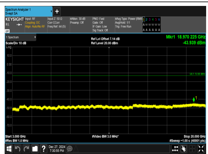
Band25-1.4MHz-16QAM-26047-1RB#0-3000~20000-PASS S
