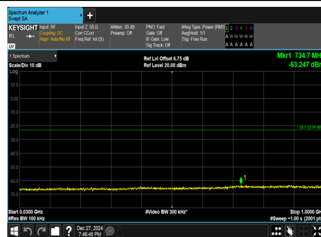
Band25-1.4MHz-16QAM-26683-6RB#0-30~1000-PASS
