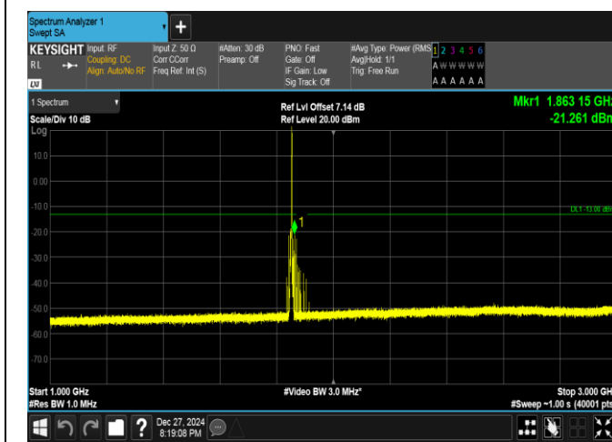
Band25-3MHz-QPSK-26055-1RB#14-1000~3000-PASS
