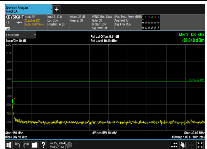
Band25-1.4MHz-16QAM-26365-6RB#0-0.15~30-PASS
