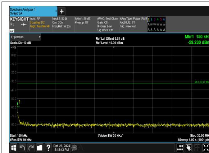
Band25-3MHz-QPSK-26055-1RB#14-0.15~30-PASS
