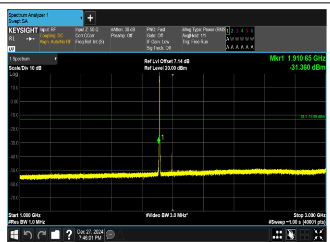
Band25-1.4MHz-QPSK-26683-6RB#0-1000~3000-PASS
