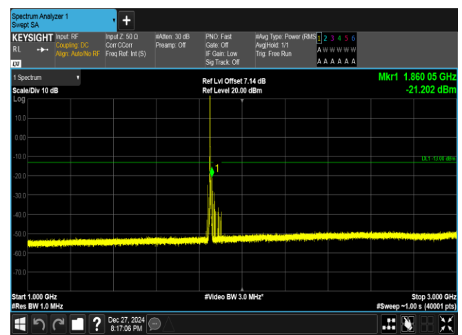
Band25-3MHz-QPSK-26055-1RB#0-1000~3000-PASS
