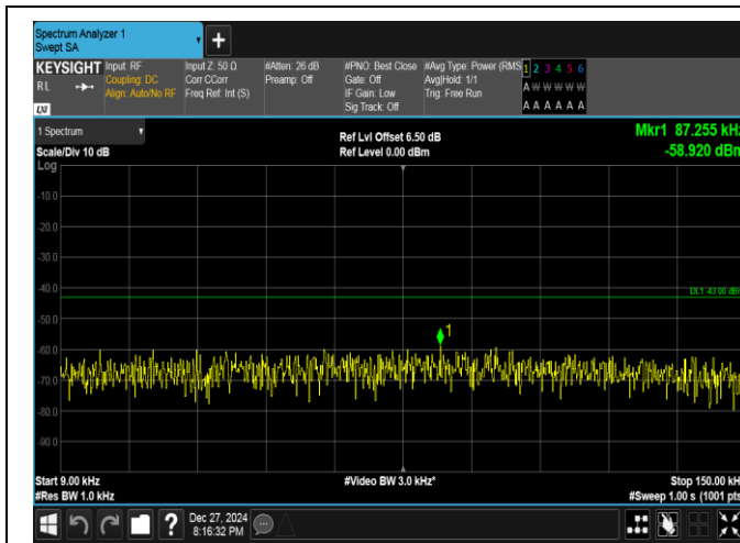
Band25-3MHz-QPSK-26055-1RB#0-0.009~0.15-PASS
