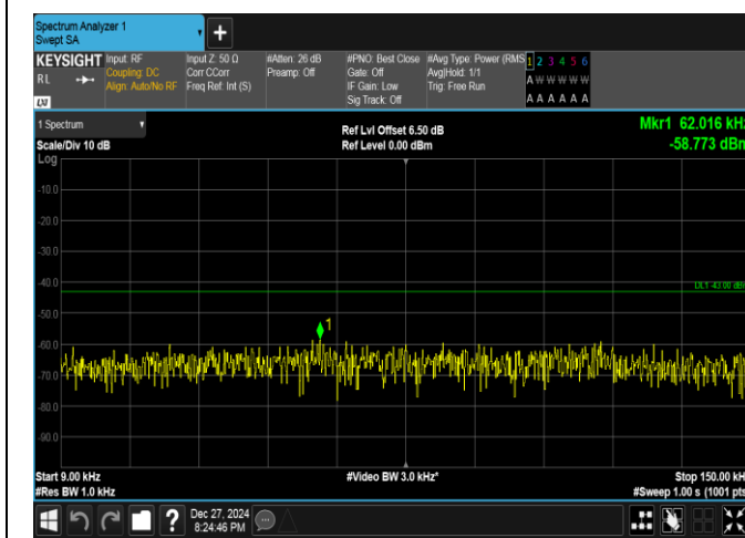
Band25-3MHz-QPSK-26365-1RB#14-0.009~0.15-PASS
