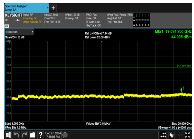
Band25-1.4MHz-16QAM-26365-1RB#5-3000~20000-PAS S
