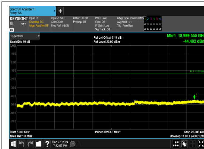
Band25-1.4MHz-16QAM-26047-1RB#5-3000~20000-PAS S
