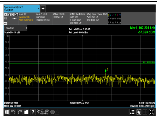
Band25-1.4MHz-16QAM-26047-6RB#0-0.009~0.15-PASS
