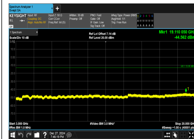
Band25-1.4MHz-QPSK-26683-6RB#0-3000~20000-PASS
