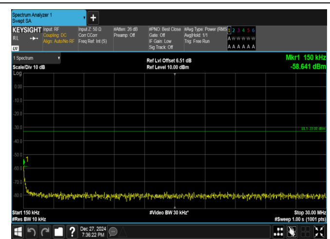
Band25-1.4MHz-16QAM-26365-1RB#0-0.15~30-PASS
