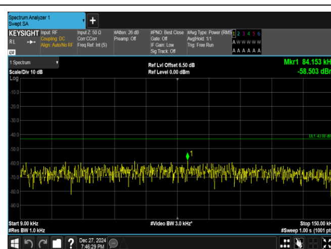
Band25-1.4MHz-16QAM-26683-6RB#0-0.009~0.15-PASS
