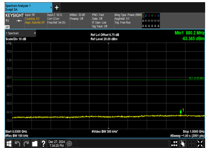
Band25-1.4MHz-16QAM-26047-6RB#0-30~1000-PASS
