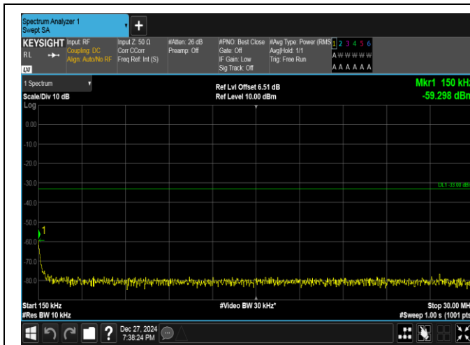
Band25-1.4MHz-16QAM-26365-1RB#5-0.15~30-PASS
