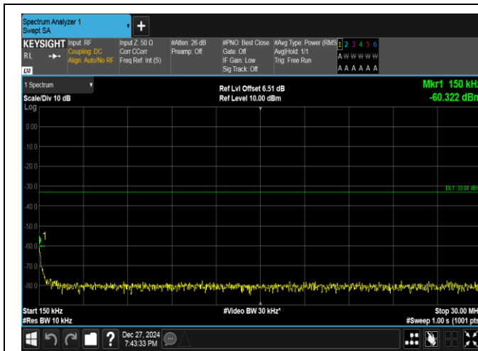
Band25-1.4MHz-QPSK-26683-1RB#5-0.15~30-PASS
