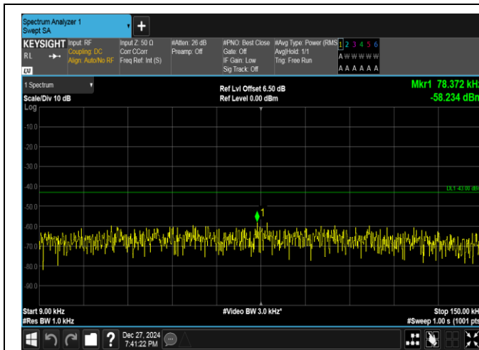
Band25-1.4MHz-QPSK-26683-1RB#0-0.009~0.15-PASS
