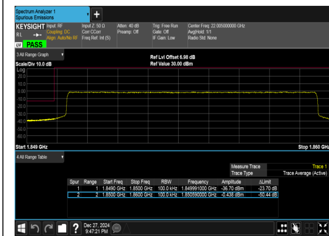
Band25-10MHz-16QAM-26090-50RB#0-PASS
