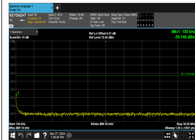
Band25-1.4MHz-QPSK-26365-6RB#0-0.15~30-PASS
