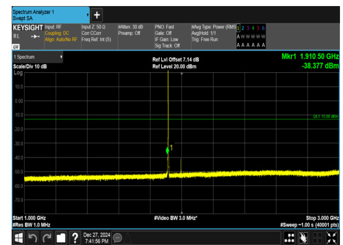
Band25-1.4MHz-QPSK-26683-1RB#0-1000~3000-PASS
