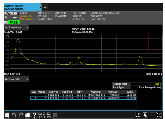
Band25-10MHz-16QAM-26640-1RB#0-PASS
