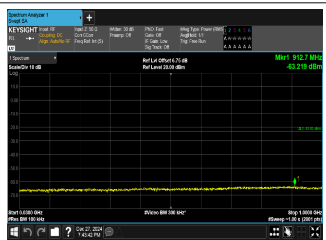
Band25-1.4MHz-QPSK-26683-1RB#5-30~1000-PASS
