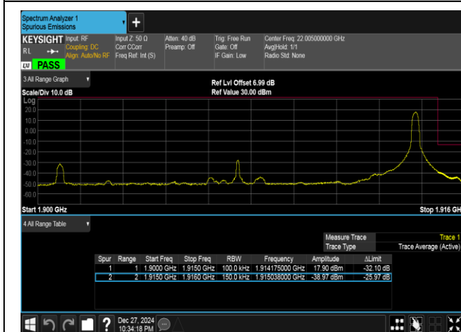
Band25-15MHz-16QAM-26615-1RB#74-PASS
