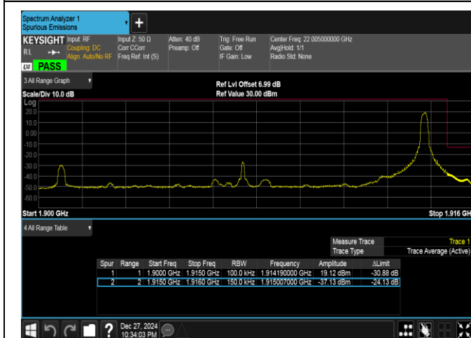
Band25-15MHz-QPSK-26615-1RB#74-PASS
