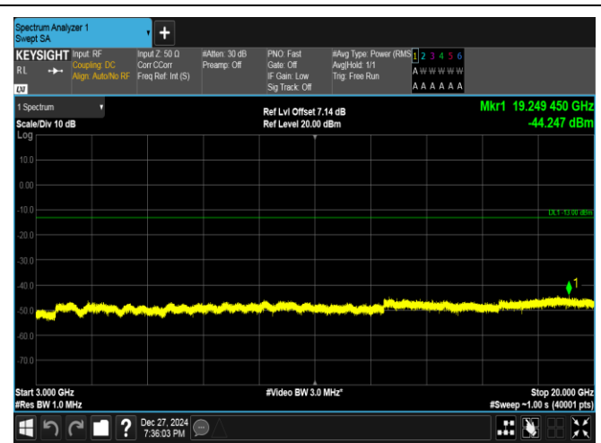
Band25-1.4MHz-QPSK-26365-1RB#0-3000~20000-PASS
