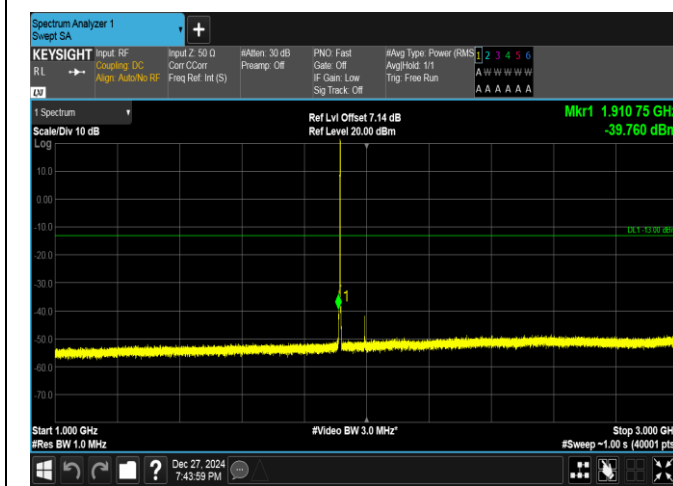
Band25-1.4MHz-QPSK-26683-1RB#5-1000~3000-PASS
