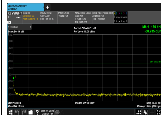
Band25-1.4MHz-QPSK-26365-1RB#0-0.15~30-PASS
