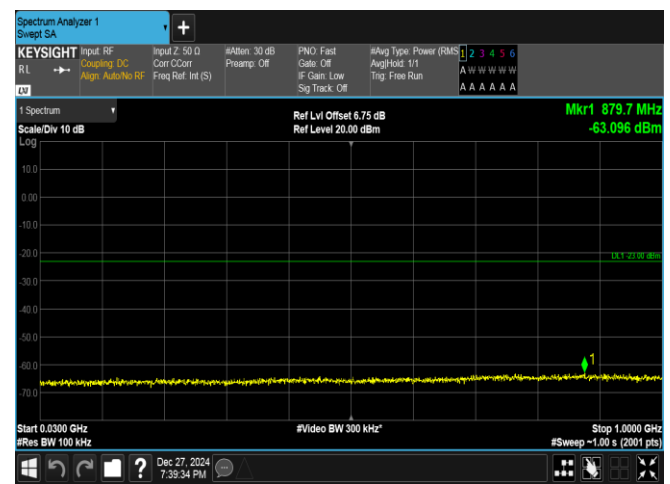
Band25-1.4MHz-QPSK-26365-6RB#0-30~1000-PASS
