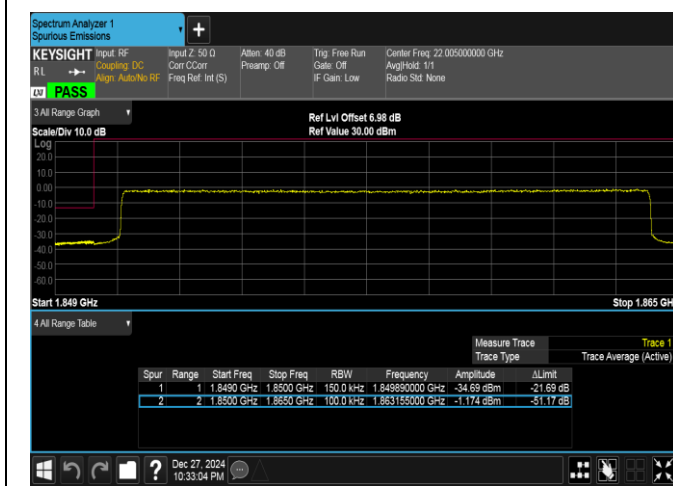
Band25-15MHz-QPSK-26115-75RB#0-PASS
