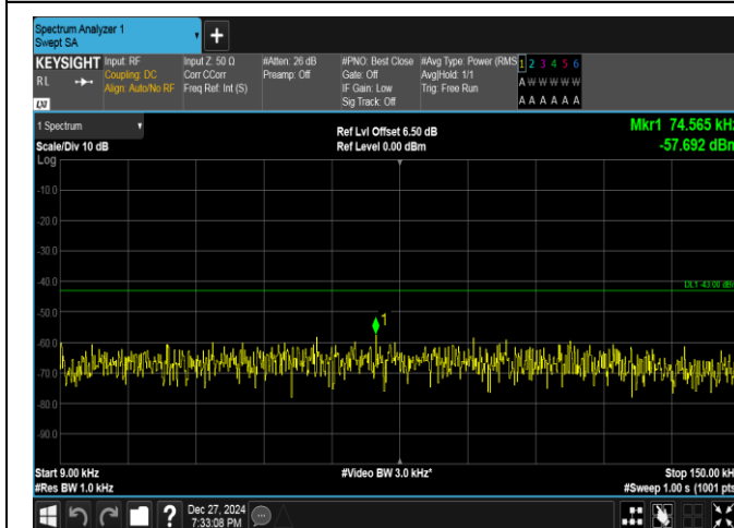
Band25-1.4MHz-QPSK-26047-6RB#0-0.009~0.15-PASS
