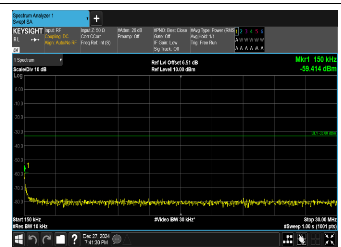
Band25-1.4MHz-QPSK-26683-1RB#0-0.15~30-PASS
