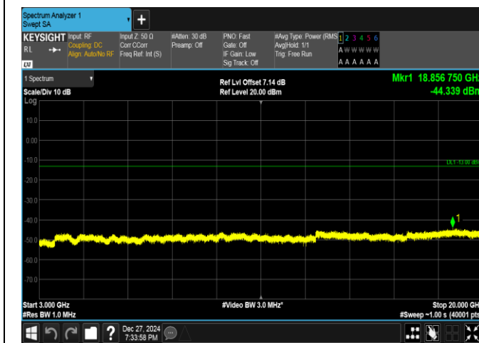
Band25-1.4MHz-QPSK-26047-6RB#0-3000~20000-PASS
