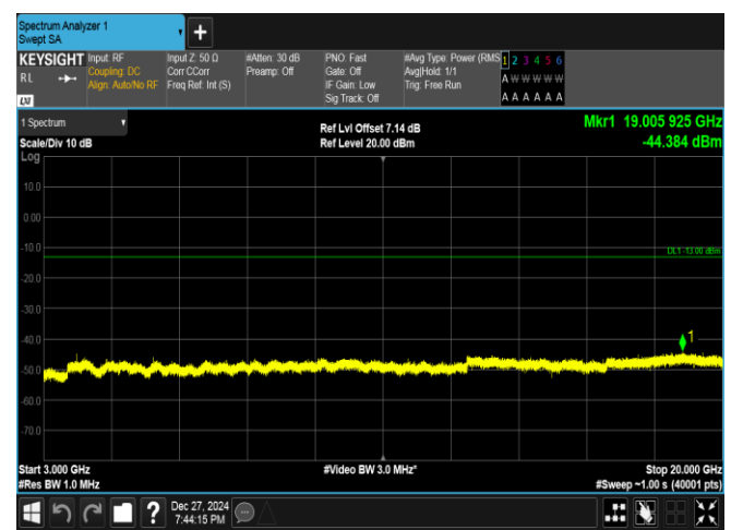
Band25-1.4MHz-QPSK-26683-1RB#5-3000~20000-PASS
