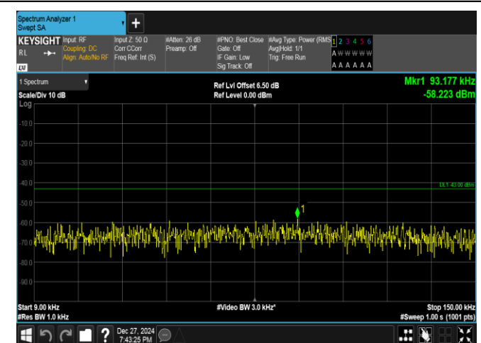
Band25-1.4MHz-QPSK-26683-1RB#5-0.009~0.15-PASS
