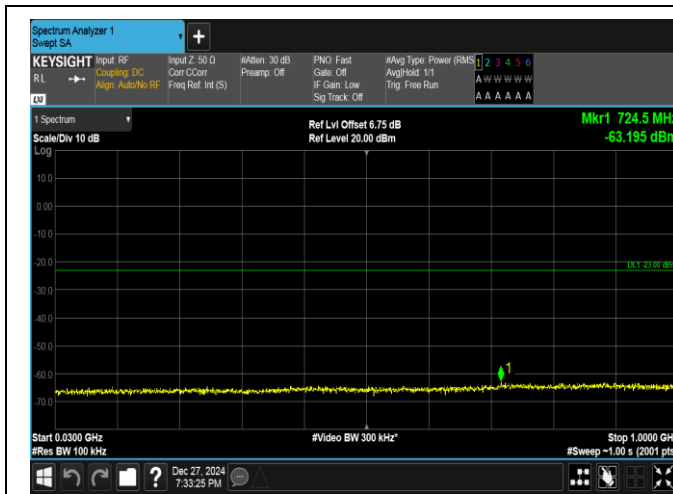
Band25-1.4MHz-QPSK-26047-6RB#0-30~1000-PASS
