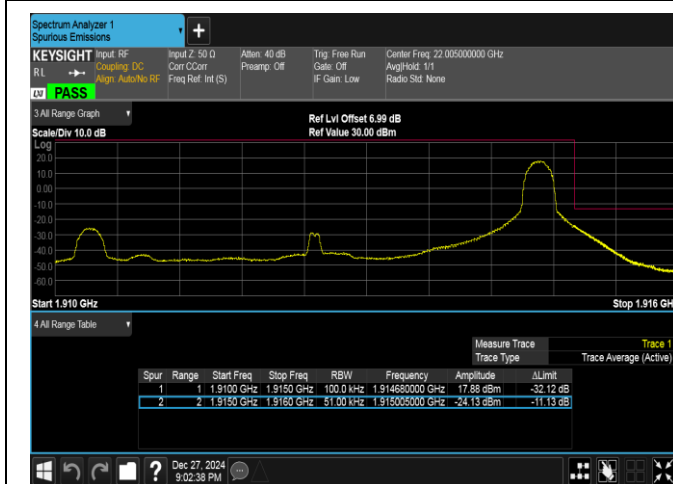
Band25-5MHz-16QAM-26665-1RB#24-PASS
