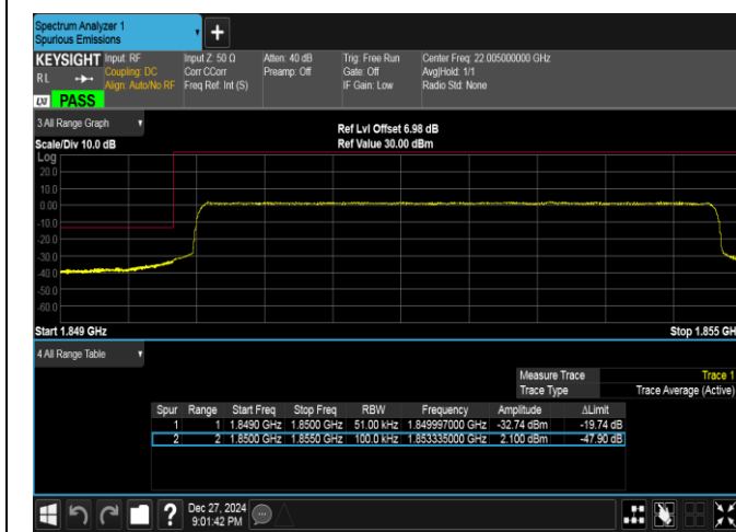
Band25-5MHz-16QAM-26065-25RB#0-PASS
