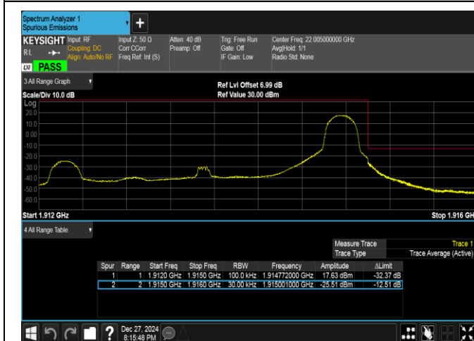
Band25-3MHz-16QAM-26675-1RB#14-PASS
