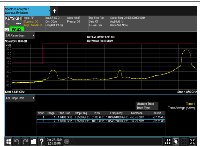
Band25-5MHz-16QAM-26065-1RB#24-PASS
