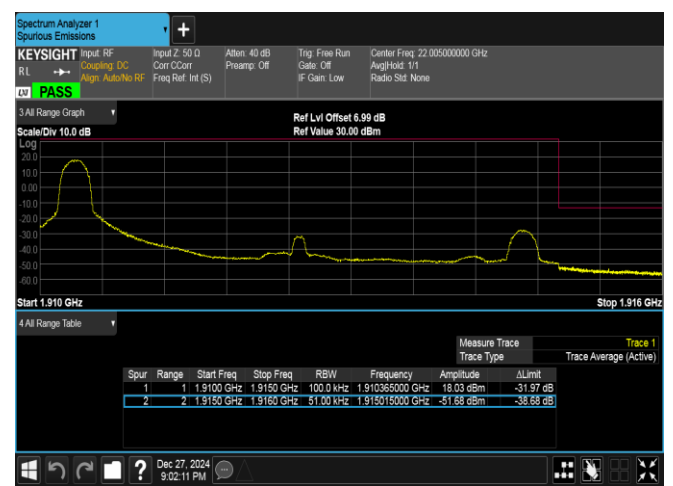
Band25-5MHz-16QAM-26665-1RB#0-PASS
