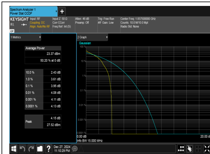
Band25-15MHz-QPSK-26115-1RB#0-PASS
