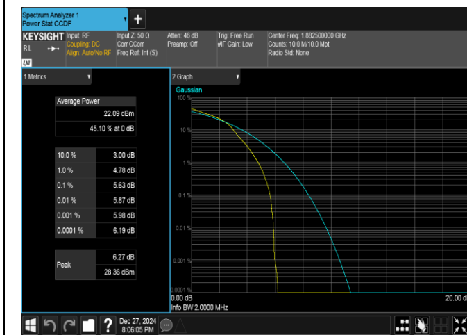
Band25-1.4MHz-16QAM-26365-1RB#0-PASS
