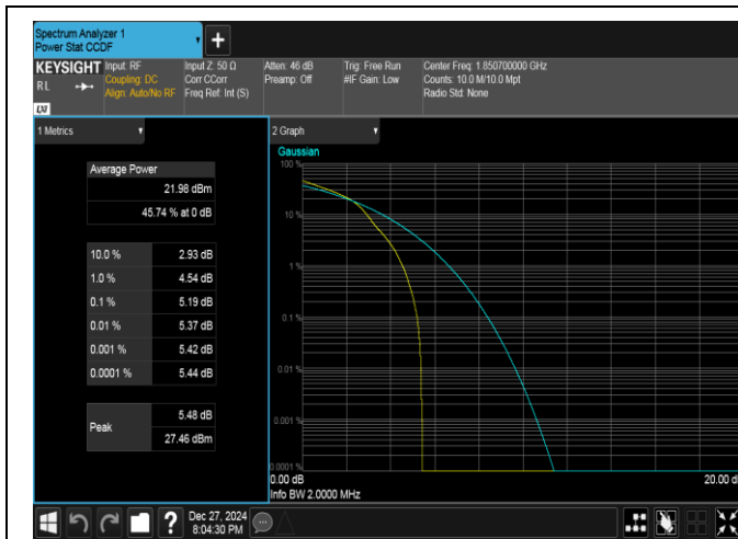
Band25-1.4MHz-16QAM-26047-1RB#0-PASS
