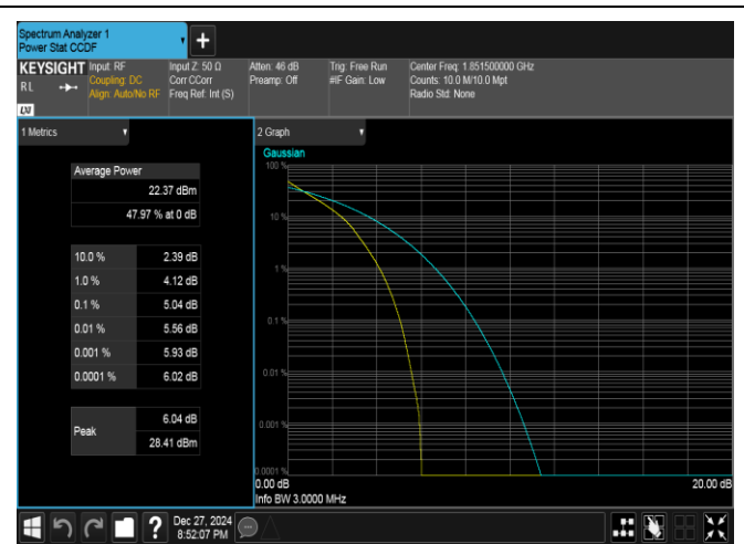
Band25-3MHz-QPSK-26055-15RB#0-PASS
