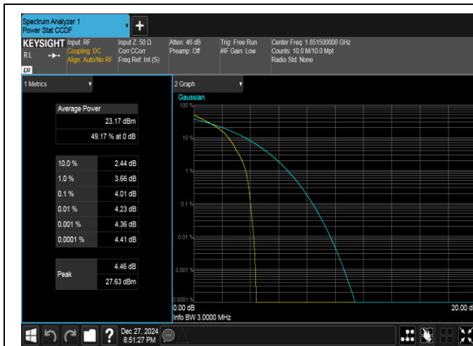
Band25-3MHz-QPSK-26055-1RB#0-PASS
