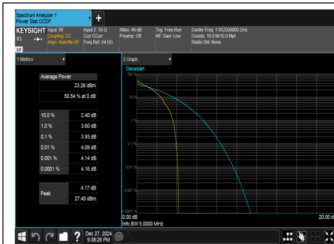
Band25-5MHz-QPSK-26065-1RB#0-PASS
