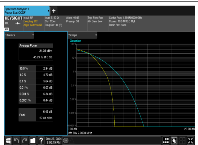
Band25-1.4MHz-16QAM-26047-6RB#0-PASS
