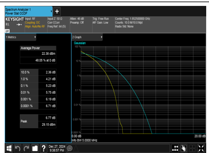
Band25-5MHz-QPSK-26065-25RB#0-PASS
