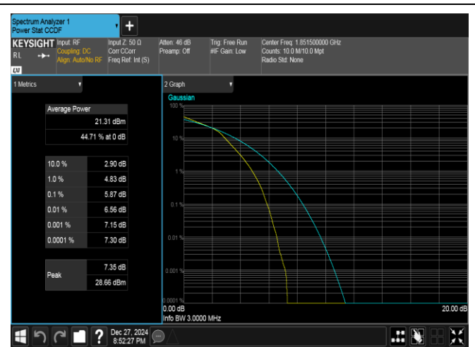
Band25-3MHz-16QAM-26055-15RB#0-PASS
