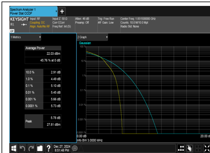
Band25-3MHz-16QAM-26055-1RB#0-PASS
