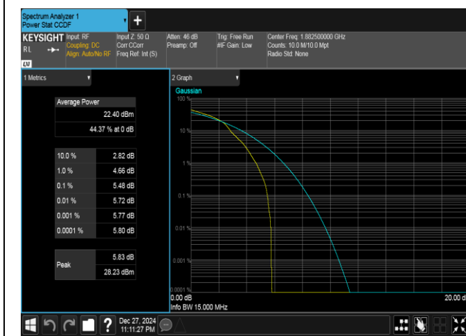
Band25-15MHz-16QAM-26365-1RB#0-PASS
