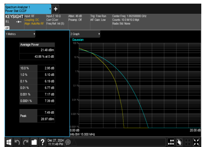
Band25-15MHz-16QAM-26365-75RB#0-PASS
