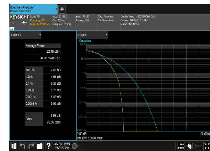
Band25-3MHz-16QAM-26365-1RB#0-PASS
