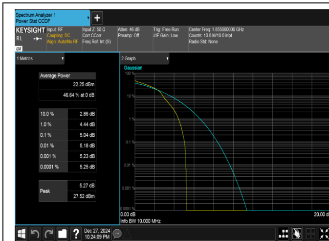
Band25-10MHz-16QAM-26090-1RB#0-PASS
