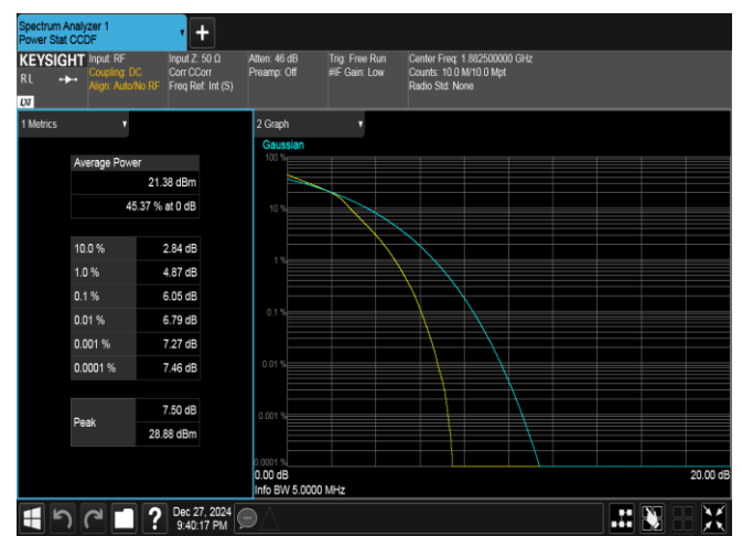
Band25-5MHz-16QAM-26365-25RB#0-PASS
