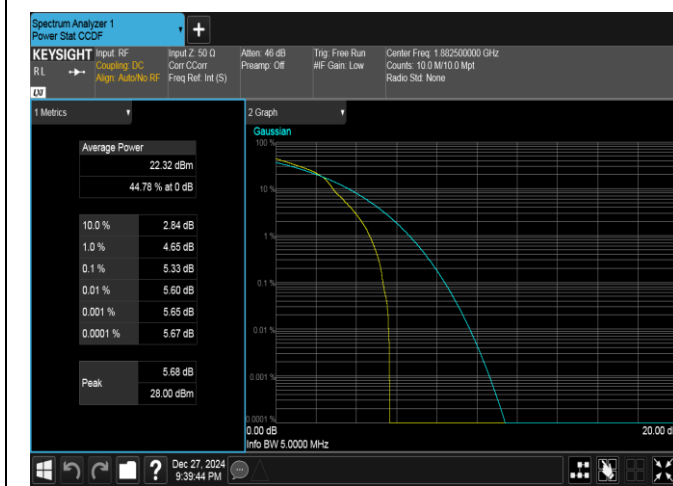
Band25-5MHz-16QAM-26365-1RB#0-PASS
