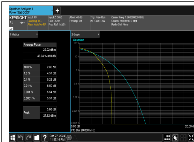
Band25-20MHz-16QAM-26140-1RB#0-PASS
