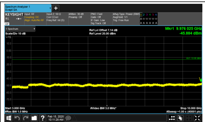
Band17-10MHz-16QAM-23780-1RB#0-3000~10000-PASS
