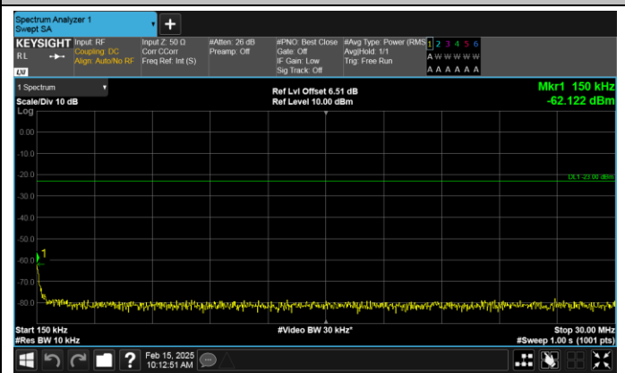
Band17-10MHz-16QAM-23780-1RB#49-0.15~30-PASS
