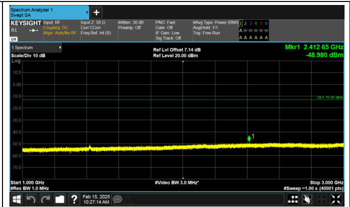
Band17-10MHz-QPSK-23800-50RB#0-1000~3000-PASS
