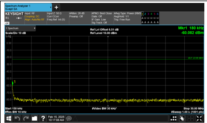
Band17-10MHz-16QAM-23790-1RB#0-0.15~30-PASS
