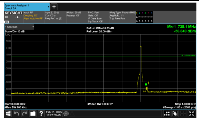
Band17-10MHz-16QAM-23800-50RB#0-30~1000-PASS
