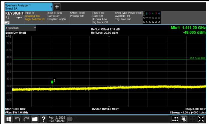
Band17-10MHz-16QAM-23790-1RB#0-1000~3000-PASS
