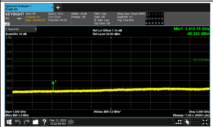
Band17-10MHz-QPSK-23800-1RB#0-1000~3000-PASS
