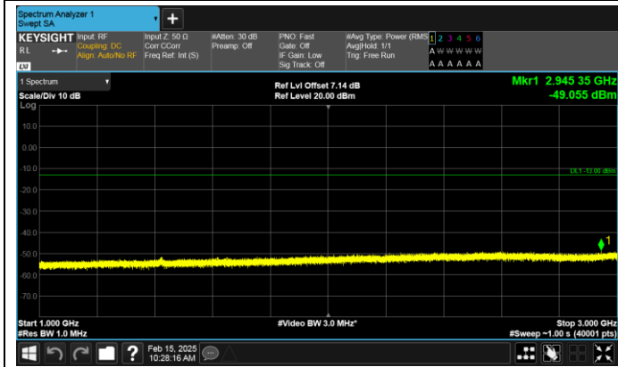
Band17-10MHz-16QAM-23800-50RB#0-1000~3000-PASS
