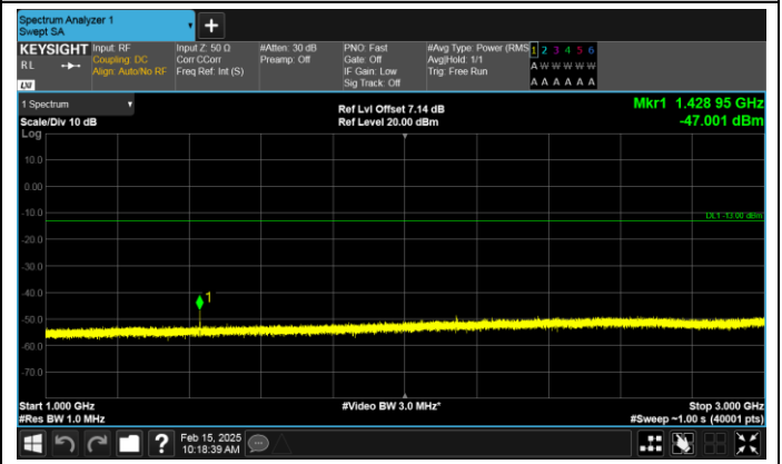
Band17-10MHz-QPSK-23790-1RB#49-1000~3000-PASS
