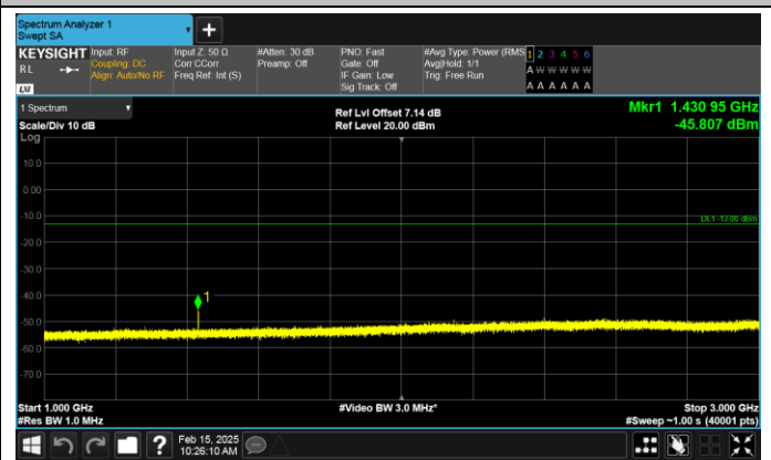
Band17-10MHz-16QAM-23800-1RB#49-1000~3000-PASS
