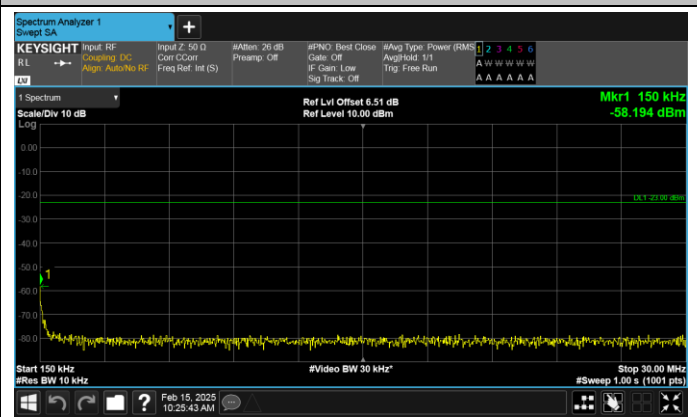
Band17-10MHz-16QAM-23800-1RB#49-0.15~30-PASS
