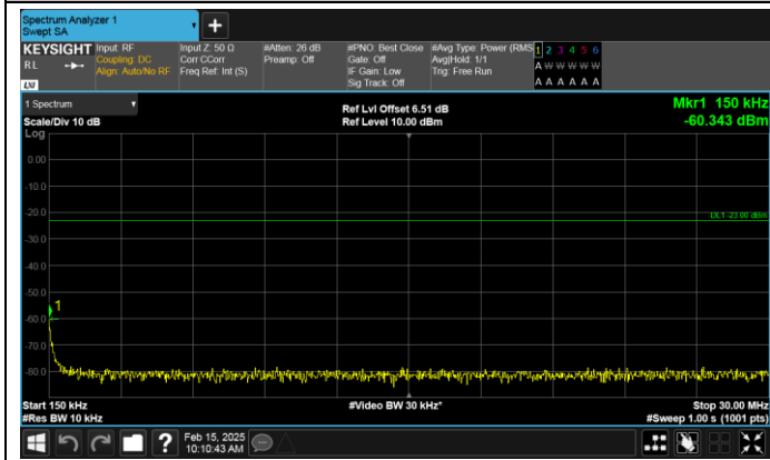
Band17-10MHz-16QAM-23780-1RB#0-0.15~30-PASS
