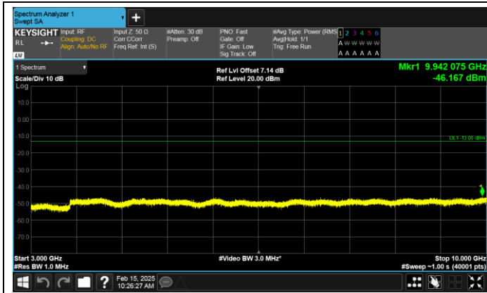
Band17-10MHz-16QAM-23800-1RB#49-3000~10000-PAS S
