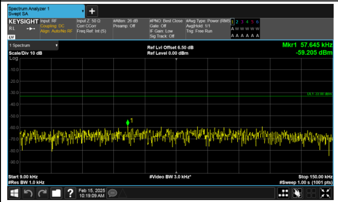
Band17-10MHz-16QAM-23790-1RB#49-0.009~0.15-PASS
