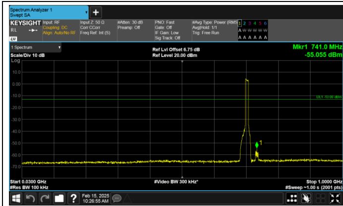
Band17-10MHz-QPSK-23800-50RB#0-30~1000-PASS
