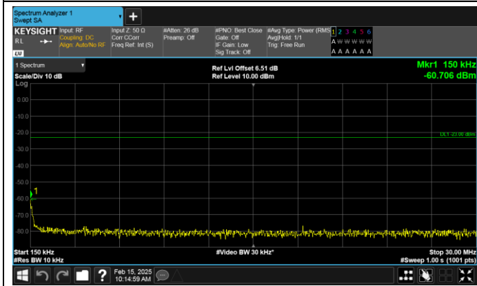
Band17-10MHz-16QAM-23780-50RB#0-0.15~30-PASS
