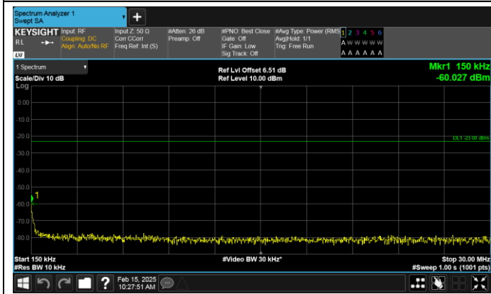
Band17-10MHz-16QAM-23800-50RB#0-0.15~30-PASS
