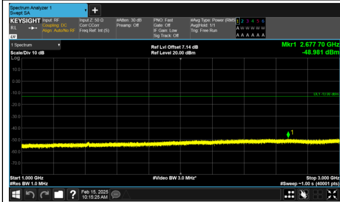
Band17-10MHz-16QAM-23780-50RB#0-1000~3000-PASS
