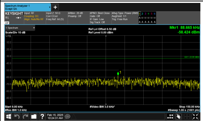
Band17-10MHz-QPSK-23800-1RB#49-0.009~0.15-PASS
