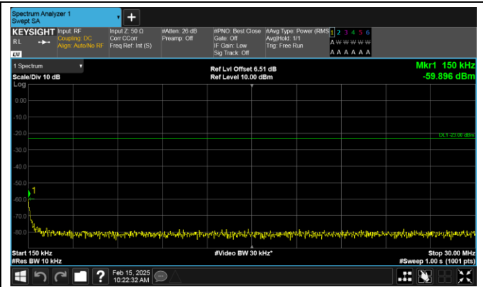
Band17-10MHz-QPSK-23800-1RB#0-0.15~30-PASS
