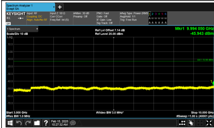
Band17-10MHz-QPSK-23800-50RB#0-3000~10000-PASS
