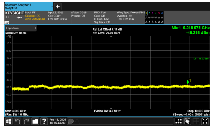
Band17-10MHz-16QAM-23780-50RB#0-3000~10000-PAS S
