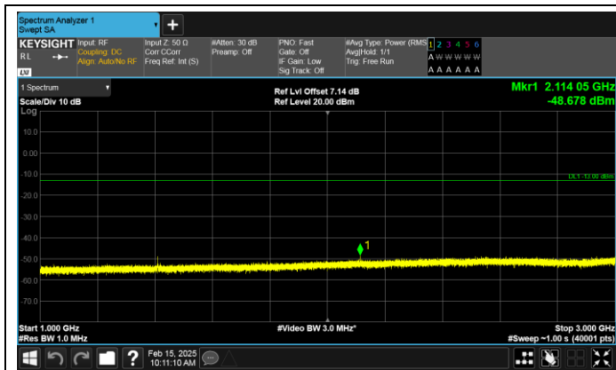
Band17-10MHz-16QAM-23780-1RB#0-1000~3000-PASS
