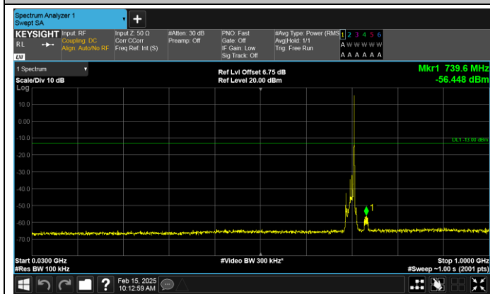
Band17-10MHz-16QAM-23780-1RB#49-30~1000-PASS
