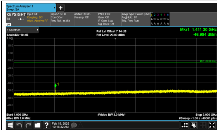
Band17-10MHz-QPSK-23790-1RB#0-1000~3000-PASS
