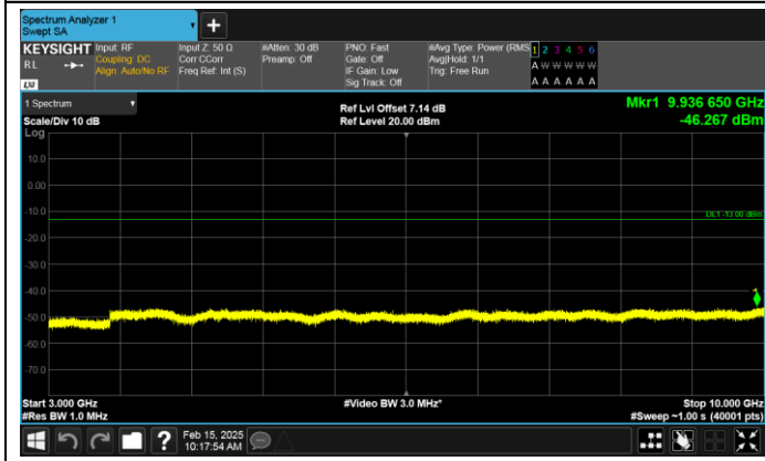
Band17-10MHz-16QAM-23790-1RB#0-3000~10000-PASS
