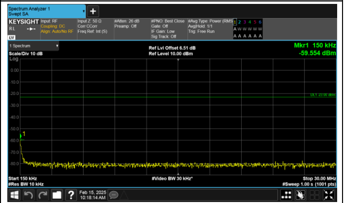
Band17-10MHz-QPSK-23790-1RB#49-0.15~30-PASS
