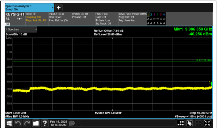
Band17-10MHz-QPSK-23790-1RB#0-3000~10000-PASS
