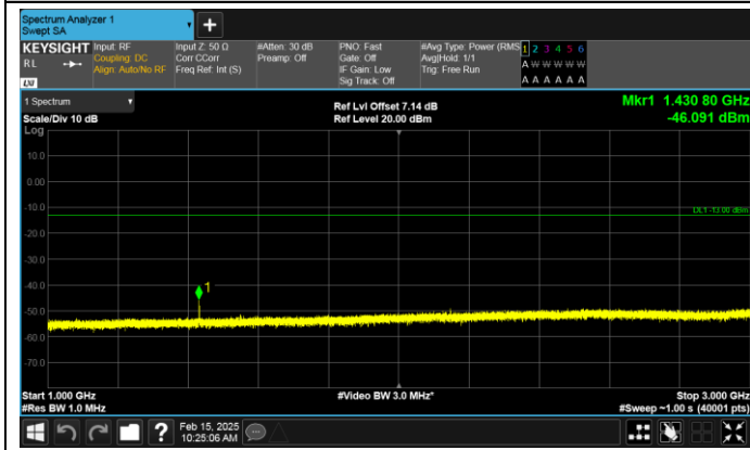
Band17-10MHz-QPSK-23800-1RB#49-1000~3000-PASS
