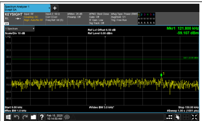
Band17-10MHz-16QAM-23780-50RB#0-0.009~0.15-PASS
