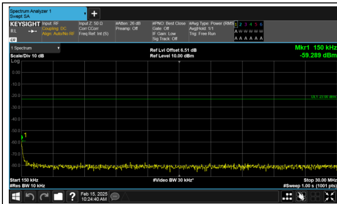
Band17-10MHz-QPSK-23800-1RB#49-0.15~30-PASS
