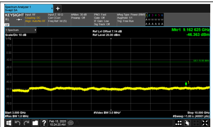
Band17-10MHz-16QAM-23800-1RB#0-3000~10000-PASS
