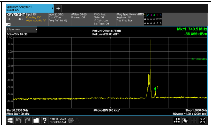
Band17-10MHz-QPSK-23800-1RB#49-30~1000-PASS
