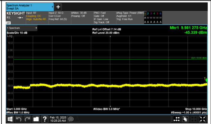
Band17-10MHz-QPSK-23800-1RB#49-3000~10000-PASS
