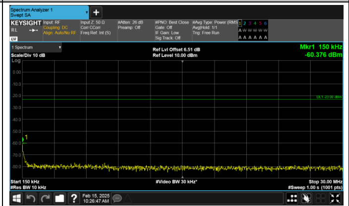
Band17-10MHz-QPSK-23800-50RB#0-0.15~30-PASS
