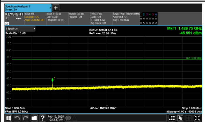
Band17-10MHz-16QAM-23780-1RB#49-1000~3000-PASS
