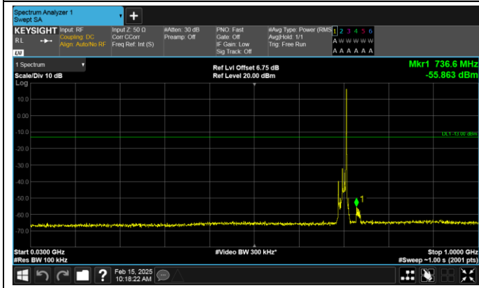
Band17-10MHz-QPSK-23790-1RB#49-30~1000-PASS
