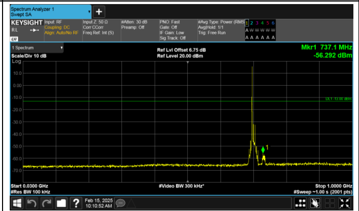
Band17-10MHz-16QAM-23780-1RB#0-30~1000-PASS
