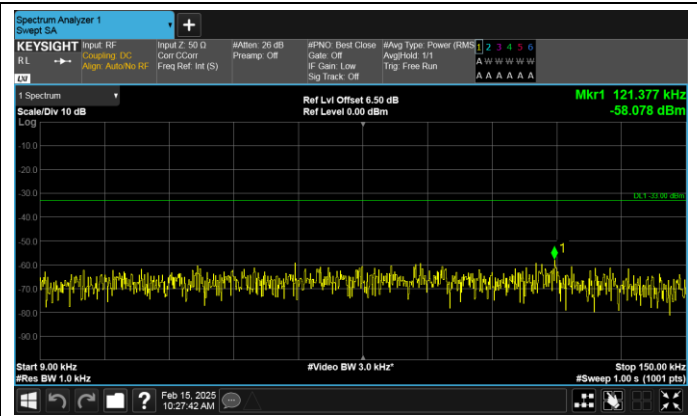
Band17-10MHz-16QAM-23800-50RB#0-0.009~0.15-PASS
