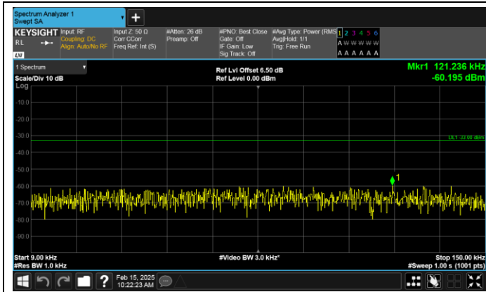
Band17-10MHz-QPSK-23800-1RB#0-0.009~0.15-PASS
