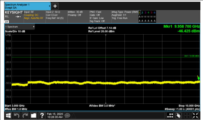
Band17-10MHz-16QAM-23800-50RB#0-3000~10000-PAS S
