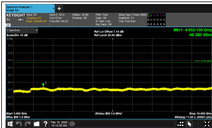
Band17-10MHz-16QAM-23780-1RB#49-3000~10000-PAS S
