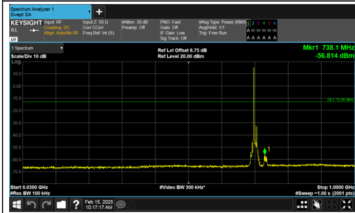
Band17-10MHz-16QAM-23790-1RB#0-30~1000-PASS
