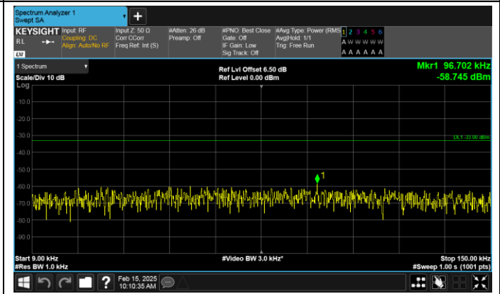
Band17-10MHz-16QAM-23780-1RB#0-0.009~0.15-PASS
