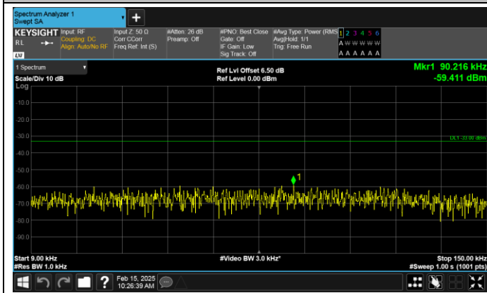
Band17-10MHz-QPSK-23800-50RB#0-0.009~0.15-PASS
