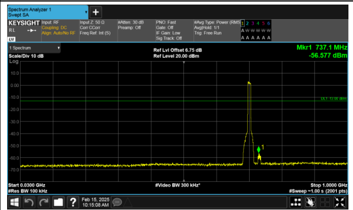
Band17-10MHz-16QAM-23780-50RB#0-30~1000-PASS
