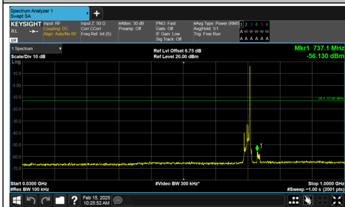
Band17-10MHz-16QAM-23800-1RB#49-30~1000-PASS
