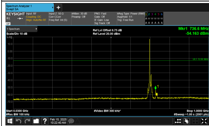
Band17-10MHz-QPSK-23800-1RB#0-30~1000-PASS
