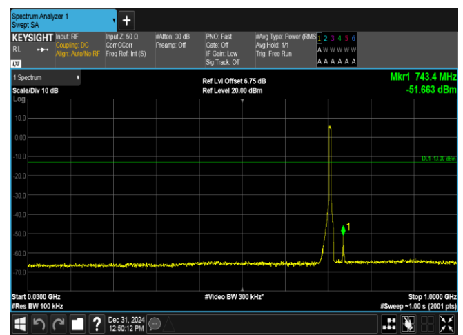
Band17-5MHz-16QAM-23825-25RB#0-30~1000-PASS
