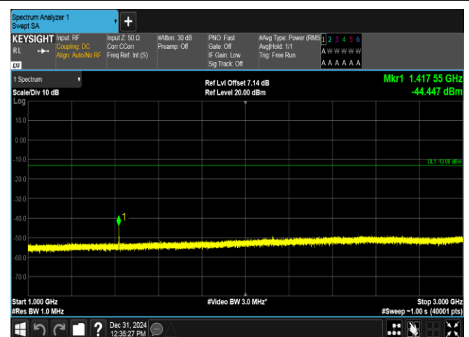
Band17-5MHz-16QAM-23755-1RB#24-1000~3000-PASS
