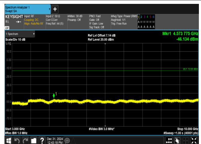
Band17-5MHz-QPSK-23790-25RB#0-3000~10000-PASS
