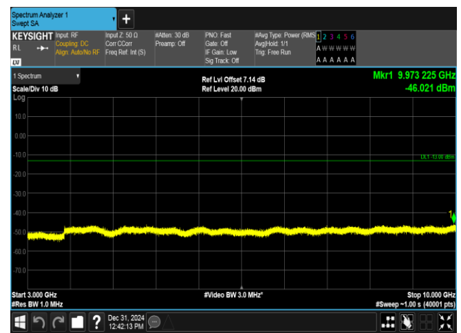
Band17-5MHz-16QAM-23790-1RB#24-3000~10000-PASS
