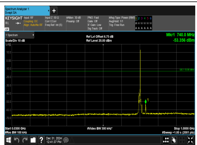
Band17-5MHz-16QAM-23790-1RB#24-30~1000-PASS
