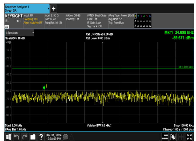
Band17-5MHz-QPSK-23790-1RB#0-0.009~0.15-PASS
