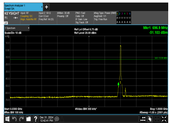
Band17-5MHz-QPSK-23790-25RB#0-30~1000-PASS
