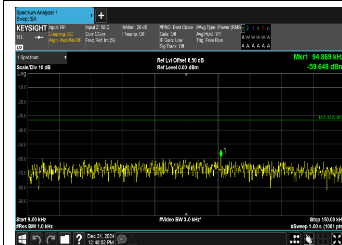
Band17-5MHz-QPSK-23825-25RB#0-0.009~0.15-PASS
