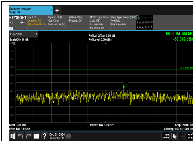
Band17-5MHz-16QAM-23790-1RB#0-0.009~0.15-PASS
