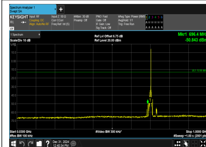
Band17-5MHz-QPSK-23790-1RB#24-30~1000-PASS
