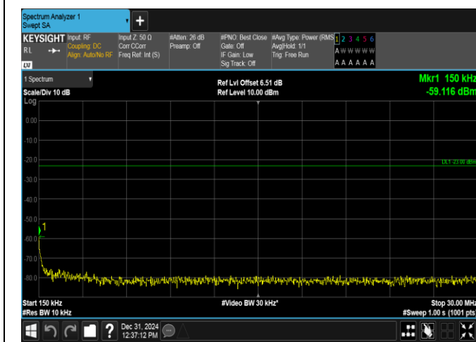
Band17-5MHz-16QAM-23755-25RB#0-0.15~30-PASS
