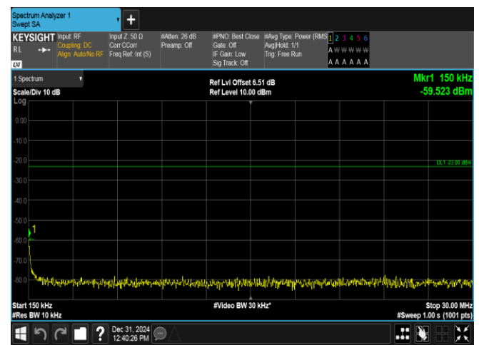
Band17-5MHz-QPSK-23790-1RB#24-0.15~30-PASS
