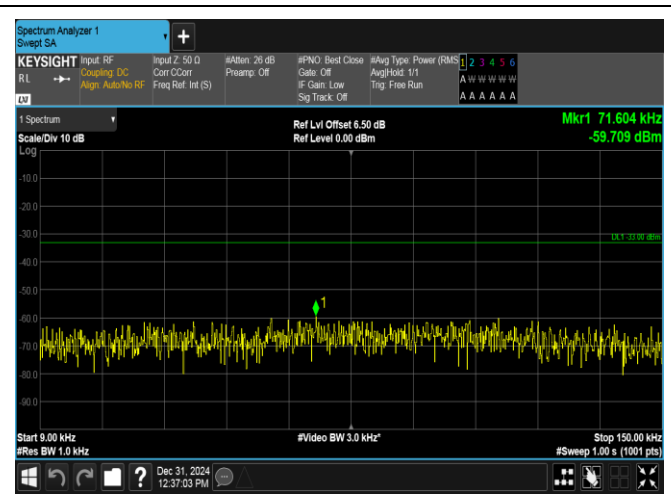
Band17-5MHz-16QAM-23755-25RB#0-0.009~0.15-PASS
