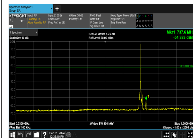
Band17-5MHz-16QAM-23755-1RB#24-30~1000-PASS
