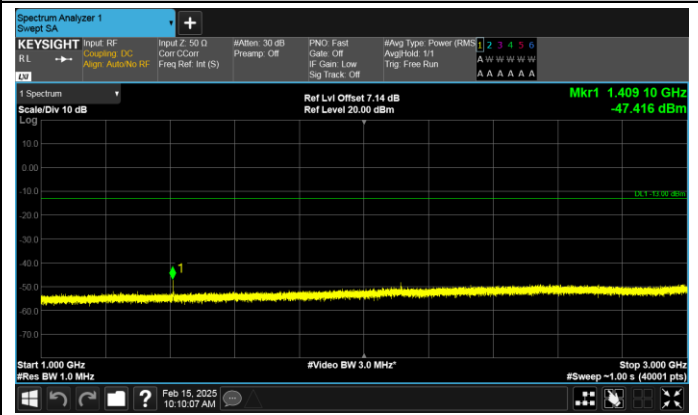
Band17-10MHz-QPSK-23780-1RB#0-1000~3000-PASS
