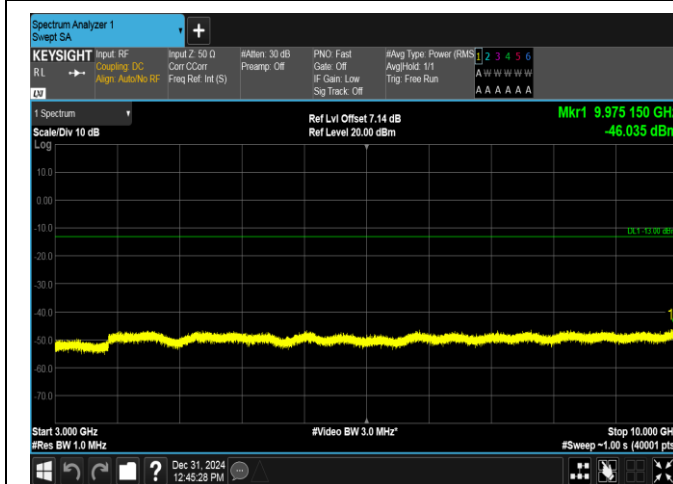
Band17-5MHz-QPSK-23825-1RB#0-3000~10000-PASS
