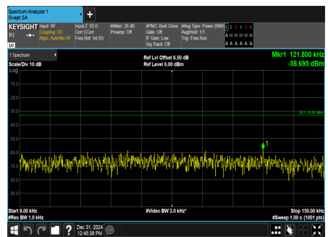
Band17-5MHz-16QAM-23825-1RB#0-0.009~0.15-PASS
