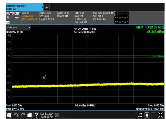
Band17-5MHz-QPSK-23825-1RB#0-1000~3000-PASS
