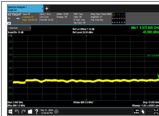
Band17-5MHz-16QAM-23755-1RB#24-3000~10000-PASS
