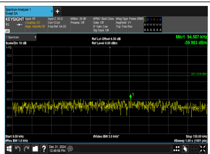
Band17-5MHz-16QAM-23825-25RB#0-0.009~0.15-PASS
