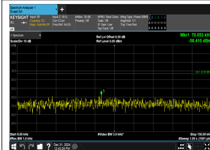
Band17-5MHz-16QAM-23790-25RB#0-0.009~0.15-PASS
