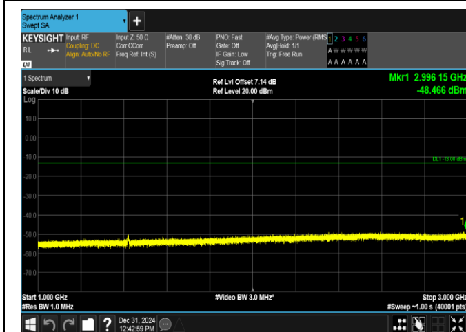
Band17-5MHz-QPSK-23790-25RB#0-1000~3000-PASS
