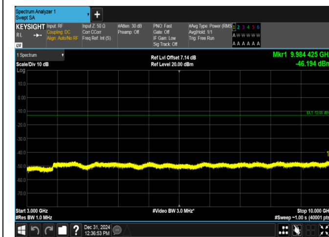
Band17-5MHz-QPSK-23755-25RB#0-3000~10000-PASS
