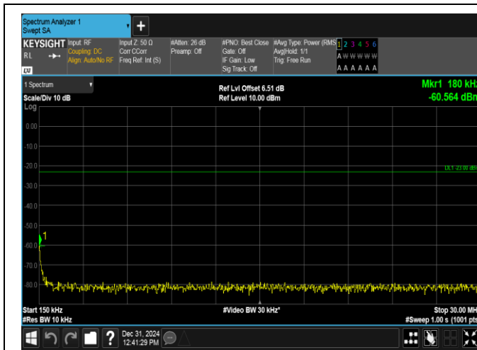
Band17-5MHz-16QAM-23790-1RB#24-0.15~30-PASS
