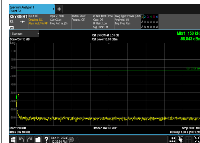
Band17-5MHz-16QAM-23755-1RB#0-0.15~30-PASS
