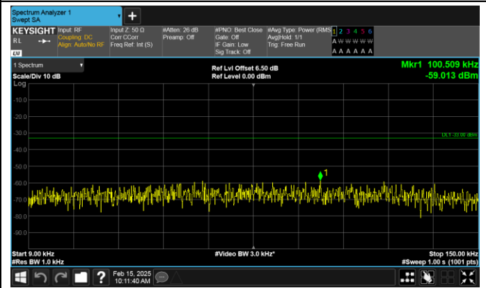
Band17-10MHz-QPSK-23780-1RB#49-0.009~0.15-PASS
