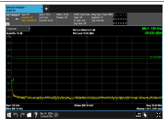
Band17-5MHz-QPSK-23825-1RB#0-0.15~30-PASS
