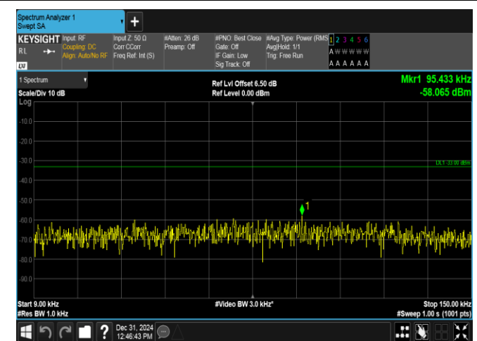
Band17-5MHz-QPSK-23825-1RB#24-0.009~0.15-PASS
