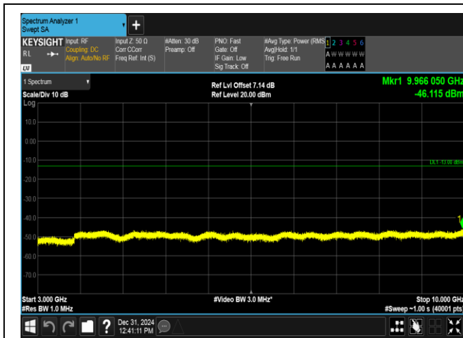
Band17-5MHz-QPSK-23790-1RB#24-3000~10000-PASS
