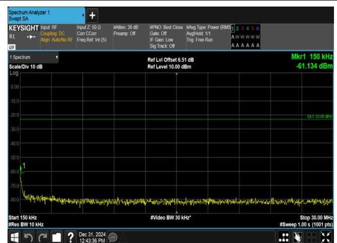
Band17-5MHz-16QAM-23790-25RB#0-0.15~30-PASS
