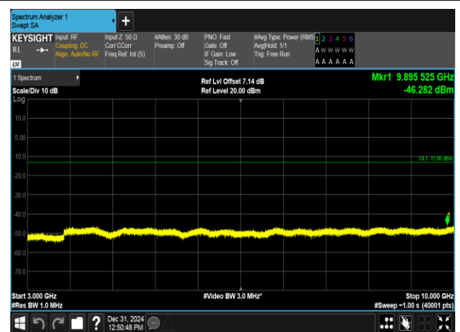
Band17-5MHz-16QAM-23825-25RB#0-3000~10000-PASS
