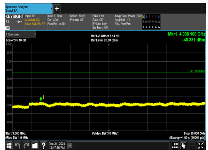
Band17-5MHz-QPSK-23825-1RB#24-3000~10000-PASS
