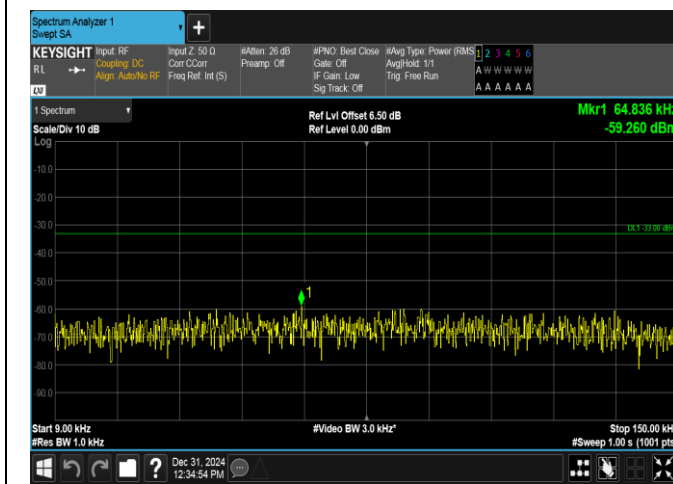
Band17-5MHz-16QAM-23755-1RB#24-0.009~0.15-PASS
