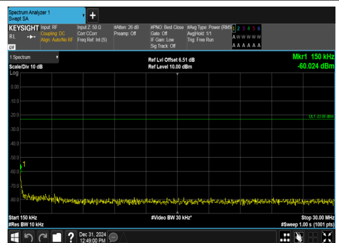
Band17-5MHz-QPSK-23825-25RB#0-0.15~30-PASS
