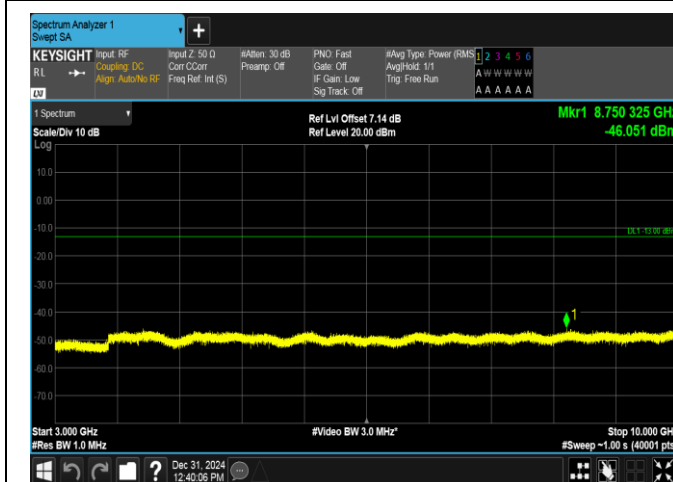
Band17-5MHz-16QAM-23790-1RB#0-3000~10000-PASS
