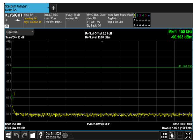
Band17-5MHz-16QAM-23755-1RB#24-0.15~30-PASS
