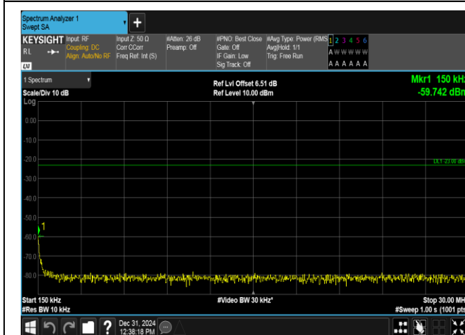
Band17-5MHz-QPSK-23790-1RB#0-0.15~30-PASS
