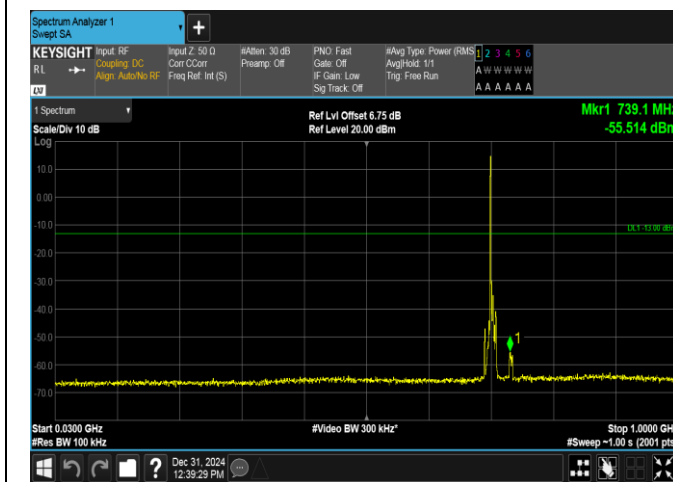
Band17-5MHz-16QAM-23790-1RB#0-30~1000-PASS
