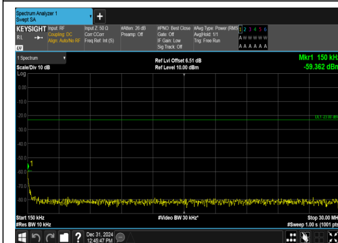
Band17-5MHz-16QAM-23825-1RB#0-0.15~30-PASS
