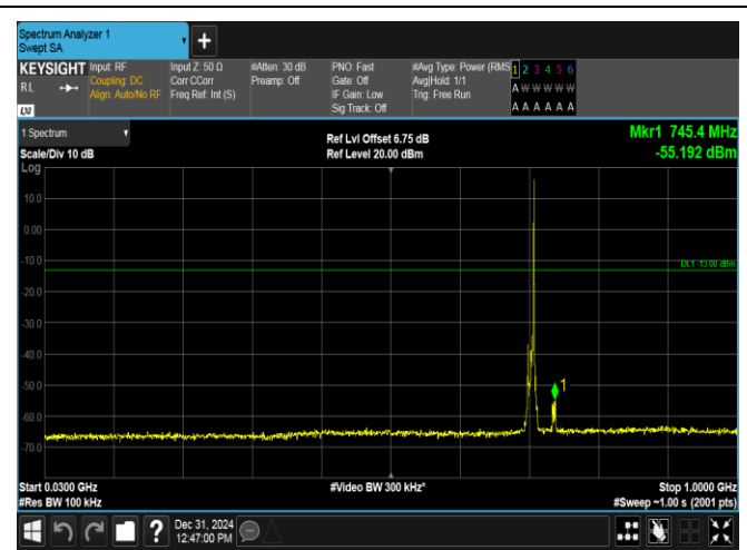
Band17-5MHz-QPSK-23825-1RB#24-30~1000-PASS
