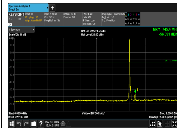
Band17-5MHz-QPSK-23825-1RB#0-30~1000-PASS
