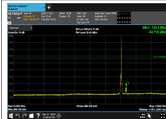
Band17-5MHz-16QAM-23825-1RB#24-30~1000-PASS
