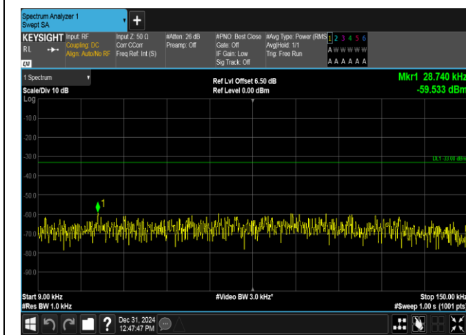
Band17-5MHz-16QAM-23825-1RB#24-0.009~0.15-PASS
