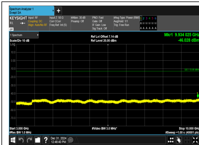
Band17-5MHz-16QAM-23825-1RB#24-3000~10000-PASS
