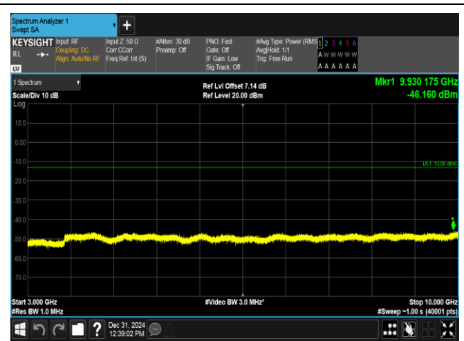
Band17-5MHz-QPSK-23790-1RB#0-3000~10000-PASS
