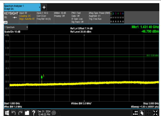
Band17-5MHz-16QAM-23825-1RB#24-1000~3000-PASS
