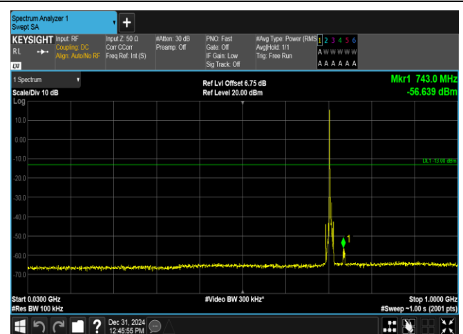
Band17-5MHz-16QAM-23825-1RB#0-30~1000-PASS
