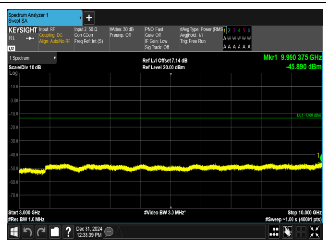
Band17-5MHz-16QAM-23755-1RB#0-3000~10000-PASS
