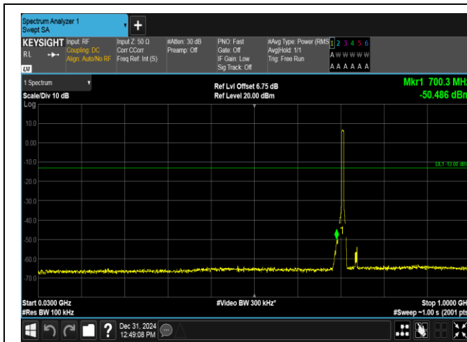
Band17-5MHz-QPSK-23825-25RB#0-30~1000-PASS
