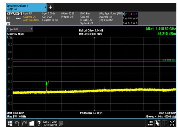
Band17-5MHz-16QAM-23790-1RB#0-1000~3000-PASS
