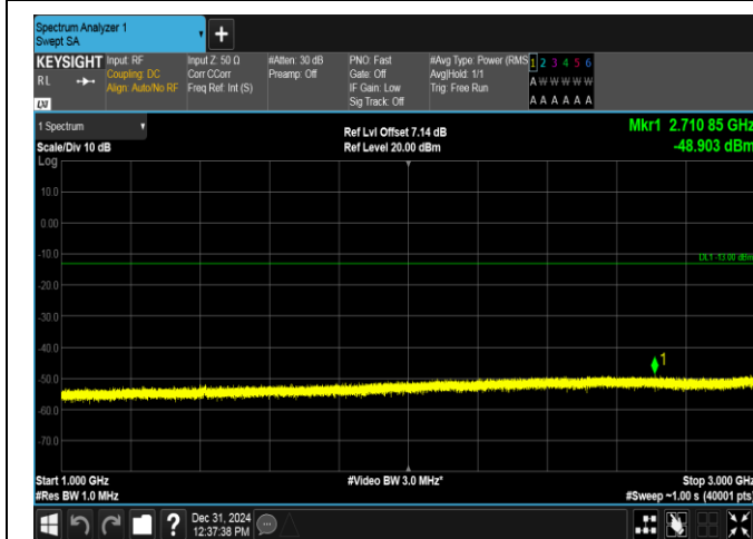
Band17-5MHz-16QAM-23755-25RB#0-1000~3000-PASS
