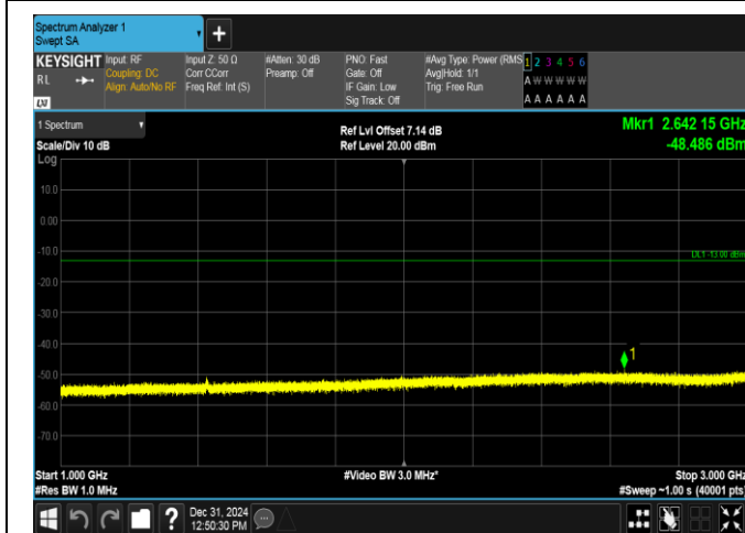
Band17-5MHz-16QAM-23825-25RB#0-1000~3000-PASS
