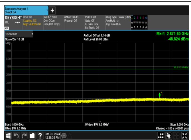
Band17-5MHz-QPSK-23755-25RB#0-1000~3000-PASS
