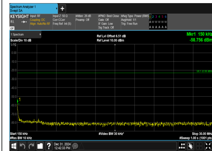
Band17-5MHz-QPSK-23790-25RB#0-0.15~30-PASS
