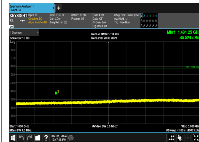
Band17-5MHz-QPSK-23825-1RB#24-1000~3000-PASS
