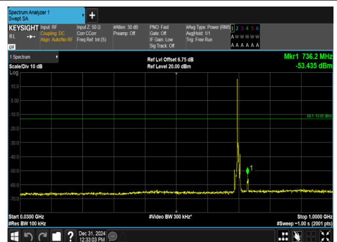
Band17-5MHz-16QAM-23755-1RB#0-30~1000-PASS
