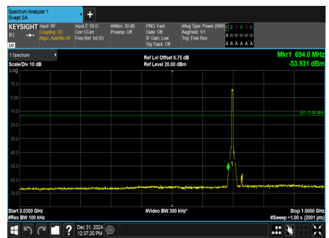
Band17-5MHz-16QAM-23755-25RB#0-30~1000-PASS
