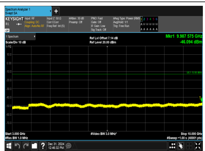
Band17-5MHz-16QAM-23825-1RB#0-3000~10000-PASS
