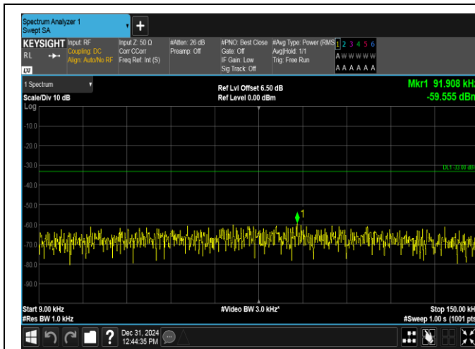
Band17-5MHz-QPSK-23825-1RB#0-0.009~0.15-PASS
