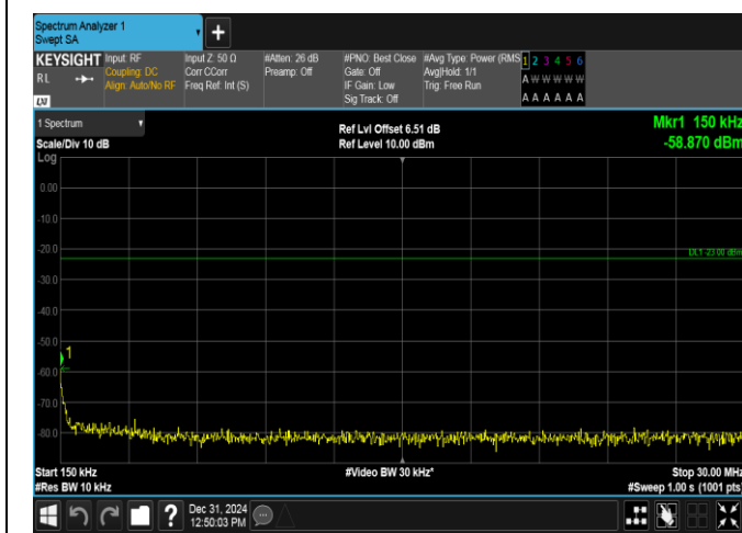
Band17-5MHz-16QAM-23825-25RB#0-0.15~30-PASS
