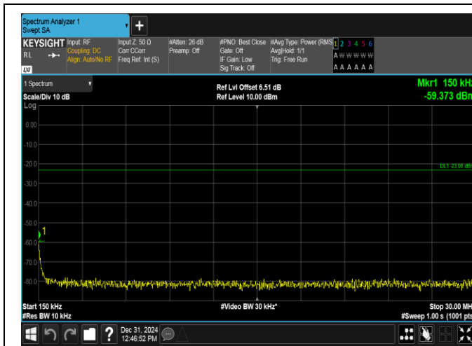
Band17-5MHz-QPSK-23825-1RB#24-0.15~30-PASS
