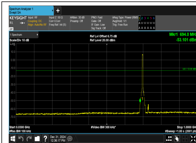
Band17-5MHz-QPSK-23755-25RB#0-30~1000-PASS
