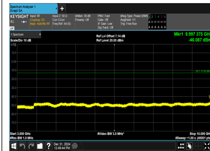
Band17-5MHz-QPSK-23825-25RB#0-3000~10000-PASS
