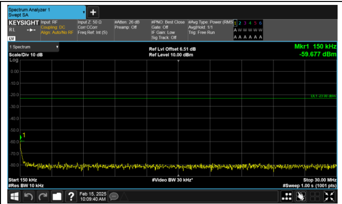
Band17-10MHz-QPSK-23780-1RB#0-0.15~30-PASS
