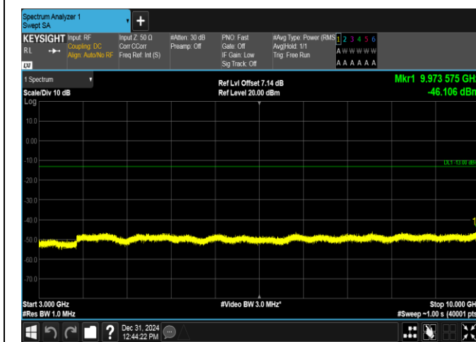
Band17-5MHz-16QAM-23790-25RB#0-3000~10000-PASS
