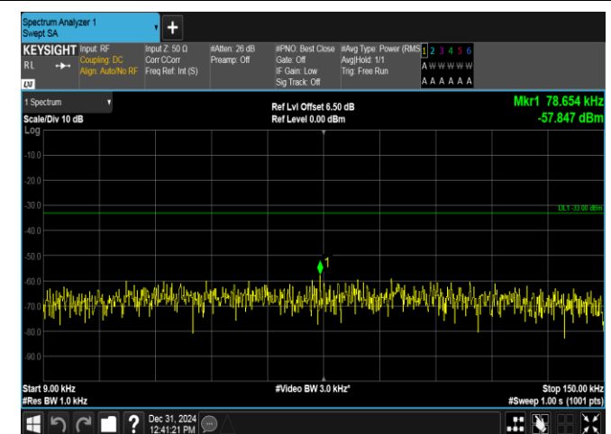
Band17-5MHz-16QAM-23790-1RB#24-0.009~0.15-PASS
