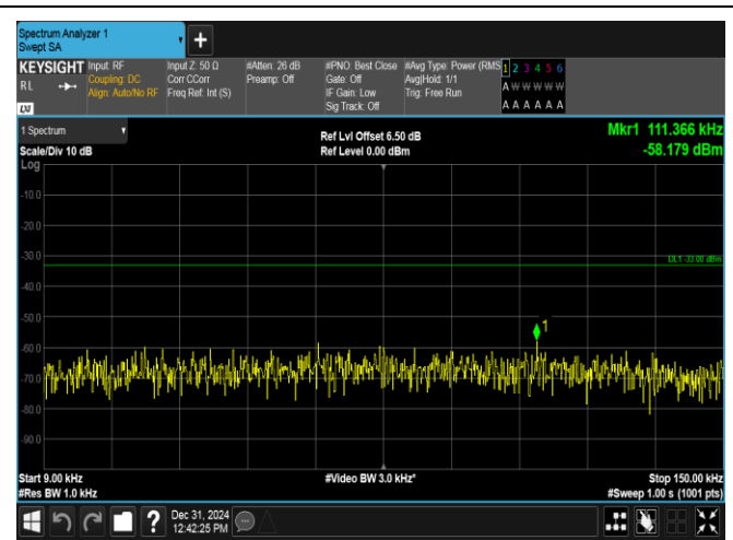
Band17-5MHz-QPSK-23790-25RB#0-0.009~0.15-PASS
