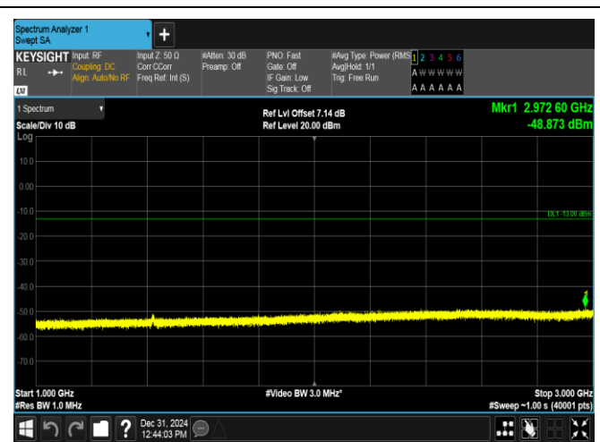
Band17-5MHz-16QAM-23790-25RB#0-1000~3000-PASS
