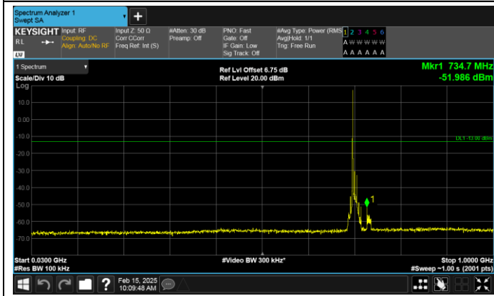
Band17-10MHz-QPSK-23780-1RB#0-30~1000-PASS
