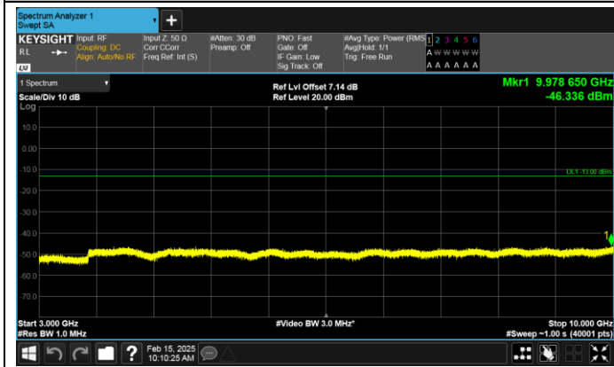
Band17-10MHz-QPSK-23780-1RB#0-3000~10000-PASS
