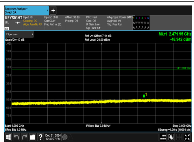
Band17-5MHz-QPSK-23825-25RB#0-1000~3000-PASS
