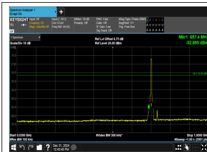
Band17-5MHz-16QAM-23790-25RB#0-30~1000-PASS
