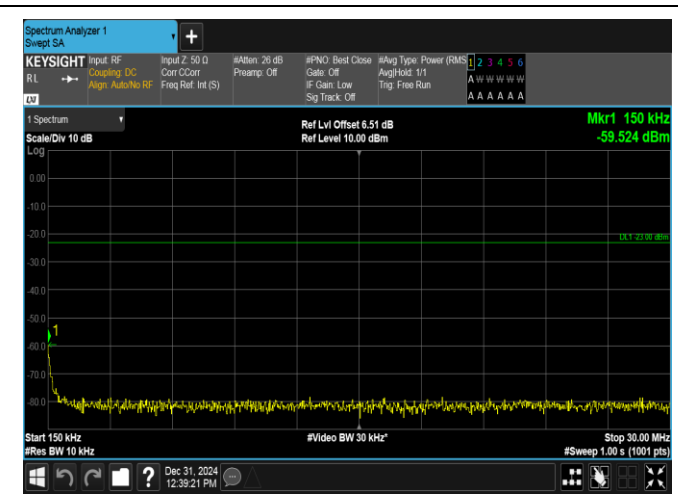
Band17-5MHz-16QAM-23790-1RB#0-0.15~30-PASS
