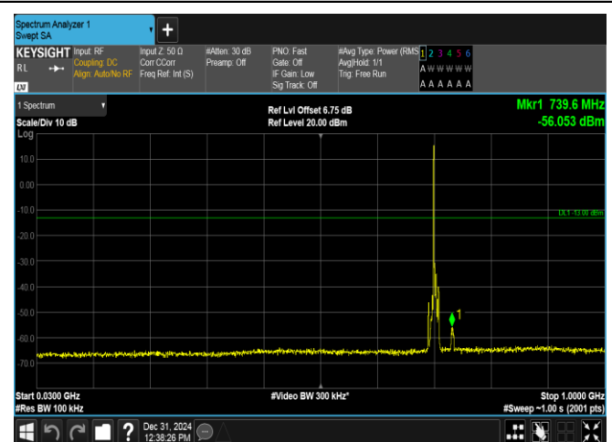
Band17-5MHz-QPSK-23790-1RB#0-30~1000-PASS
