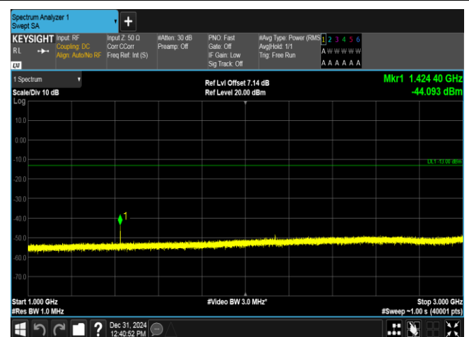
Band17-5MHz-QPSK-23790-1RB#24-1000~3000-PASS
