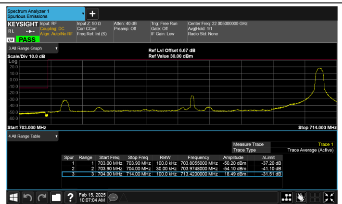
Band17-10MHz-16QAM-23780-1RB#49-PASS
