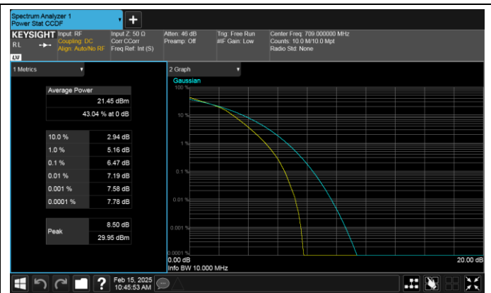
Band17-10MHz-16QAM-23780-50RB#0-PASS
