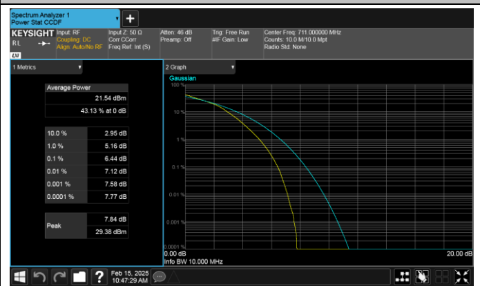
Band17-10MHz-16QAM-23800-50RB#0-PASS
