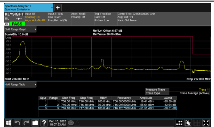
Band17-10MHz-QPSK-23800-1RB#0-PASS
