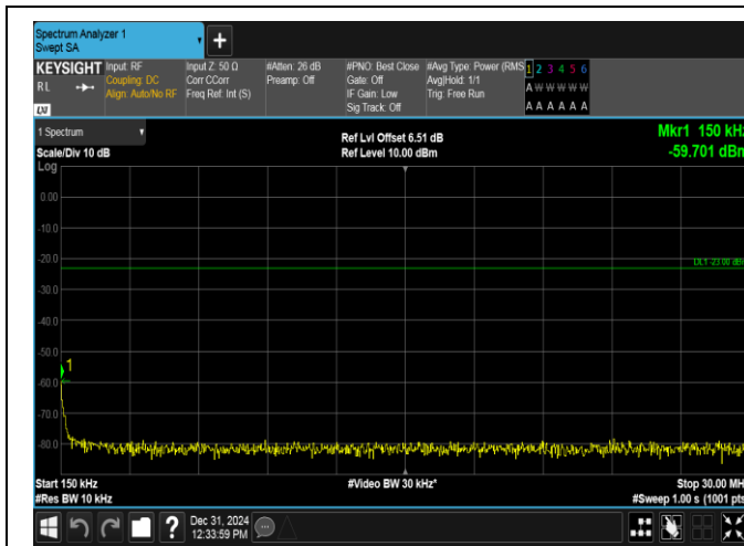
Band17-5MHz-QPSK-23755-1RB#24-0.15~30-PASS
