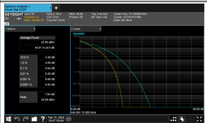
Band17-10MHz-QPSK-23800-50RB#0-PASS
