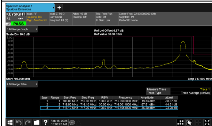
Band17-10MHz-QPSK-23800-1RB#49-PASS
