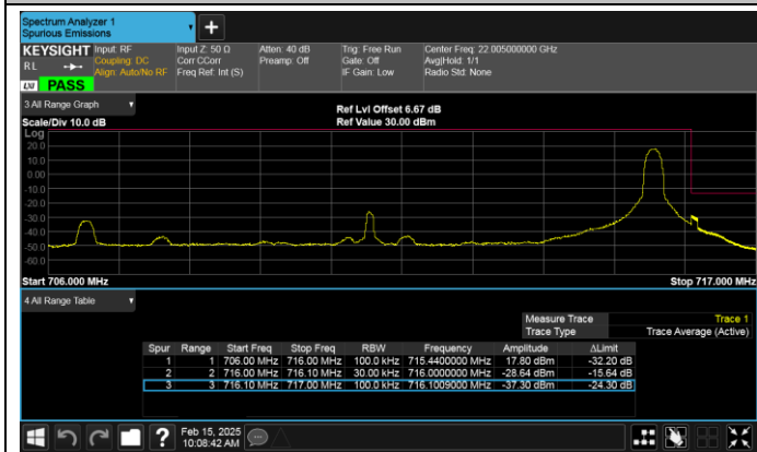
Band17-10MHz-16QAM-23800-1RB#49-PASS
