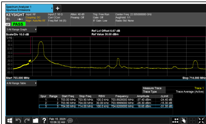
Band17-10MHz-16QAM-23780-1RB#0-PASS
