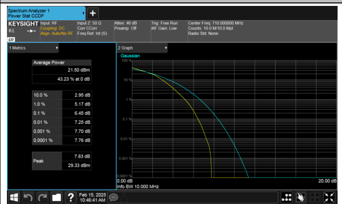
Band17-10MHz-16QAM-23790-50RB#0-PASS
