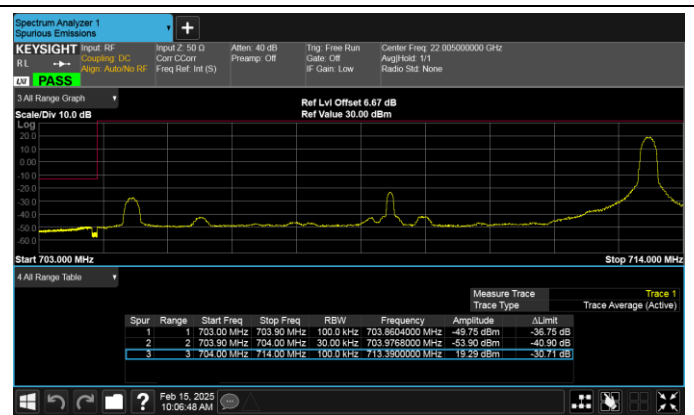
Band17-10MHz-QPSK-23780-1RB#49-PASS
