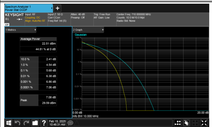
Band17-10MHz-QPSK-23790-50RB#0-PASS
