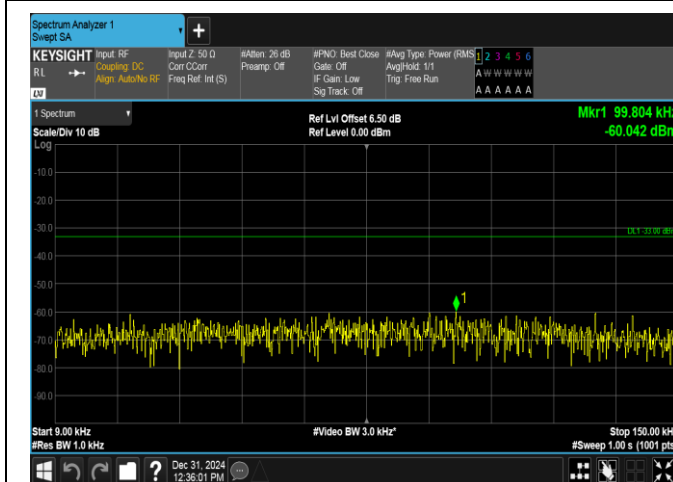
Band17-5MHz-QPSK-23755-25RB#0-0.009~0.15-PASS
