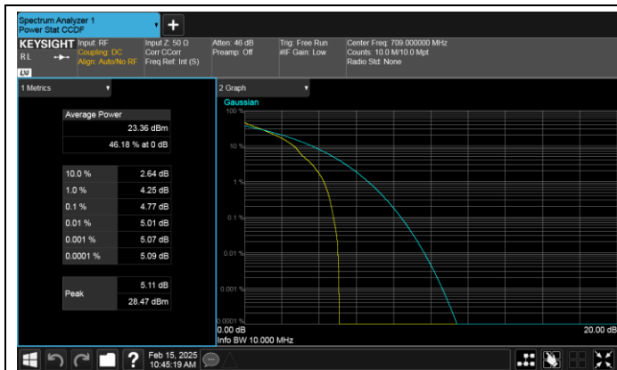
Band17-10MHz-QPSK-23780-1RB#0-PASS
