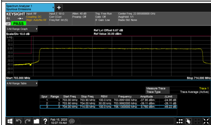
Band17-10MHz-QPSK-23780-50RB#0-PASS
