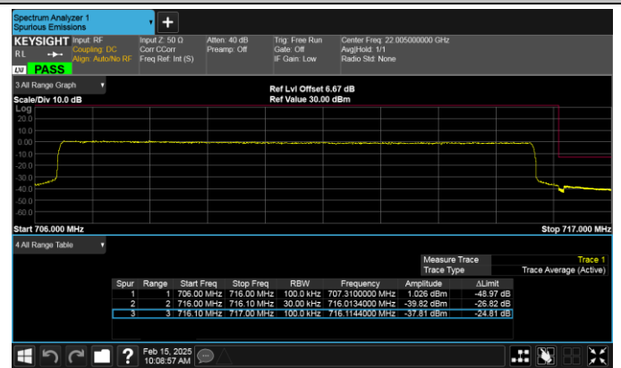
Band17-10MHz-QPSK-23800-50RB#0-PASS
