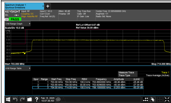
Band17-10MHz-16QAM-23780-50RB#0-PASS
