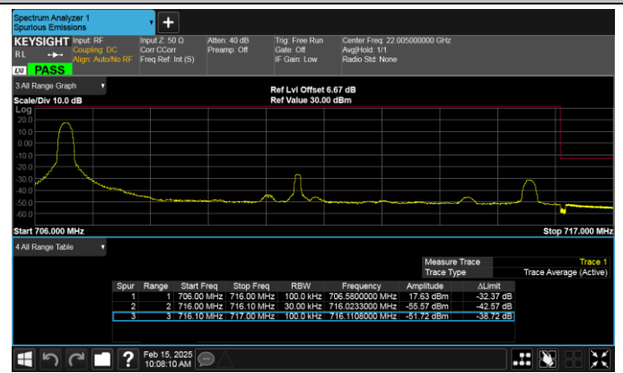
Band17-10MHz-16QAM-23800-1RB#0-PASS
