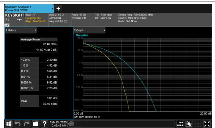
Band17-10MHz-QPSK-23780-50RB#0-PASS
