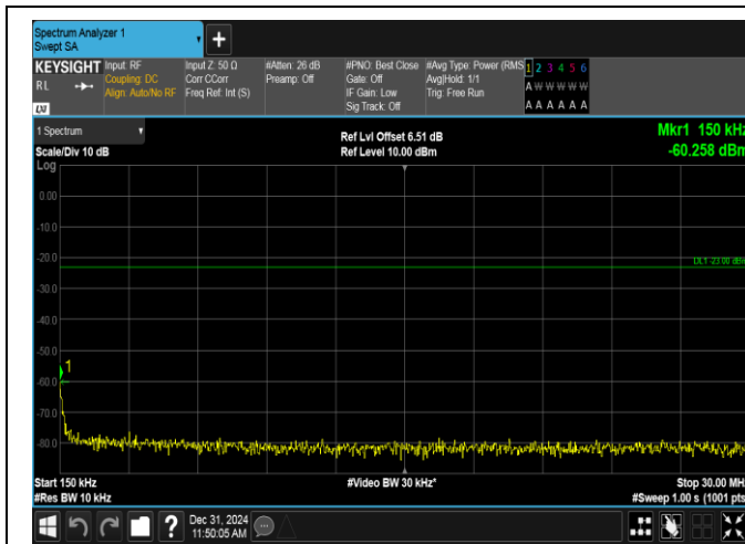
Band12-10MHz-16QAM-23060-50RB#0-0.15~30-PASS
