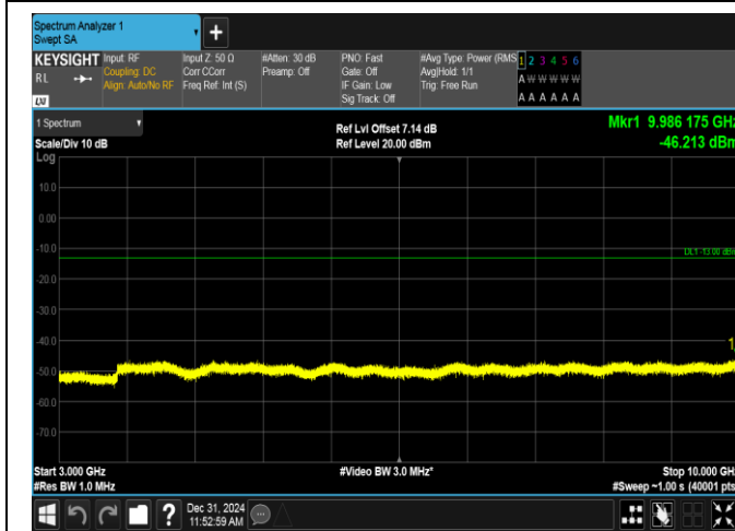
Band12-10MHz-16QAM-23095-1RB#0-3000~10000-PASS
