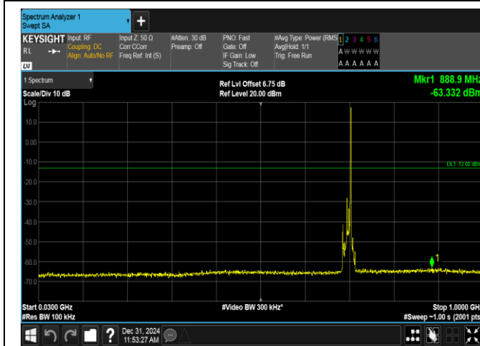
Band12-10MHz-QPSK-23095-1RB#49-30~1000-PASS
