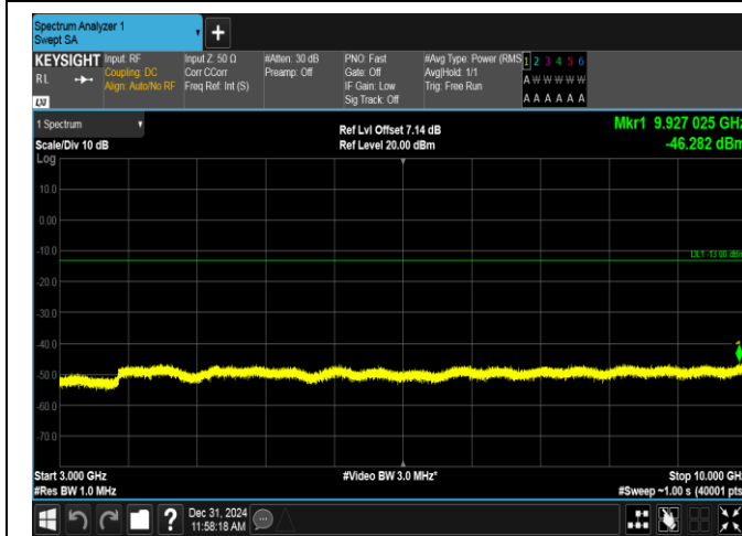
Band12-10MHz-QPSK-23130-1RB#0-3000~10000-PASS
