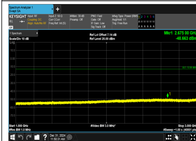
Band12-10MHz-16QAM-23060-50RB#0-1000~3000-PASS
