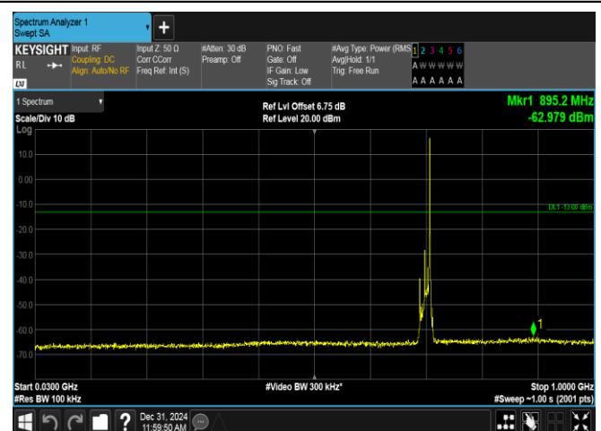
Band12-10MHz-QPSK-23130-1RB#49-30~1000-PASS
