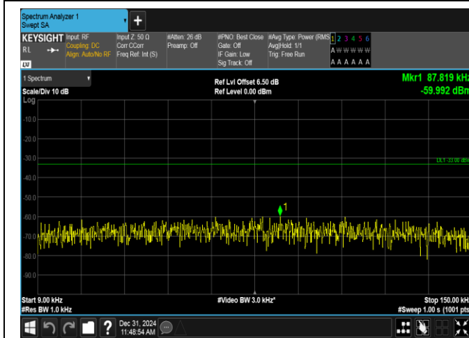
Band12-10MHz-QPSK-23060-50RB#0-0.009~0.15-PASS
