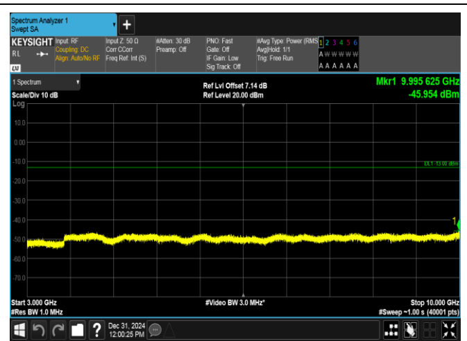
Band12-10MHz-QPSK-23130-1RB#49-3000~10000-PASS
