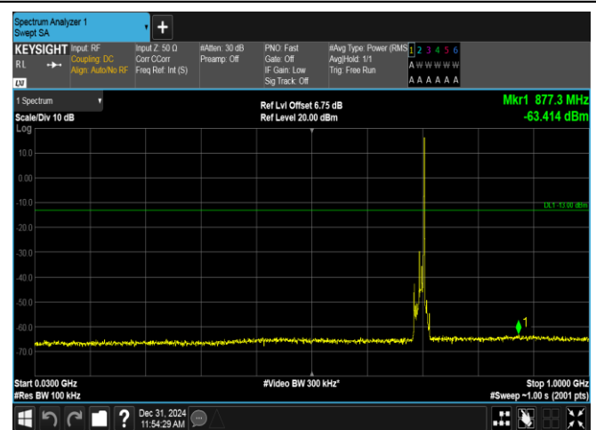
Band12-10MHz-16QAM-23095-1RB#49-30~1000-PASS
