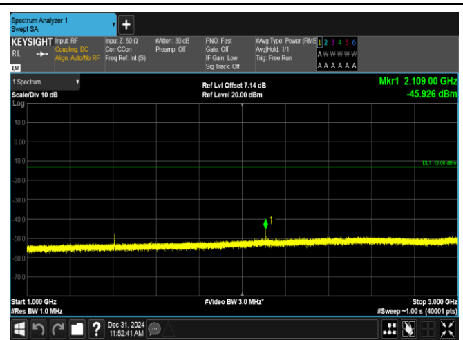
Band12-10MHz-16QAM-23095-1RB#0-1000~3000-PASS
