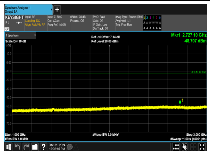
Band12-10MHz-QPSK-23130-50RB#0-1000~3000-PASS
