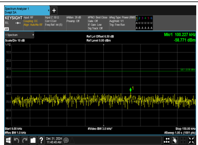
Band12-10MHz-16QAM-23060-1RB#0-0.009~0.15-PASS
