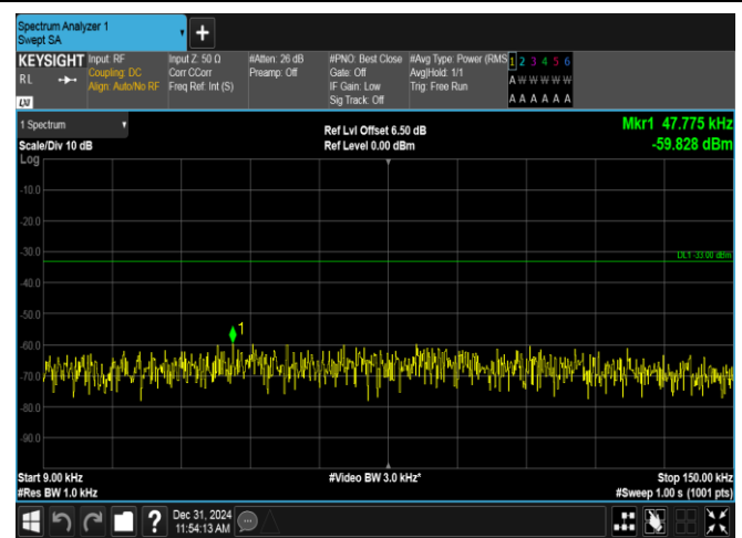
Band12-10MHz-16QAM-23095-1RB#49-0.009~0.15-PASS
