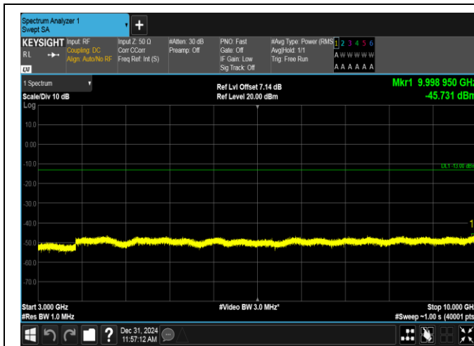
Band12-10MHz-16QAM-23095-50RB#0-3000~10000-PASS
