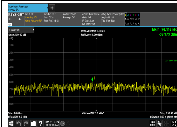
Band12-10MHz-QPSK-23130-1RB#0-0.009~0.15-PASS
