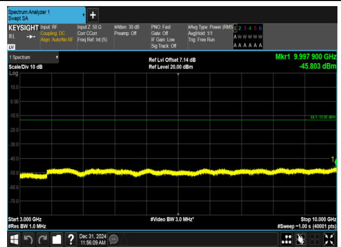
Band12-10MHz-QPSK-23095-50RB#0-3000~10000-PASS
