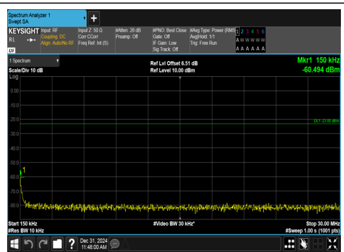
Band12-10MHz-16QAM-23060-1RB#49-0.15~30-PASS
