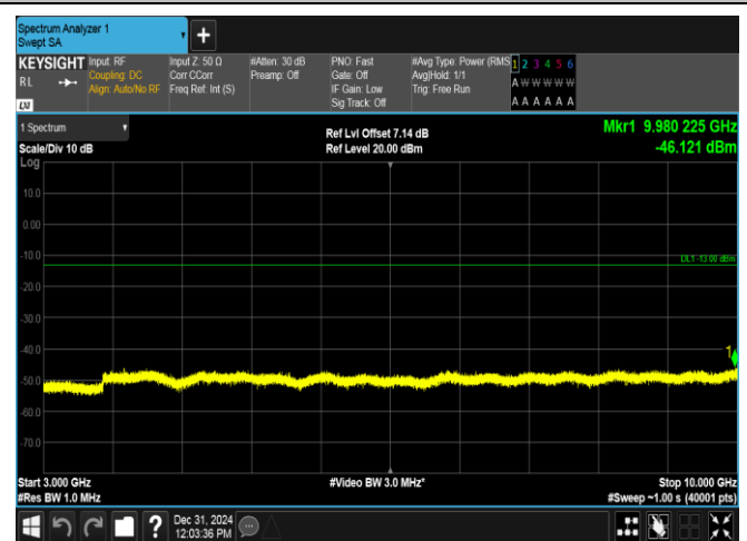
Band12-10MHz-16QAM-23130-50RB#0-3000~10000-PASS
