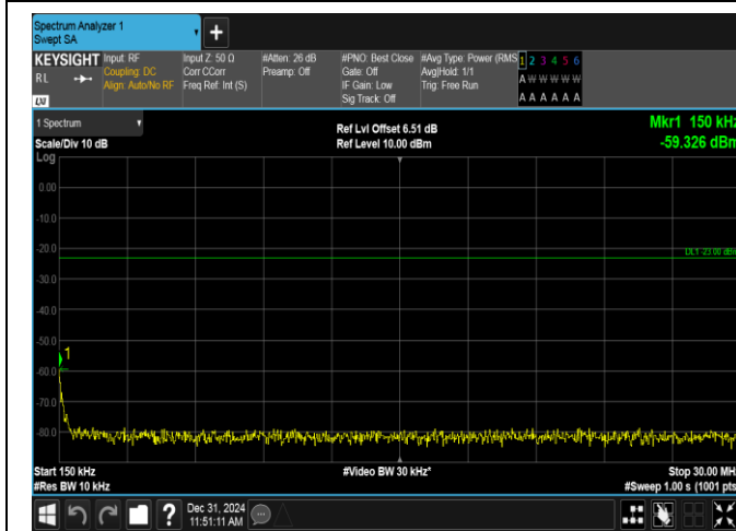
Band12-10MHz-QPSK-23095-1RB#0-0.15~30-PASS
