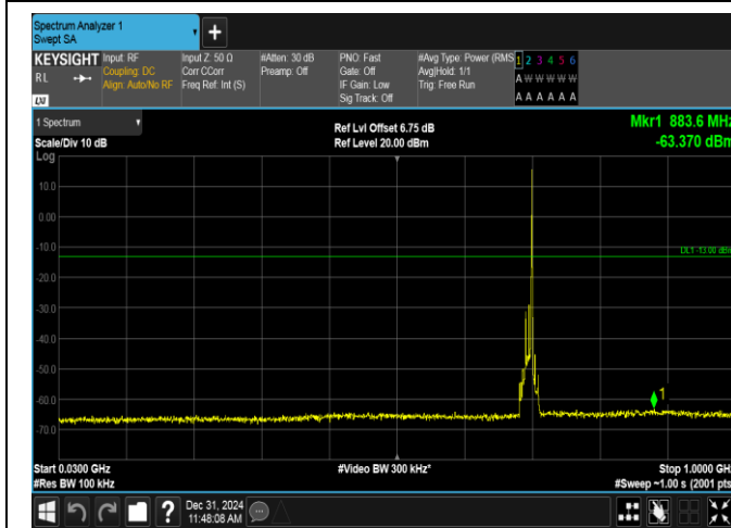
Band12-10MHz-16QAM-23060-1RB#49-30~1000-PASS
