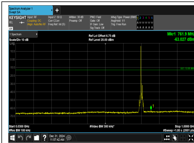
Band12-10MHz-QPSK-23130-1RB#0-30~1000-PASS
