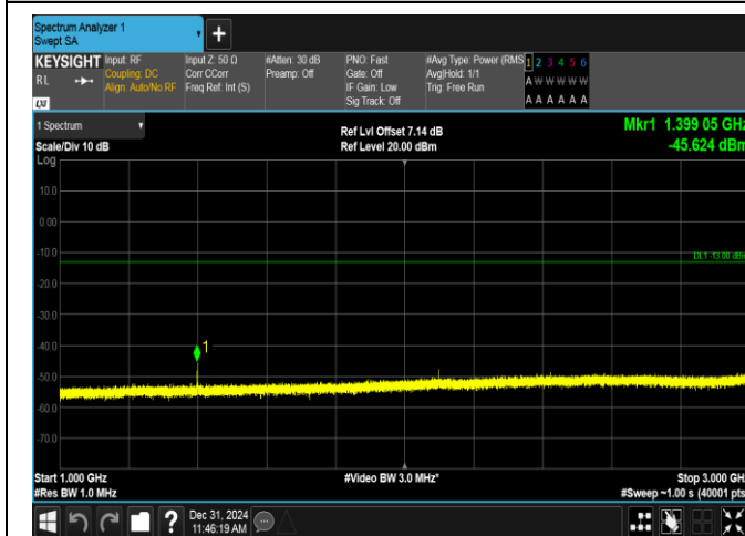
Band12-10MHz-16QAM-23060-1RB#0-1000~3000-PASS
