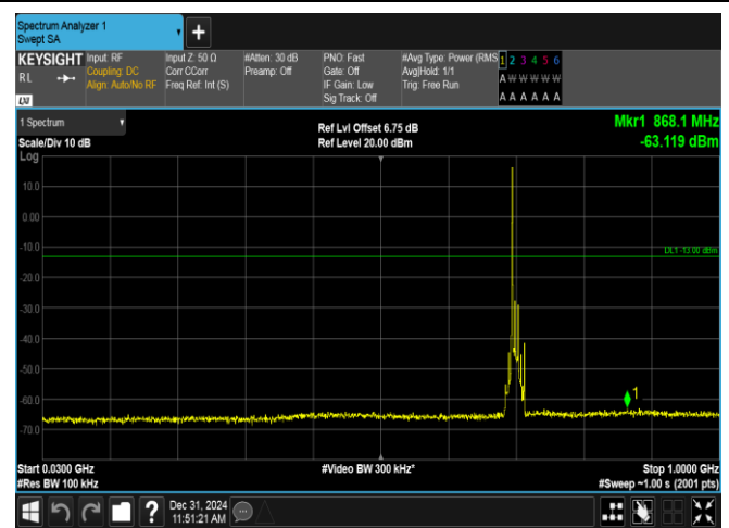
Band12-10MHz-QPSK-23095-1RB#0-30~1000-PASS
