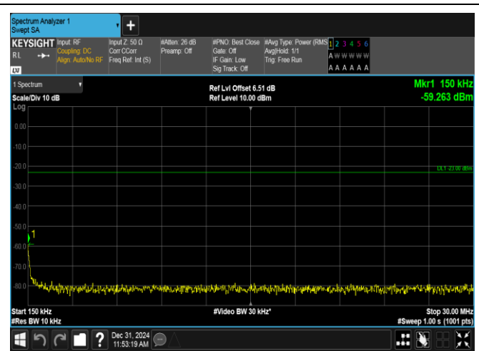
Band12-10MHz-QPSK-23095-1RB#49-0.15~30-PASS
