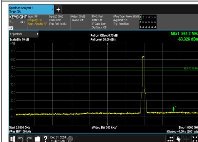
Band12-10MHz-QPSK-23060-50RB#0-30~1000-PASS
