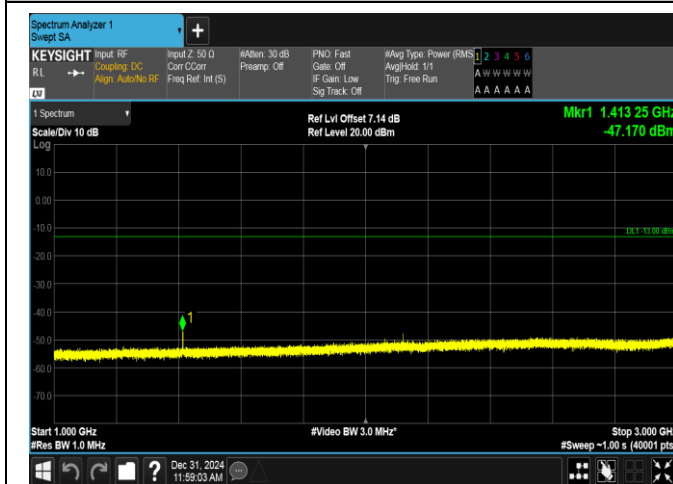
Band12-10MHz-16QAM-23130-1RB#0-1000~3000-PASS
