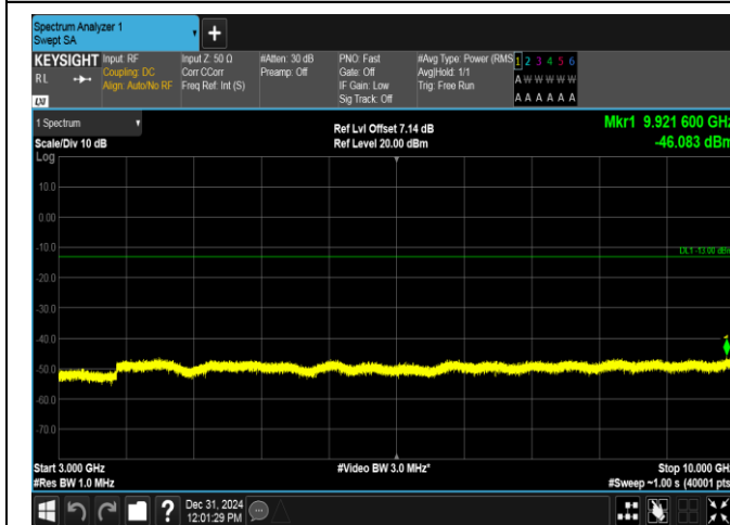
Band12-10MHz-16QAM-23130-1RB#49-3000~10000-PASS
