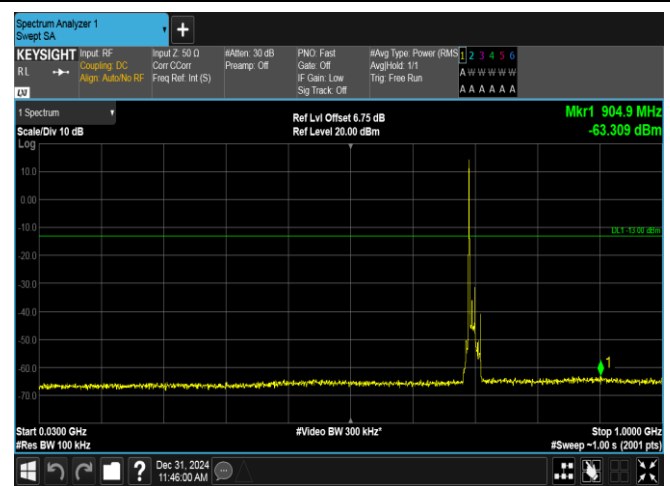
Band12-10MHz-16QAM-23060-1RB#0-30~1000-PASS
