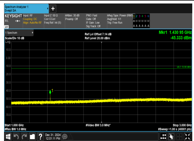
Band12-10MHz-16QAM-23130-1RB#49-1000~3000-PASS
