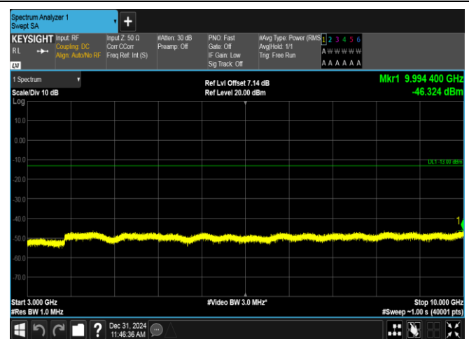
Band12-10MHz-16QAM-23060-1RB#0-3000~10000-PASS
