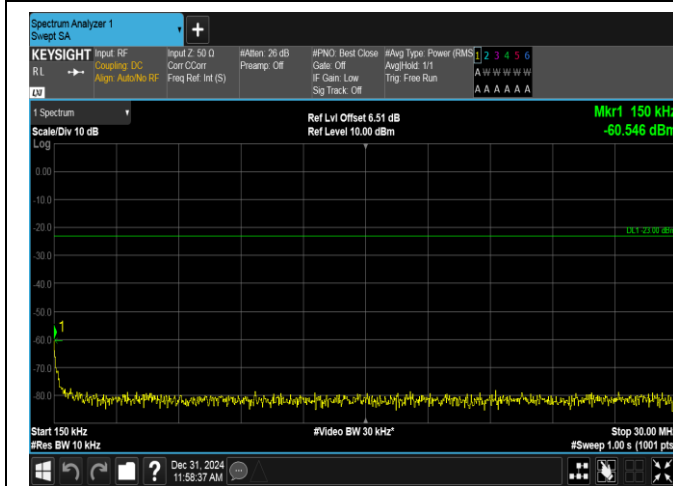
Band12-10MHz-16QAM-23130-1RB#0-0.15~30-PASS
