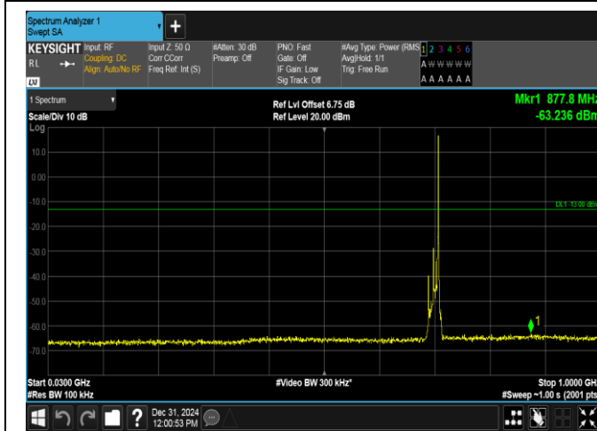
Band12-10MHz-16QAM-23130-1RB#49-30~1000-PASS
