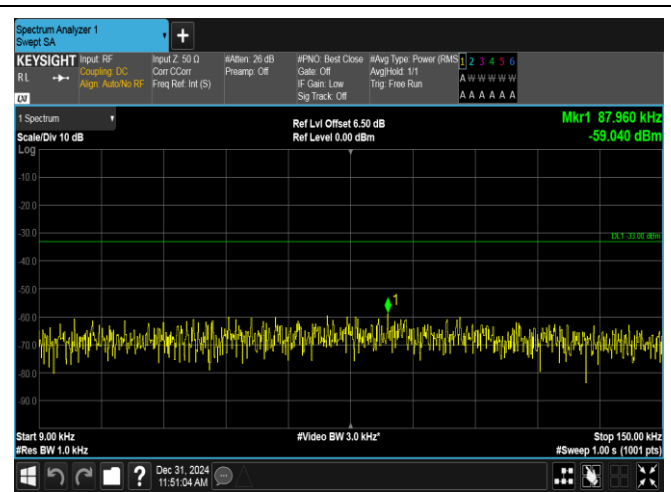
Band12-10MHz-QPSK-23095-1RB#0-0.009~0.15-PASS
