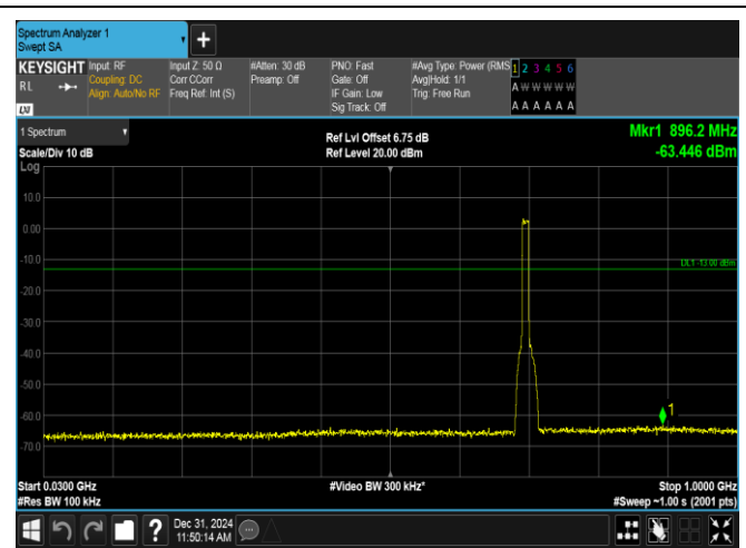
Band12-10MHz-16QAM-23060-50RB#0-30~1000-PASS
