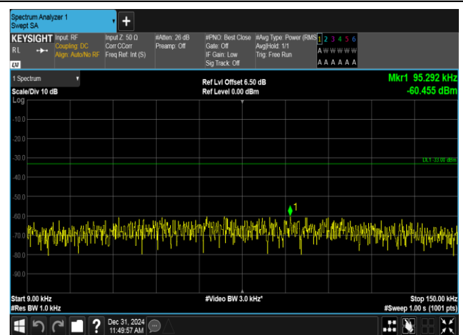
Band12-10MHz-16QAM-23060-50RB#0-0.009~0.15-PASS
