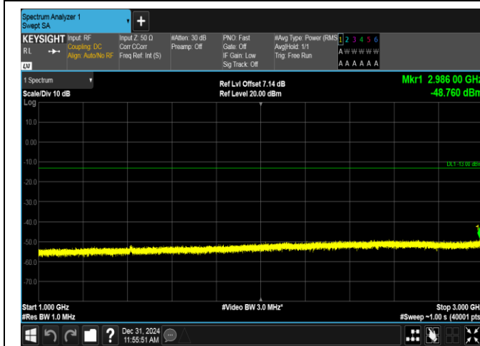
Band12-10MHz-QPSK-23095-50RB#0-1000~3000-PASS
