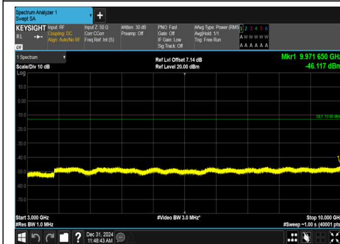
Band12-10MHz-16QAM-23060-1RB#49-3000~10000-PASS
