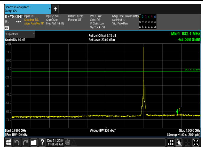
Band12-10MHz-16QAM-23130-1RB#0-30~1000-PASS
