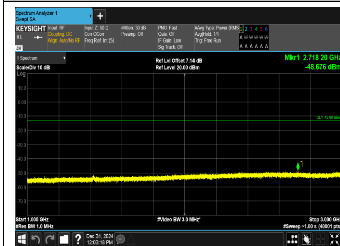
Band12-10MHz-16QAM-23130-50RB#0-1000~3000-PASS
