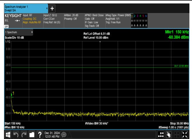
Band12-10MHz-QPSK-23130-50RB#0-0.15~30-PASS
