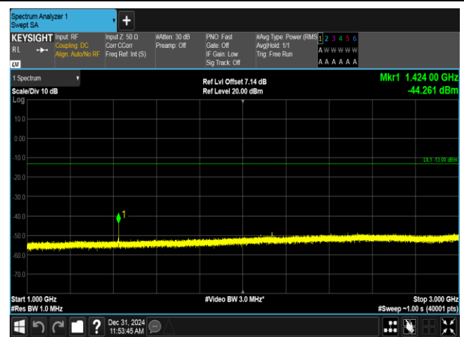
Band12-10MHz-QPSK-23095-1RB#49-1000~3000-PASS
