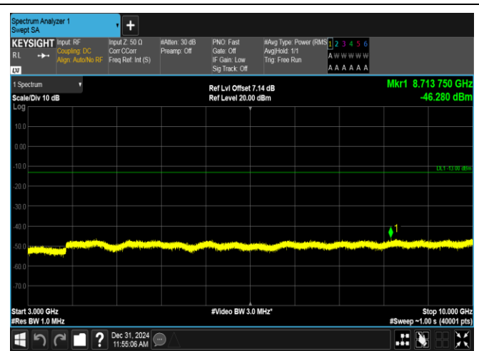
Band12-10MHz-16QAM-23095-1RB#49-3000~10000-PASS
