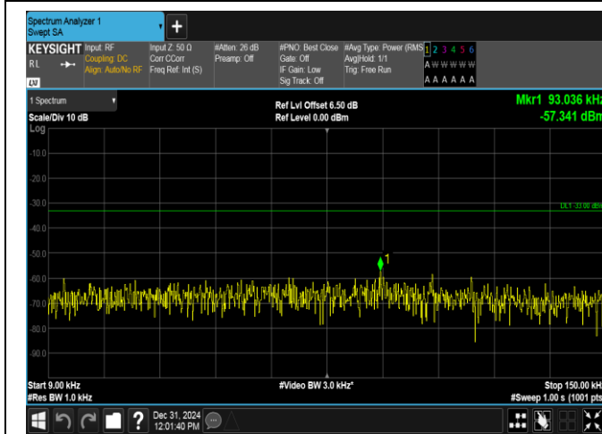
Band12-10MHz-QPSK-23130-50RB#0-0.009~0.15-PASS
