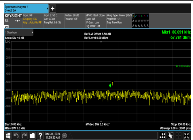
Band12-10MHz-QPSK-23130-1RB#49-0.009~0.15-PASS
