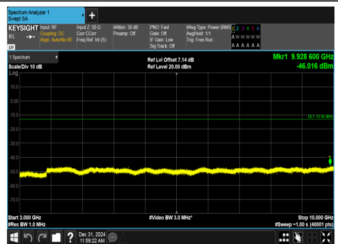
Band12-10MHz-16QAM-23130-1RB#0-3000~10000-PASS
