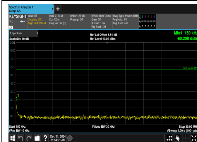
Band12-10MHz-16QAM-23095-1RB#49-0.15~30-PASS
