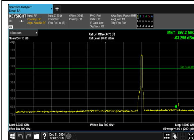
Band12-10MHz-QPSK-23130-50RB#0-30~1000-PASS
