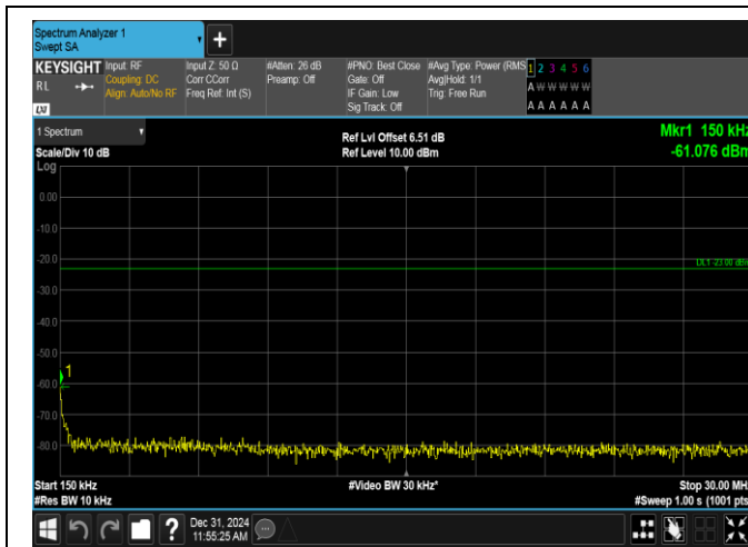
Band12-10MHz-QPSK-23095-50RB#0-0.15~30-PASS
