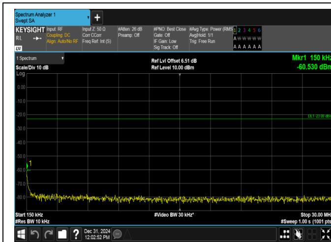
Band12-10MHz-16QAM-23130-50RB#0-0.15~30-PASS
