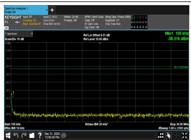
Band12-10MHz-16QAM-23130-1RB#49-0.15~30-PASS
