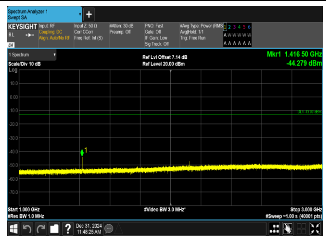
Band12-10MHz-16QAM-23060-1RB#49-1000~3000-PASS
