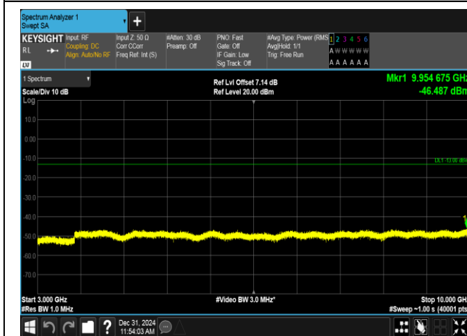
Band12-10MHz-QPSK-23095-1RB#49-3000~10000-PASS
