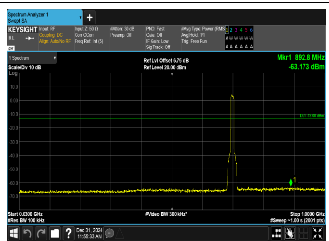
Band12-10MHz-QPSK-23095-50RB#0-30~1000-PASS
