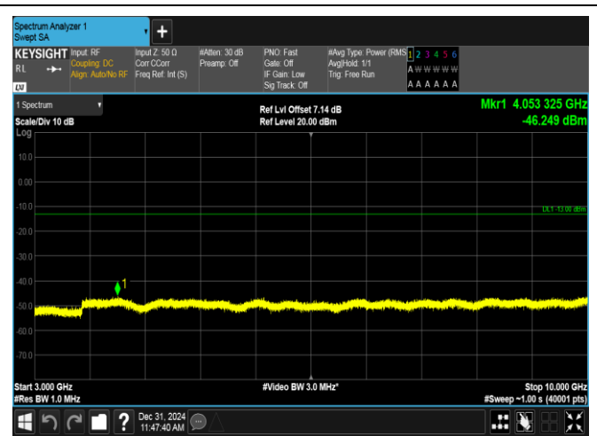
Band12-10MHz-QPSK-23060-1RB#49-3000~10000-PASS
