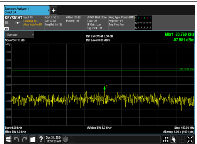
Band12-10MHz-16QAM-23130-1RB#0-0.009~0.15-PASS
