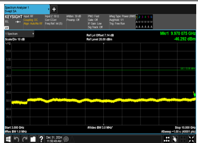
Band12-10MHz-16QAM-23060-50RB#0-3000~10000-PASS
