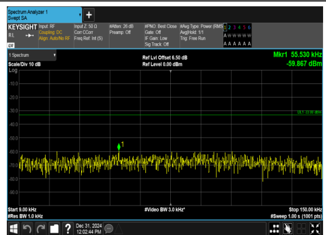
Band12-10MHz-16QAM-23130-50RB#0-0.009~0.15-PASS
