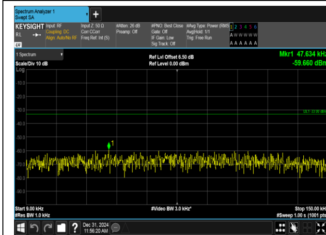
Band12-10MHz-16QAM-23095-50RB#0-0.009~0.15-PASS
