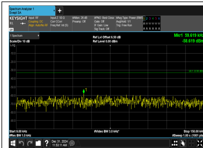
Band12-10MHz-QPSK-23095-1RB#49-0.009~0.15-PASS
