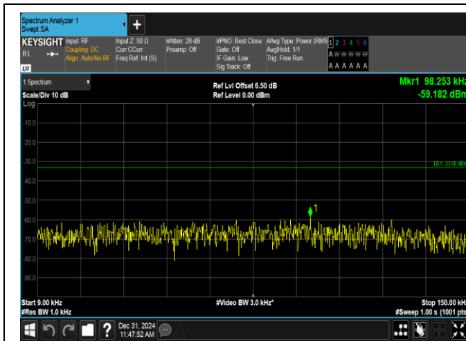
Band12-10MHz-16QAM-23060-1RB#49-0.009~0.15-PASS
