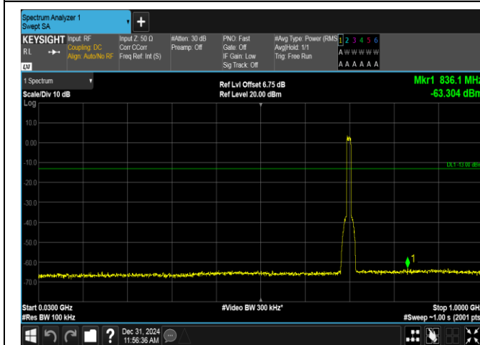
Band12-10MHz-16QAM-23095-50RB#0-30~1000-PASS
