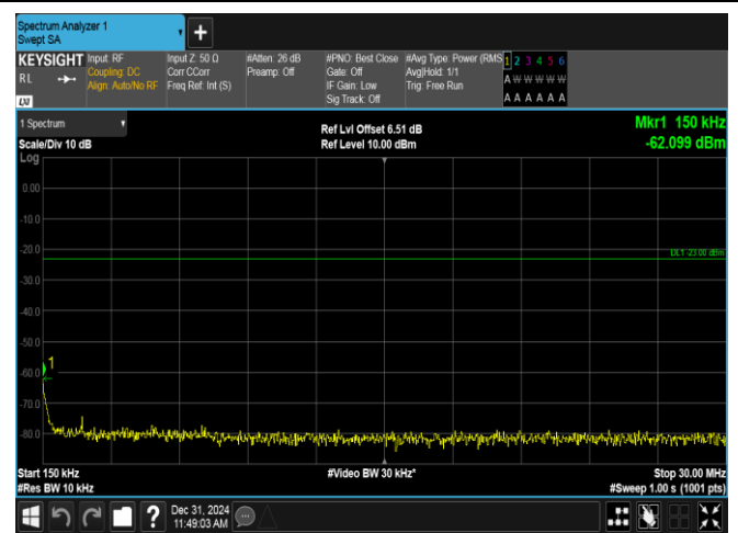
Band12-10MHz-QPSK-23060-50RB#0-0.15~30-PASS
