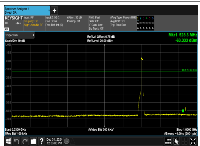
Band12-10MHz-16QAM-23130-50RB#0-30~1000-PASS
