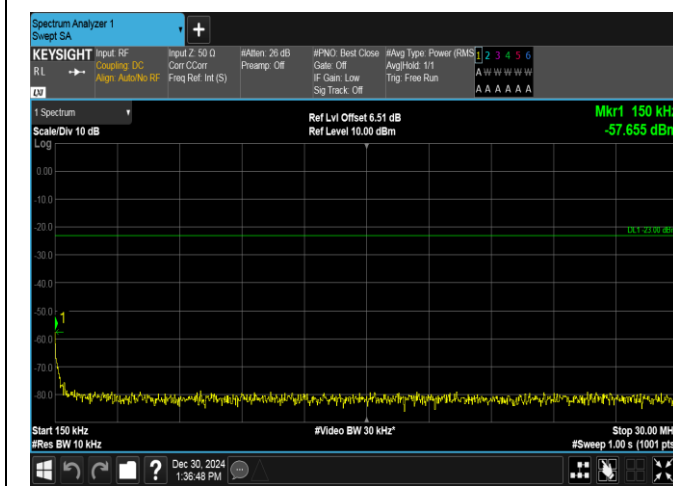
Band12-5MHz-16QAM-23155-1RB#0-0.15~30-PASS
