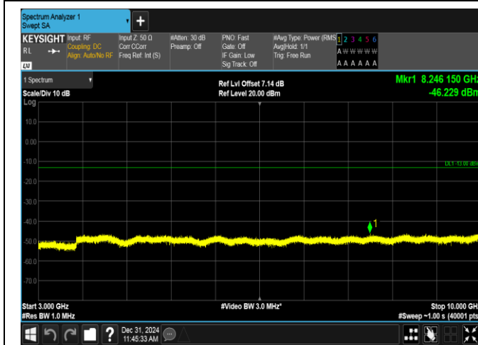
Band12-10MHz-QPSK-23060-1RB#0-3000~10000-PASS
