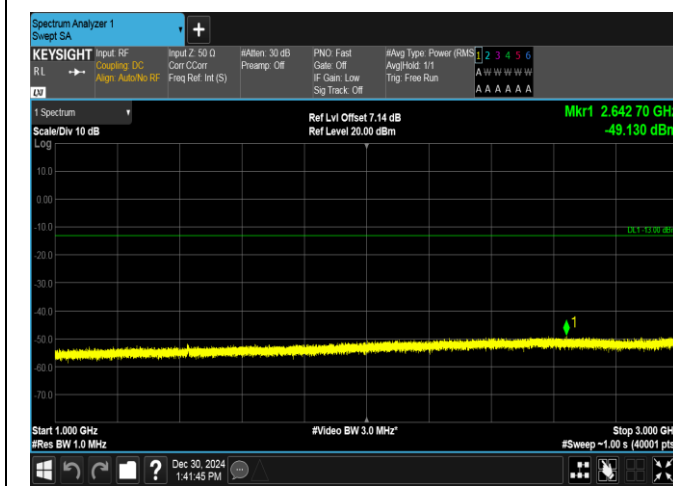
Band12-5MHz-16QAM-23155-25RB#0-1000~3000-PASS
