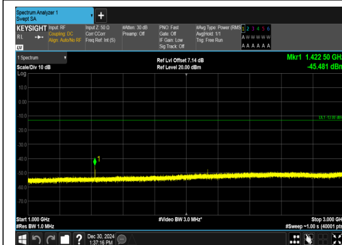
Band12-5MHz-16QAM-23155-1RB#0-1000~3000-PASS
