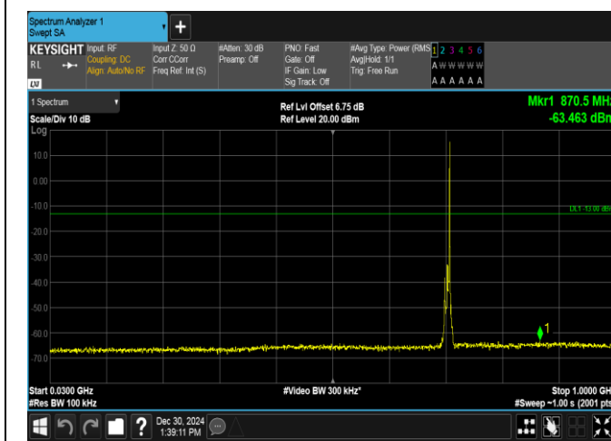
Band12-5MHz-16QAM-23155-1RB#24-30~1000-PASS
