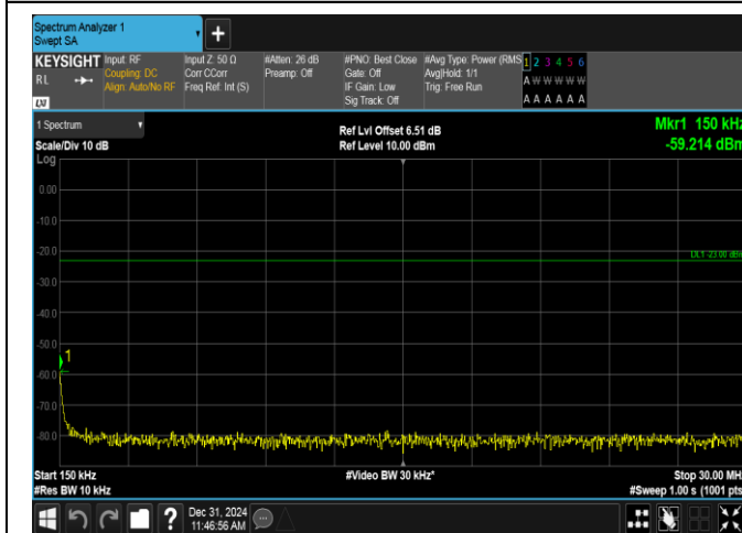
Band12-10MHz-QPSK-23060-1RB#49-0.15~30-PASS
