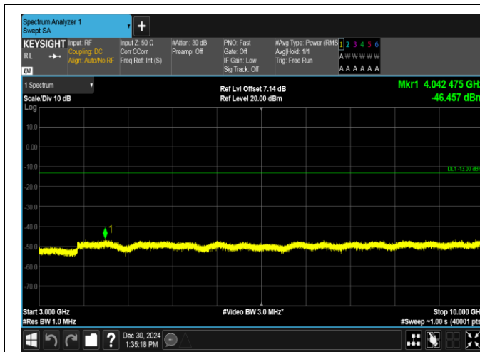
Band12-5MHz-16QAM-23095-25RB#0-3000~10000-PASS
