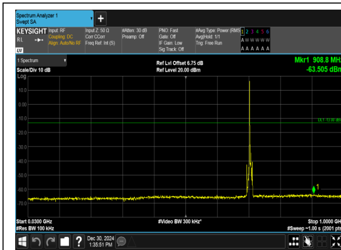
Band12-5MHz-QPSK-23155-1RB#0-30~1000-PASS
