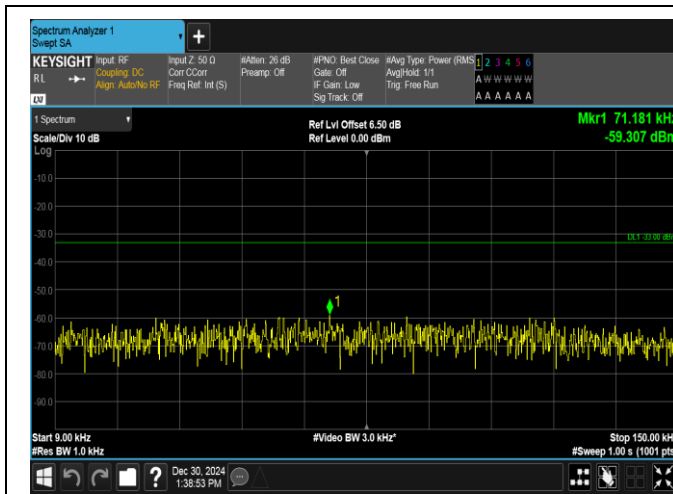
Band12-5MHz-16QAM-23155-1RB#24-0.009~0.15-PASS
