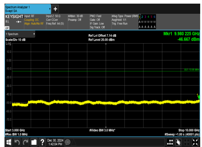
Band12-5MHz-16QAM-23155-25RB#0-3000~10000-PASS
