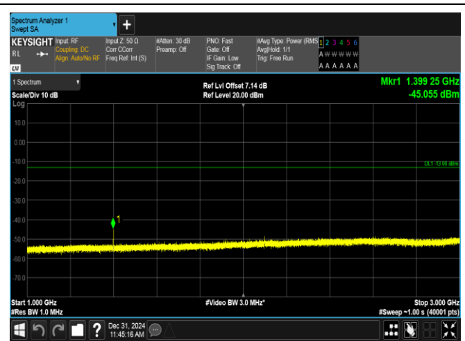
Band12-10MHz-QPSK-23060-1RB#0-1000~3000-PASS
