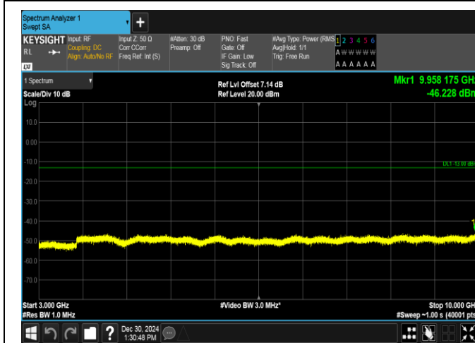
Band12-5MHz-16QAM-23095-1RB#0-3000~10000-PASS
