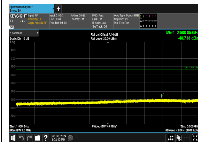
Band12-5MHz-16QAM-23035-25RB#0-1000~3000-PASS
