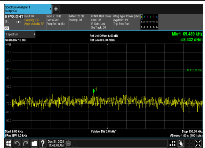
Band12-10MHz-QPSK-23060-1RB#49-0.009~0.15-PASS
