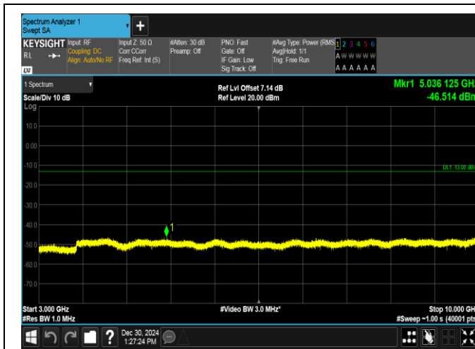
Band12-5MHz-QPSK-23035-25RB#0-3000~10000-PASS
