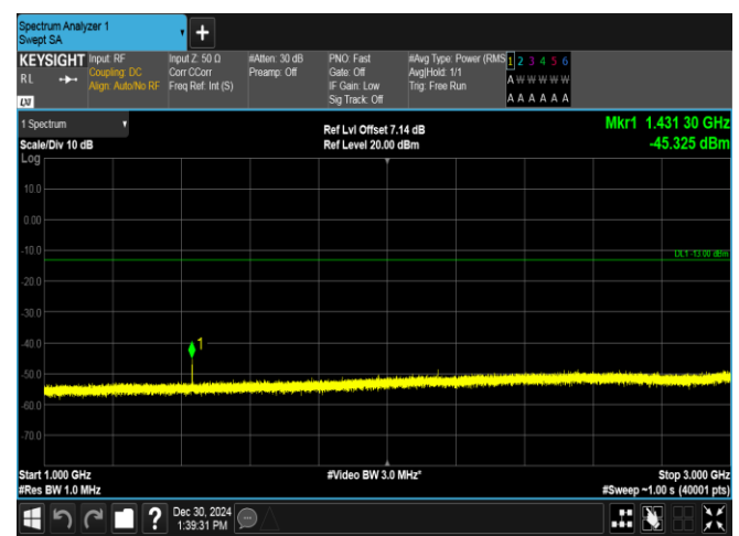
Band12-5MHz-16QAM-23155-1RB#24-1000~3000-PASS
