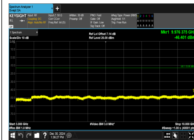
Band12-5MHz-QPSK-23155-1RB#0-3000~10000-PASS
