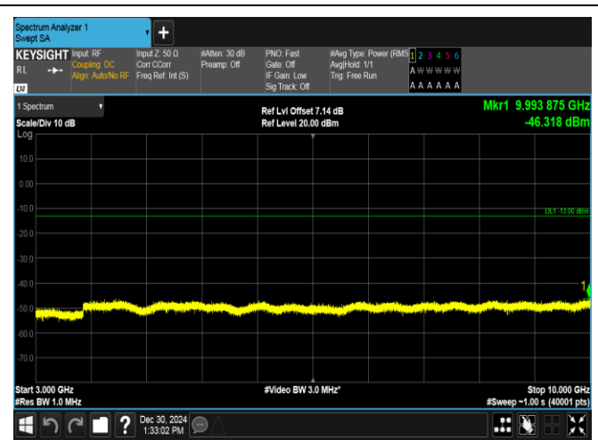
Band12-5MHz-16QAM-23095-1RB#24-3000~10000-PASS
