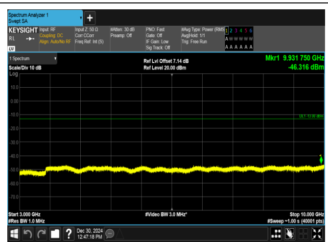
Band12-3MHz-QPSK-23165-1RB#14-3000~10000-PASS
