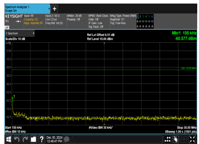
Band12-3MHz-QPSK-23165-15RB#0-0.15~30-PASS
