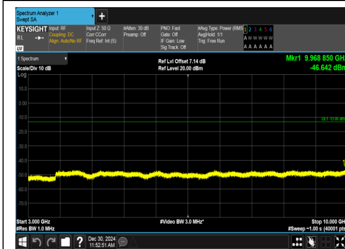
Band12-1.4MHz-QPSK-23173-1RB#0-3000~10000-PASS
