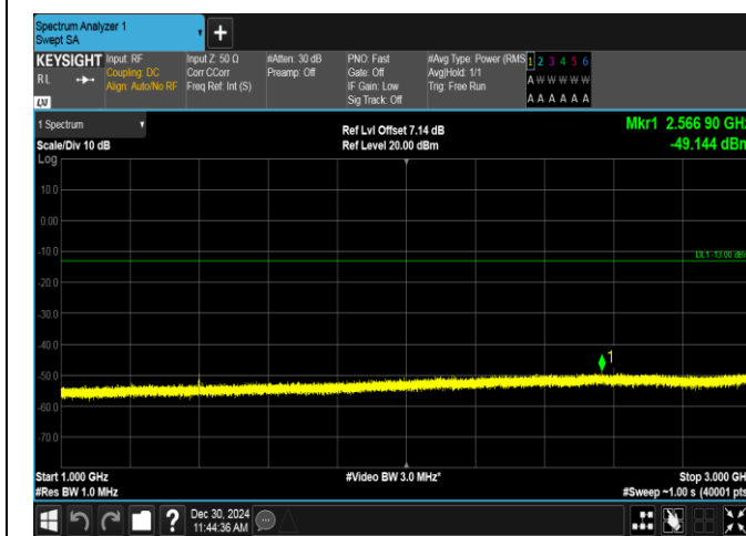
Band12-1.4MHz-16QAM-23017-6RB#0-1000~3000-PASS
