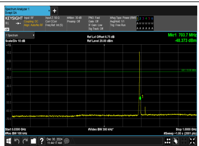
Band12-1.4MHz-16QAM-23017-6RB#0-30~1000-PASS
