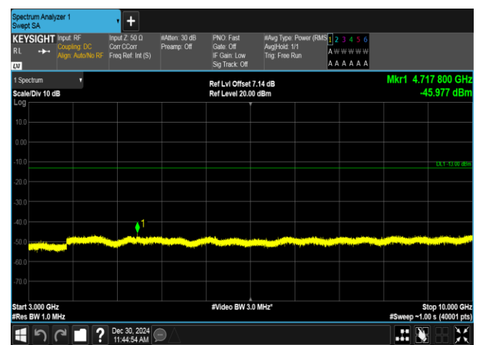
Band12-1.4MHz-16QAM-23017-6RB#0-3000~10000-PASS
