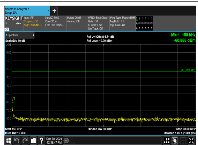
Band12-3MHz-QPSK-23095-1RB#14-0.15~30-PASS
