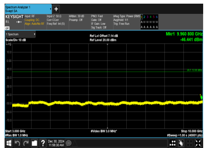
Band12-1.4MHz-16QAM-23173-6RB#0-3000~10000-PASS
