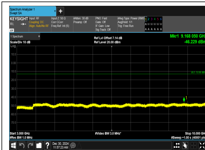
Band12-1.4MHz-QPSK-23173-6RB#0-3000~10000-PASS
