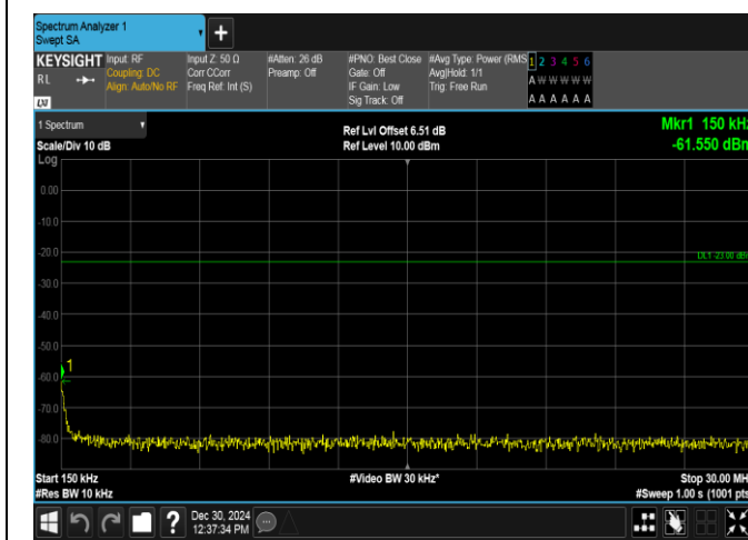
Band12-3MHz-QPSK-23095-1RB#0-0.15~30-PASS
