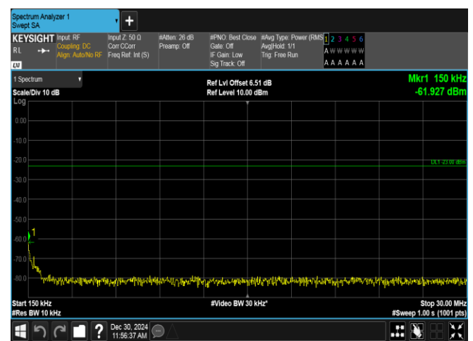
Band12-1.4MHz-QPSK-23173-6RB#0-0.15~30-PASS
