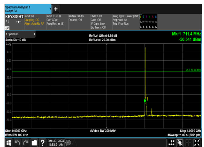
Band12-1.4MHz-16QAM-23173-1RB#0-30~1000-PASS
