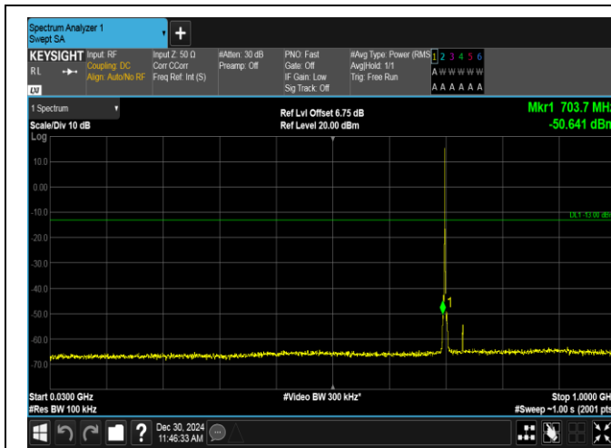
Band12-1.4MHz-16QAM-23095-1RB#0-30~1000-PASS
