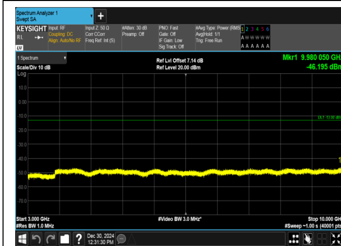
Band12-3MHz-QPSK-23025-1RB#0-3000~10000-PASS
