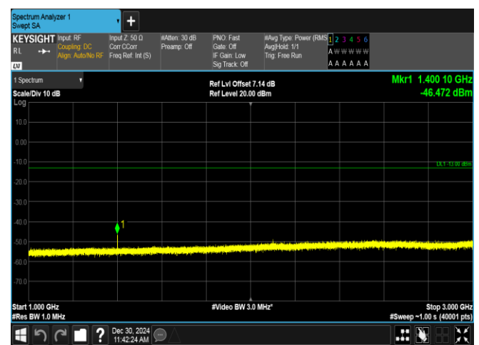
Band12-1.4MHz-16QAM-23017-1RB#5-1000~3000-PASS
