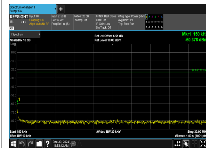
Band12-1.4MHz-16QAM-23173-1RB#0-0.15~30-PASS
