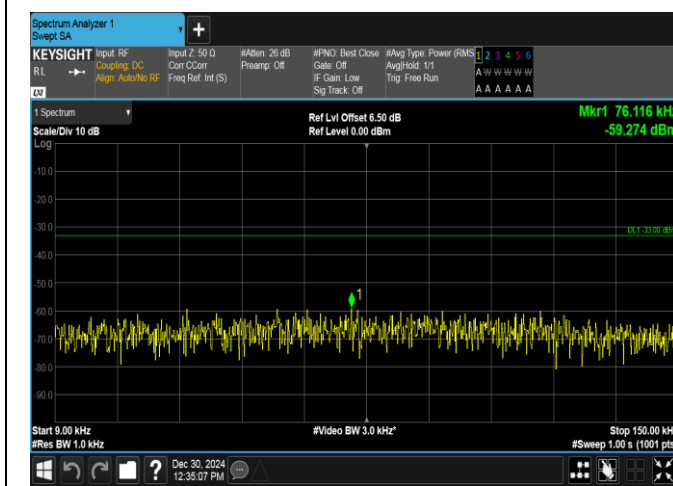
Band12-3MHz-QPSK-23025-15RB#0-0.009~0.15-PASS
