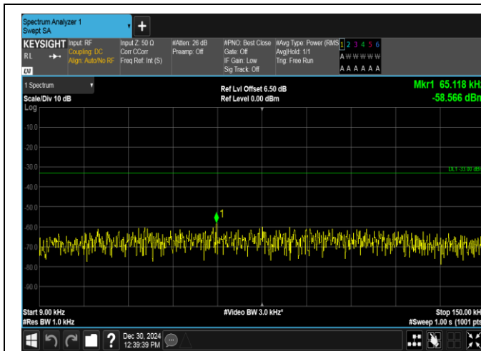
Band12-3MHz-QPSK-23095-1RB#14-0.009~0.15-PASS
