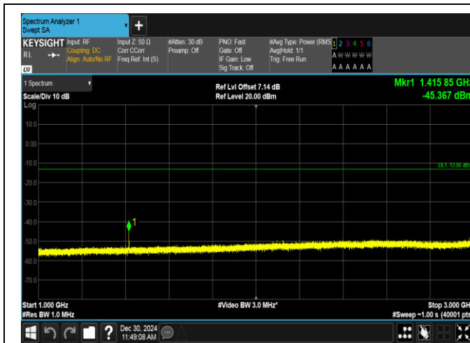
Band12-1.4MHz-16QAM-23095-1RB#5-1000~3000-PASS
