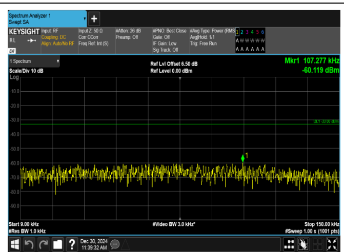
Band12-1.4MHz-16QAM-23017-1RB#0-0.009~0.15-PASS
