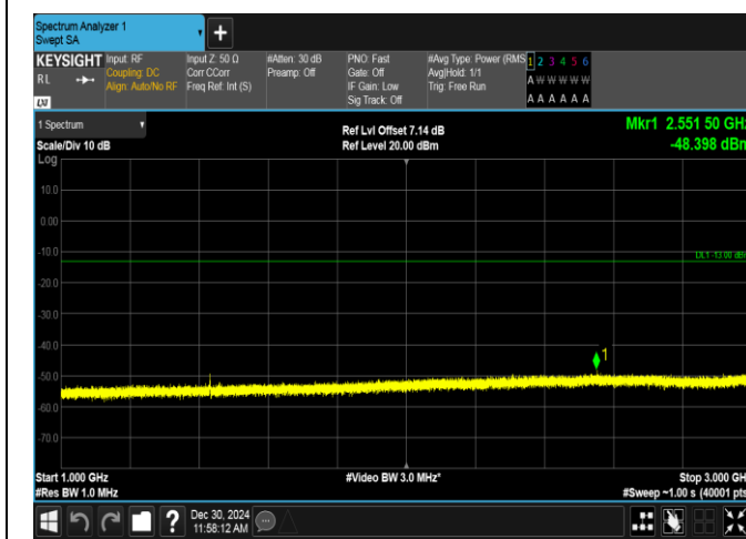
Band12-1.4MHz-16QAM-23173-6RB#0-1000~3000-PASS
