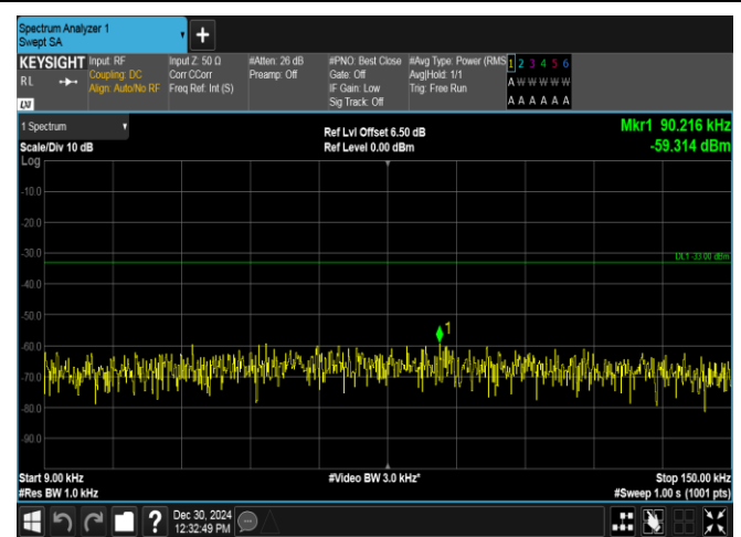
Band12-3MHz-QPSK-23025-1RB#14-0.009~0.15-PASS
