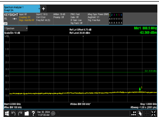
Band7-20MHz-16QAM-21350-100RB#0-30~1000-PASS
