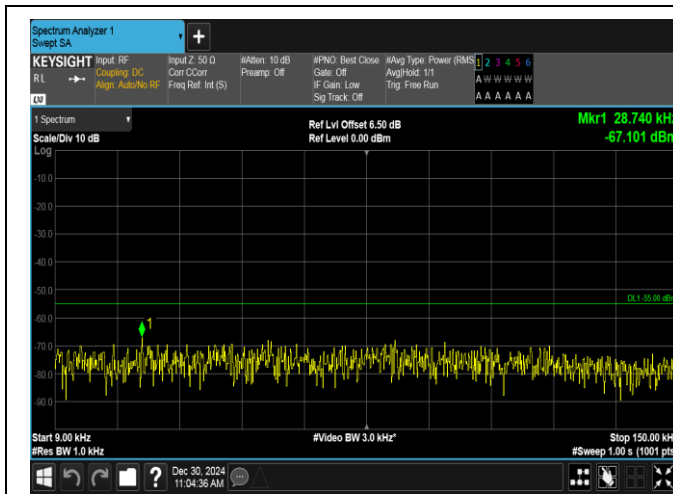
Band7-20MHz-16QAM-21350-1RB#99-0.009~0.15-PASS
