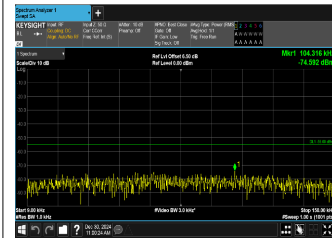
Band7-20MHz-16QAM-21100-100RB#0-0.009~0.15-PASS
