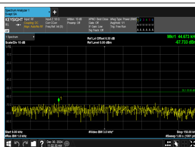
Band7-20MHz-16QAM-21350-1RB#0-0.009~0.15-PASS
