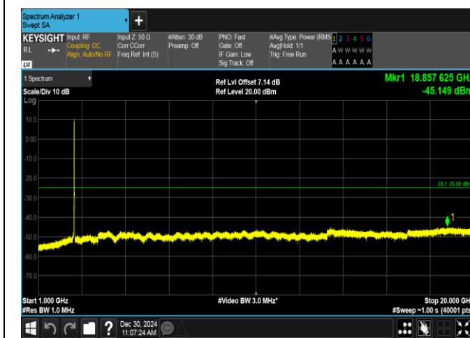
Band7-20MHz-16QAM-21350-100RB#0-1000~20000-PAS
