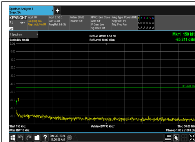
Band7-20MHz-16QAM-21350-100RB#0-0.15~30-PASS
