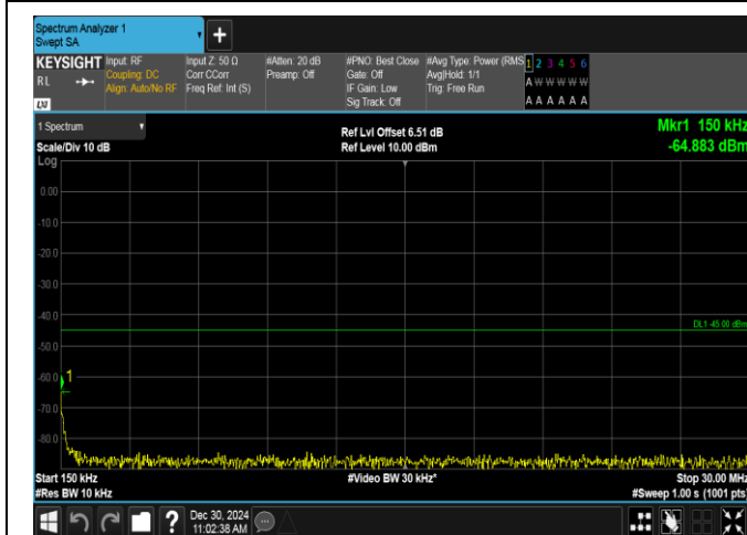
Band7-20MHz-16QAM-21350-1RB#0-0.15~30-PASS
