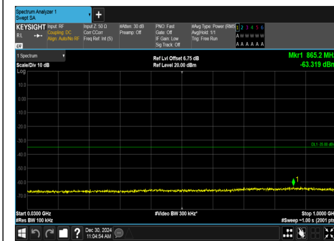
Band7-20MHz-16QAM-21350-1RB#99-30~1000-PASS
