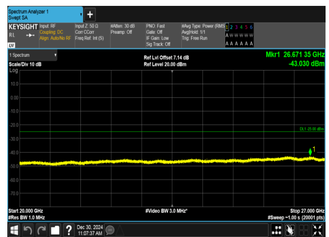
Band7-20MHz-16QAM-21350-100RB#0-20000~27000-PA
