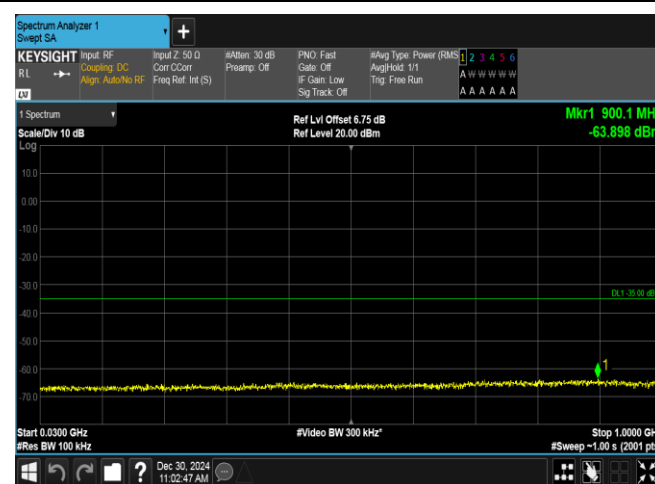
Band7-20MHz-16QAM-21350-1RB#0-30~1000-PASS
