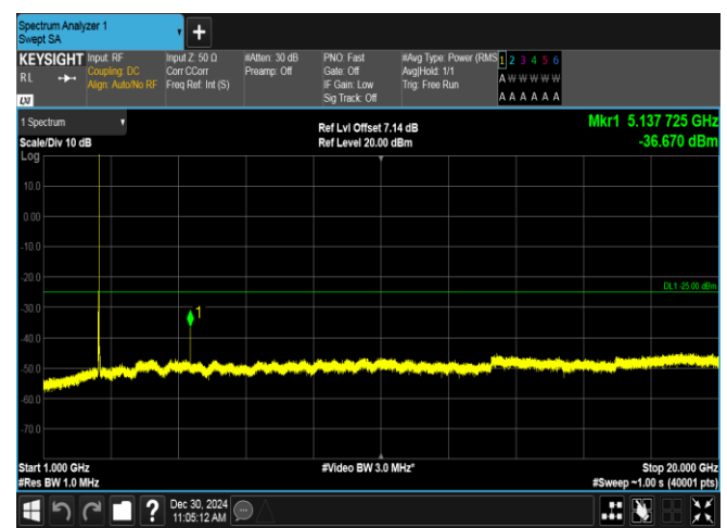
Band7-20MHz-16QAM-21350-1RB#99-1000~20000-PASS
