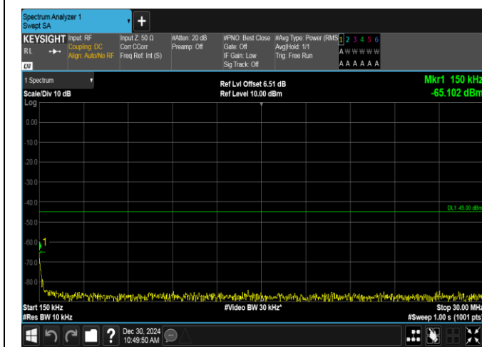
Band7-20MHz-16QAM-20850-1RB#0-0.15~30-PASS
