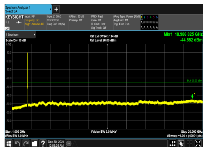
Band7-20MHz-QPSK-20850-100RB#0-1000~20000-PASS
