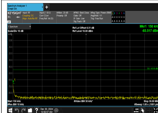
Band7-20MHz-QPSK-20850-1RB#99-0.15~30-PASS
