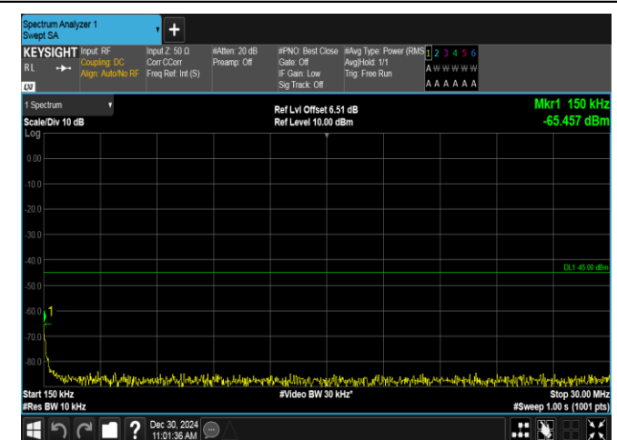
Band7-20MHz-QPSK-21350-1RB#0-0.15~30-PASS
