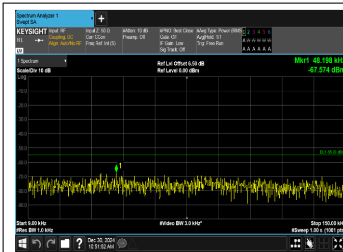
Band7-20MHz-16QAM-20850-1RB#99-0.009~0.15-PASS
