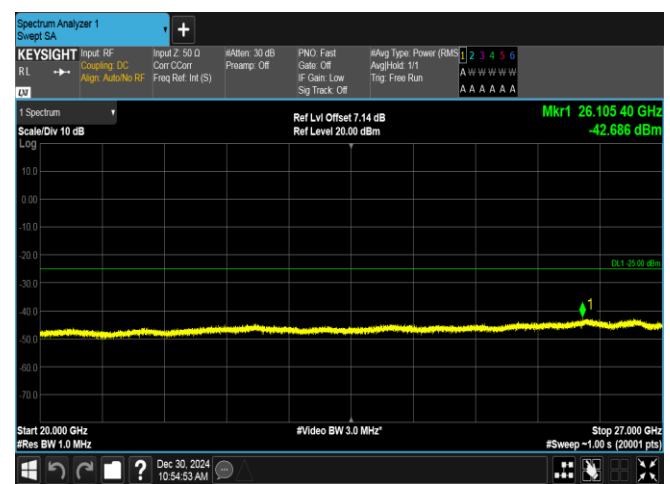
Band7-20MHz-16QAM-20850-100RB#0-20000~27000-PA
