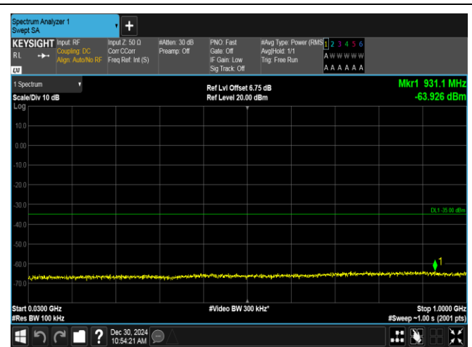
Band7-20MHz-16QAM-20850-100RB#0-30~1000-PASS
