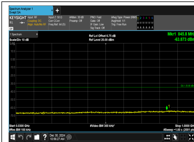
Band7-20MHz-16QAM-21100-1RB#0-30~1000-PASS
