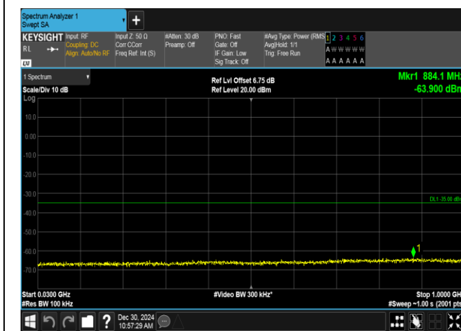
Band7-20MHz-QPSK-21100-1RB#99-30~1000-PASS
