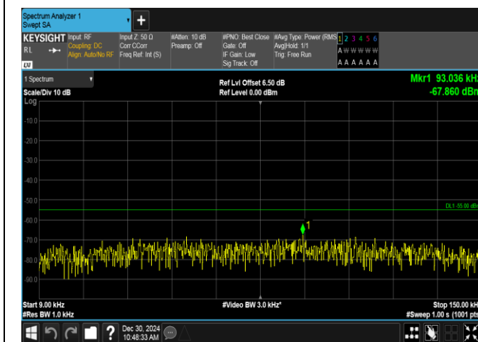
Band7-20MHz-QPSK-20850-1RB#0-0.009~0.15-PASS
