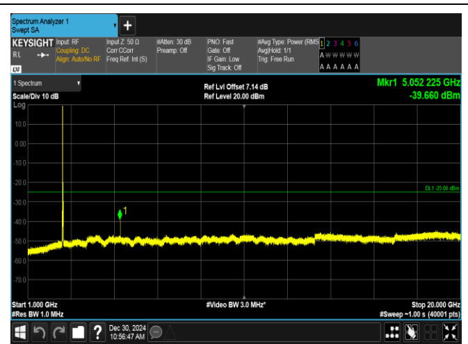
Band7-20MHz-16QAM-21100-1RB#0-1000~20000-PASS
