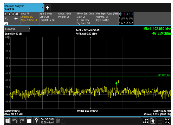
Band7-20MHz-QPSK-20850-1RB#99-0.009~0.15-PASS
