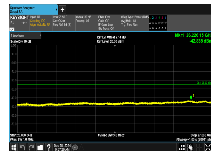
Band7-15MHz-16QAM-21375-1RB#74-20000~27000-PAS
