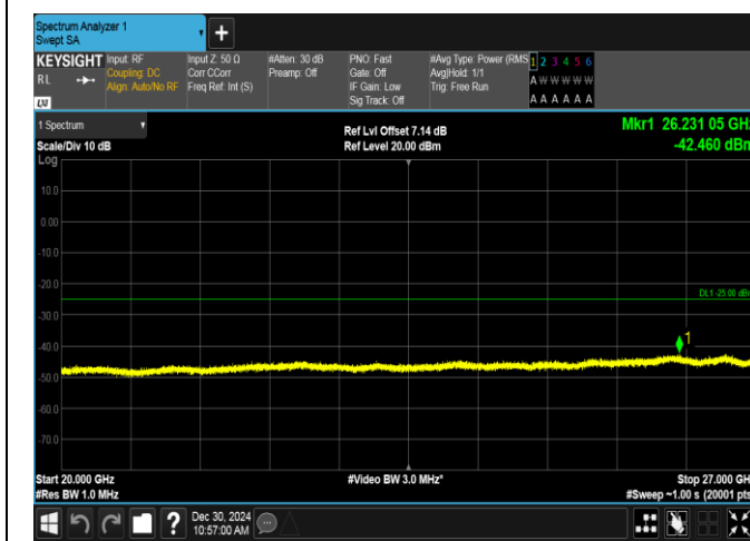
Band7-20MHz-16QAM-21100-1RB#0-20000~27000-PASS
