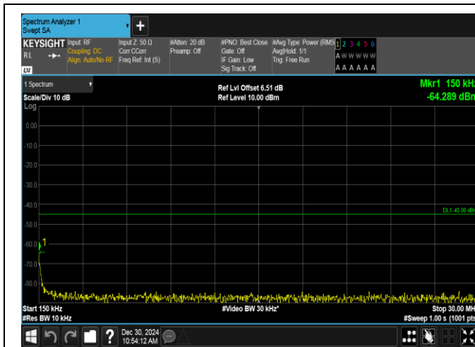
Band7-20MHz-16QAM-20850-100RB#0-0.15~30-PASS
