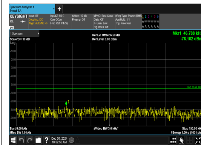
Band7-20MHz-QPSK-20850-100RB#0-0.009~0.15-PASS
