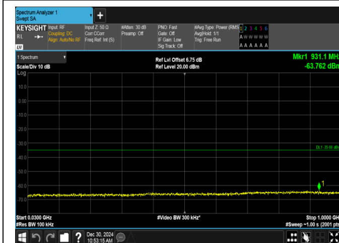
Band7-20MHz-QPSK-20850-100RB#0-30~1000-PASS
