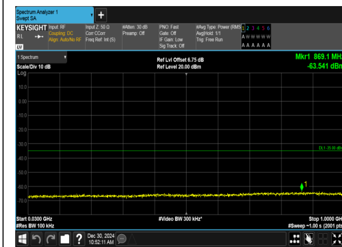
Band7-20MHz-16QAM-20850-1RB#99-30~1000-PASS
