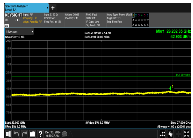
Band7-15MHz-16QAM-21375-75RB#0-20000~27000-PASS S
