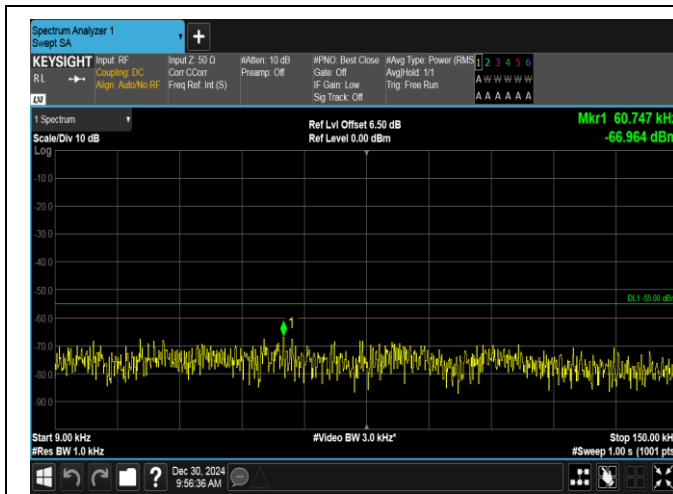
Band7-15MHz-16QAM-21375-1RB#74-0.009~0.15-PASS
