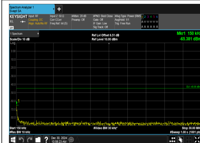
Band7-20MHz-16QAM-21100-1RB#99-0.15~30-PASS
