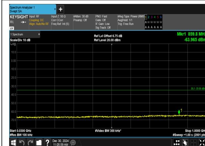
Band7-20MHz-QPSK-21350-100RB#0-30~1000-PASS
