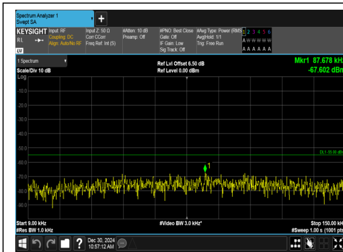
Band7-20MHz-QPSK-21100-1RB#99-0.009~0.15-PASS
