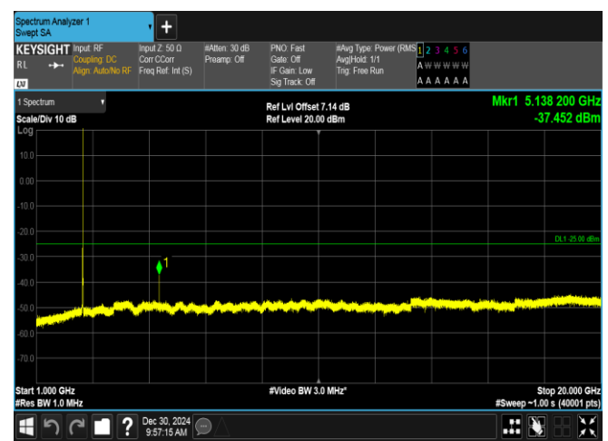
Band7-15MHz-16QAM-21375-1RB#74-1000~20000-PASS
