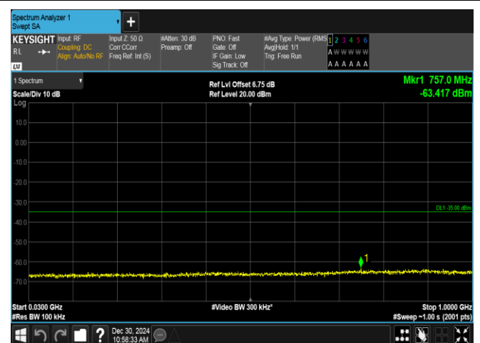
Band7-20MHz-16QAM-21100-1RB#99-30~1000-PASS
