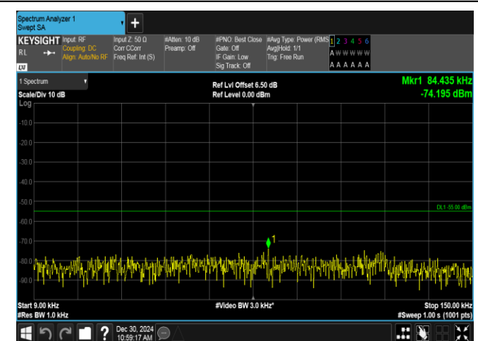
Band7-20MHz-QPSK-21100-100RB#0-0.009~0.15-PASS
