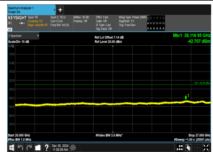
Band7-20MHz-QPSK-21100-100RB#0-20000~27000-PASS
