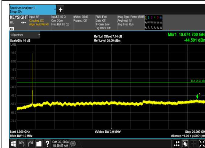
Band7-20MHz-QPSK-21100-100RB#0-1000~20000-PASS
