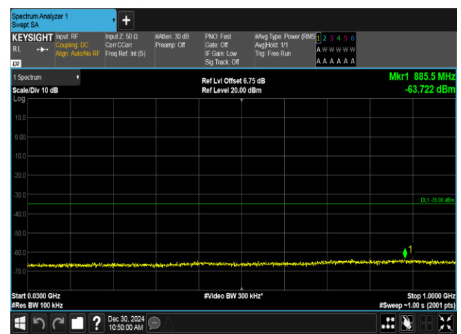
Band7-20MHz-16QAM-20850-1RB#0-30~1000-PASS
