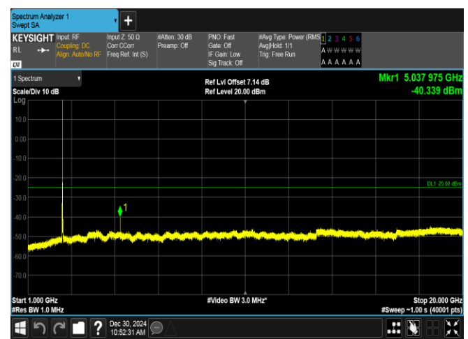
Band7-20MHz-16QAM-20850-1RB#99-1000~20000-PASS
