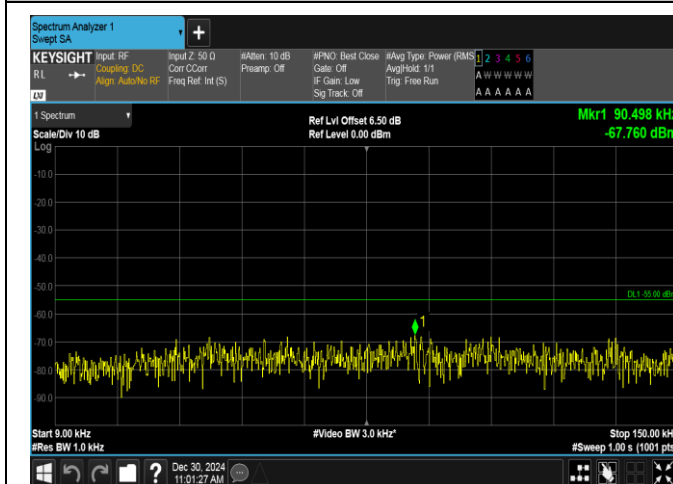
Band7-20MHz-QPSK-21350-1RB#0-0.009~0.15-PASS
