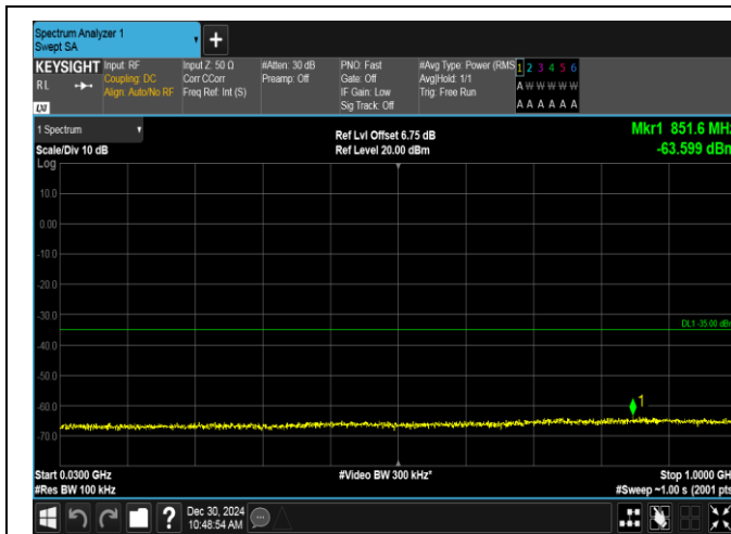
Band7-20MHz-QPSK-20850-1RB#0-30~1000-PASS
