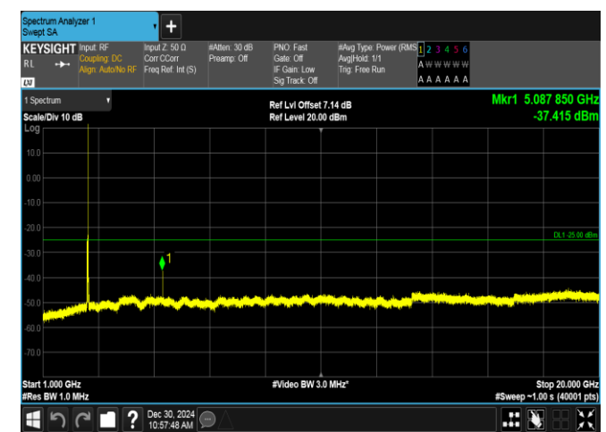
Band7-20MHz-QPSK-21100-1RB#99-1000~20000-PASS
