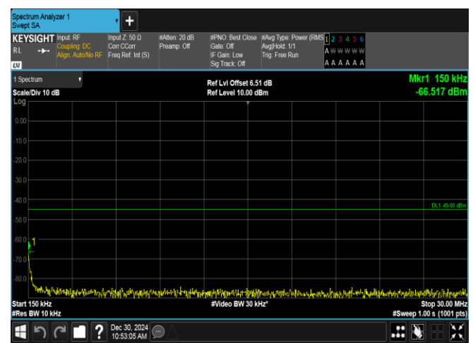
Band7-20MHz-QPSK-20850-100RB#0-0.15~30-PASS
