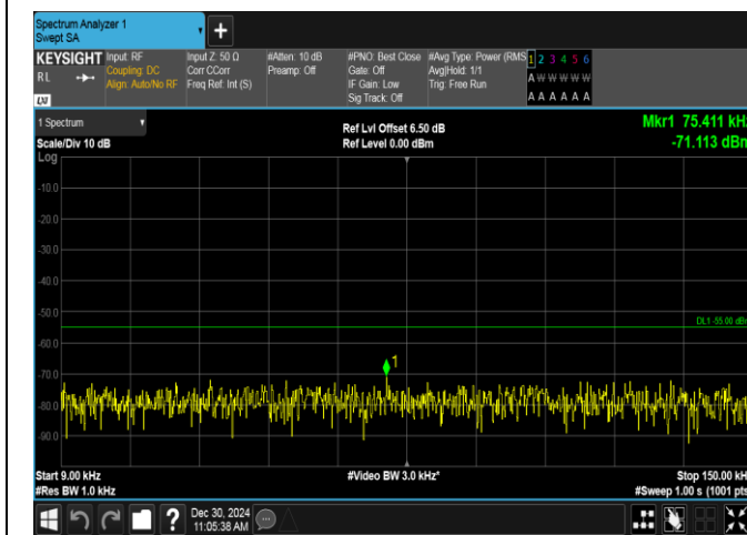
Band7-20MHz-QPSK-21350-100RB#0-0.009~0.15-PASS
