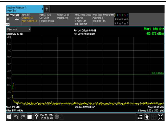
Band7-20MHz-QPSK-21100-1RB#99-0.15~30-PASS
