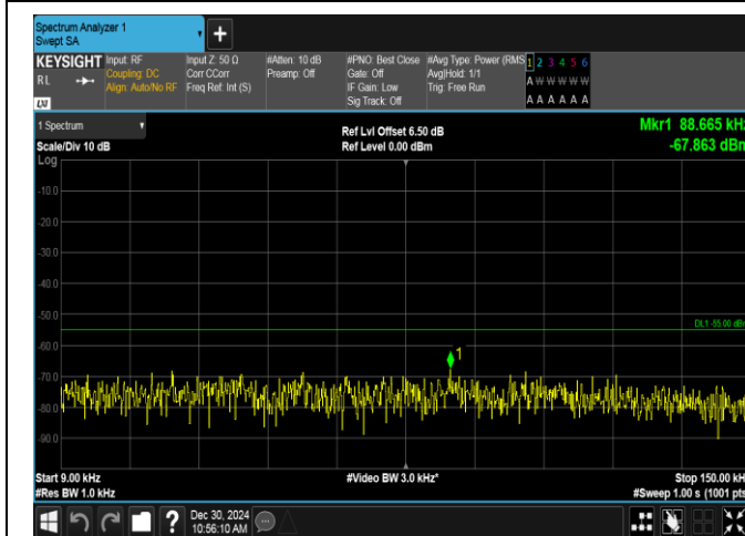
Band7-20MHz-16QAM-21100-1RB#0-0.009~0.15-PASS
