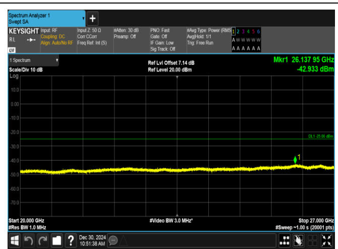
Band7-20MHz-QPSK-20850-1RB#99-20000~27000-PASS
