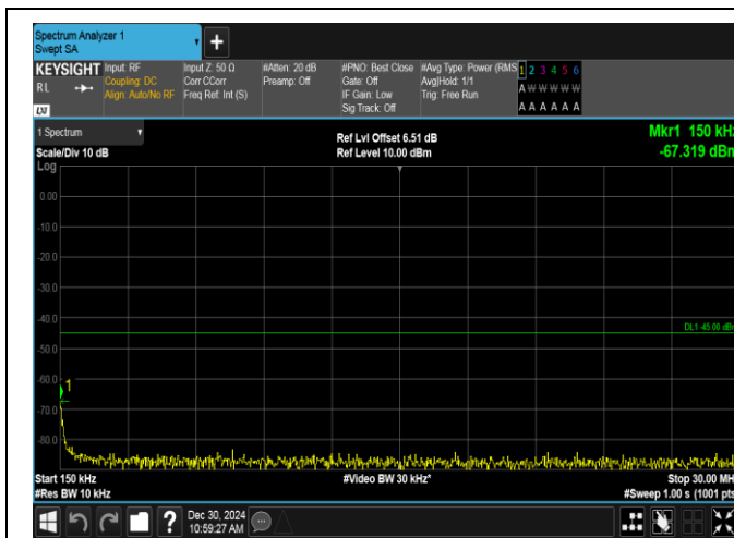
Band7-20MHz-QPSK-21100-100RB#0-0.15~30-PASS
