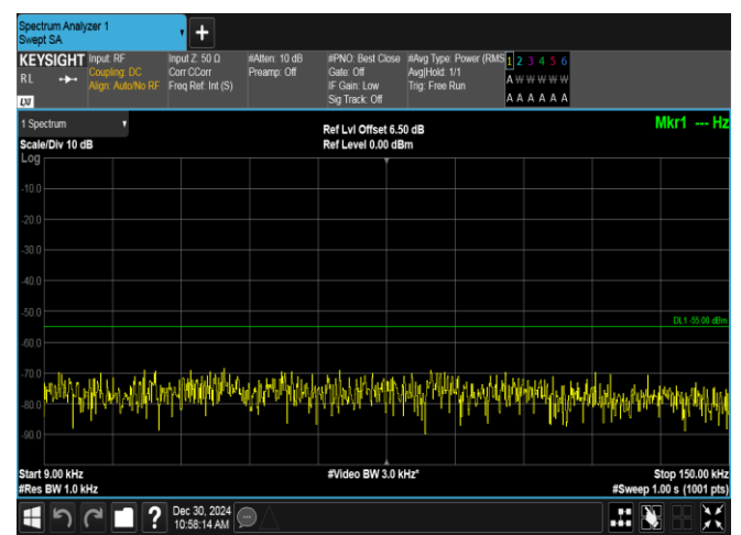
Band7-20MHz-16QAM-21100-1RB#99-0.009~0.15-PASS
