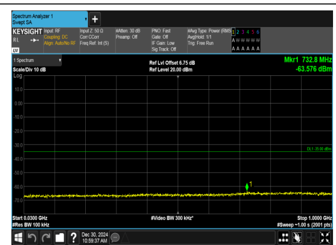
Band7-20MHz-QPSK-21100-100RB#0-30~1000-PASS
