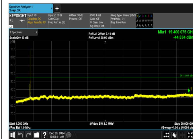
Band7-20MHz-16QAM-20850-100RB#0-1000~20000-PAS
