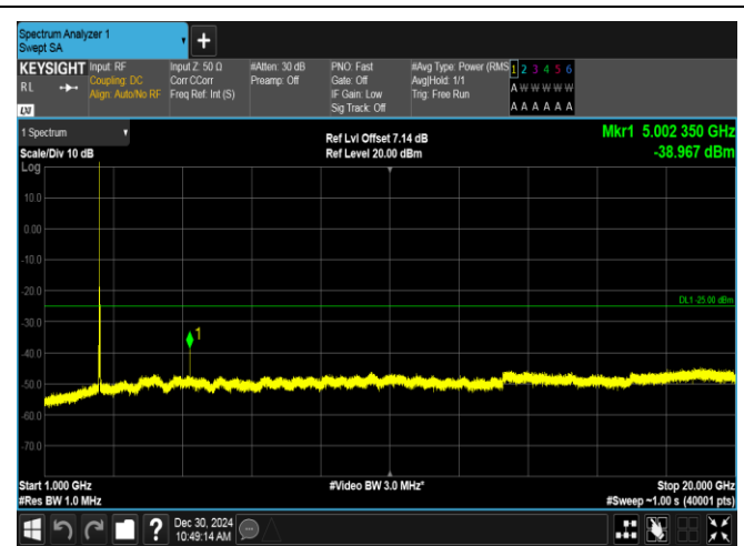
Band7-20MHz-QPSK-20850-1RB#0-1000~20000-PASS
