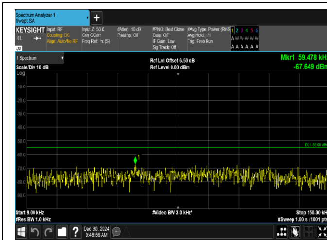
Band7-15MHz-QPSK-21100-1RB#74-0.009~0.15-PASS
