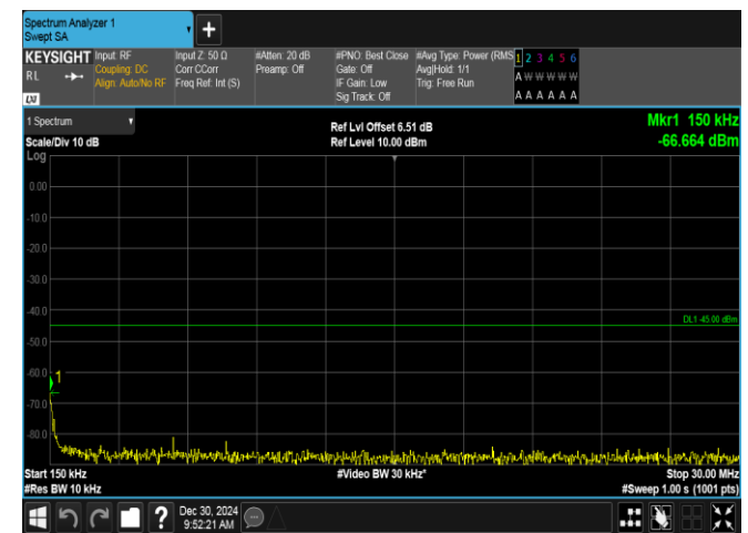
Band7-15MHz-16QAM-21100-75RB#0-0.15~30-PASS
