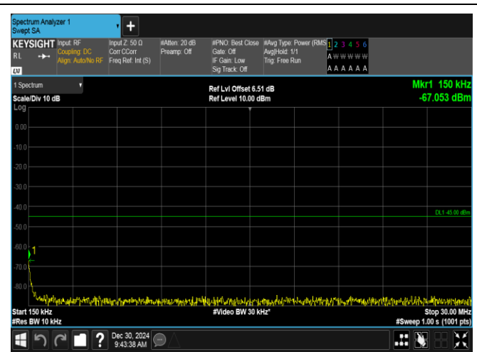
Band7-15MHz-16QAM-20825-1RB#74-0.15~30-PASS
