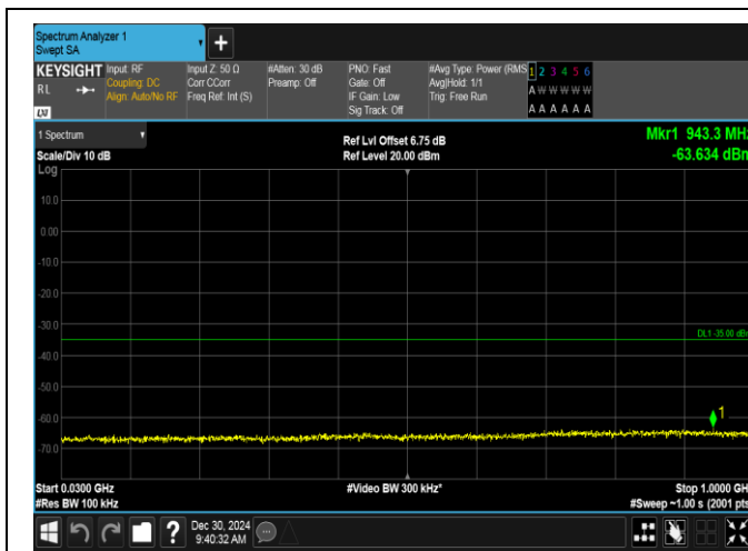
Band7-15MHz-QPSK-20825-1RB#0-30~1000-PASS
