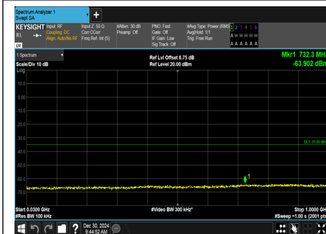
Band7-15MHz-QPSK-20825-75RB#0-30~1000-PASS
