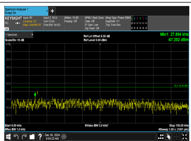
Band7-15MHz-16QAM-21375-1RB#0-0.009~0.15-PASS
