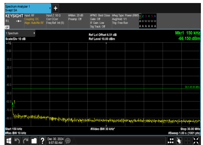
Band7-15MHz-QPSK-21375-75RB#0-0.15~30-PASS
