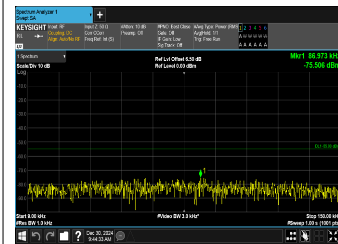
Band7-15MHz-QPSK-20825-75RB#0-0.009~0.15-PASS
