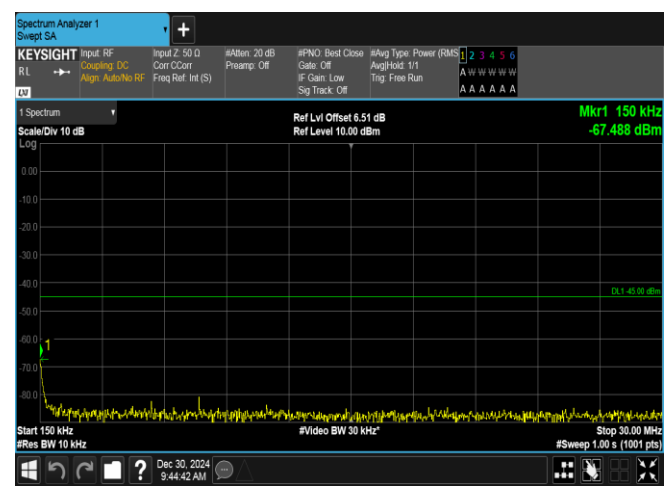
Band7-15MHz-QPSK-20825-75RB#0-0.15~30-PASS
