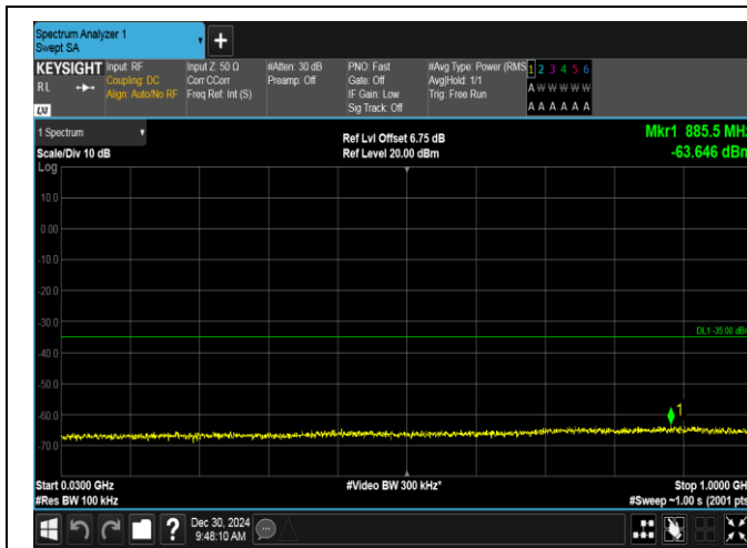
Band7-15MHz-16QAM-21100-1RB#0-30~1000-PASS
