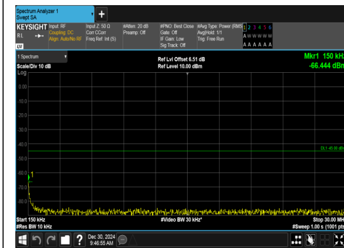
Band7-15MHz-QPSK-21100-1RB#0-0.15~30~PASS
