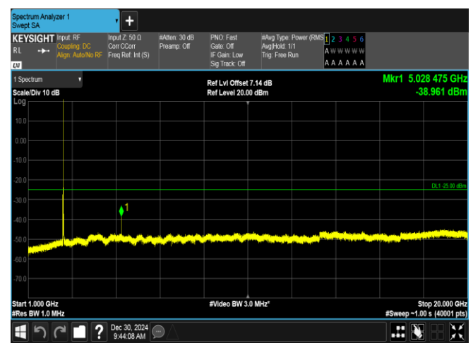
Band7-15MHz-16QAM-20825-1RB#74-1000~20000-PASS
