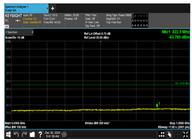
Band7-15MHz-16QAM-20825-1RB#0-30~1000-PASS
