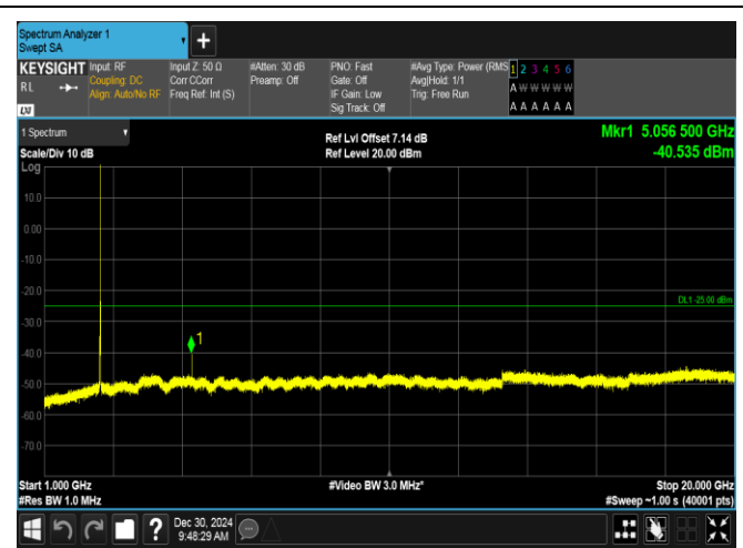
Band7-15MHz-16QAM-21100-1RB#0-1000~20000-PASS
