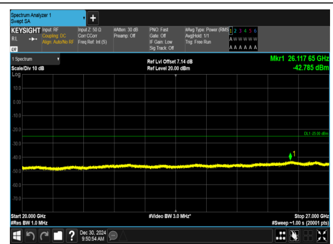
Band7-15MHz-16QAM-21100-1RB#74-20000~27000-PAS S
