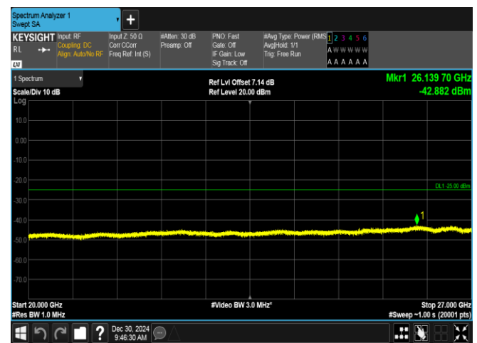
Band7-15MHz-16QAM-20825-75RB#0-20000~27000-PAS S
