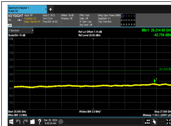
Band7-15MHz-QPSK-20825-75RB#0-20000~27000-PASS
