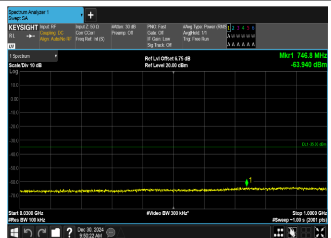
Band7-15MHz-16QAM-21100-1RB#74-30~1000-PASS
