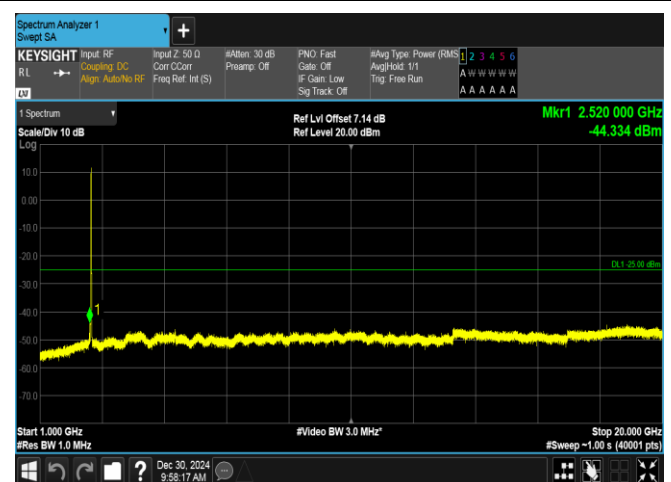
Band7-15MHz-QPSK-21375-75RB#0-1000~20000-PASS
