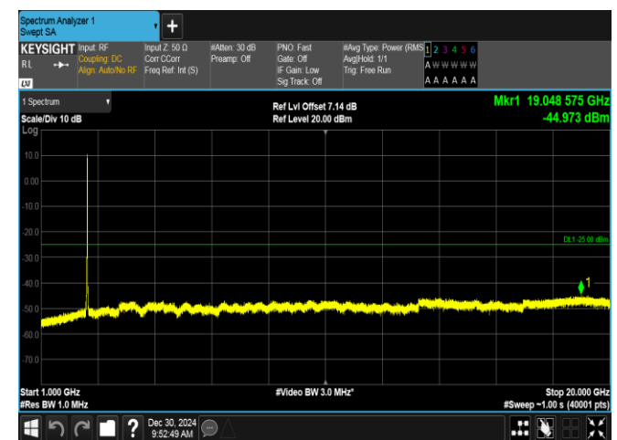
Band7-15MHz-16QAM-21100-75RB#0-1000~20000-PASS
