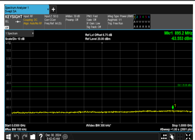
Band7-15MHz-QPSK-20825-1RB#74-30~1000-PASS
