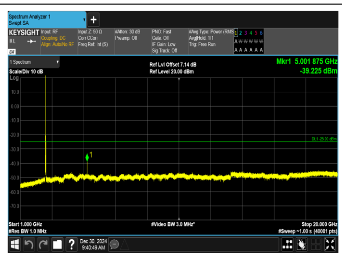
Band7-15MHz-QPSK-20825-1RB#0-1000~20000-PASS
