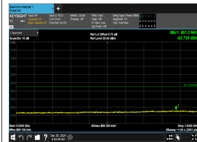
Band7-15MHz-16QAM-20825-1RB#74-30~1000-PASS
