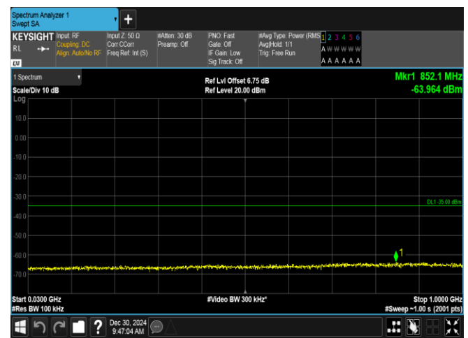
Band7-15MHz-QPSK-21100-1RB#0-30~1000~PASS
