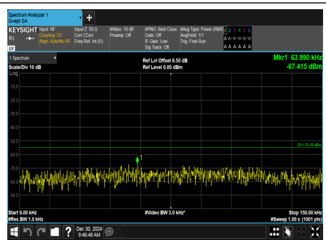
Band7-15MHz-QPSK-21100-1RB#0-0.009~0.15~PASS
