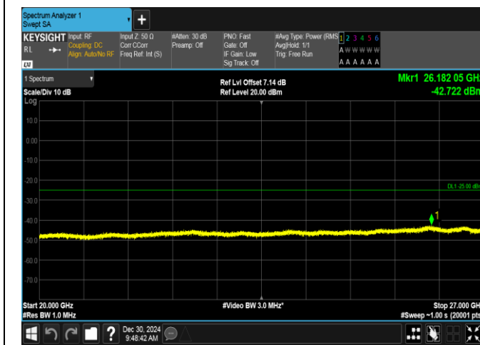
Band7-15MHz-16QAM-21100-1RB#0-20000~27000-PASS
