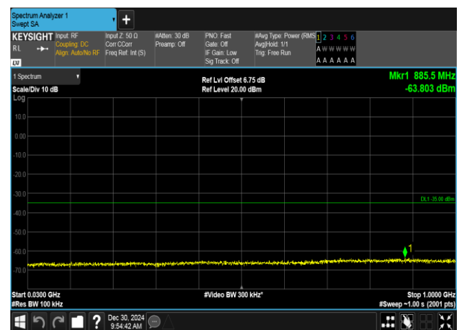
Band7-15MHz-16QAM-21375-1RB#0-30~1000-PASS
