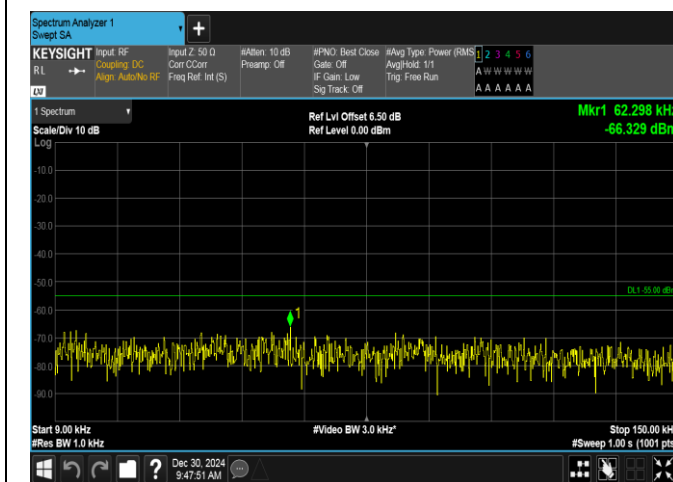
Band7-15MHz-16QAM-21100-1RB#0-0.009~0.15-PASS
