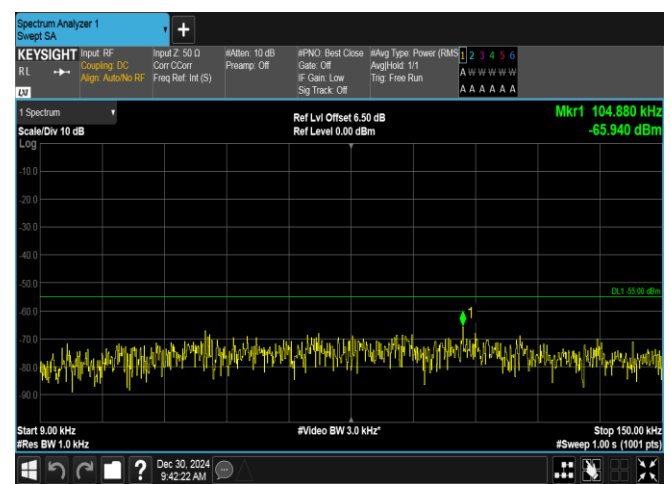
Band7-15MHz-QPSK-20825-1RB#74-0.009~0.15-PASS
