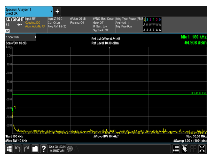
Band7-15MHz-QPSK-21100-1RB#74-0.15~30-PASS
