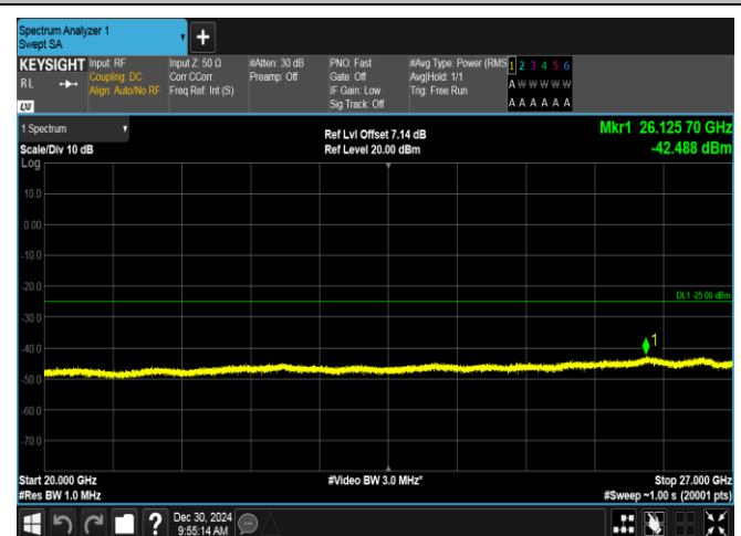
Band7-15MHz-16QAM-21375-1RB#0-20000~27000-PASS
