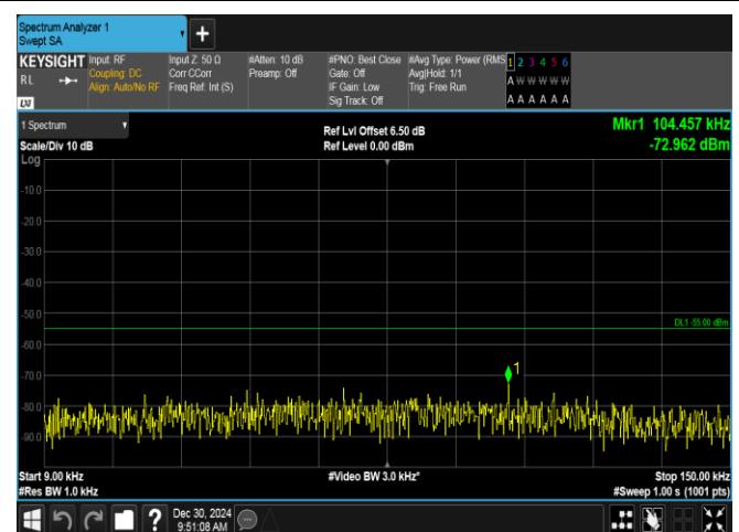
Band7-15MHz-QPSK-21100-75RB#0-0.009~0.15-PASS
