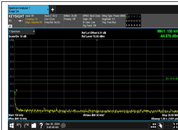
Band7-15MHz-16QAM-20825-75RB#0-0.15~30-PASS
