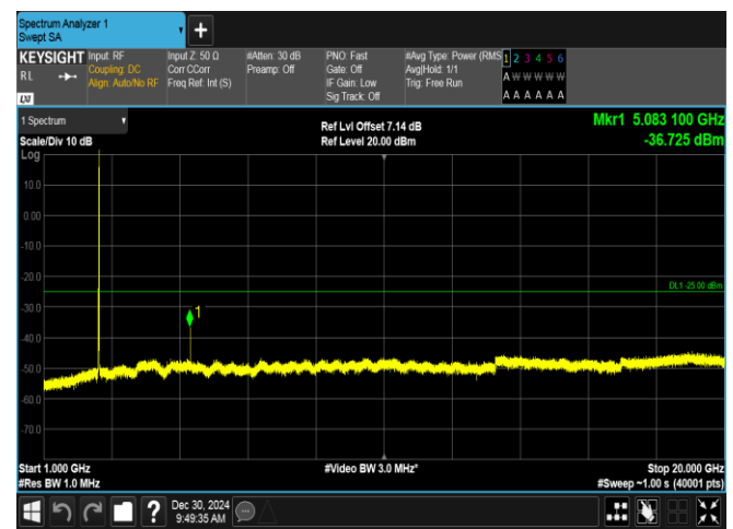
Band7-15MHz-QPSK-21100-1RB#74-1000~20000-PASS
