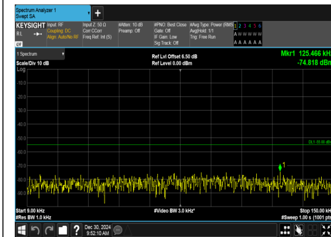
Band7-15MHz-16QAM-21100-75RB#0-0.009~0.15-PASS
