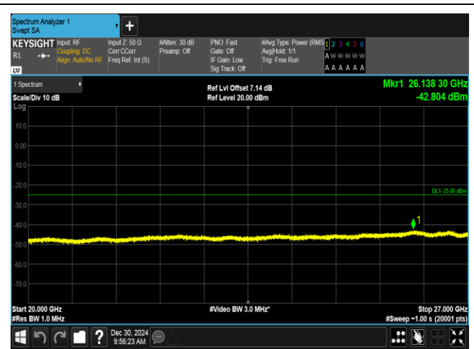
Band7-15MHz-QPSK-21375-1RB#74-20000~27000-PASS
