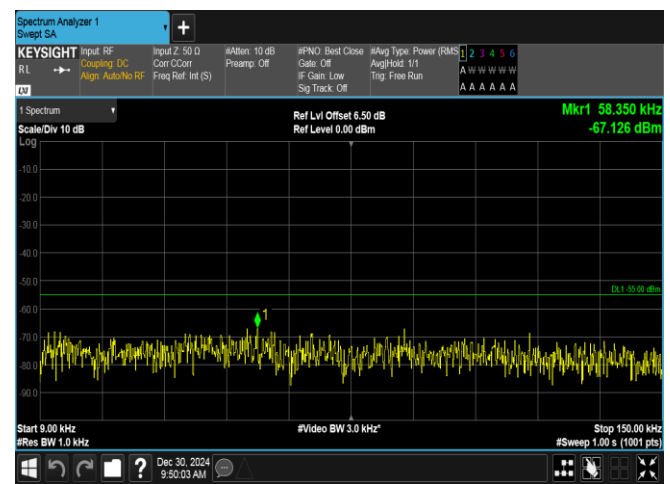
Band7-15MHz-16QAM-21100-1RB#74-0.009~0.15-PASS
