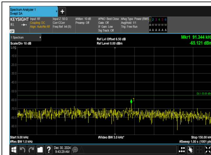
Band7-15MHz-16QAM-20825-1RB#74-0.009~0.15-PASS
