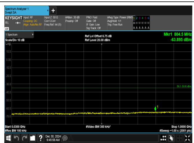
Band7-15MHz-16QAM-20825-75RB#0-30~1000-PASS
