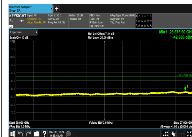
Band7-15MHz-QPSK-21100-1RB#74-20000~27000-PASS
