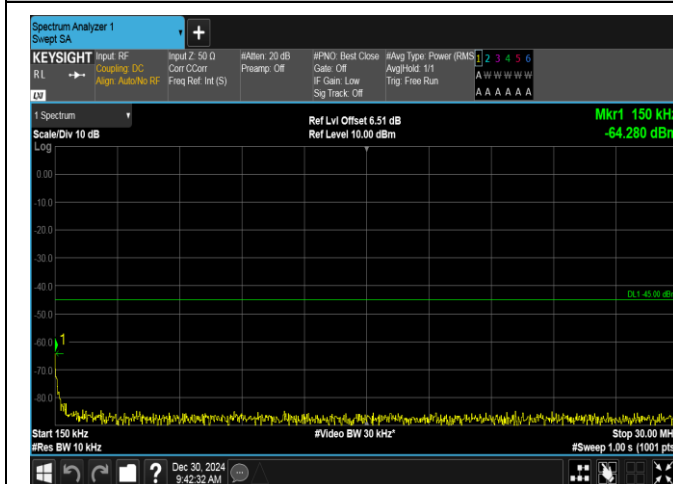
Band7-15MHz-QPSK-20825-1RB#74-0.15~30-PASS
