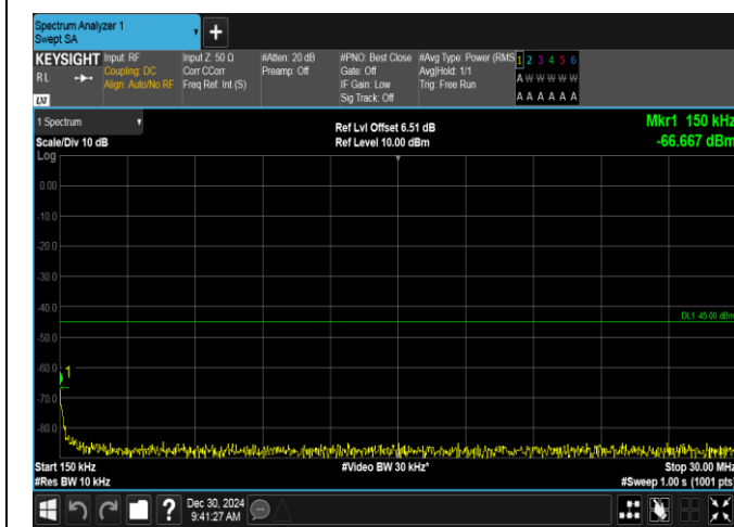
Band7-15MHz-16QAM-20825-1RB#0-0.15~30-PASS
