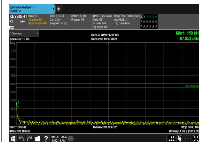
Band7-15MHz-16QAM-21100-1RB#74-0.15~30-PASS
