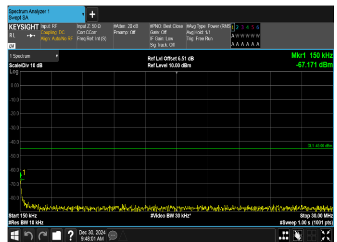
Band7-15MHz-16QAM-21100-1RB#0-0.15~30-PASS
