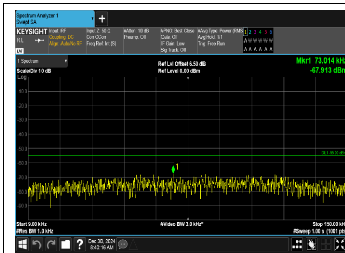
Band7-10MHz-QPSK-21100-1RB#49-0.009~0.15-PASS
