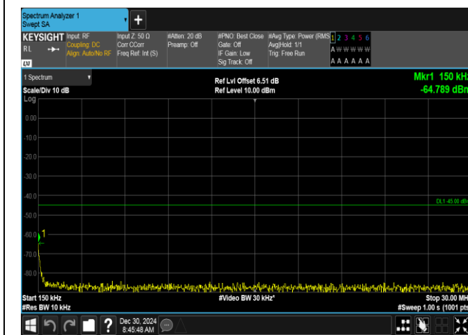
Band7-10MHz-16QAM-21400-1RB#0-0.15~30-PASS
