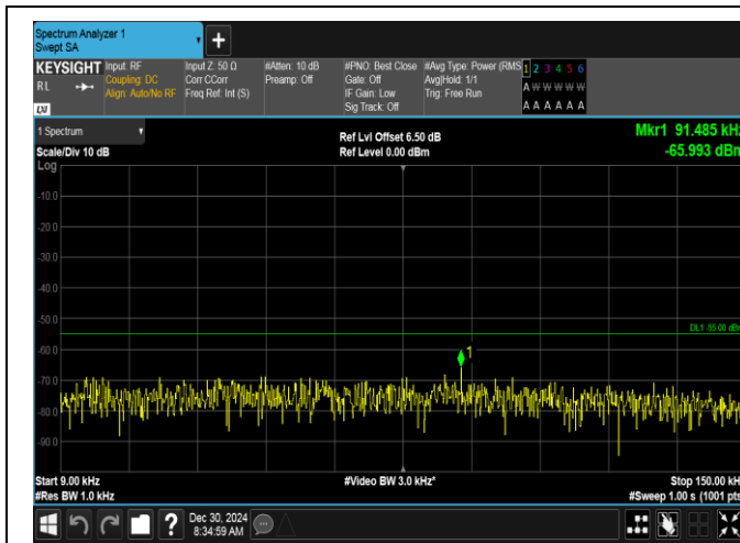
Band7-10MHz-16QAM-20800-1RB#49-0.009~0.15-PASS
