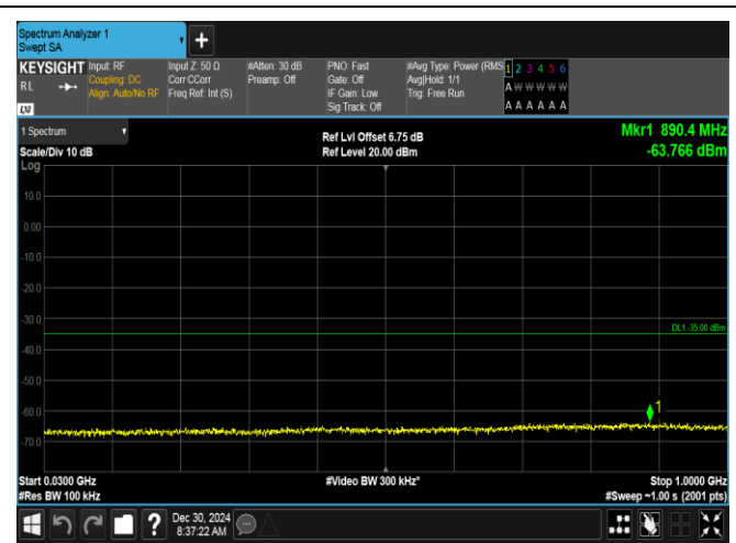
Band7-10MHz-16QAM-20800-50RB#0-30~1000-PASS
