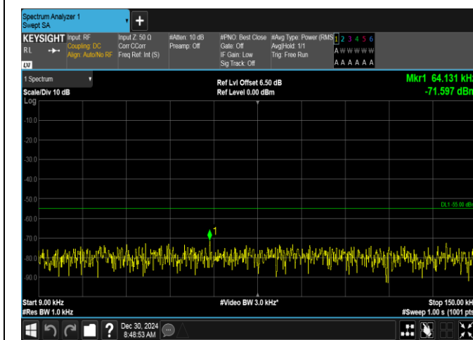
Band7-10MHz-QPSK-21400-50RB#0-0.009~0.15-PASS
