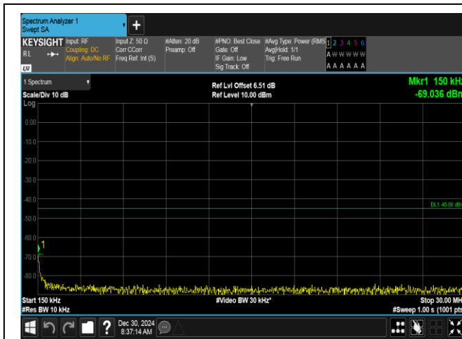
Band7-10MHz-16QAM-20800-50RB#0-0.15~30-PASS
