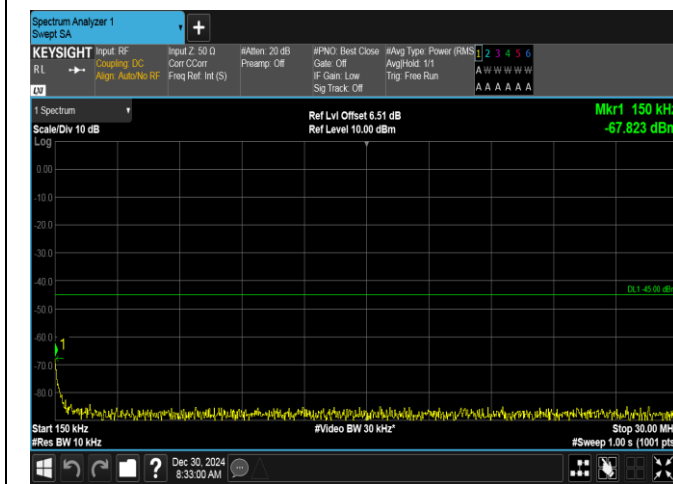
Band7-10MHz-16QAM-20800-1RB#0-0.15~30-PASS
