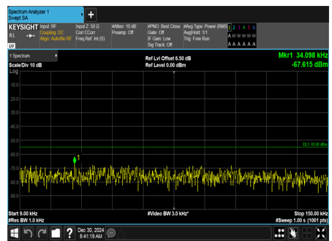
Band7-10MHz-16QAM-21100-1RB#49-0.009~0.15-PASS
