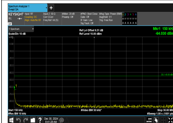
Band7-10MHz-16QAM-21100-1RB#49-0.15~30-PASS
