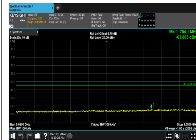
Band7-10MHz-QPSK-21100-1RB#49-30~1000-PASS
