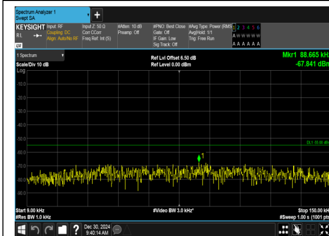
Band7-15MHz-QPSK-20825-1RB#0-0.009~0.15-PASS
