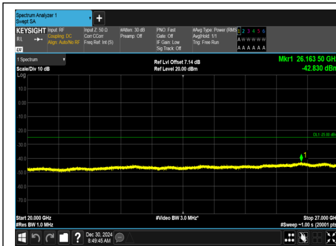
Band7-10MHz-QPSK-21400-50RB#0-20000~27000-PASS
