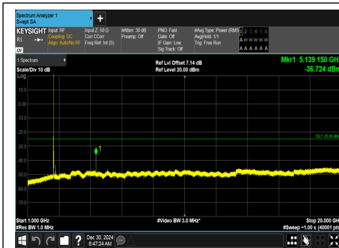
Band7-10MHz-QPSK-21400-1RB#49-1000~20000-PASS
