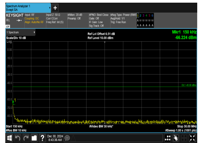
Band7-10MHz-16QAM-21100-50RB#0-0.15~30-PASS
