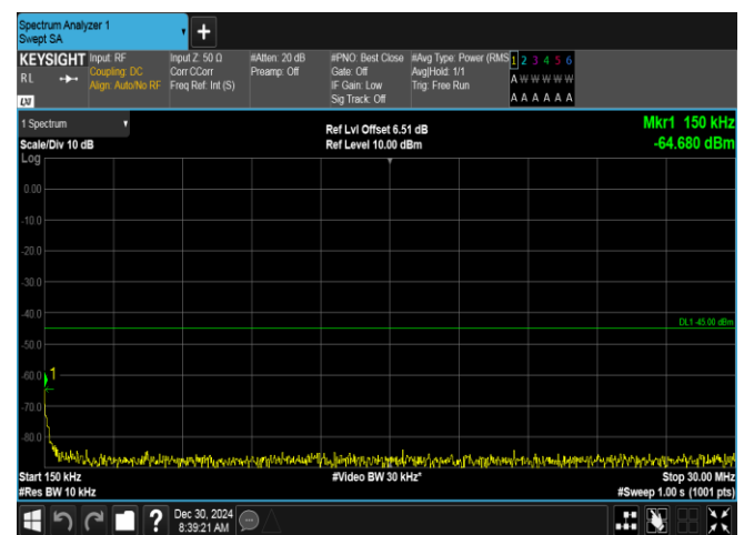
Band7-10MHz-16QAM-21100-1RB#0-0.15~30-PASS
