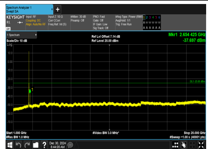
Band7-10MHz-16QAM-21100-50RB#0-1000~20000-PASS
