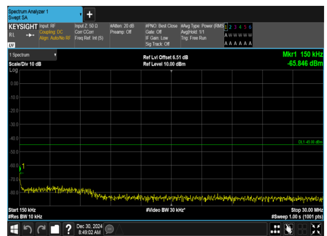
Band7-10MHz-QPSK-21400-50RB#0-0.15~30-PASS
