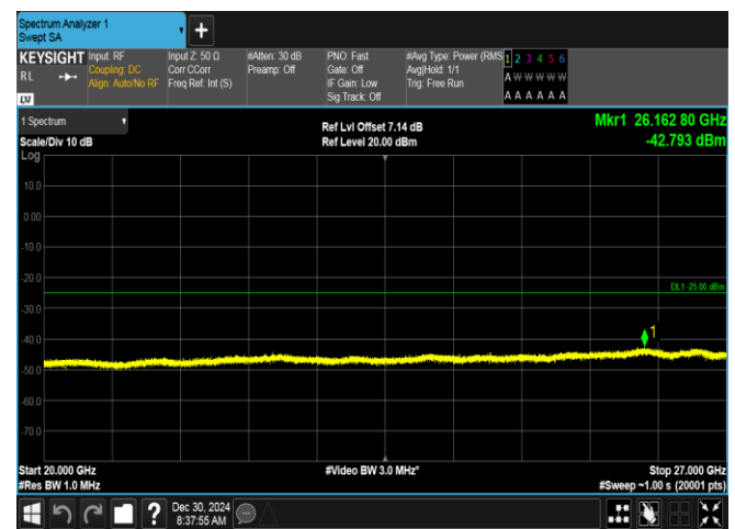
Band7-10MHz-16QAM-20800-50RB#0-20000~27000-PAS S
