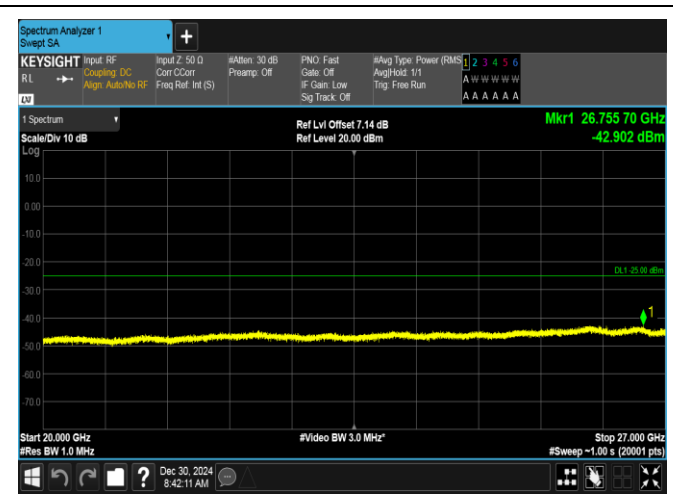
Band7-10MHz-16QAM-21100-1RB#49-20000~27000-PAS S
