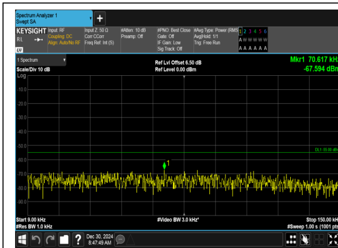
Band7-10MHz-16QAM-21400-1RB#49-0.009~0.15-PASS
