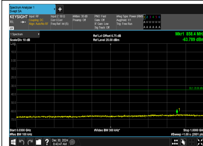
Band7-10MHz-16QAM-21100-50RB#0-30~1000-PASS
