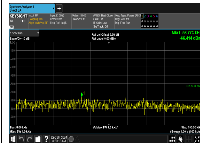
Band7-10MHz-16QAM-21100-1RB#0-0.009~0.15-PASS
