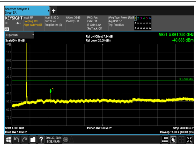
Band7-10MHz-16QAM-21100-1RB#0-1000~20000-PASS
