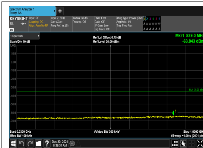
Band7-10MHz-16QAM-21100-1RB#0-30~1000-PASS
