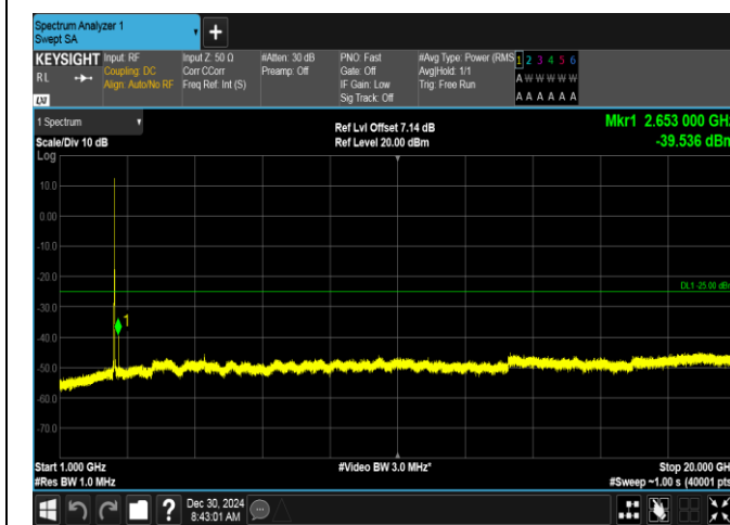
Band7-10MHz-QPSK-21100-50RB#0-1000~20000-PASS
