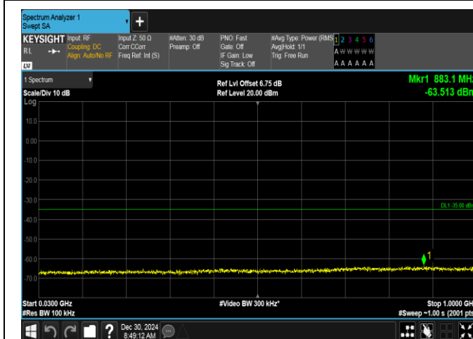
Band7-10MHz-QPSK-21400-50RB#0-30~1000-PASS
