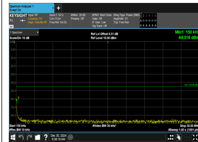
Band7-10MHz-QPSK-21100-1RB#0-0.15~30-PASS
