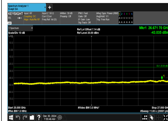
Band7-5MHz-QPSK-21425-1RB#0-20000~27000-PASS
