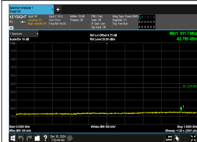
Band7-5MHz-16QAM-21100-25RB#0-30~1000-PASS
