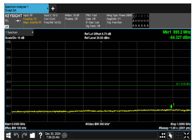
Band7-5MHz-16QAM-21425-1RB#0-30~1000-PASS
