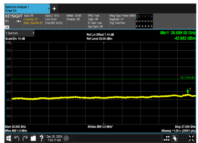
Band7-5MHz-QPSK-21100-25RB#0-20000~27000-PASS
