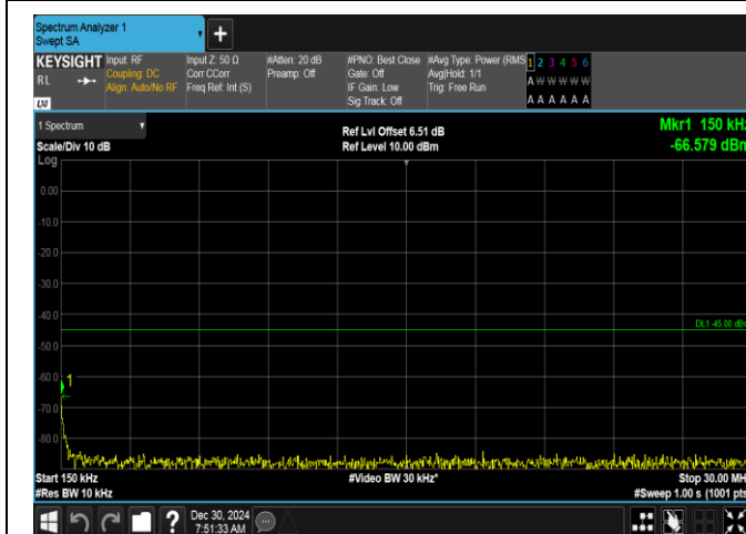
Band7-5MHz-16QAM-21100-1RB#24-0.15~30-PASS
