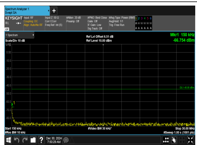
Band7-5MHz-QPSK-21100-1RB#24-0.15~30-PASS
