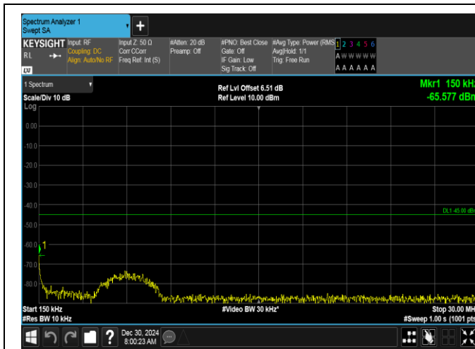
Band7-5MHz-16QAM-21425-25RB#0-0.15~30-PASS
