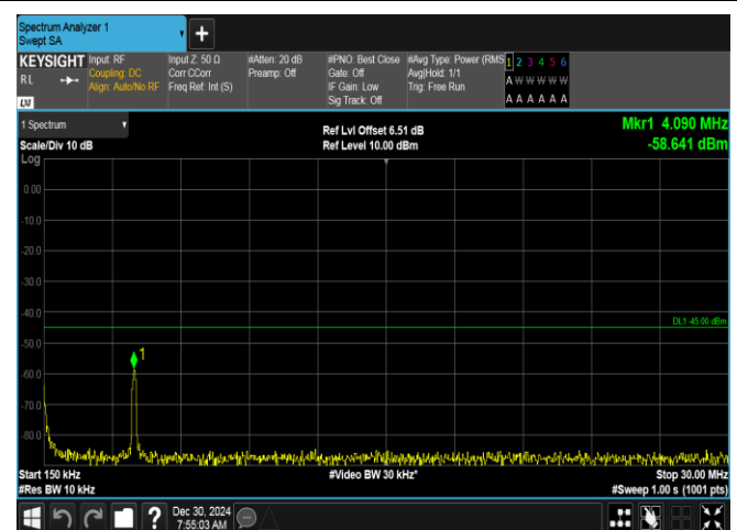
Band7-5MHz-QPSK-21425-1RB#0-0.15~30-PASS
