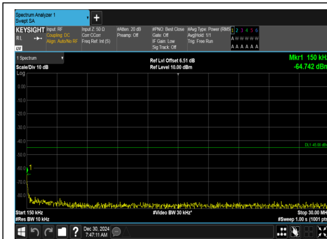
Band7-5MHz-16QAM-20775-25RB#0-0.15~30-PASS
