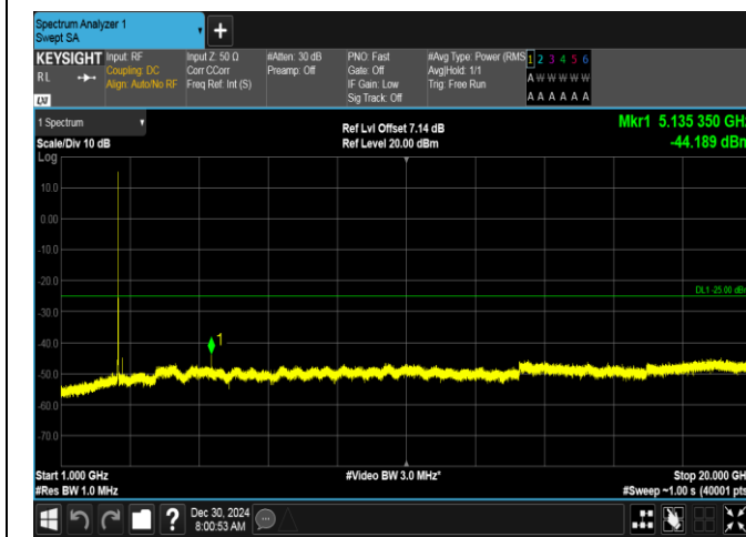
Band7-5MHz-16QAM-21425-25RB#0-1000~20000-PASS
