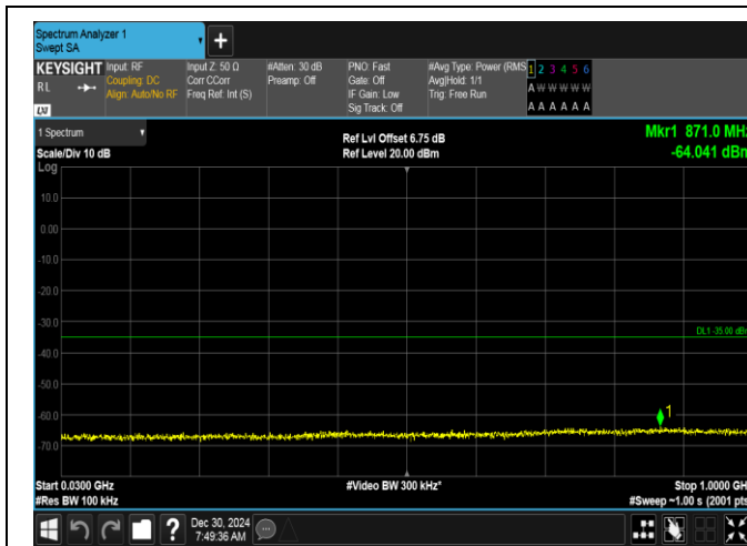
Band7-5MHz-16QAM-21100-1RB#0-30~1000-PASS
