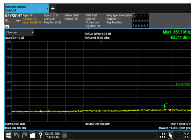
Band7-5MHz-16QAM-20775-1RB#0-30~1000-PASS
