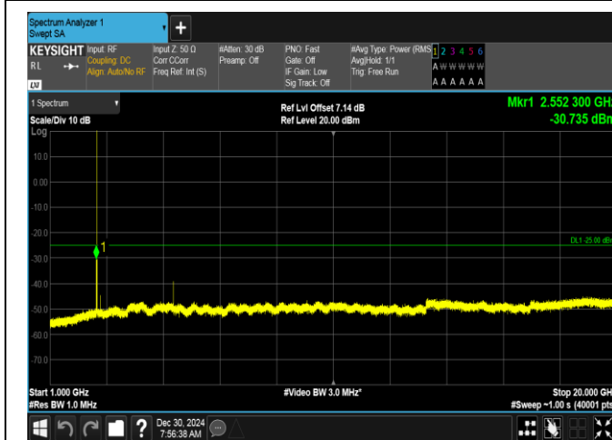
Band7-5MHz-16QAM-21425-1RB#0-1000~20000-PASS
