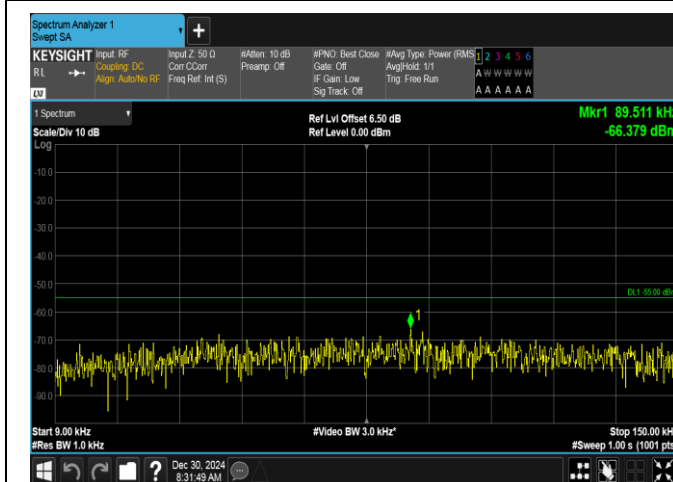
Band7-10MHz-QPSK-20800-1RB#0-0.009~0.15-PASS
