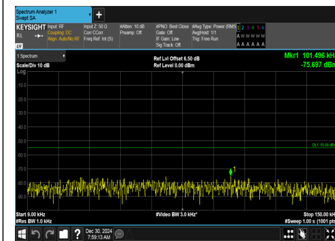
Band7-5MHz-QPSK-21425-25RB#0-0.009~0.15-PASS
