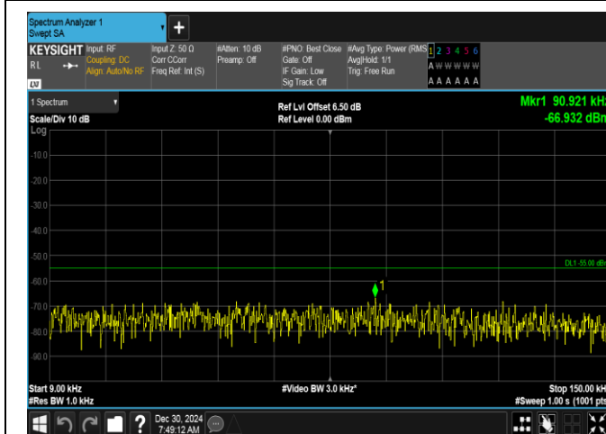
Band7-5MHz-16QAM-21100-1RB#0-0.009~0.15-PASS
