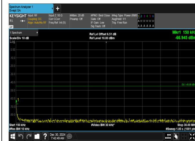
Band7-5MHz-16QAM-20775-1RB#0-0.15~30-PASS
