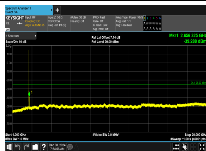
Band7-5MHz-16QAM-21100-25RB#0-1000~20000-PASS
