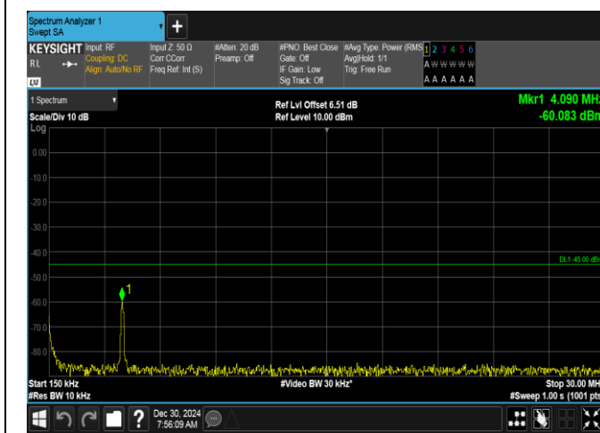
Band7-5MHz-16QAM-21425-1RB#0-0.15~30-PASS
