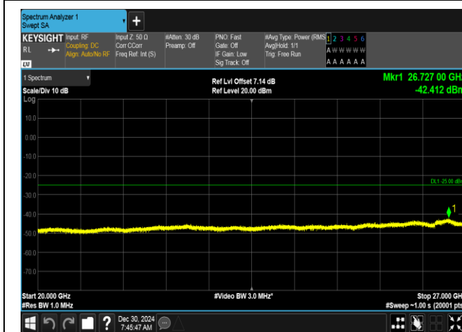
Band7-5MHz-16QAM-20775-1RB#24-20000~27000-PASS
