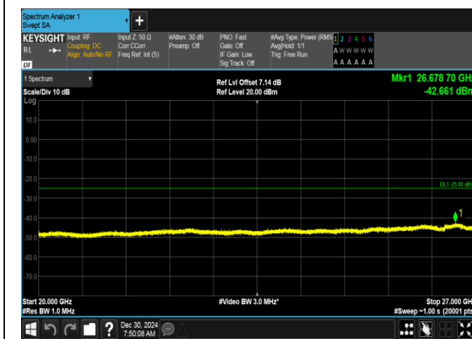
Band7-5MHz-16QAM-21100-1RB#0-20000~27000-PASS
