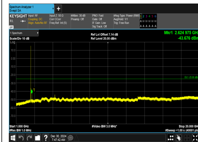
Band7-5MHz-16QAM-20775-25RB#0-1000~20000-PASS
