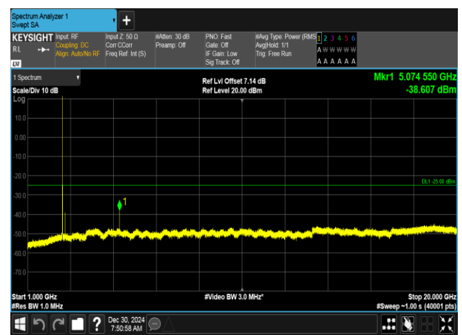
Band7-5MHz-QPSK-21100-1RB#24-1000~20000-PASS
