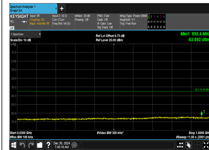
Band7-5MHz-16QAM-20775-1RB#24-30~1000-PASS
