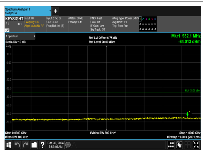
Band7-5MHz-QPSK-21100-25RB#0-30~1000-PASS
