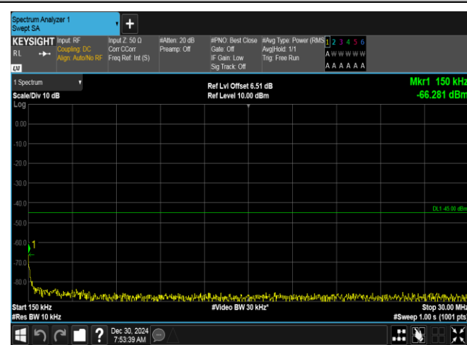
Band7-5MHz-16QAM-21100-25RB#0-0.15~30-PASS
