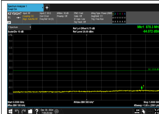
Band7-5MHz-QPSK-21425-25RB#0-30~1000-PASS
