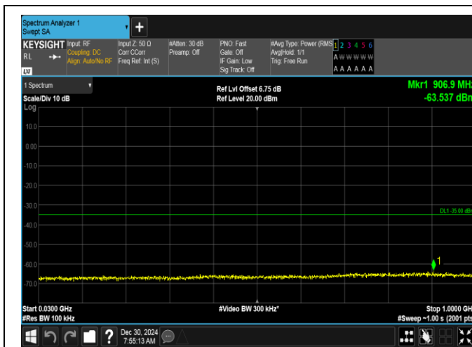
Band7-5MHz-QPSK-21425-1RB#0-30~1000-PASS
