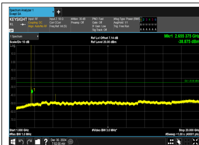
Band7-5MHz-16QAM-21100-1RB#24-1000~20000-PASS
