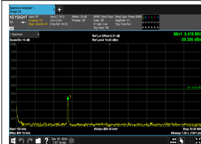
Band7-5MHz-QPSK-21425-1RB#24-0.15~30-PASS
