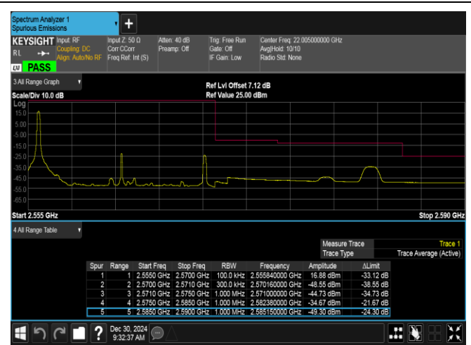
Band7-15MHz-16QAM-21375-1RB#0-PASS
