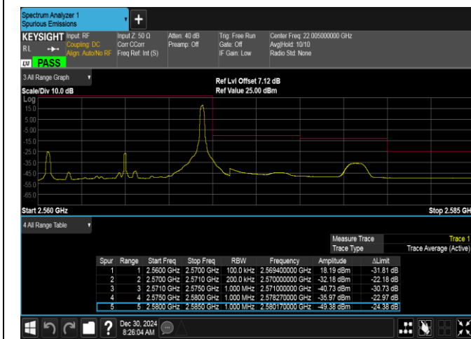
Band7-10MHz-QPSK-21400-1RB#49-PASS
