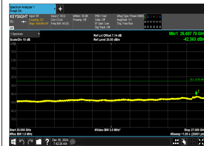
Band7-5MHz-QPSK-20775-1RB#0-20000~27000-PASS
