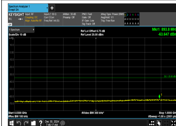
Band7-5MHz-QPSK-20775-25RB#0-30~1000-PASS
