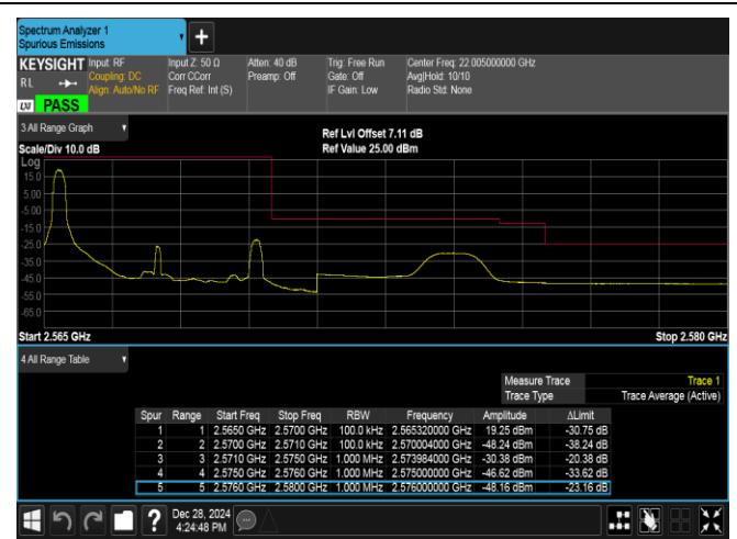
Band7-5MHz-QPSK-21425-1RB#0-PASS
