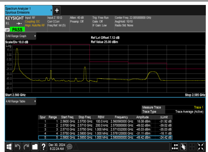
Band7-10MHz-QPSK-21400-1RB#0-PASS
