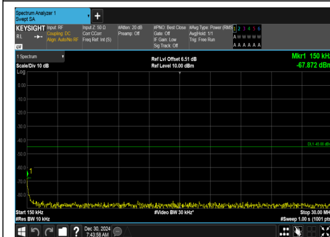
Band7-5MHz-QPSK-20775-1RB#24-0.15~30-PASS
