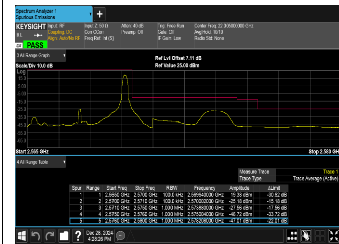
Band7-5MHz-QPSK-21425-1RB#24-PASS
