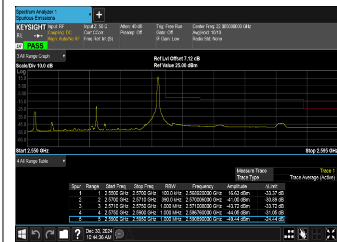
Band7-20MHz-16QAM-21350-1RB#99-PASS
