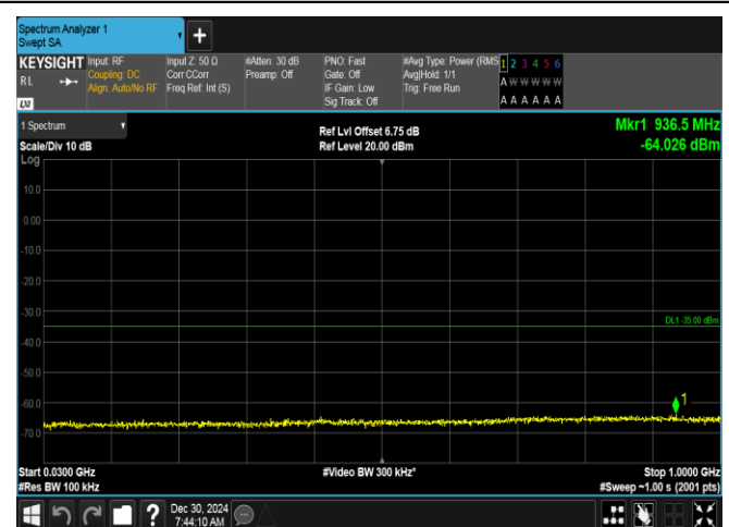
Band7-5MHz-QPSK-20775-1RB#24-30~1000-PASS
