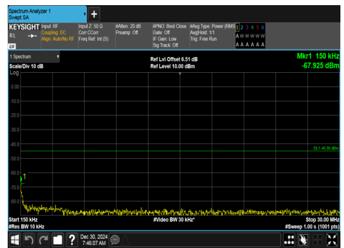
Band7-5MHz-QPSK-20775-25RB#0-0.15~30-PASS
