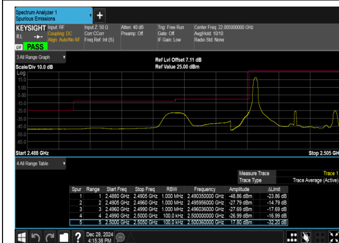
Band7-5MHz-16QAM-20775-1RB#0-PASS
