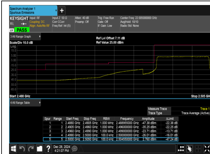
Band7-5MHz-QPSK-20775-25RB#0-PASS
