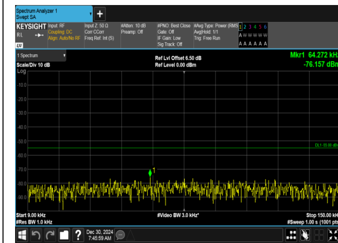
Band7-5MHz-QPSK-20775-25RB#0-0.009~0.15-PASS
