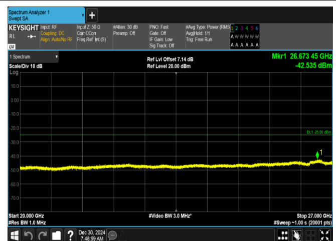
Band7-5MHz-QPSK-21100-1RB#0-20000~27000-PASS
