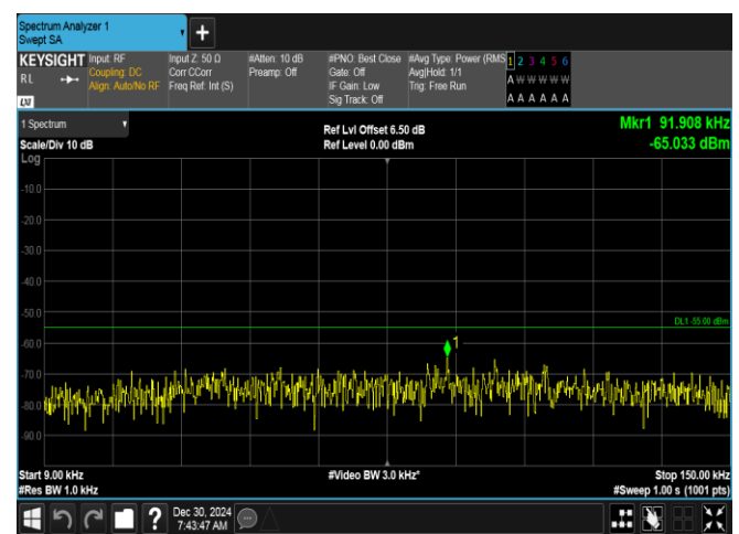
Band7-5MHz-QPSK-20775-1RB#24-0.009~0.15-PASS
