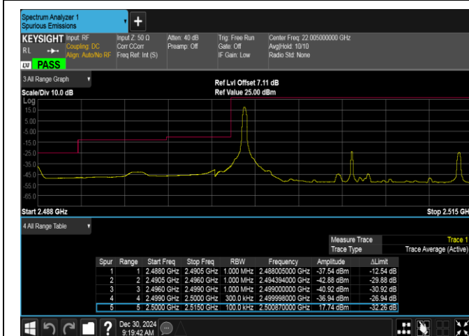
Band7-15MHz-QPSK-20825-1RB#0-PASS
