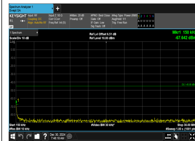
Band7-5MHz-QPSK-21100-1RB#0-0.15~30-PASS
