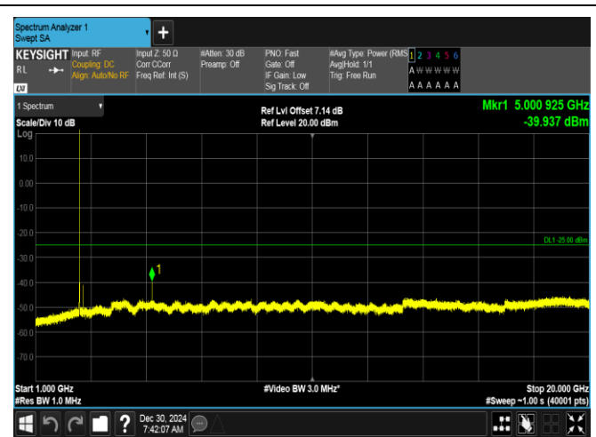
Band7-5MHz-QPSK-20775-1RB#0-1000~20000-PASS
