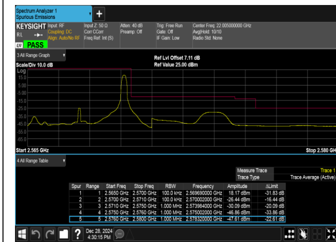
Band7-5MHz-16QAM-21425-1RB#24-PASS
