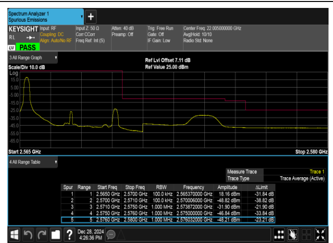
Band7-5MHz-16QAM-21425-1RB#0-PASS
