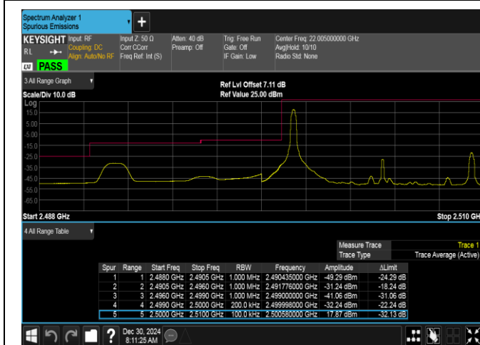
Band7-10MHz-QPSK-20800-1RB#0-PASS
