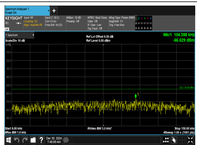
Band7-5MHz-QPSK-21100-1RB#0-0.009~0.15-PASS
