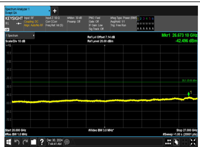
Band7-5MHz-QPSK-20775-1RB#24-20000~27000-PASS
