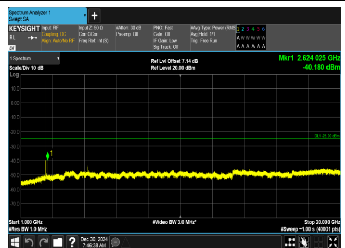
Band7-5MHz-QPSK-20775-25RB#0-1000~20000-PASS
