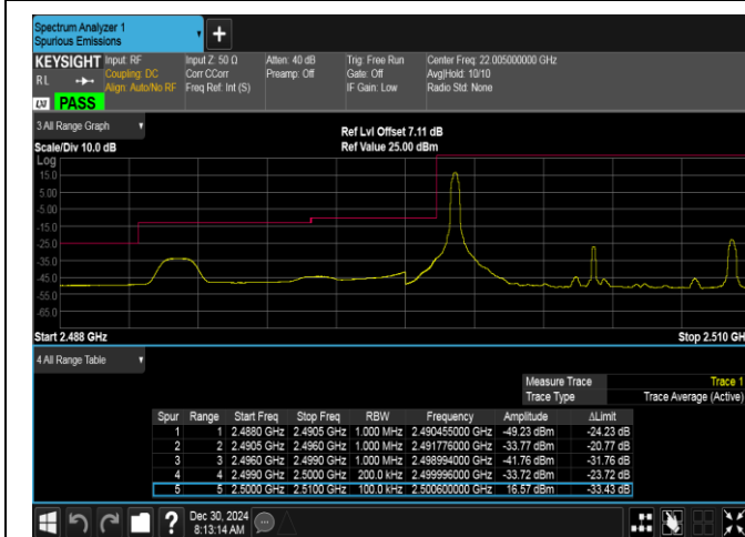
Band7-10MHz-16QAM-20800-1RB#0-PASS
