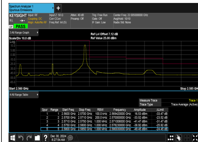
Band7-10MHz-16QAM-21400-1RB#49-PASS
