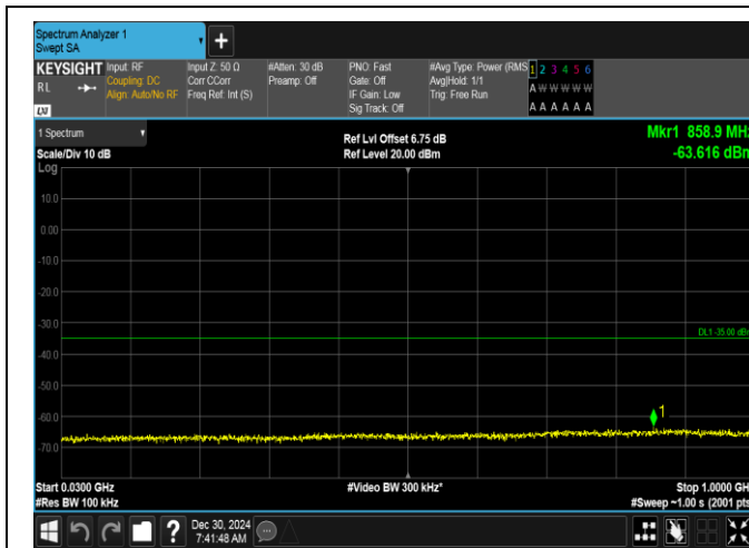
Band7-5MHz-QPSK-20775-1RB#0-30~1000-PASS
