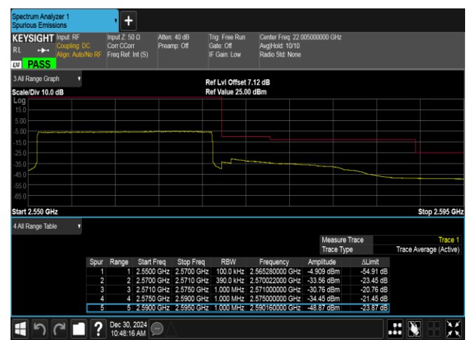
Band7-20MHz-16QAM-21350-100RB#0-PASS
