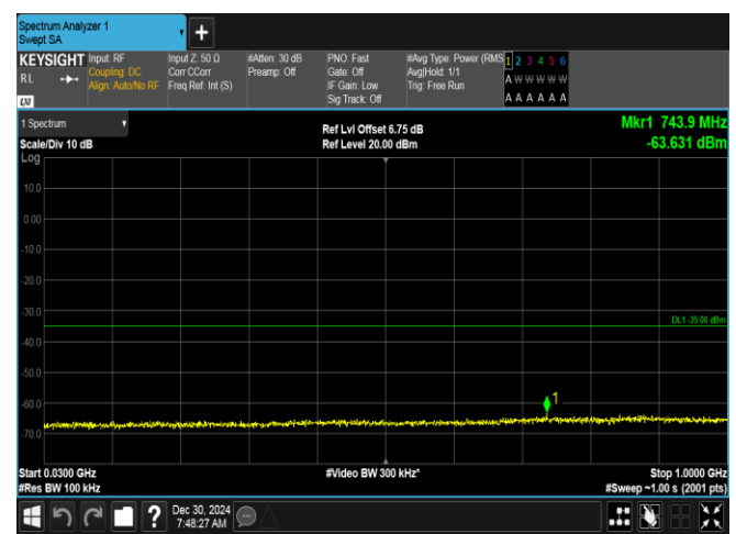
Band7-5MHz-QPSK-21100-1RB#0-30~1000-PASS
