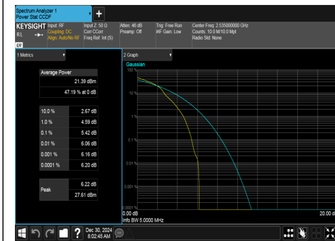
Band7-5MHz-16QAM-21100-1RB#0-PASS
