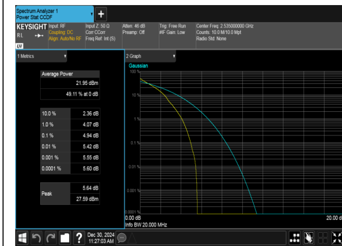
Band7-20MHz-QPSK-21100-1RB#0-PASS
