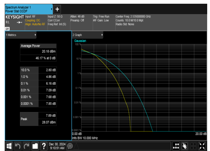
Band7-10MHz-16QAM-21100-50RB#0-PASS
