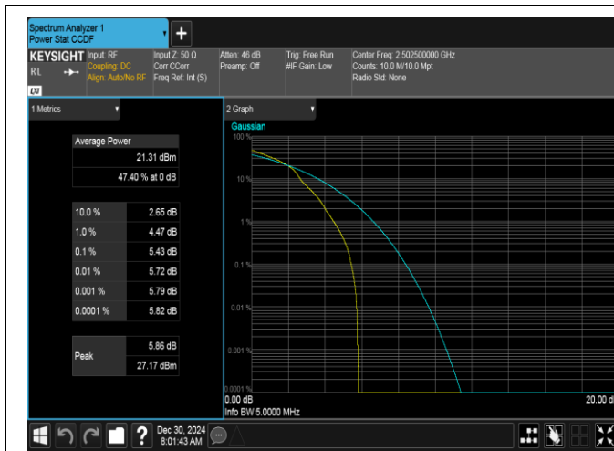
Band7-5MHz-16QAM-20775-1RB#0-PASS
