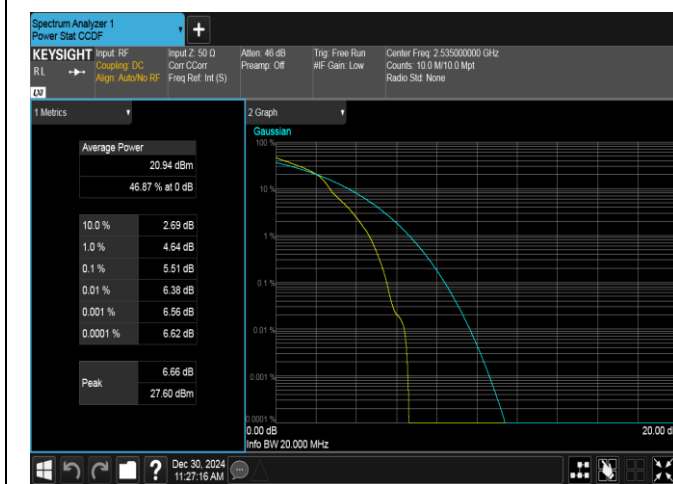
Band7-20MHz-16QAM-21100-1RB#0-PASS
