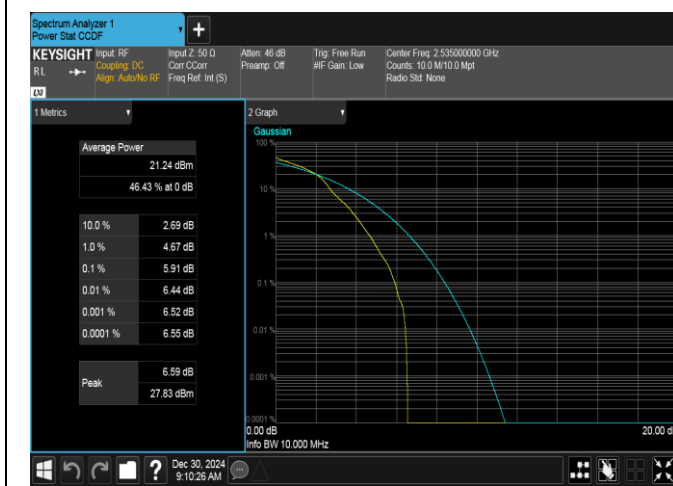
Band7-10MHz-16QAM-21100-1RB#0-PASS
