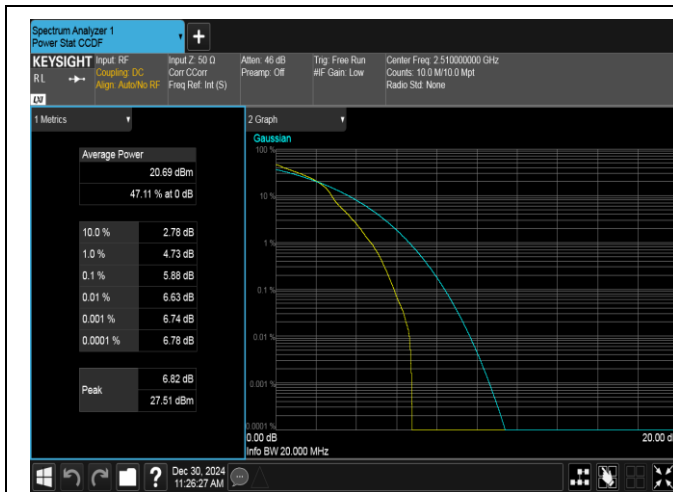
Band7-20MHz-16QAM-20850-1RB#0-PASS
