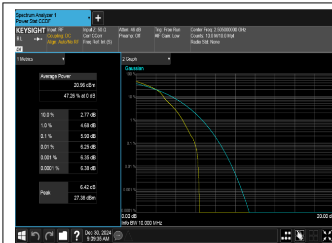
Band7-10MHz-16QAM-20800-1RB#0-PASS
