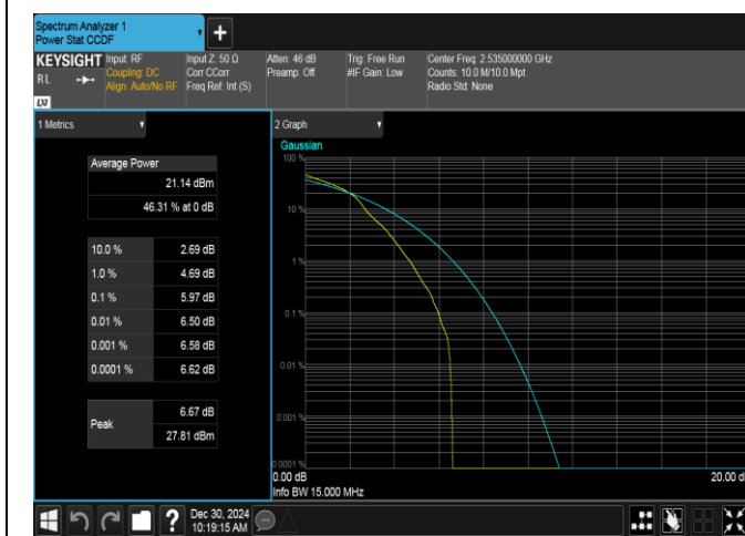
Band7-15MHz-16QAM-21100-1RB#0-PASS
