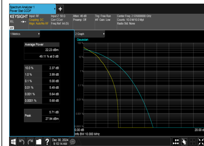
Band7-10MHz-QPSK-21100-1RB#0-PASS
