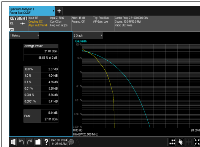
Band7-20MHz-QPSK-20850-1RB#0-PASS
