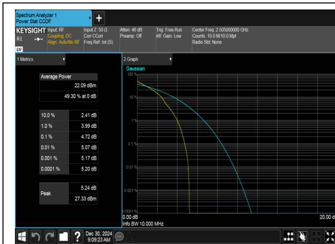
Band7-10MHz-QPSK-20800-1RB#0-PASS
