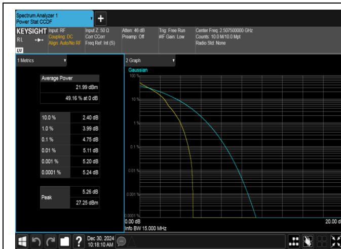
Band7-15MHz-QPSK-20825-1RB#0-PASS
