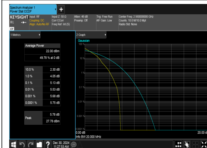
Band7-20MHz-QPSK-21350-1RB#0-PASS
