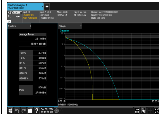
Band7-15MHz-QPSK-21100-1RB#0-PASS
