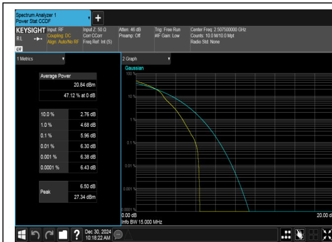
Band7-15MHz-16QAM-20825-1RB#0-PASS
