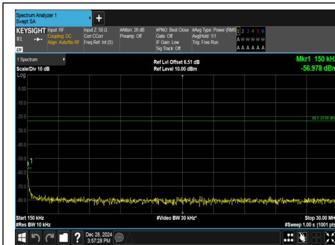
Band5-10MHz-16QAM-20600-50RB#0-0.15~30-PASS
