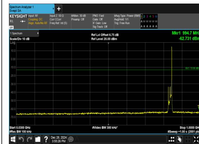
Band5-10MHz-16QAM-20600-1RB#49-30~1000-PASS
