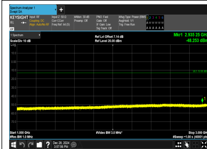
Band5-10MHz-16QAM-20600-50RB#0-1000~3000-PASS
