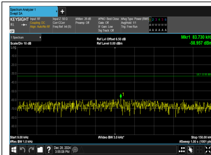
Band5-10MHz-16QAM-20600-1RB#49-0.009~0.15-PASS
