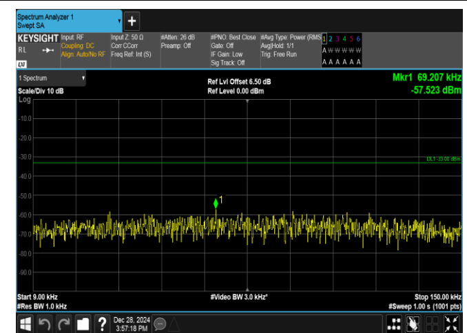
Band5-10MHz-16QAM-20600-50RB#0-0.009~0.15-PASS
