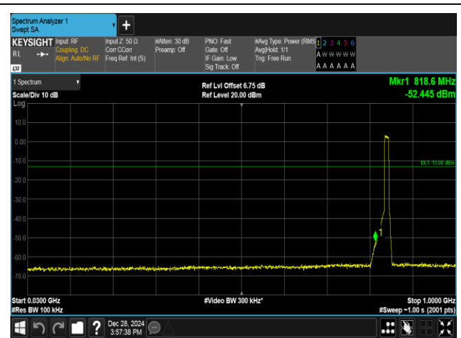
Band5-10MHz-16QAM-20600-50RB#0-30~1000-PASS
