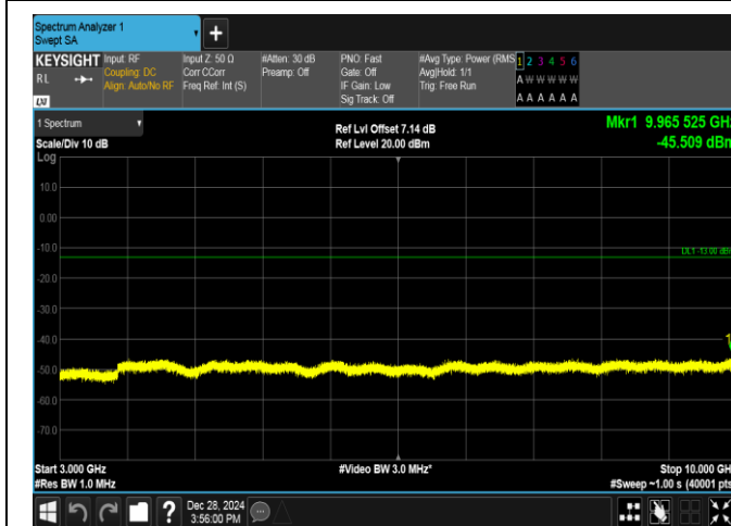
Band5-10MHz-16QAM-20600-1RB#49-3000~10000-PASS
