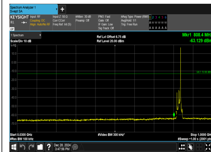
Band5-10MHz-QPSK-20525-1RB#49-30~1000-PASS
