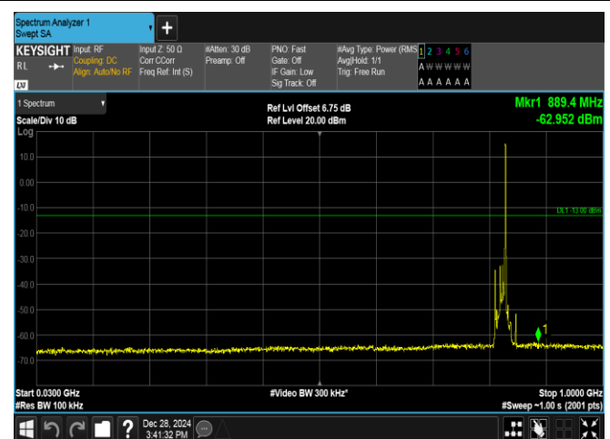
Band5-10MHz-QPSK-20450-1RB#49-30~1000-PASS
