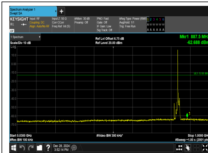
Band5-10MHz-QPSK-20600-1RB#0-30~1000-PASS
