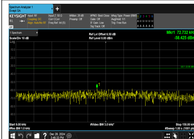
Band5-10MHz-16QAM-20525-1RB#0-0.009~0.15-PASS
