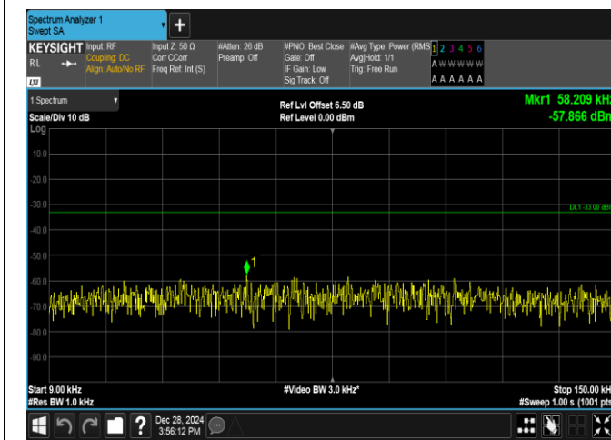
Band5-10MHz-QPSK-20600-50RB#0-0.009~0.15-PASS
