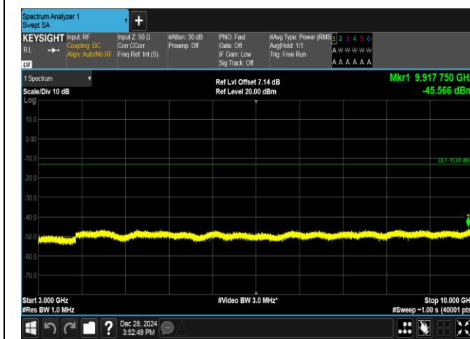
Band5-10MHz-QPSK-20600-1RB#0-3000~10000-PASS
