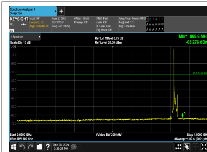
Band5-10MHz-QPSK-20450-1RB#0-30~1000-PASS
