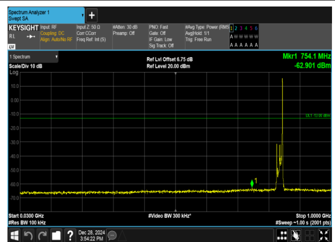
Band5-10MHz-QPSK-20600-1RB#49-30~1000-PASS
