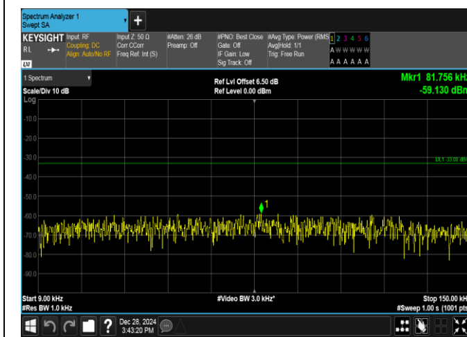
Band5-10MHz-QPSK-20450-50RB#0-0.009~0.15-PASS
