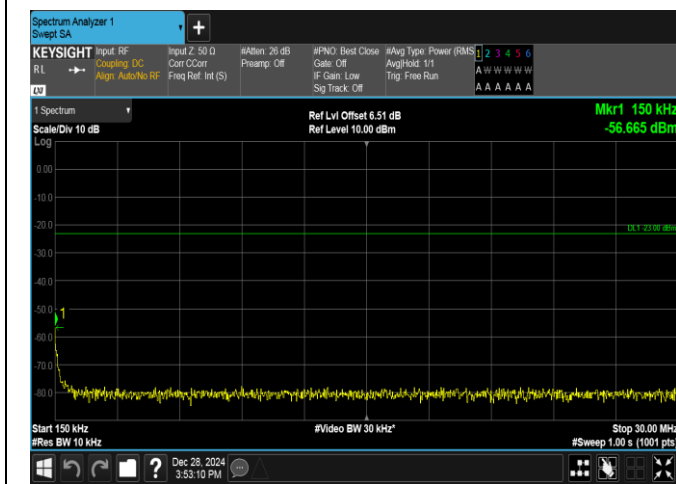
Band5-10MHz-16QAM-20600-1RB#0-0.15~30-PASS
