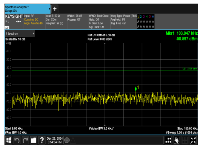
Band5-10MHz-QPSK-20600-1RB#49-0.009~0.15-PASS
