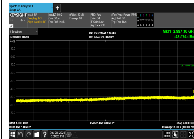
Band5-10MHz-QPSK-20525-50RB#0-1000~3000-PASS
