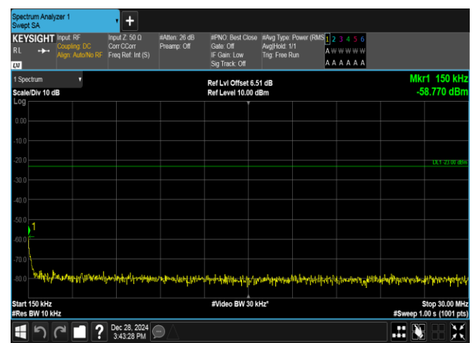
Band5-10MHz-QPSK-20450-50RB#0-0.15~30-PASS
