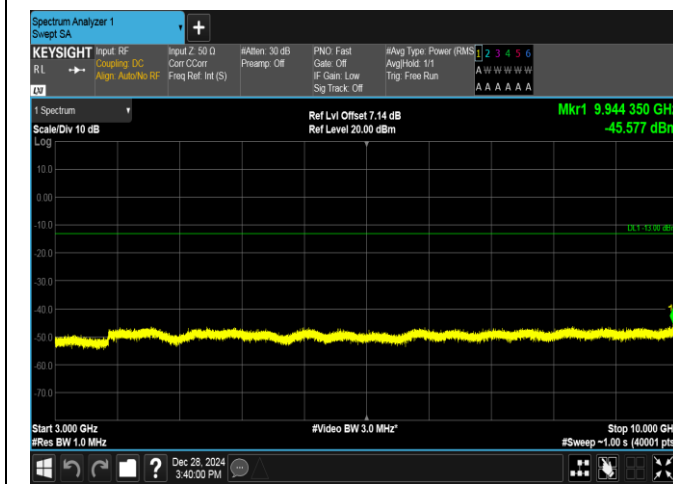
Band5-10MHz-QPSK-20450-1RB#0-3000~10000-PASS
