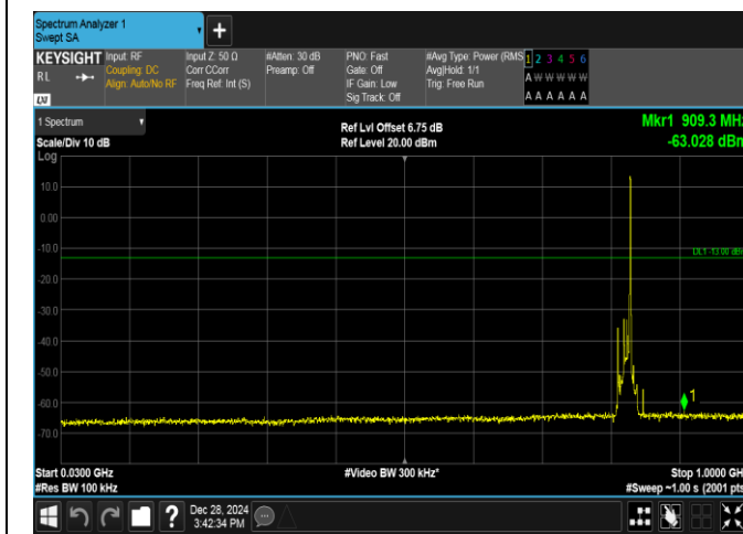
Band5-10MHz-16QAM-20450-1RB#49-30~1000-PASS
