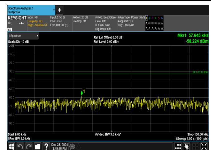
Band5-10MHz-QPSK-20525-50RB#0-0.009~0.15-PASS
