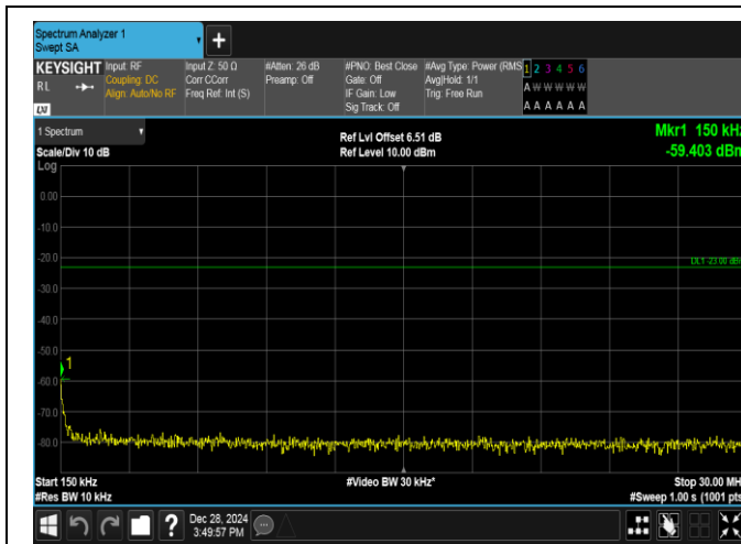
Band5-10MHz-QPSK-20525-50RB#0-0.15~30-PASS
