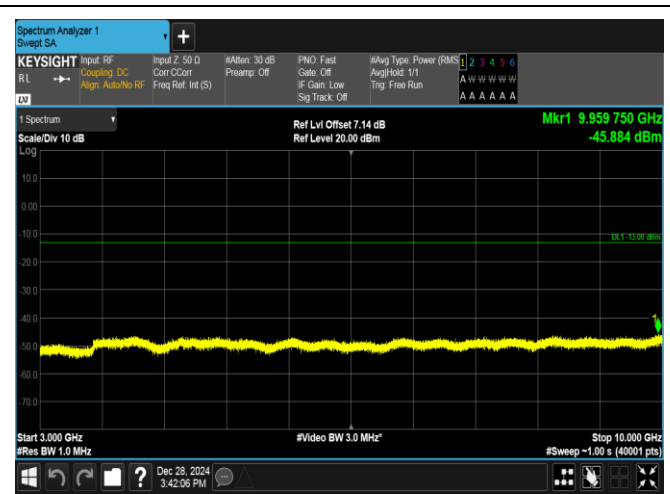
Band5-10MHz-QPSK-20450-1RB#49-3000~10000-PASS
