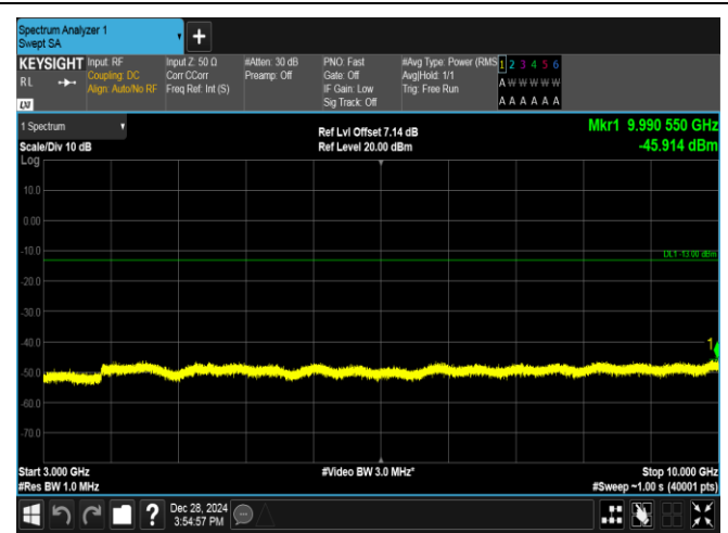
Band5-10MHz-QPSK-20600-1RB#49-3000~10000-PASS
