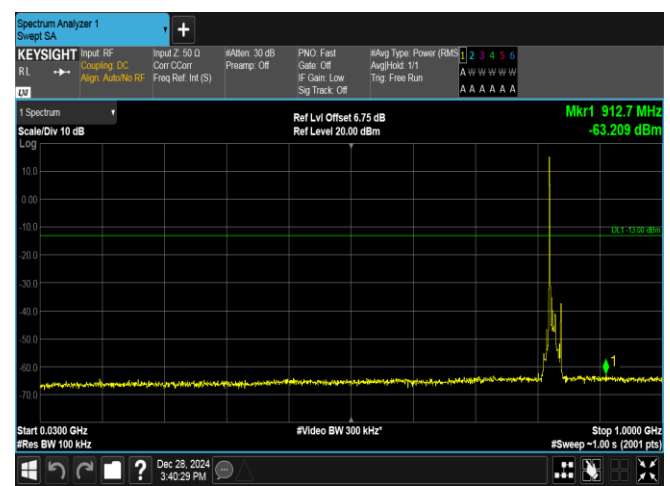
Band5-10MHz-16QAM-20450-1RB#0-30~1000-PASS
