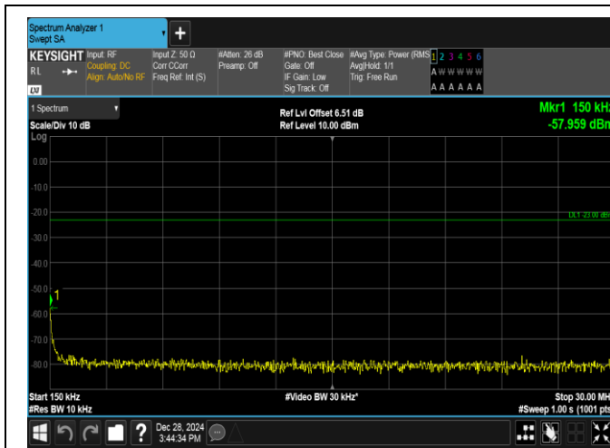
Band5-10MHz-16QAM-20450-50RB#0-0.15~30-PASS
