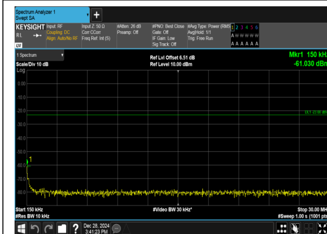
Band5-10MHz-QPSK-20450-1RB#49-0.15~30-PASS
