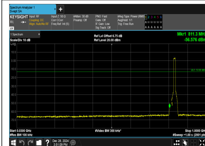
Band5-10MHz-16QAM-20525-50RB#0-30~1000-PASS
