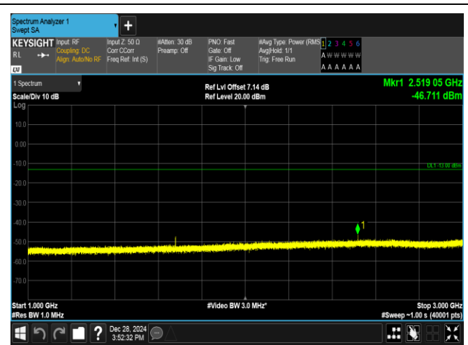
Band5-10MHz-QPSK-20600-1RB#0-1000~3000-PASS
