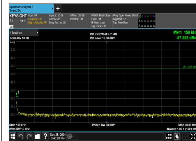
Band5-10MHz-16QAM-20450-1RB#0-0.15~30-PASS
