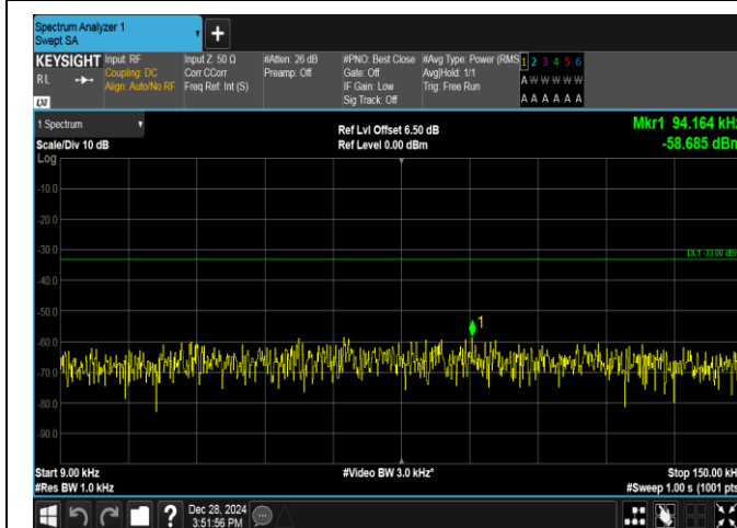
Band5-10MHz-QPSK-20600-1RB#0-0.009~0.15-PASS
