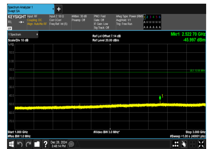
Band5-10MHz-QPSK-20525-1RB#49-1000~3000-PASS
