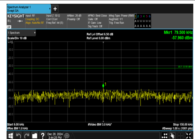
Band5-10MHz-16QAM-20450-50RB#0-0.009~0.15-PASS
