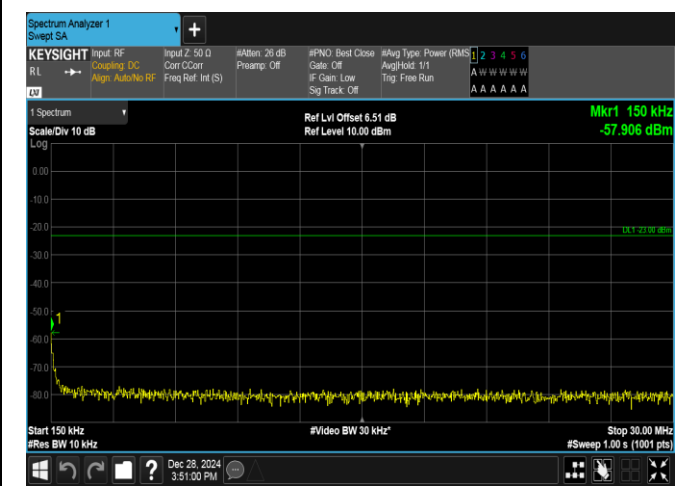
Band5-10MHz-16QAM-20525-50RB#0-0.15~30-PASS
