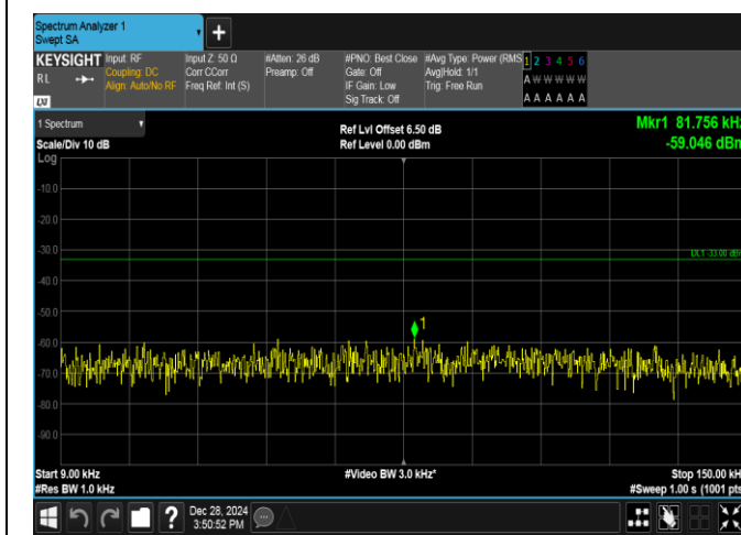
Band5-10MHz-16QAM-20525-50RB#0-0.009~0.15-PASS
