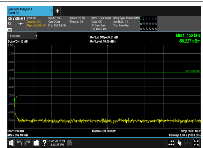
Band5-10MHz-16QAM-20450-1RB#49-0.15~30-PASS
