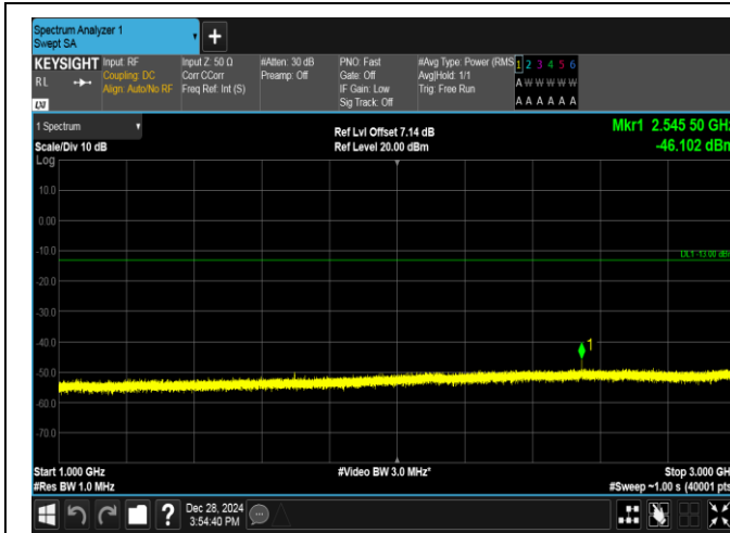
Band5-10MHz-QPSK-20600-1RB#49-1000~3000-PASS
