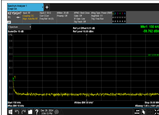
Band5-10MHz-QPSK-20600-1RB#49-0.15~30-PASS
