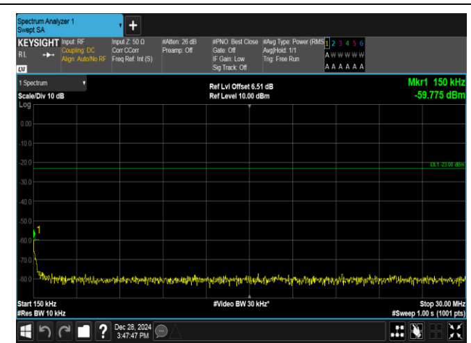
Band5-10MHz-QPSK-20525-1RB#49-0.15~30-PASS
