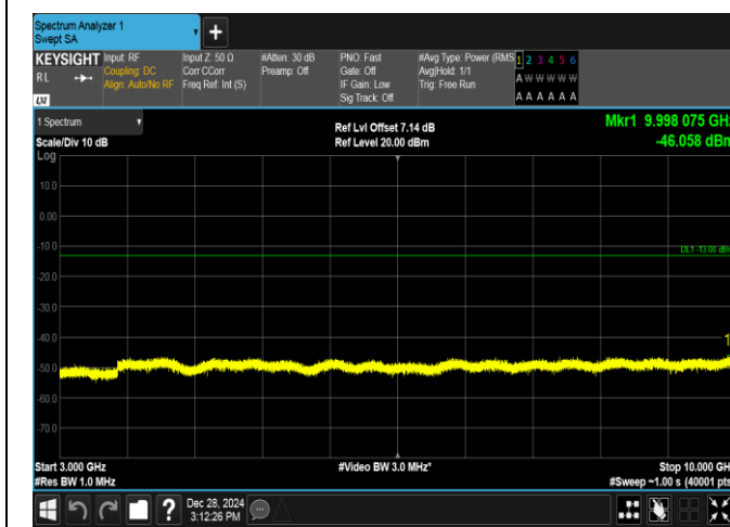
Band5-5MHz-16QAM-20525-1RB#0-3000~10000-PASS
