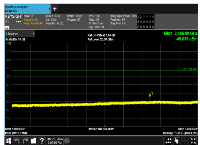
Band5-5MHz-16QAM-20425-1RB#24-1000~3000-PASS
