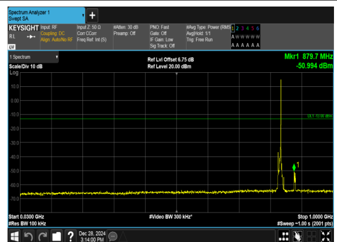
Band5-5MHz-16QAM-20525-1RB#24-30~1000-PASS
