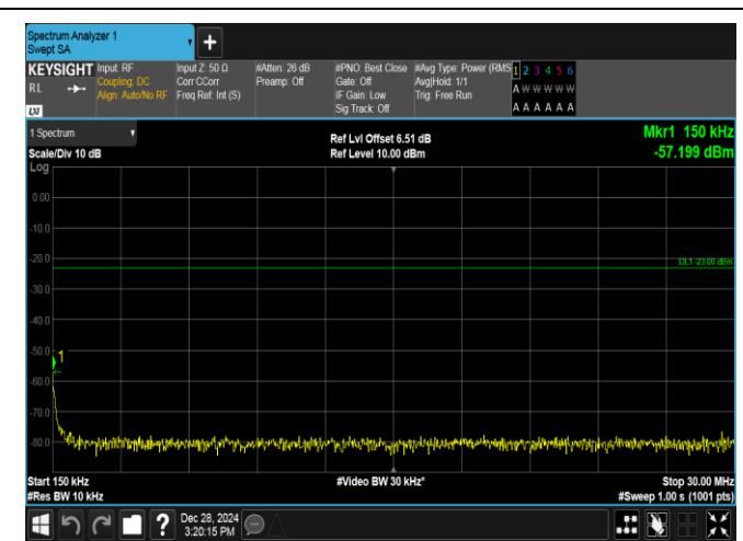
Band5-5MHz-16QAM-20625-1RB#24-0.15~30-PASS
