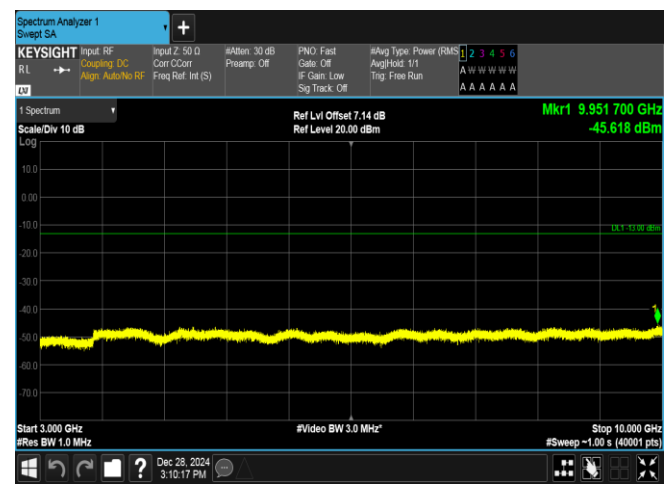
Band5-5MHz-16QAM-20425-25RB#0-3000~10000-PASS
