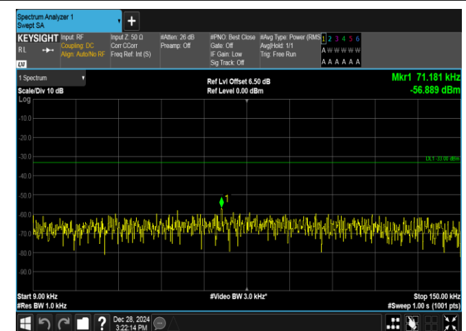
Band5-5MHz-16QAM-20625-25RB#0-0.009~0.15-PASS
