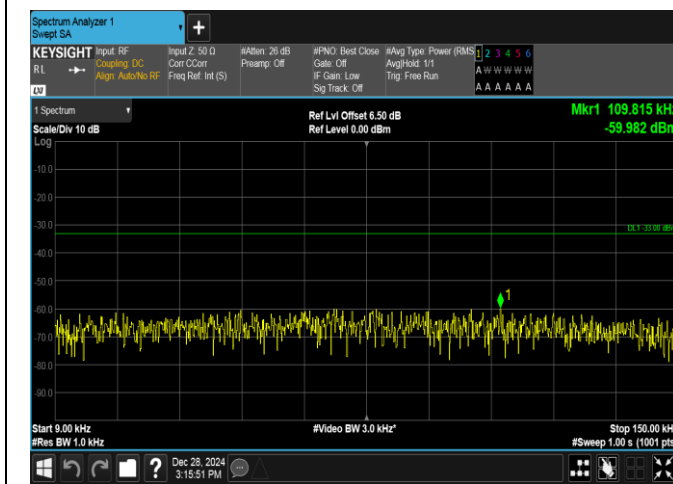
Band5-5MHz-16QAM-20525-25RB#0-0.009~0.15-PASS
