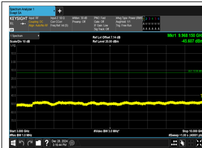
Band5-5MHz-16QAM-20525-25RB#0-3000~10000-PASS
