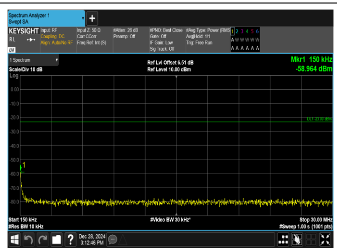
Band5-5MHz-QPSK-20525-1RB#24-0.15~30-PASS
