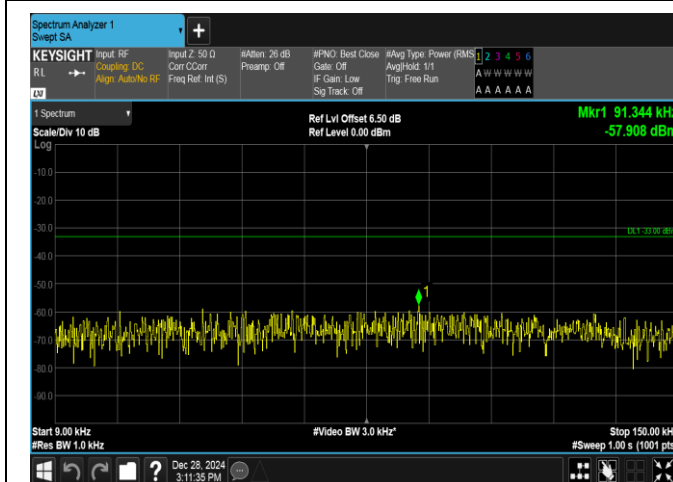
Band5-5MHz-16QAM-20525-1RB#0-0.009~0.15-PASS
