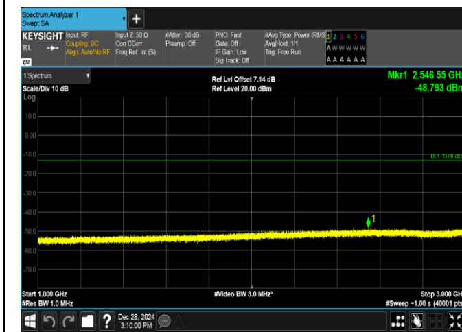
Band5-5MHz-16QAM-20425-25RB#0-1000~3000-PASS
