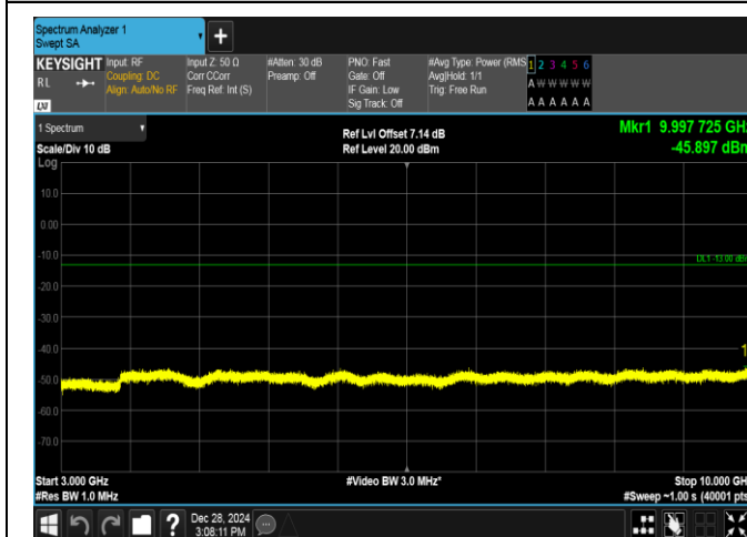
Band5-5MHz-16QAM-20425-1RB#24-3000~10000-PASS
