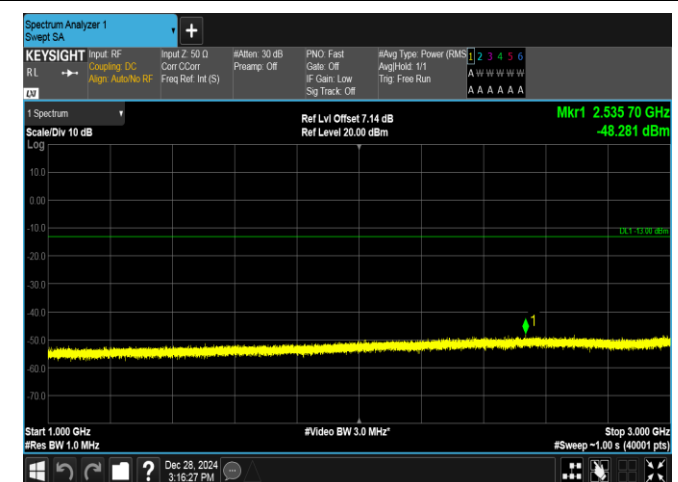
Band5-5MHz-16QAM-20525-25RB#0-1000~3000-PASS
