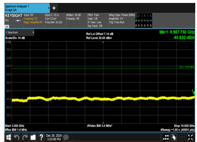
Band5-5MHz-16QAM-20625-25RB#0-3000~10000-PASS
