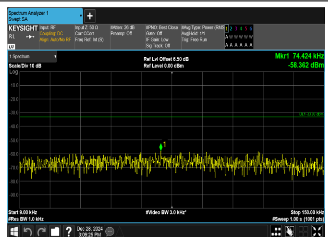
Band5-5MHz-16QAM-20425-25RB#0-0.009~0.15-PASS
