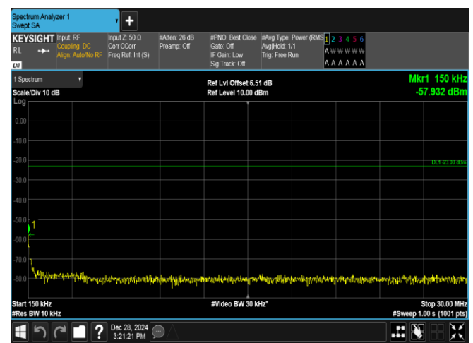
Band5-5MHz-QPSK-20625-25RB#0-0.15~30-PASS
