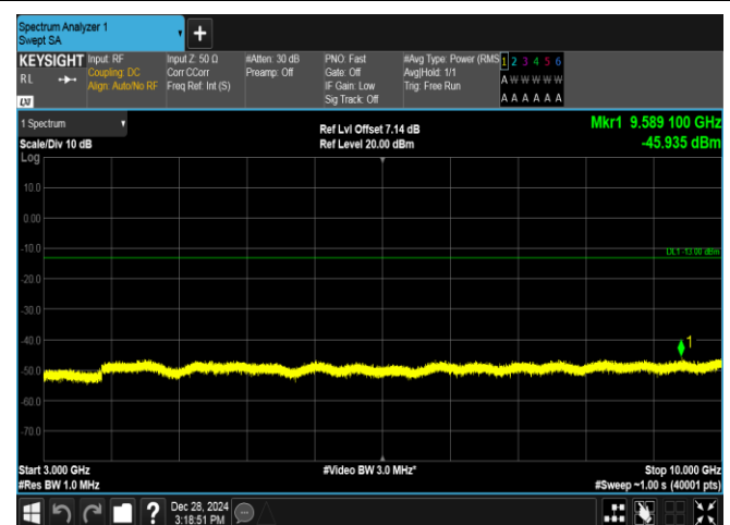
Band5-5MHz-16QAM-20625-1RB#0-3000~10000-PASS
