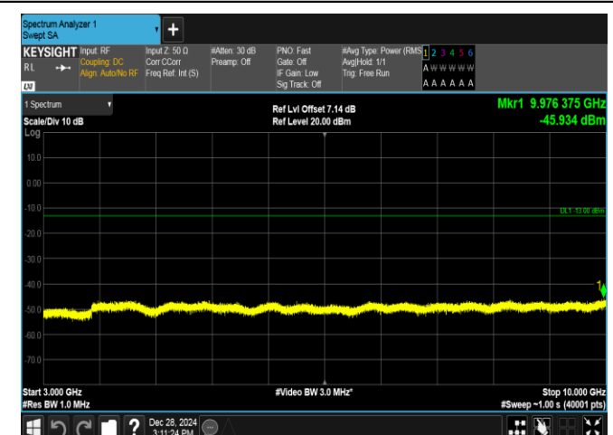
Band5-5MHz-QPSK-20525-1RB#0-3000~10000-PASS
