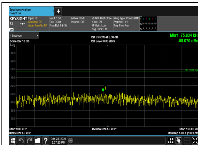
Band5-5MHz-16QAM-20425-1RB#24-0.009~0.15-PASS
