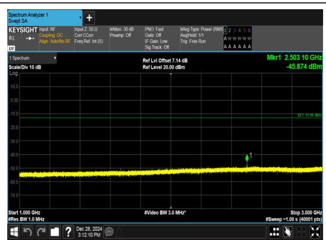
Band5-5MHz-16QAM-20525-1RB#0-1000~3000-PASS
