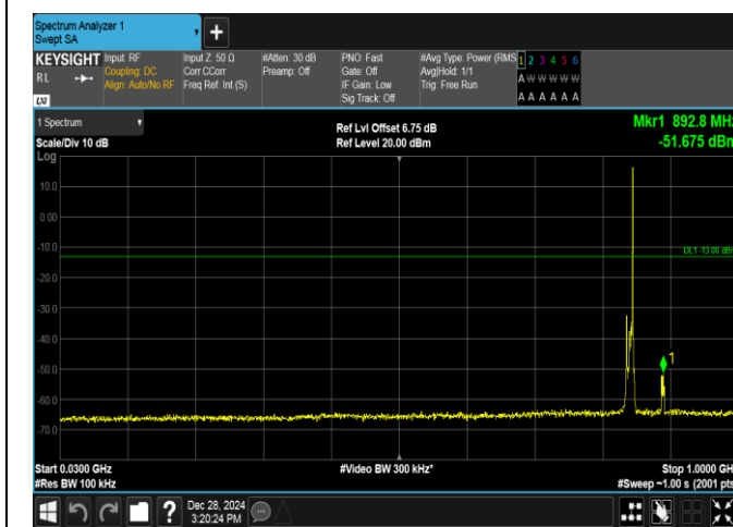
Band5-5MHz-16QAM-20625-1RB#24-30~1000-PASS
