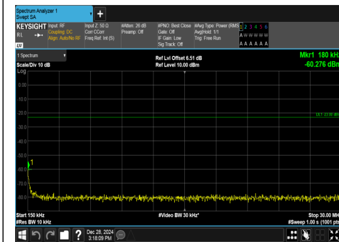
Band5-5MHz-16QAM-20625-1RB#0-0.15~30-PASS
