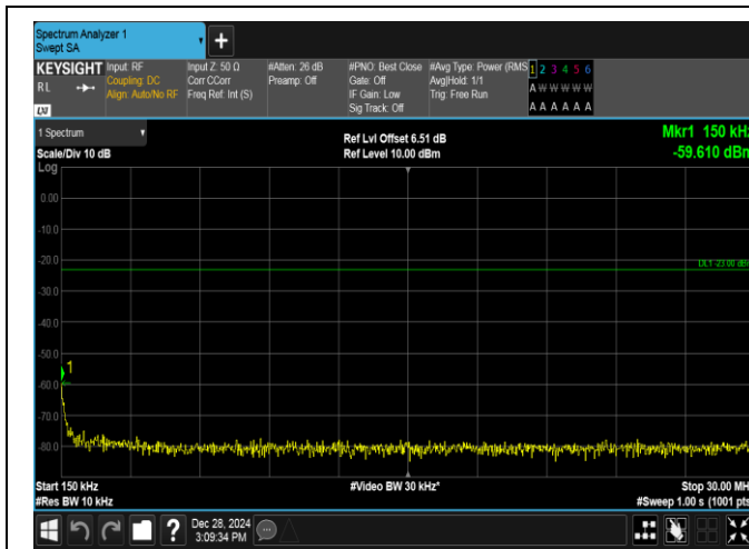
Band5-5MHz-16QAM-20425-25RB#0-0.15~30-PASS
