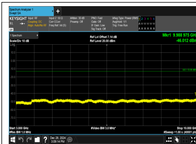
Band5-5MHz-QPSK-20425-25RB#0-3000~10000-PASS
