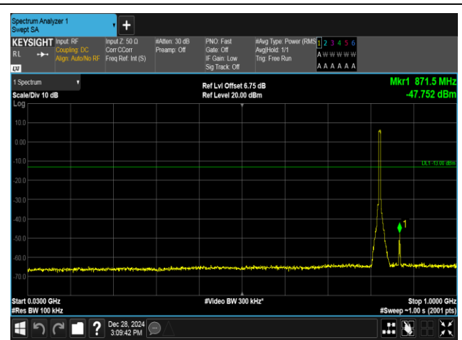
Band5-5MHz-16QAM-20425-25RB#0-30~1000-PASS
