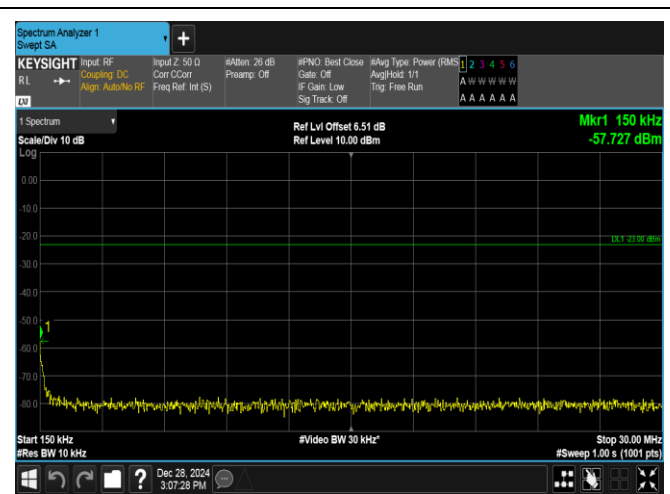
Band5-5MHz-16QAM-20425-1RB#24-0.15~30-PASS
