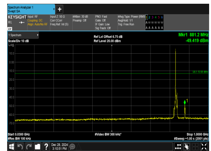
Band5-5MHz-QPSK-20525-1RB#0-30~1000-PASS
