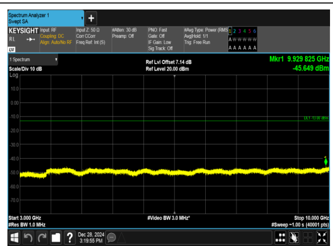
Band5-5MHz-QPSK-20625-1RB#24-3000~10000-PASS
