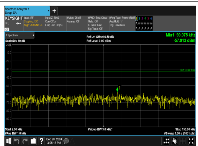
Band5-5MHz-16QAM-20425-1RB#0-0.009~0.15-PASS
