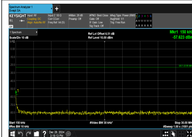
Band5-5MHz-QPSK-20625-1RB#24-0.15~30-PASS
