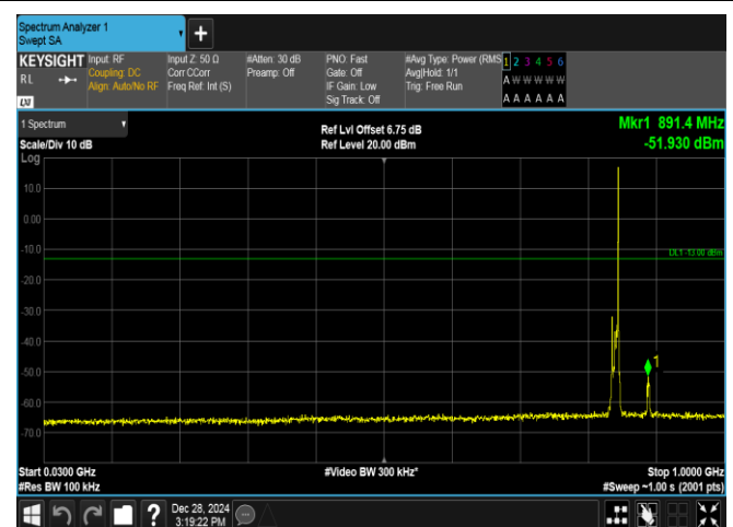
Band5-5MHz-QPSK-20625-1RB#24-30~1000-PASS
