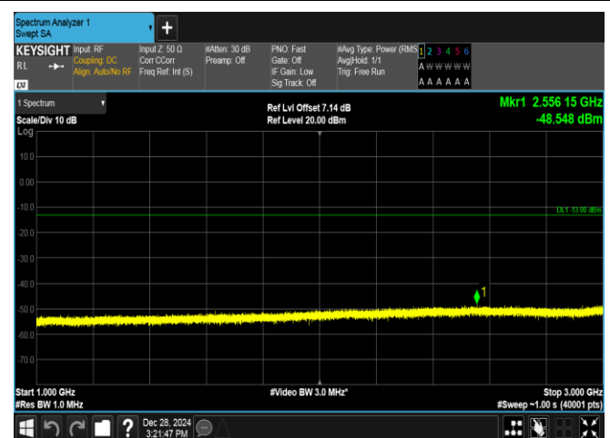
Band5-5MHz-QPSK-20625-25RB#0-1000~3000-PASS
