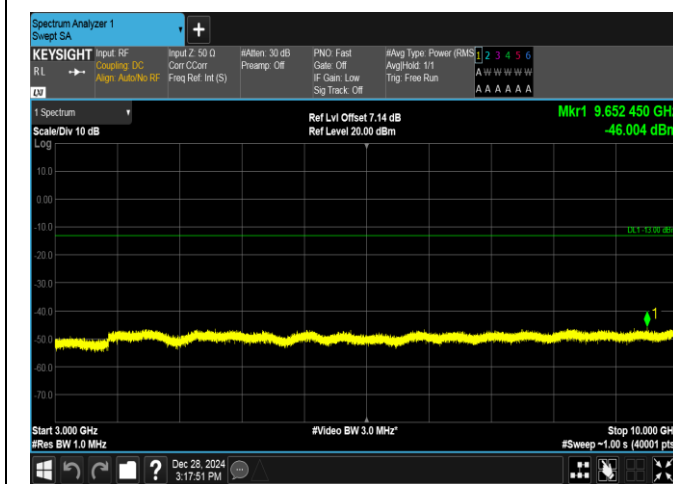
Band5-5MHz-QPSK-20625-1RB#0-3000~10000-PASS
