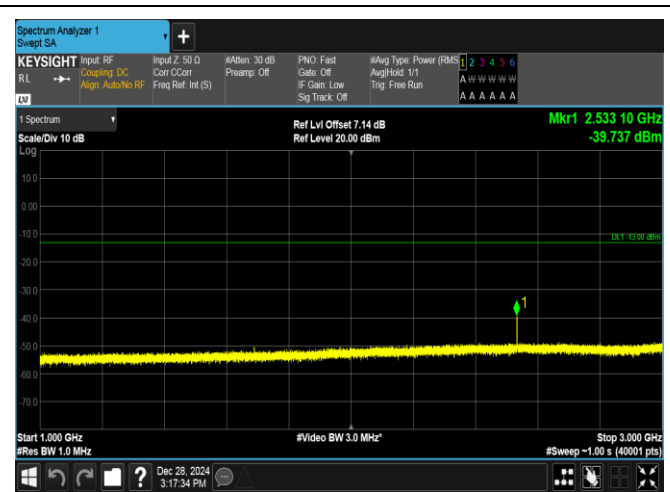
Band5-5MHz-QPSK-20625-1RB#0-1000~3000-PASS
