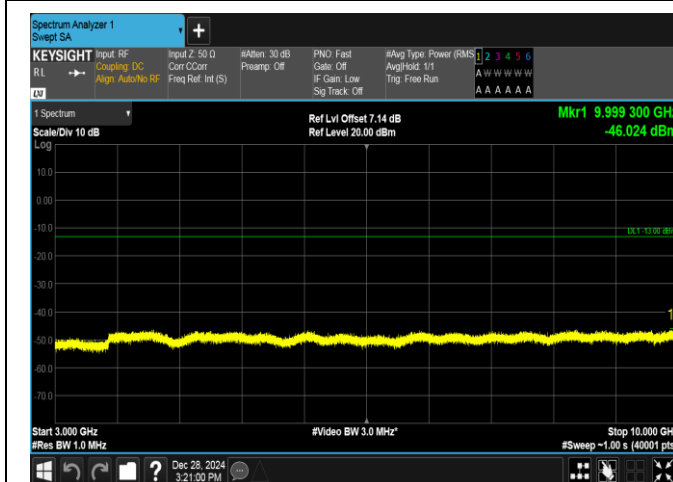
Band5-5MHz-16QAM-20625-1RB#24-3000~10000-PASS
