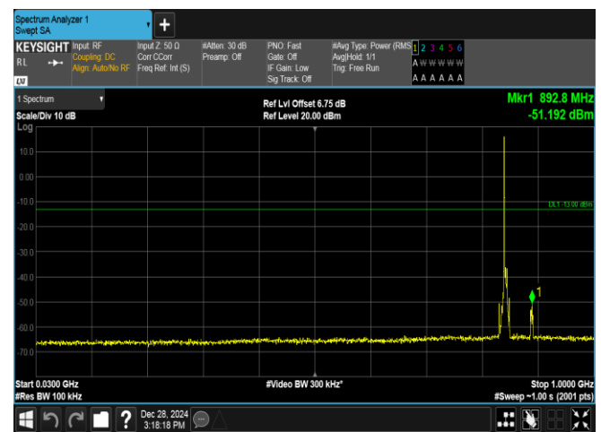
Band5-5MHz-16QAM-20625-1RB#0-30~1000-PASS
