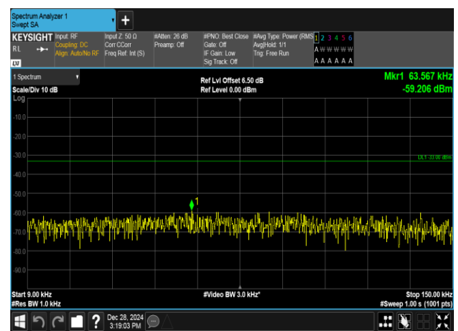
Band5-5MHz-QPSK-20625-1RB#24-0.009~0.15-PASS
