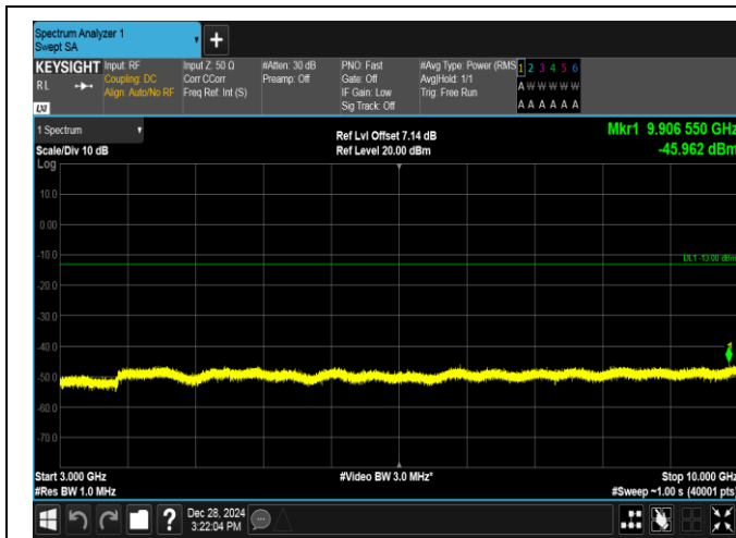
Band5-5MHz-QPSK-20625-25RB#0-3000~10000-PASS
