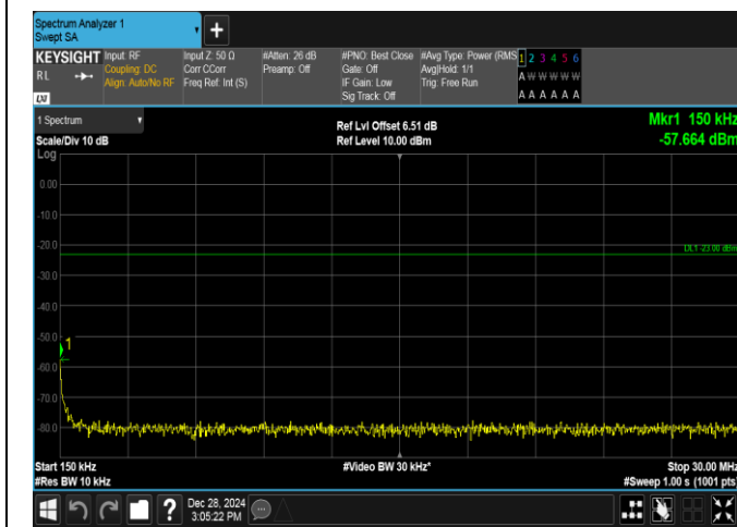
Band5-5MHz-16QAM-20425-1RB#0-0.15~30-PASS
