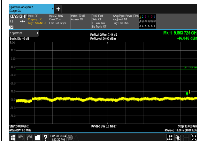
Band5-5MHz-QPSK-20525-1RB#24-3000~10000-PASS
