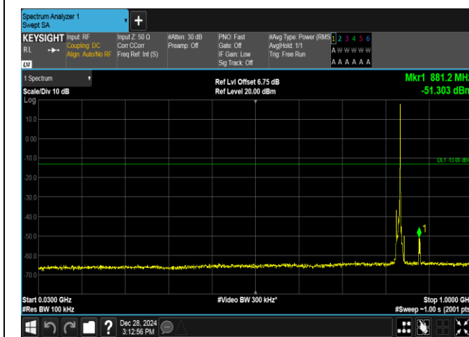
Band5-5MHz-QPSK-20525-1RB#24-30~1000-PASS
