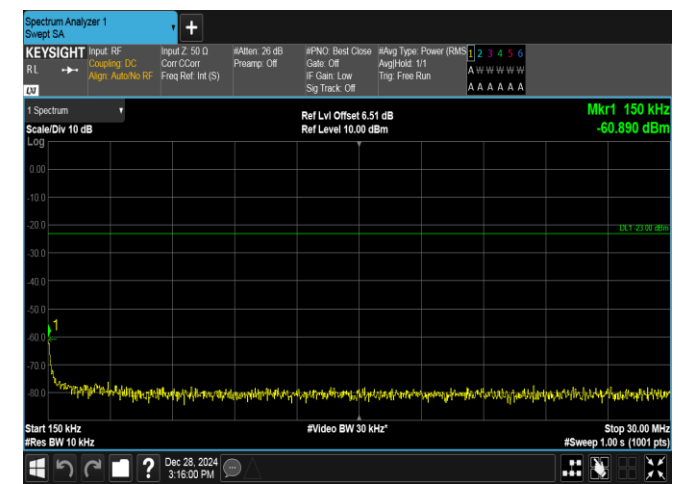
Band5-5MHz-16QAM-20525-25RB#0-0.15~30-PASS
