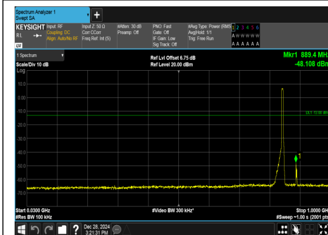
Band5-5MHz-QPSK-20625-25RB#0-30~1000-PASS
