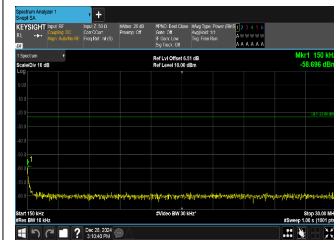
Band5-5MHz-QPSK-20525-1RB#0-0.15~30-PASS
