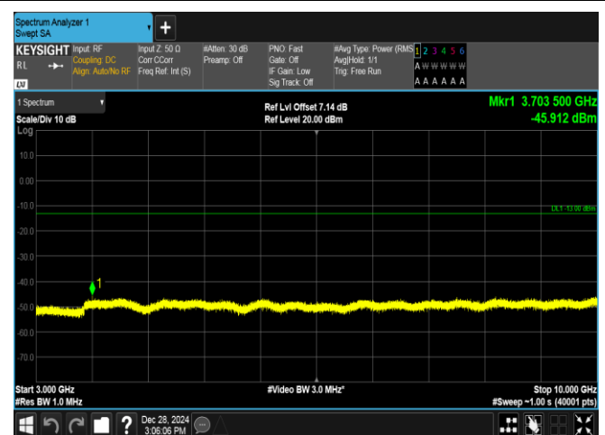
Band5-5MHz-16QAM-20425-1RB#0-3000~10000-PASS
