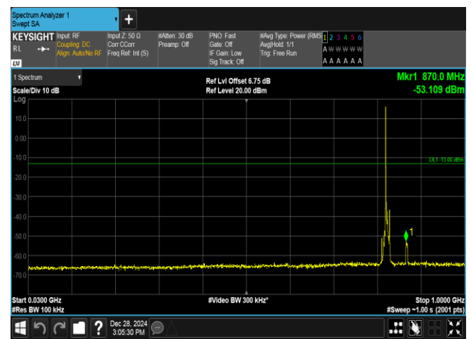
Band5-5MHz-16QAM-20425-1RB#0-30~1000-PASS
