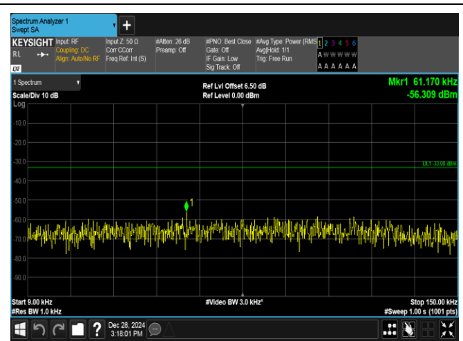
Band5-5MHz-16QAM-20625-1RB#0-0.009~0.15-PASS
