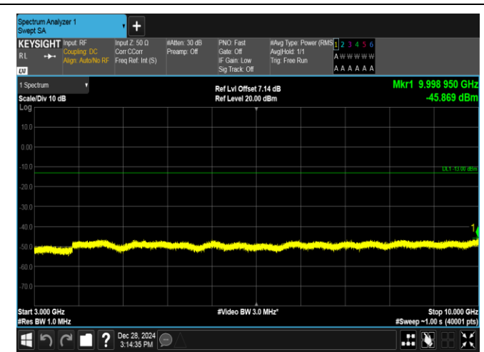
Band5-5MHz-16QAM-20525-1RB#24-3000~10000-PASS
