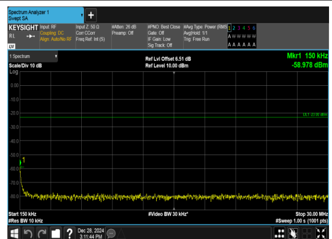
Band5-5MHz-16QAM-20525-1RB#0-0.15~30-PASS
