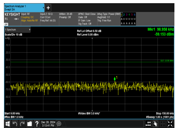
Band5-5MHz-16QAM-20525-1RB#24-0.009~0.15-PASS
