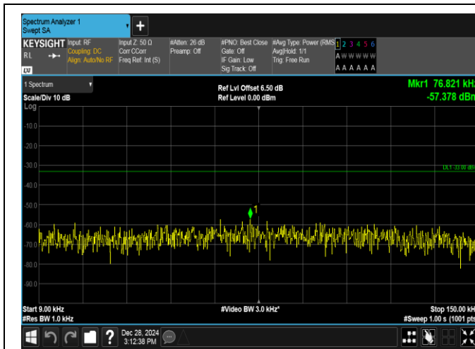
Band5-5MHz-QPSK-20525-1RB#24-0.009~0.15-PASS
