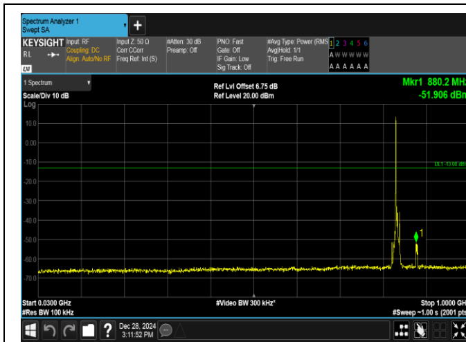
Band5-5MHz-16QAM-20525-1RB#0-30~1000-PASS
