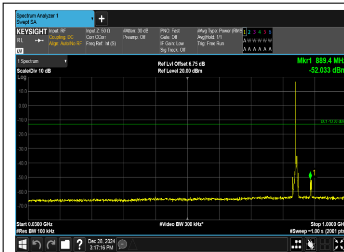
Band5-5MHz-QPSK-20625-1RB#0-30~1000-PASS
