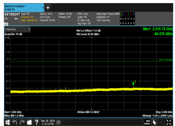
Band5-5MHz-QPSK-20525-1RB#24-1000~3000-PASS
