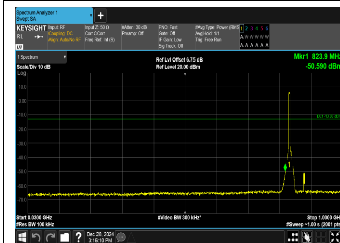
Band5-5MHz-16QAM-20525-25RB#0-30~1000-PASS
