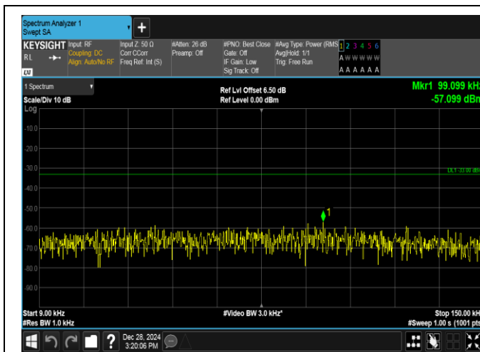
Band5-5MHz-16QAM-20625-1RB#24-0.009~0.15-PASS
