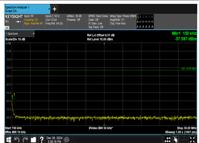
Band5-10MHz-QPSK-20450-1RB#0-0.15~30-PASS
