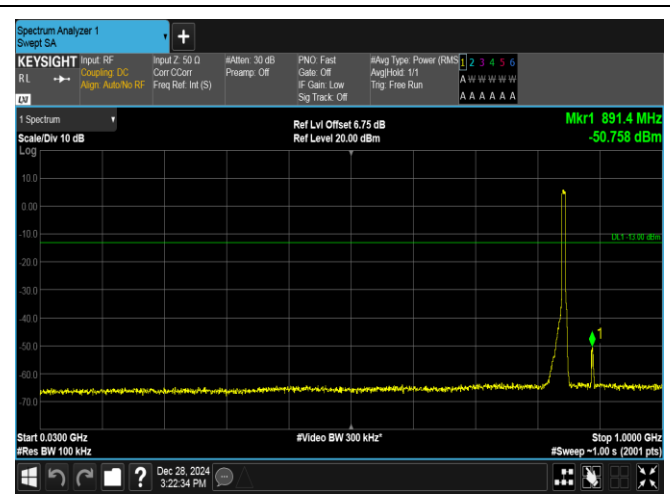
Band5-5MHz-16QAM-20625-25RB#0-30~1000-PASS
