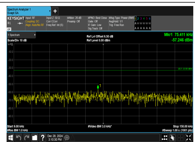
Band5-5MHz-QPSK-20525-1RB#0-0.009~0.15-PASS
