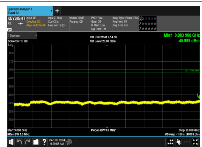
Band5-3MHz-16QAM-20525-1RB#14-3000~10000-PASS
