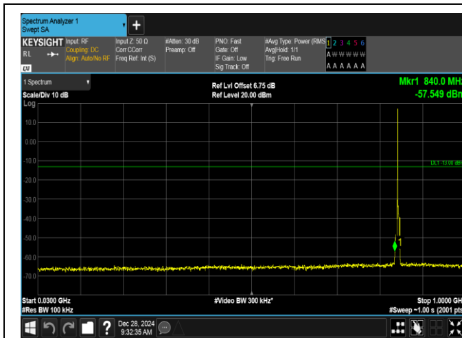
Band5-3MHz-QPSK-20635-1RB#0-30~1000-PASS
