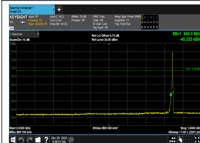
Band5-3MHz-QPSK-20635-15RB#0-30~1000-PASS
