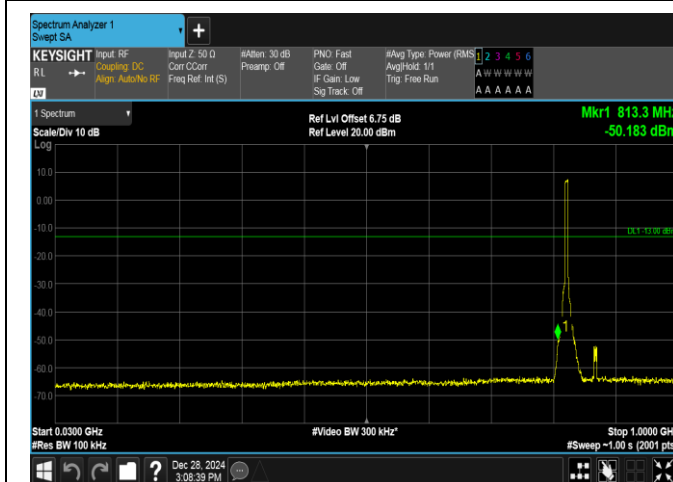
Band5-5MHz-QPSK-20425-25RB#0-30~1000-PASS
