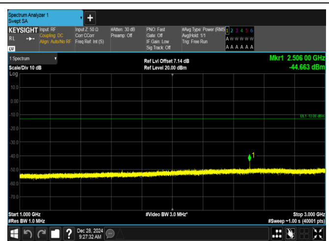
Band5-3MHz-16QAM-20525-1RB#0-1000~3000-PASS
