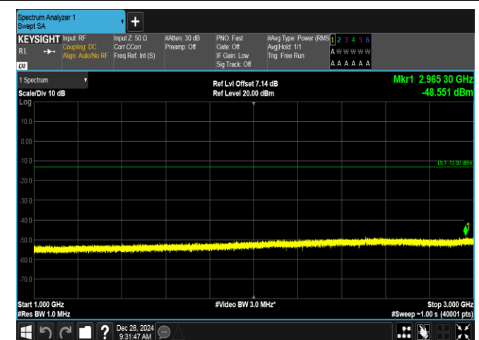
Band5-3MHz-16QAM-20525-15RB#0-1000~3000-PASS
