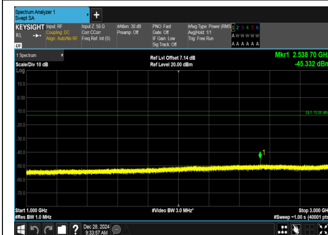
Band5-3MHz-16QAM-20635-1RB#0-1000~3000-PASS
