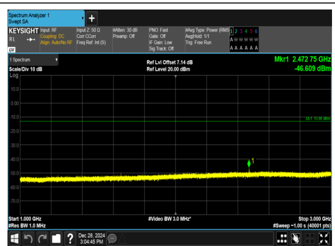
Band5-5MHz-QPSK-20425-1RB#0-1000~3000-PASS
