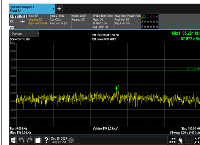
Band5-5MHz-QPSK-20425-25RB#0-0.009~0.15-PASS
