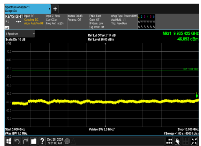
Band5-3MHz-QPSK-20525-15RB#0-3000~10000-PASS
