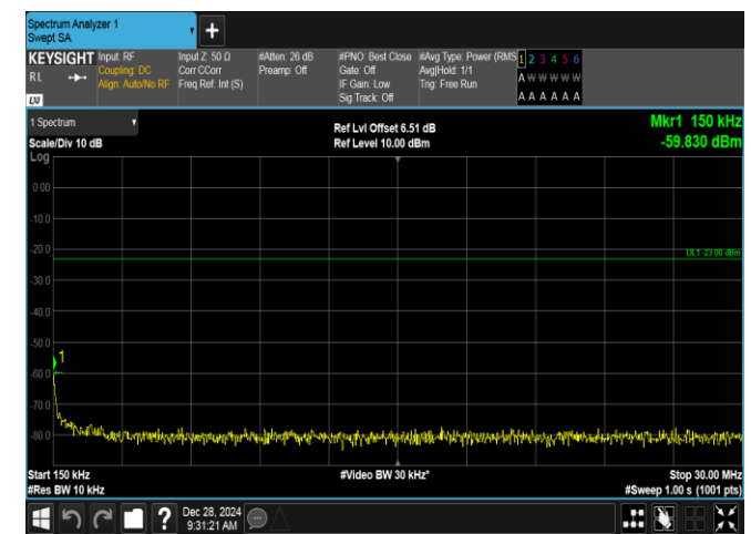
Band5-3MHz-16QAM-20525-15RB#0-0.15~30-PASS
