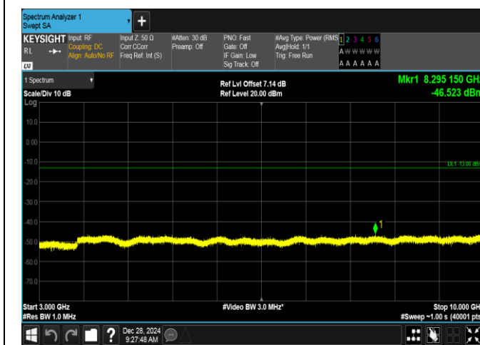
Band5-3MHz-16QAM-20525-1RB#0-3000~10000-PASS
