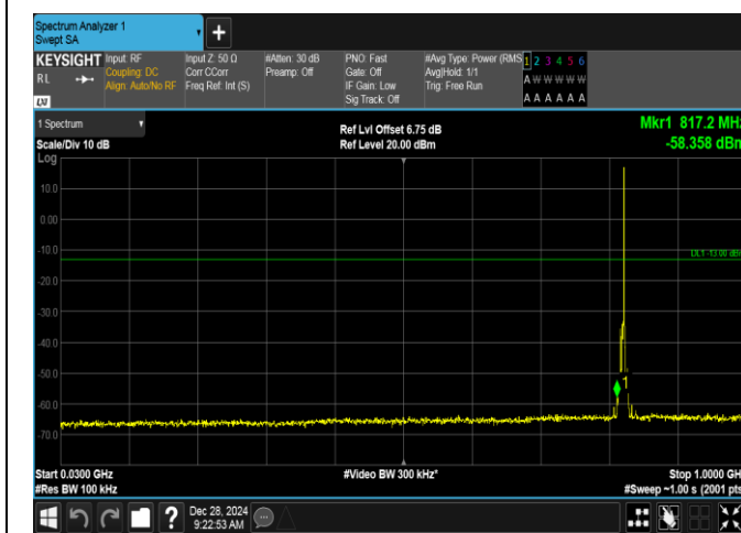
Band5-3MHz-16QAM-20415-1RB#14-30~1000-PASS
