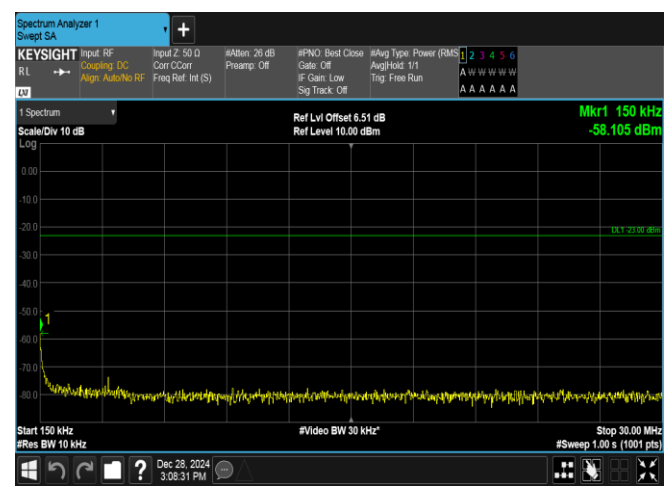
Band5-5MHz-QPSK-20425-25RB#0-0.15~30-PASS
