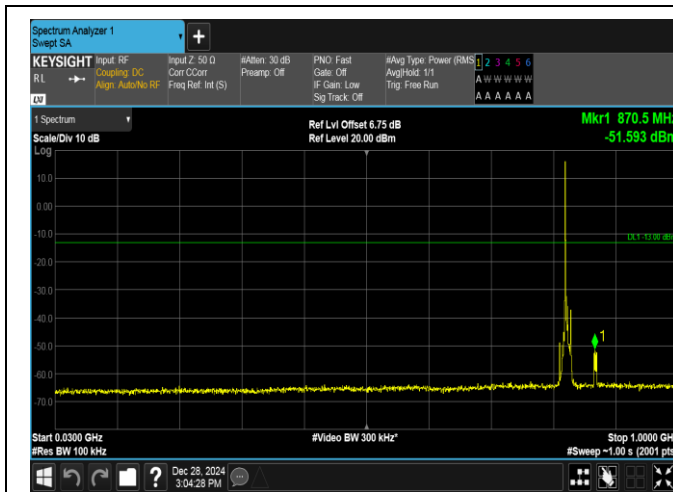
Band5-5MHz-QPSK-20425-1RB#0-30~1000-PASS
