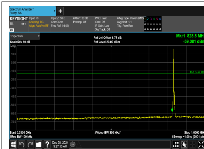
Band5-3MHz-16QAM-20525-1RB#0-30~1000-PASS
