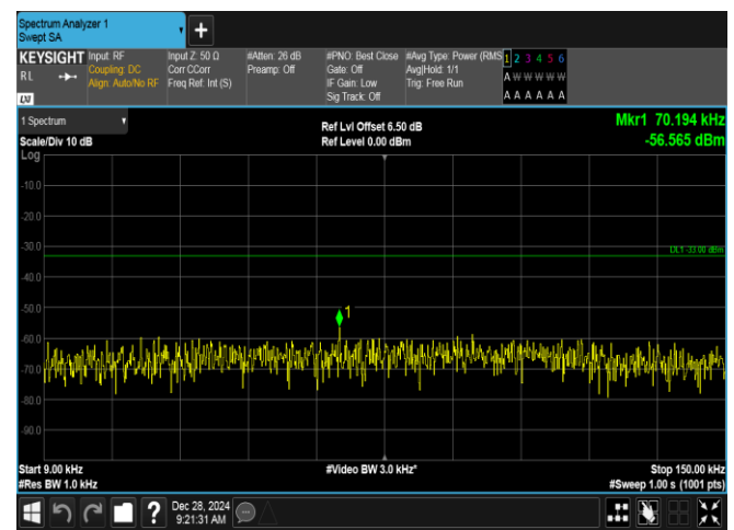
Band5-3MHz-QPSK-20415-1RB#14-0.009~0.15-PASS
