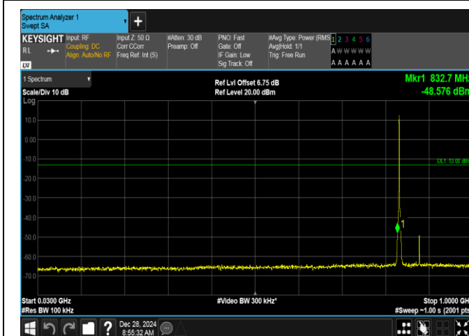
Band5-1.4MHz-16QAM-20525-6RB#0-30~1000-PASS
