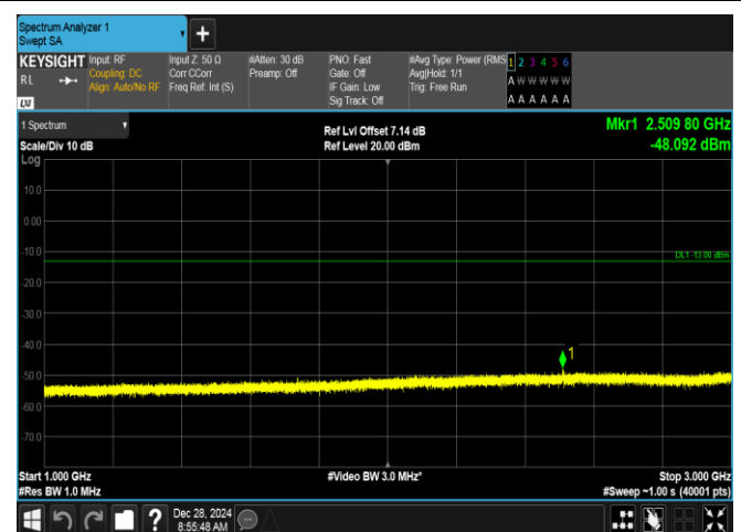
Band5-1.4MHz-16QAM-20525-6RB#0-1000~3000-PASS
