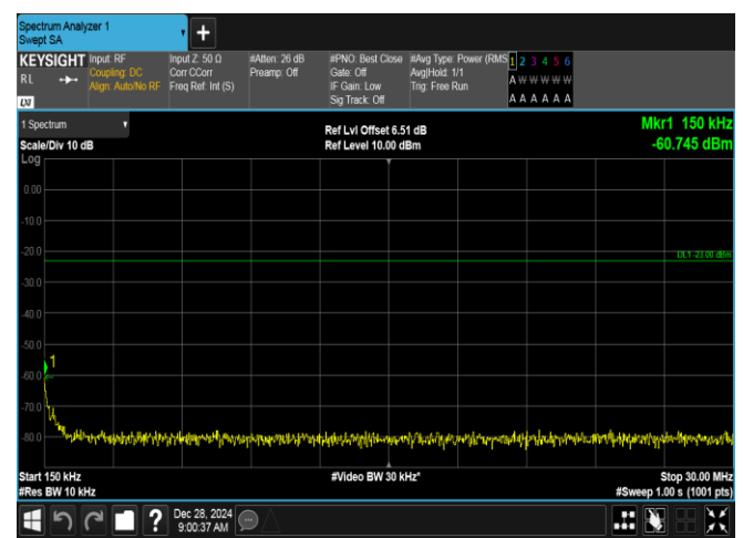
Band5-1.4MHz-QPSK-20643-6RB#0-0.15~30-PASS
