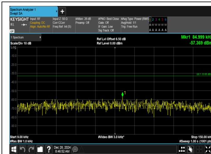
Band5-1.4MHz-16QAM-20407-1RB#5-0.009~0.15-PASS
