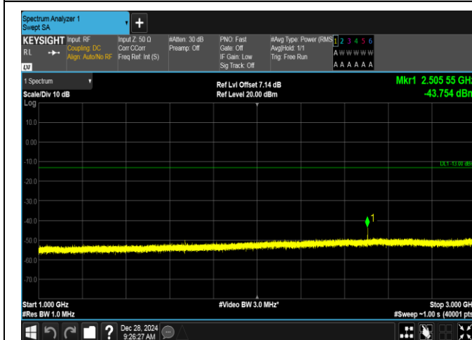
Band5-3MHz-QPSK-20525-1RB#0-1000~3000-PASS
