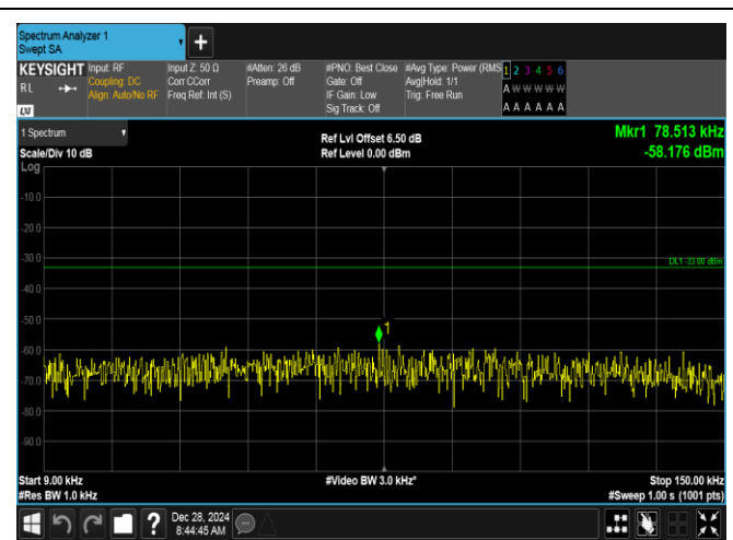
Band5-1.4MHz-16QAM-20407-1RB#0-0.009~0.15-PASS
