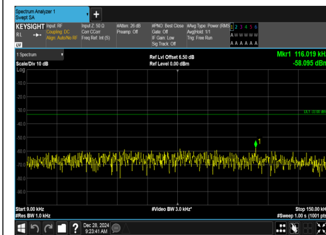
Band5-3MHz-QPSK-20415-15RB#0-0.009~0.15-PASS
