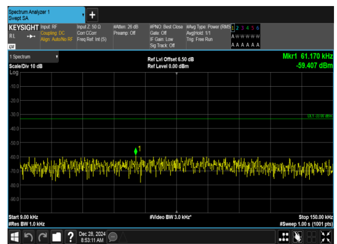
Band5-1.4MHz-16QAM-20525-1RB#5-0.009~0.15-PASS
