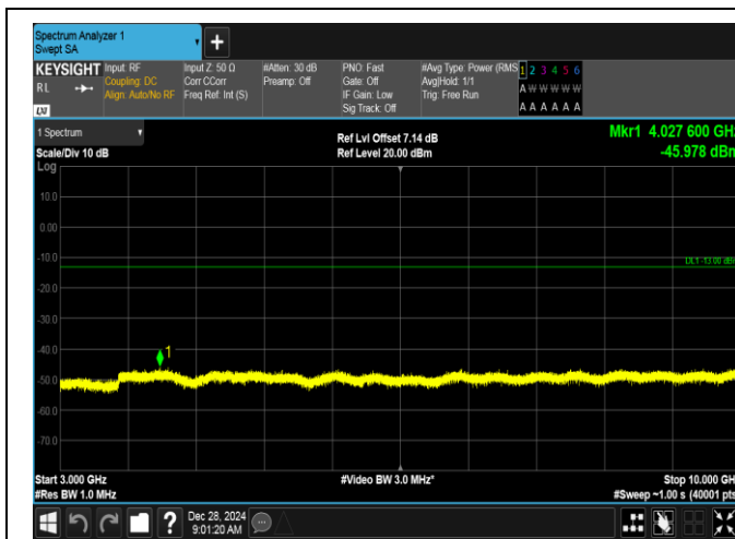
Band5-1.4MHz-QPSK-20643-6RB#0-3000~10000-PASS
