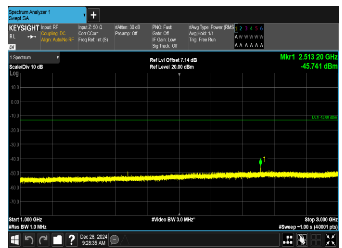
Band5-3MHz-QPSK-20525-1RB#14-1000~3000-PASS
