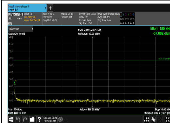
Band5-3MHz-QPSK-20525-1RB#0-0.15~30-PASS
