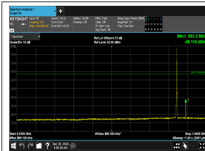
Band5-1.4MHz-QPSK-20643-1RB#0-30~1000-PASS
