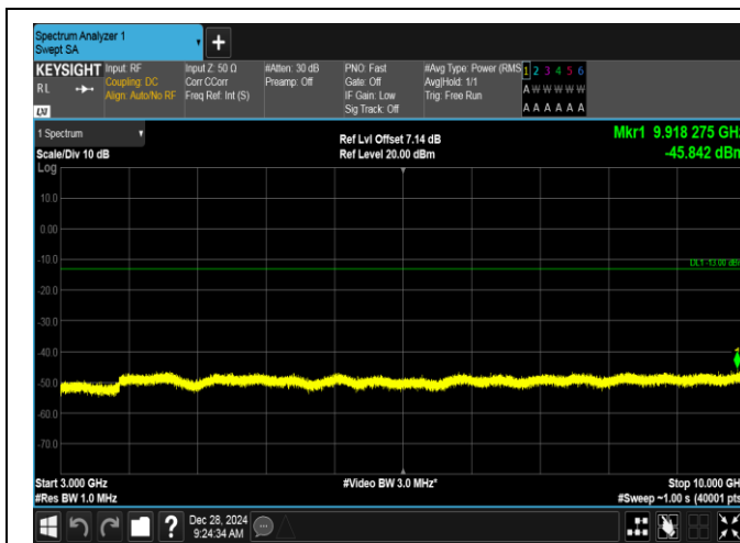
Band5-3MHz-QPSK-20415-15RB#0-3000~10000-PASS
