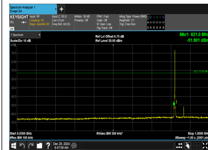
Band5-1.4MHz-16QAM-20407-1RB#5-30~1000-PASS
