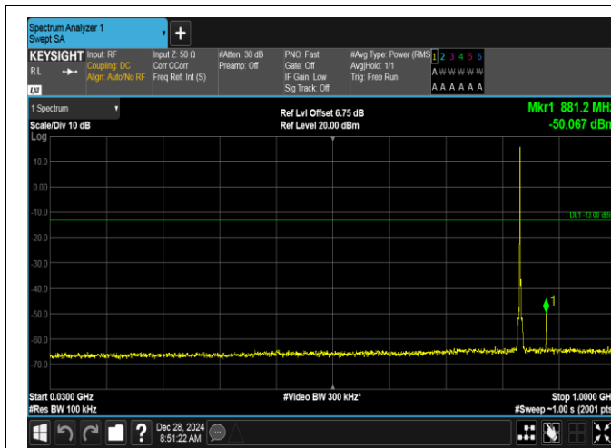
Band5-1.4MHz-16QAM-20525-1RB#0-30~1000-PASS
