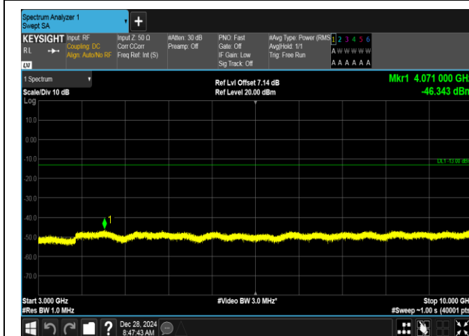
Band5-1.4MHz-16QAM-20407-1RB#5-3000~10000-PASS
