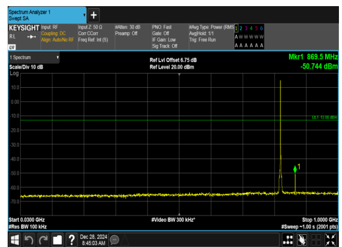
Band5-1.4MHz-16QAM-20407-1RB#0-30~1000-PASS
