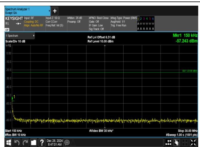
Band5-1.4MHz-16QAM-20407-1RB#5-0.15~30-PASS
