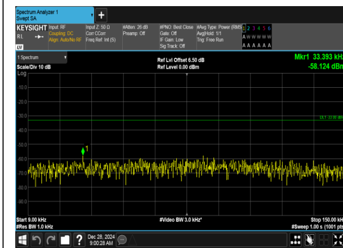
Band5-1.4MHz-QPSK-20643-6RB#0-0.009~0.15-PASS
