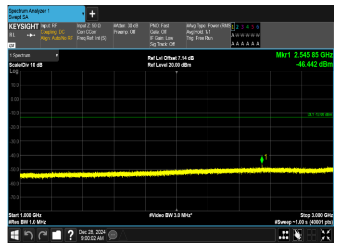
Band5-1.4MHz-16QAM-20643-1RB#5-1000~3000-PASS
