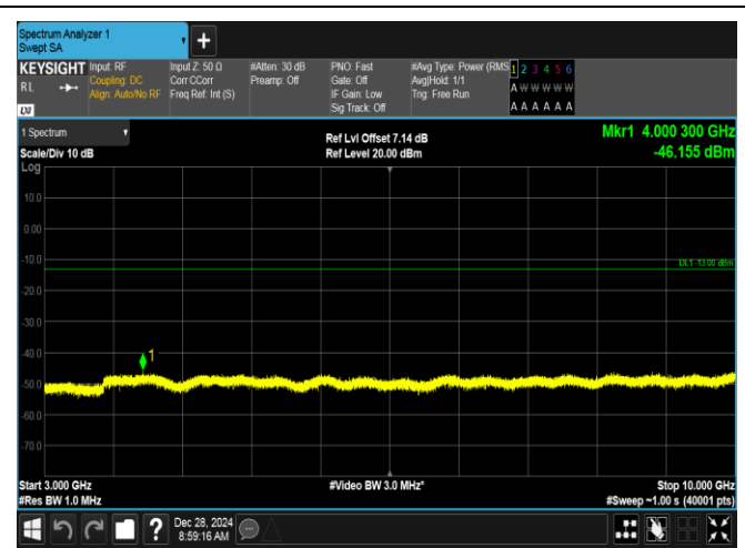
Band5-1.4MHz-QPSK-20643-1RB#5-3000~10000-PASS
