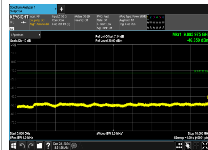
Band5-1.4MHz-16QAM-20525-1RB#0-3000~10000-PASS
