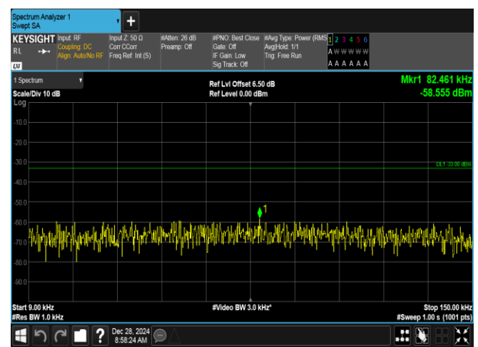
Band5-1.4MHz-QPSK-20643-1RB#5-0.009~0.15-PASS
