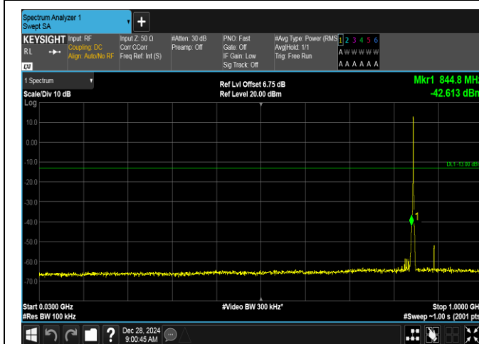
Band5-1.4MHz-QPSK-20643-6RB#0-30~1000-PASS
