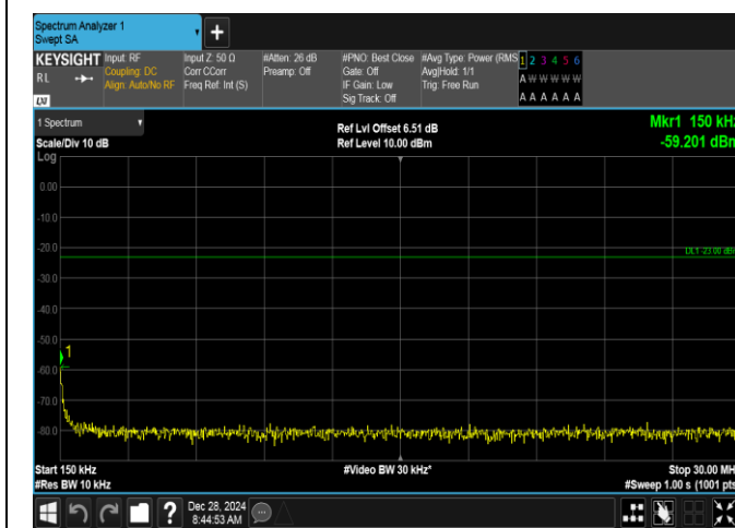
Band5-1.4MHz-16QAM-20407-1RB#0-0.15~30-PASS
