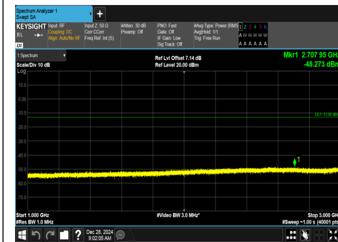
Band5-1.4MHz-16QAM-20643-6RB#0-1000~3000-PASS
