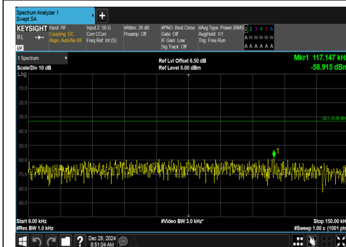
Band5-1.4MHz-16QAM-20525-1RB#0-0.009~0.15-PASS
