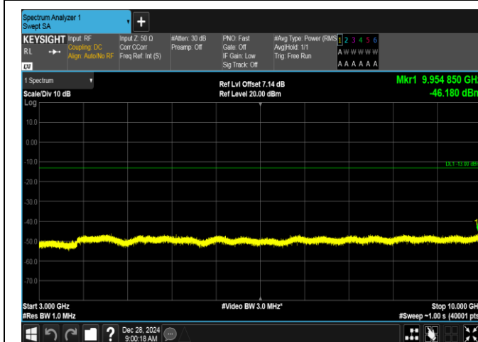
Band5-1.4MHz-16QAM-20643-1RB#5-3000~10000-PASS
