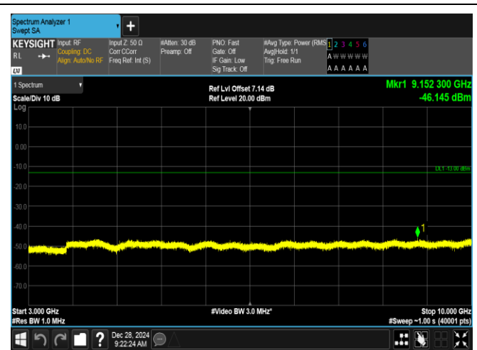
Band5-3MHz-QPSK-20415-1RB#14-3000~10000-PASS
