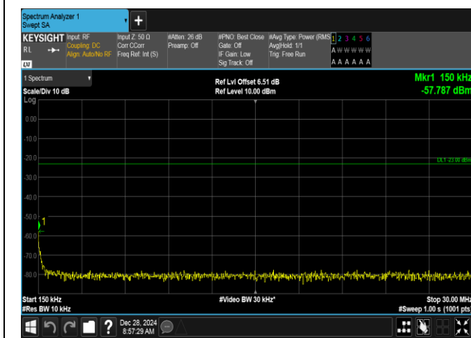
Band5-1.4MHz-16QAM-20643-1RB#0-0.15~30-PASS
