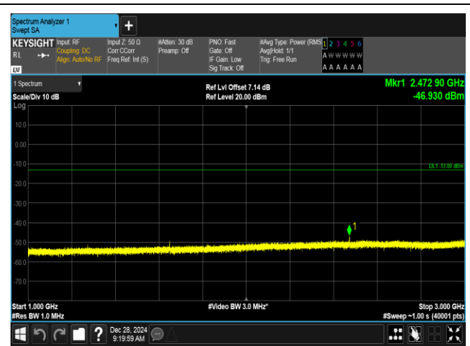
Band5-3MHz-QPSK-20415-1RB#0-1000~3000-PASS
