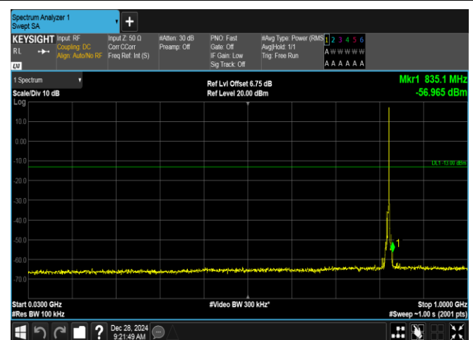
Band5-3MHz-QPSK-20415-1RB#14-30~1000-PASS
