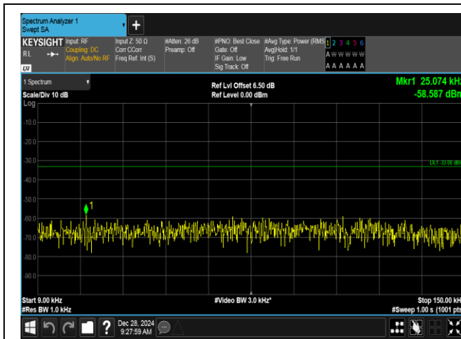
Band5-3MHz-QPSK-20525-1RB#14-0.009~0.15-PASS
