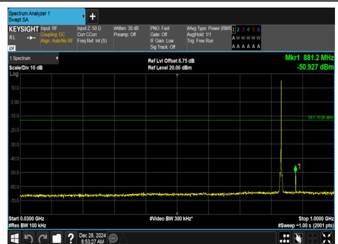
Band5-1.4MHz-16QAM-20525-1RB#5-30~1000-PASS
