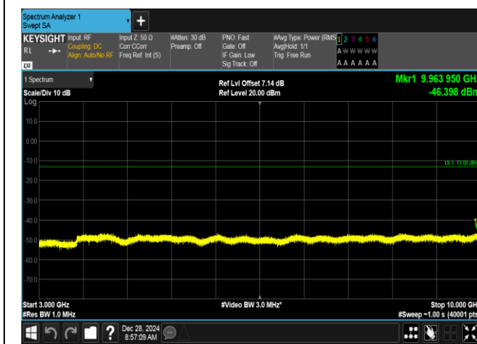
Band5-1.4MHz-QPSK-20643-1RB#0-3000~10000-PASS
