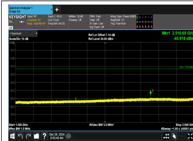
Band5-1.4MHz-16QAM-20525-1RB#5-1000~3000-PASS
