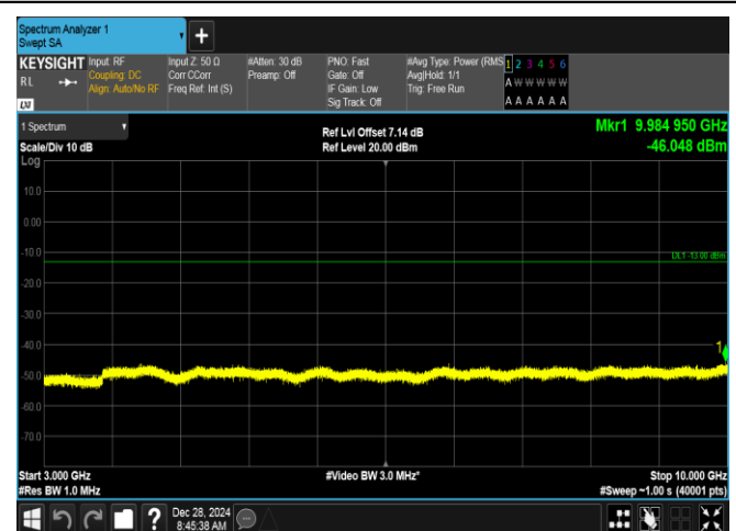
Band5-1.4MHz-16QAM-20407-1RB#0-3000~10000-PASS
