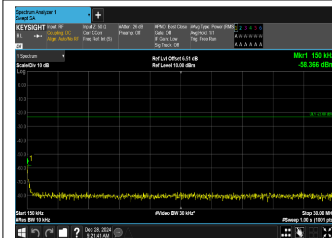
Band5-3MHz-QPSK-20415-1RB#14-0.15~30-PASS
