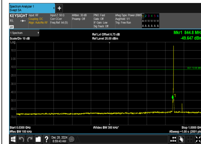
Band5-1.4MHz-16QAM-20643-1RB#5-30~1000-PASS
