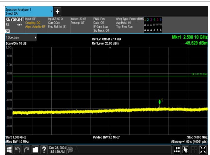
Band5-1.4MHz-16QAM-20525-1RB#0-1000~3000-PASS
