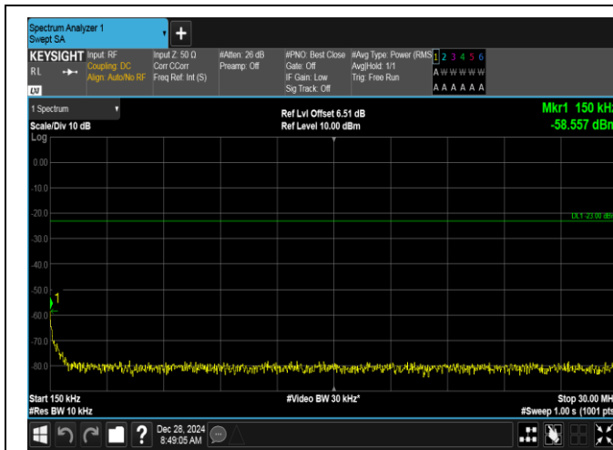
Band5-1.4MHz-16QAM-20407-6RB#0-0.15~30-PASS
