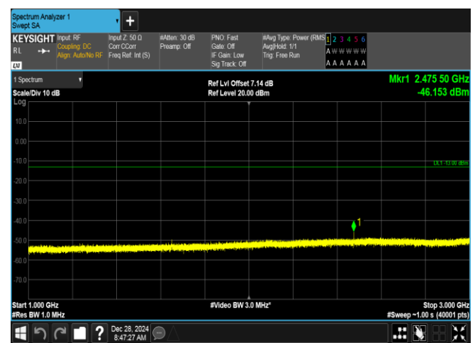
Band5-1.4MHz-16QAM-20407-1RB#5-1000~3000-PASS
