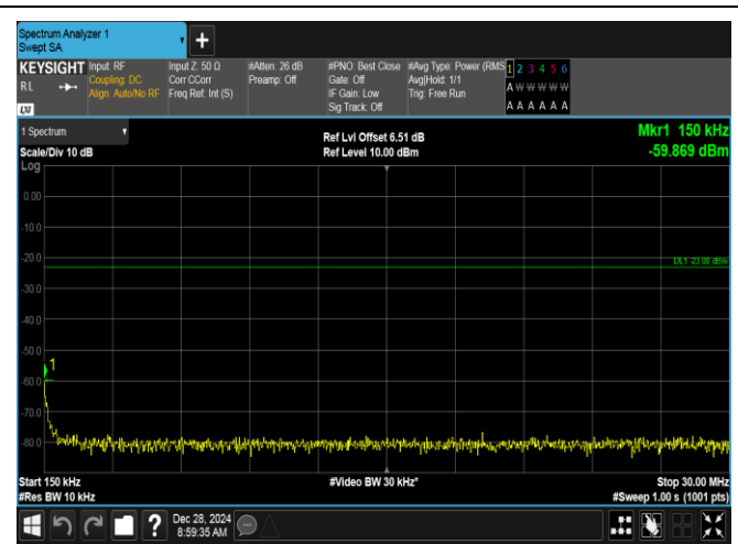
Band5-1.4MHz-16QAM-20643-1RB#5-0.15~30-PASS
