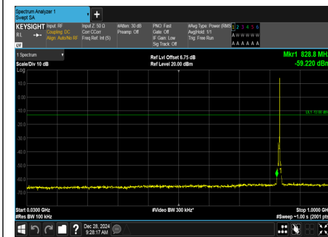
Band5-3MHz-QPSK-20525-1RB#14-30~1000-PASS
