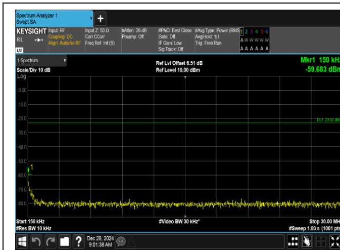
Band5-1.4MHz-16QAM-20643-6RB#0-0.15~30-PASS
