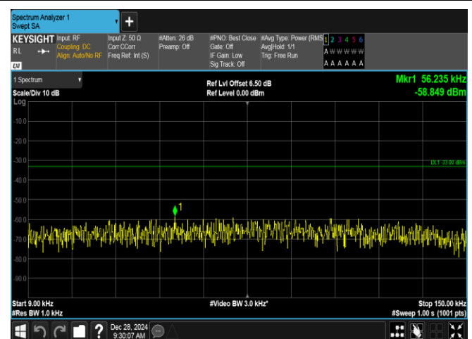
Band5-3MHz-QPSK-20525-15RB#0-0.009~0.15-PASS
