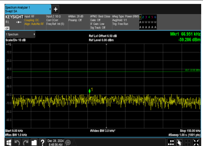
Band5-1.4MHz-16QAM-20407-6RB#0-0.009~0.15-PASS
