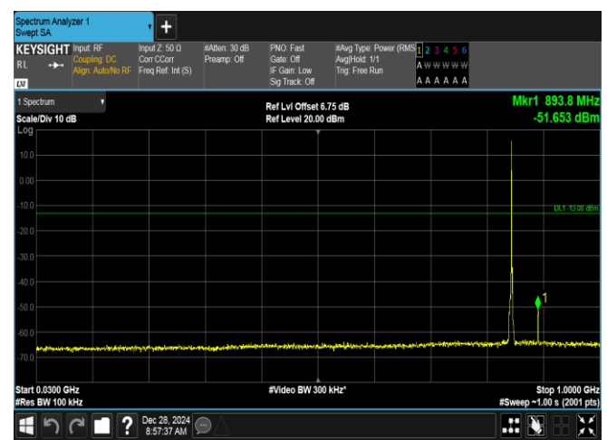
Band5-1.4MHz-16QAM-20643-1RB#0-30~1000-PASS
