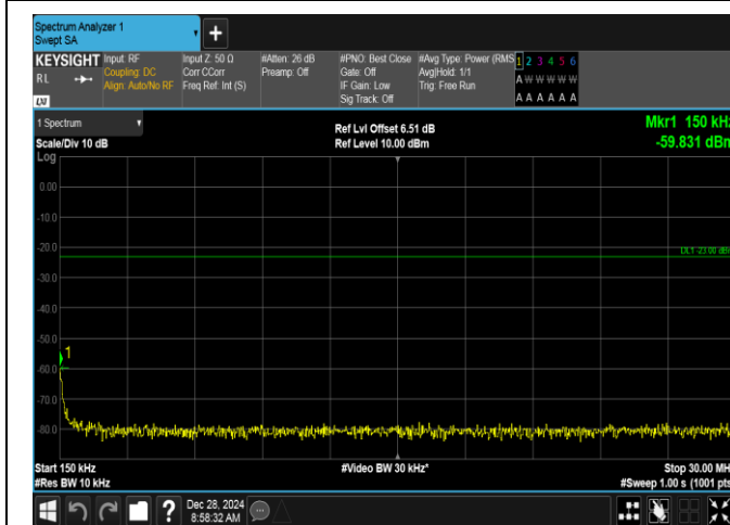
Band5-1.4MHz-QPSK-20643-1RB#5-0.15~30-PASS
