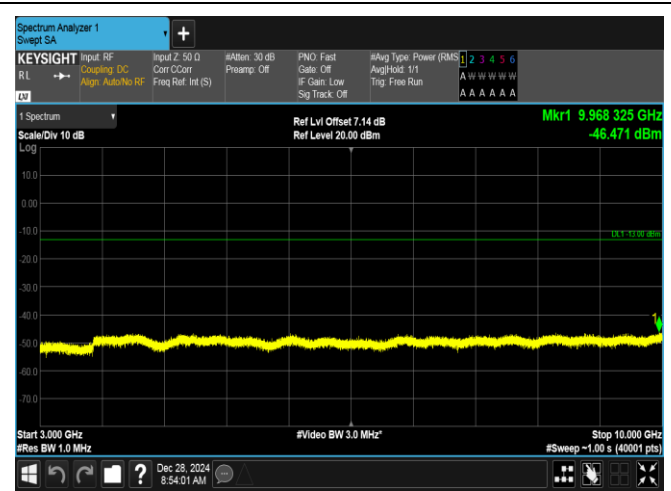
Band5-1.4MHz-16QAM-20525-1RB#5-3000~10000-PASS
