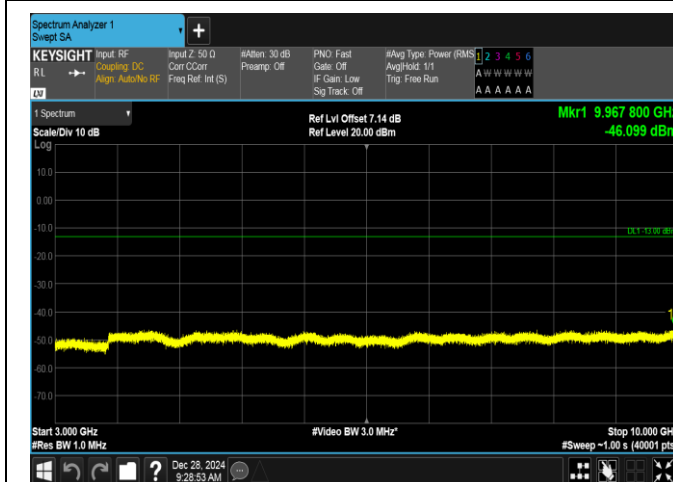
Band5-3MHz-QPSK-20525-1RB#14-3000~10000-PASS
