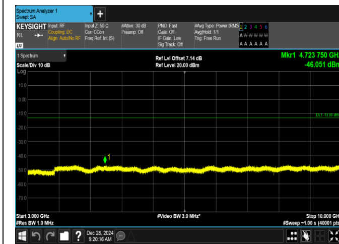
Band5-3MHz-QPSK-20415-1RB#0-3000~10000-PASS
