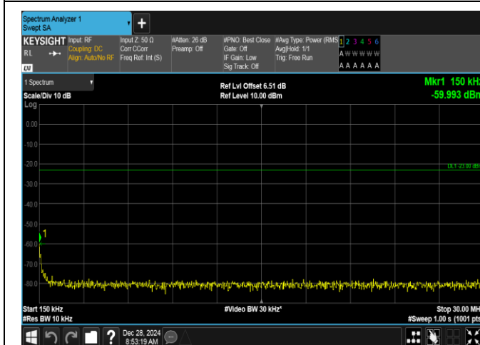
Band5-1.4MHz-16QAM-20525-1RB#5-0.15~30-PASS
