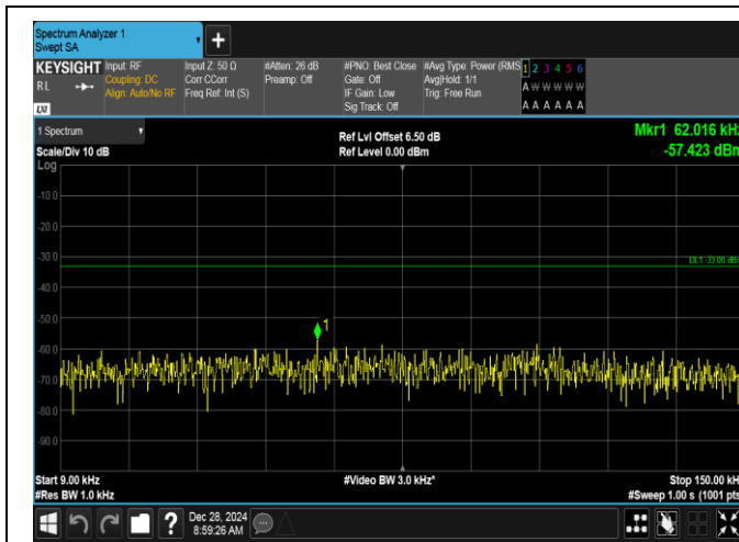
Band5-1.4MHz-16QAM-20643-1RB#5-0.009~0.15-PASS
