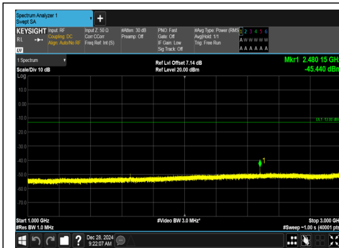
Band5-3MHz-QPSK-20415-1RB#14-1000~3000-PASS
