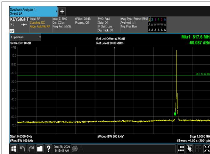
Band5-3MHz-QPSK-20415-1RB#0-30~1000-PASS
