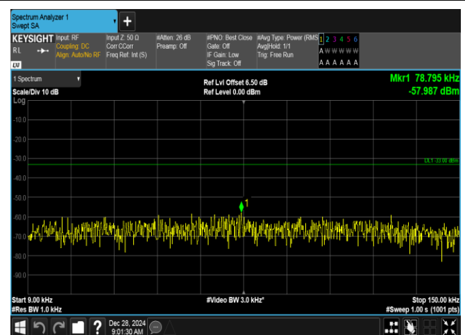
Band5-1.4MHz-16QAM-20643-6RB#0-0.009~0.15-PASS
