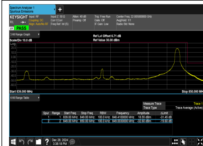
Band5-10MHz-16QAM-20600-1RB#49-PASS
