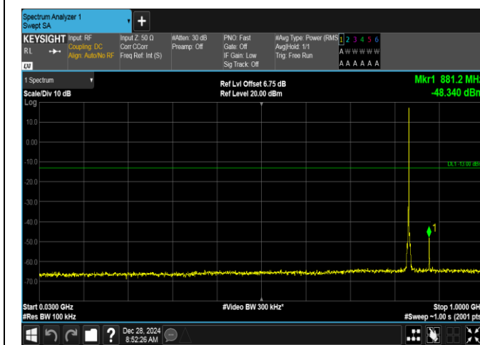
Band5-1.4MHz-QPSK-20525-1RB#5-30~1000-PASS
