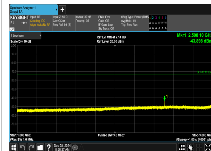
Band5-1.4MHz-QPSK-20525-1RB#0-1000~3000-PASS
