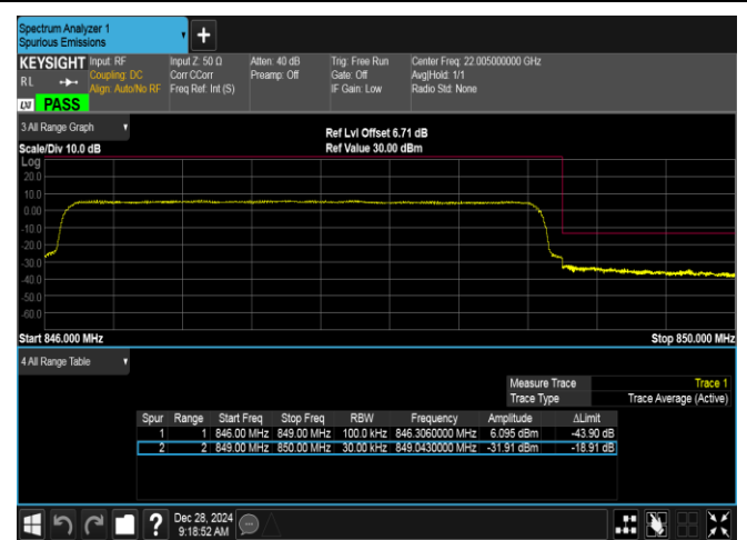
Band5-3MHz-QPSK-20635-15RB#0-PASS
