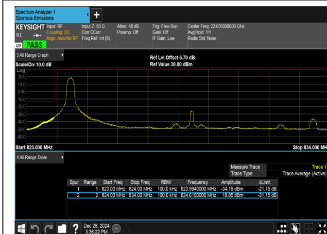
Band5-10MHz-16QAM-20450-1RB#0-PASS
