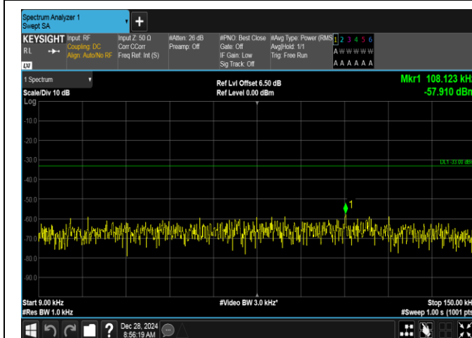
Band5-1.4MHz-QPSK-20643-1RB#0-0.009~0.15-PASS
