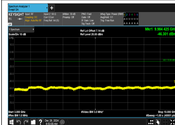
Band5-1.4MHz-QPSK-20525-1RB#5-3000~10000-PASS
