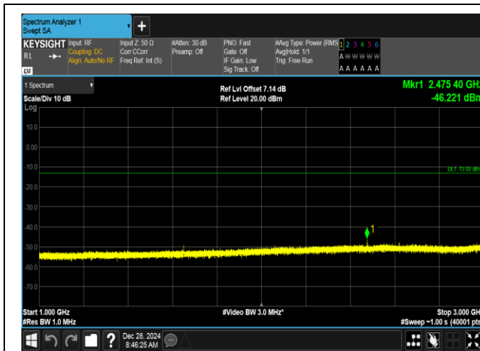
Band5-1.4MHz-QPSK-20407-1RB#5-1000~3000-PASS
