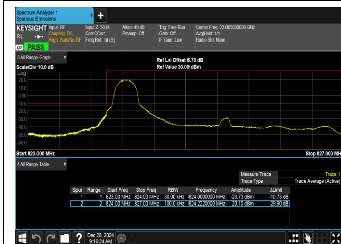
Band5-3MHz-QPSK-20415-1RB#0-PASS
