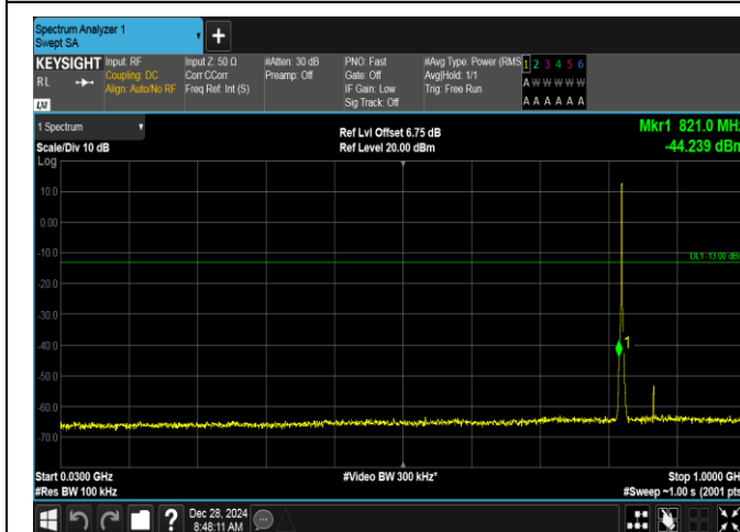
Band5-1.4MHz-QPSK-20407-6RB#0-30~1000-PASS
