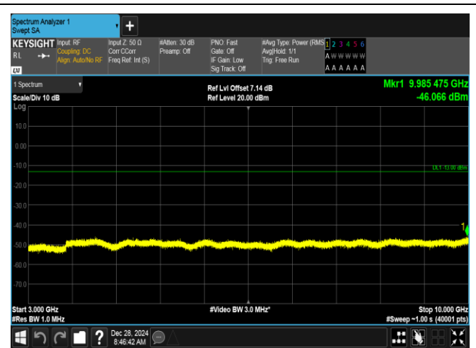
Band5-1.4MHz-QPSK-20407-1RB#5-3000~10000-PASS
