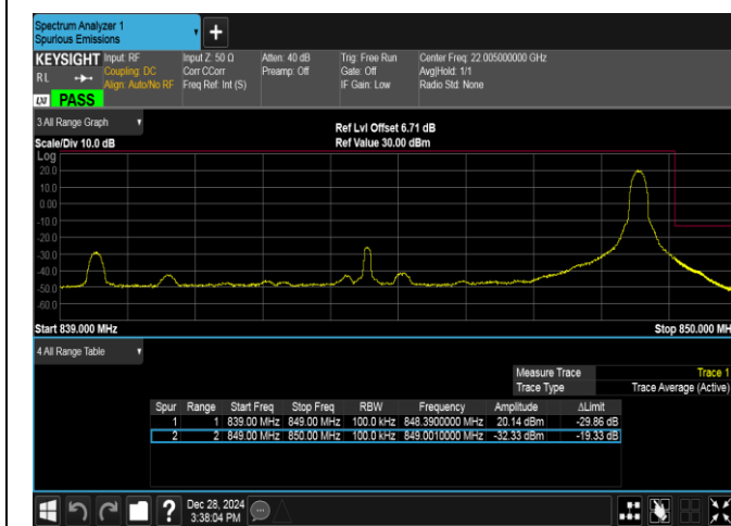
Band5-10MHz-QPSK-20600-1RB#49-PASS
