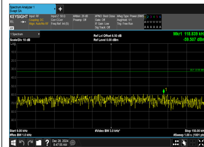
Band5-1.4MHz-QPSK-20407-6RB#0-0.009~0.15-PASS
