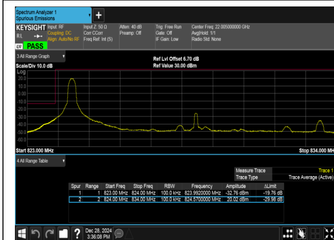
Band5-10MHz-QPSK-20450-1RB#0-PASS
