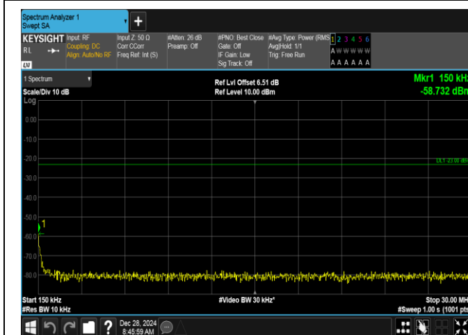
Band5-1.4MHz-QPSK-20407-1RB#5-0.15~30-PASS
