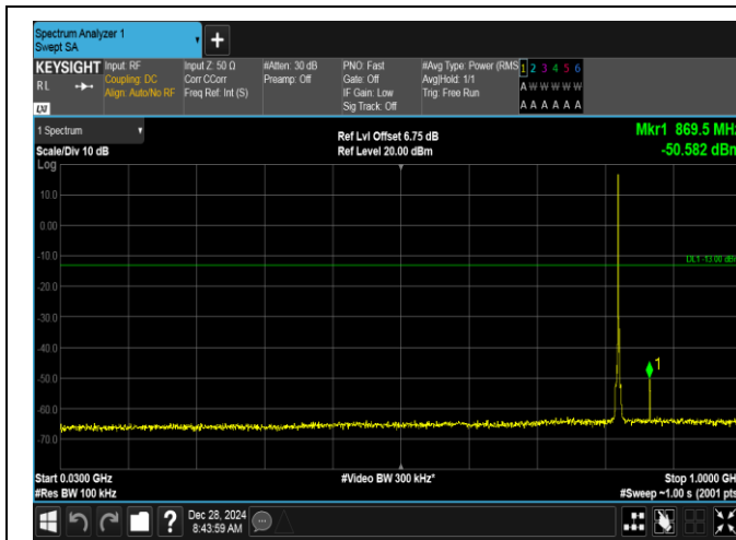
Band5-1.4MHz-QPSK-20407-1RB#0-30~1000-PASS
