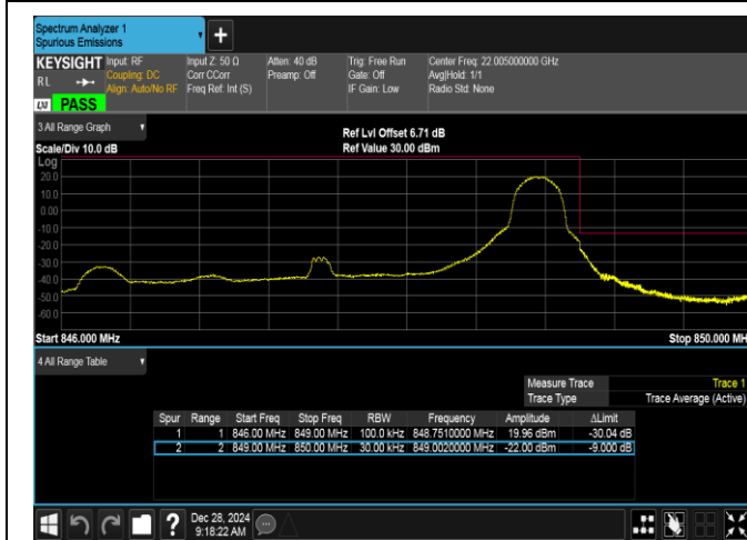
Band5-3MHz-QPSK-20635-1RB#14-PASS
