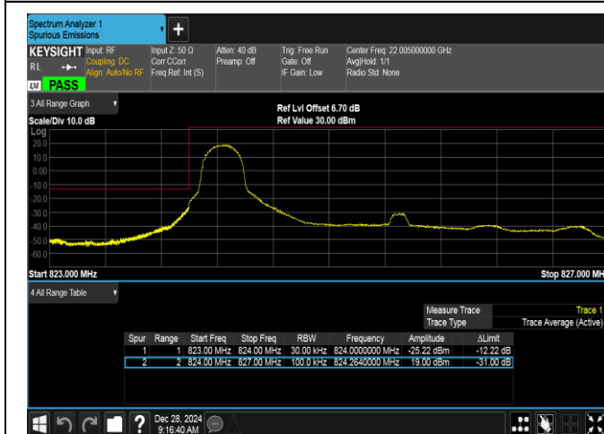
Band5-3MHz-16QAM-20415-1RB#0-PASS
