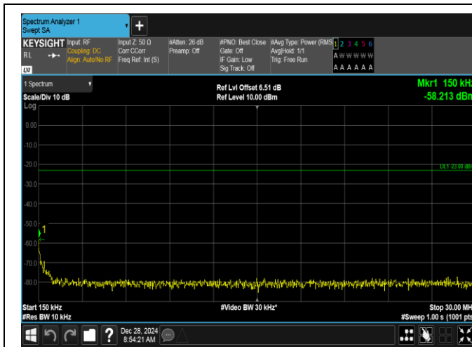
Band5-1.4MHz-QPSK-20525-6RB#0-0.15~30-PASS
