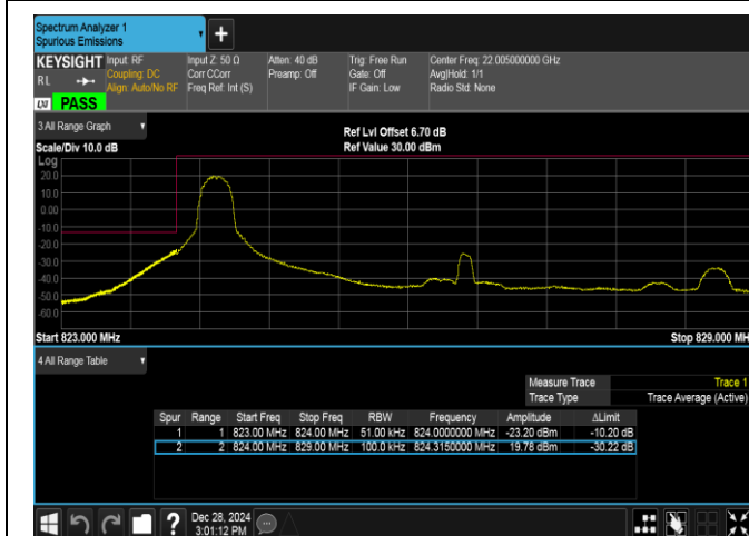
Band5-5MHz-QPSK-20425-1RB#0-PASS
