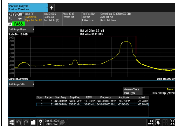
Band5-3MHz-16QAM-20635-1RB#14-PASS
