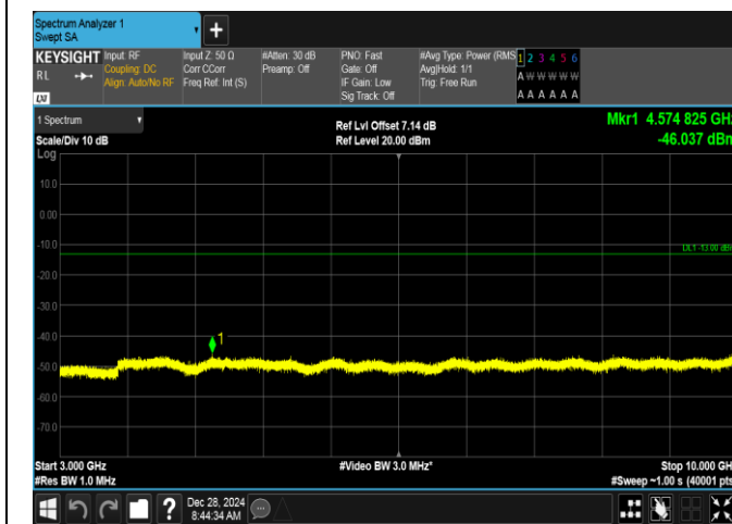
Band5-1.4MHz-QPSK-20407-1RB#0-3000~10000-PASS
