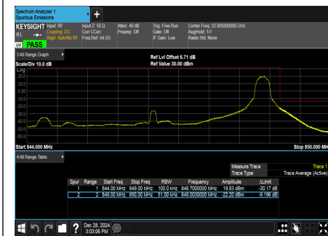
Band5-5MHz-QPSK-20625-1RB#24-PASS
