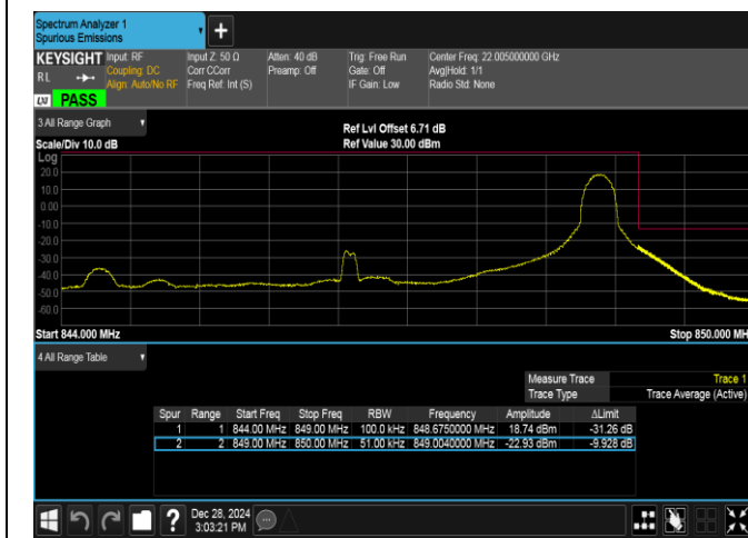
Band5-5MHz-16QAM-20625-1RB#24-PASS
