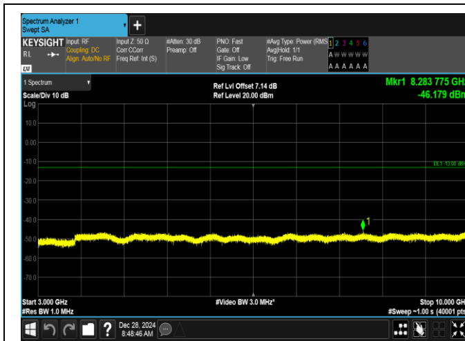
Band5-1.4MHz-QPSK-20407-6RB#0-3000~10000-PASS
