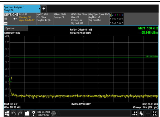
Band5-1.4MHz-QPSK-20525-1RB#5-0.15~30-PASS
