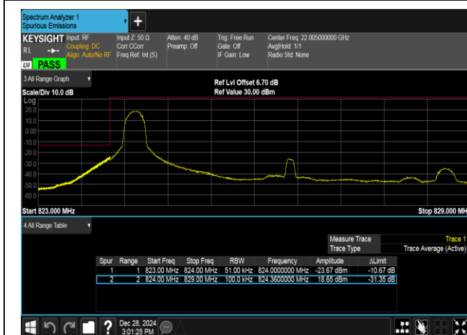
Band5-5MHz-16QAM-20425-1RB#0-PASS
