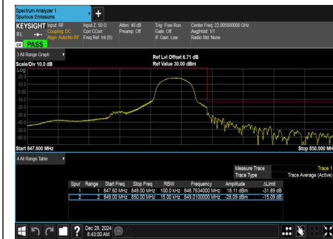
Band5-1.4MHz-16QAM-20643-1RB#5-PASS
