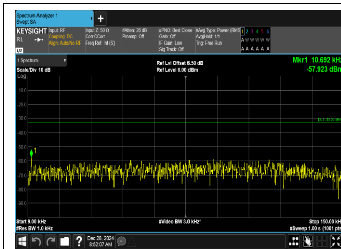
Band5-1.4MHz-QPSK-20525-1RB#5-0.009~0.15-PASS
