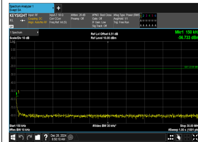
Band5-1.4MHz-QPSK-20525-1RB#0-0.15~30-PASS
