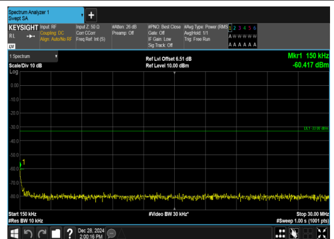
Band4-20MHz-QPSK-20050-100RB#0-0.15~30-PASS
