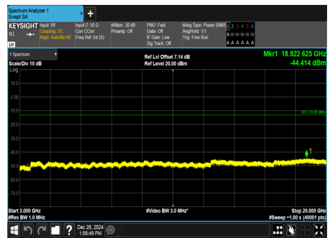
Band4-20MHz-QPSK-20050-1RB#99-3000~20000-PASS
