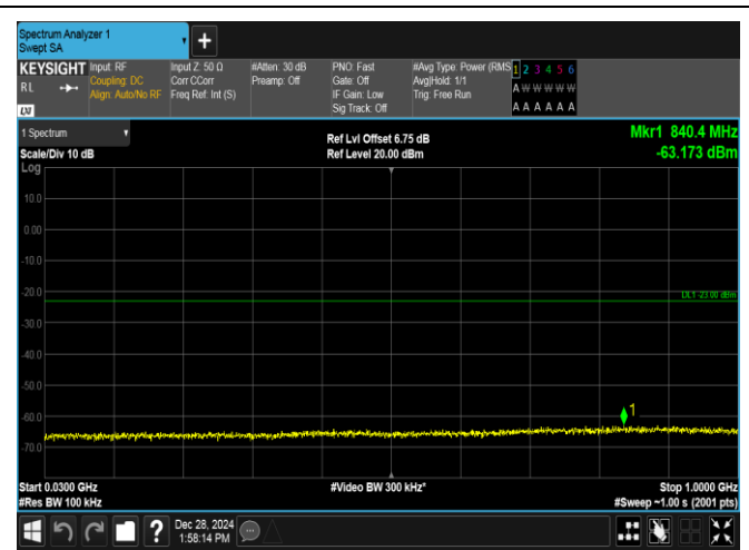
Band4-20MHz-QPSK-20050-1RB#99-30~1000-PASS
