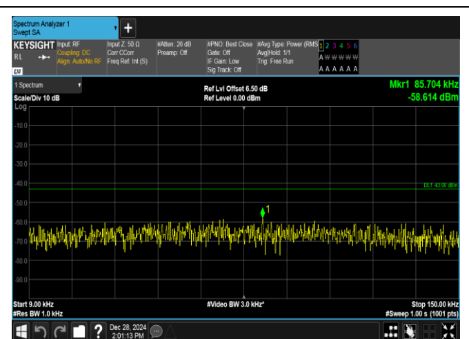
Band4-20MHz-16OAM-20050-100RB#0-0.009~0.15-PASS
