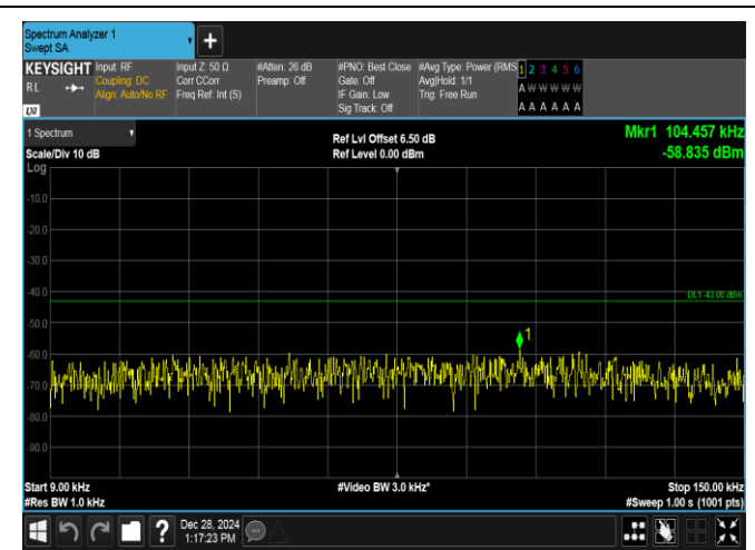
Band4-15MHz-QPSK-20175-75RB#0-0.009~0.15-PASS
