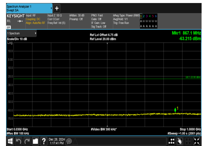
Band4-15MHz-QPSK-20175-75RB#0-30~1000-PASS
