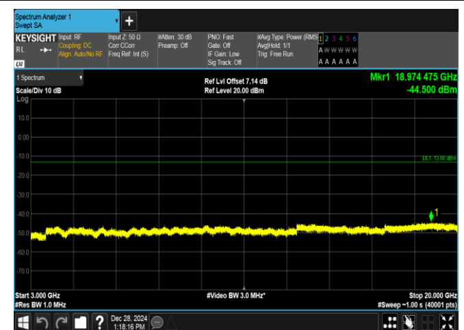
Band4-15MHz-QPSK-20175-75RB#0-3000~20000-PASS
