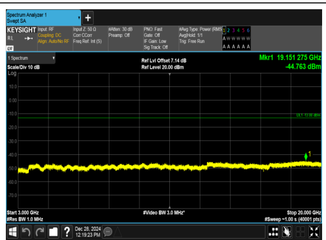
Band4-10MHz-16QAM-20000-1RB#0-3000~20000-PASS
