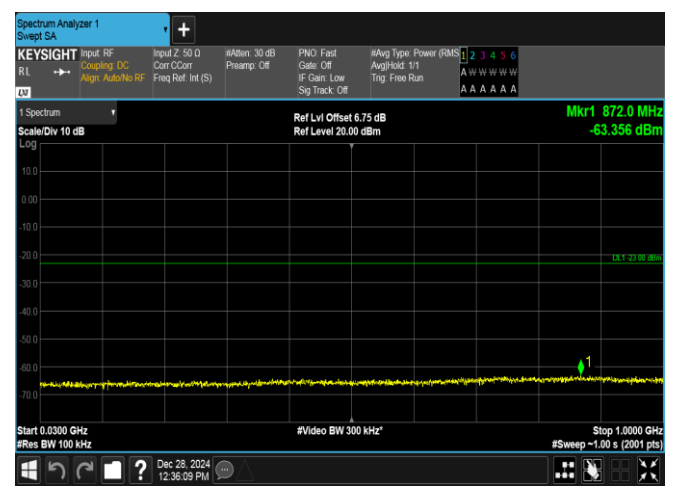
Band4-10MHz-16QAM-20350-50RB#0-30~1000-PASS
