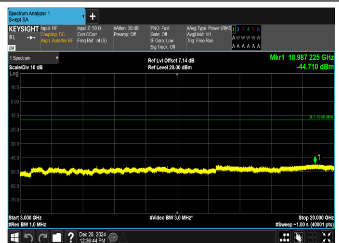
Band4-10MHz-16QAM-20350-50RB#0-3000~20000-PASS
