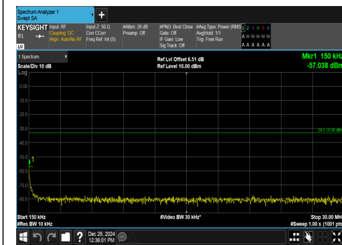
Band4-10MHz-16QAM-20350-50RB#0-0.15~30-PASS
