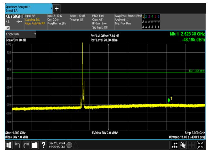
Band4-10MHz-16QAM-20175-1RB#0-1000~3000-PASS
