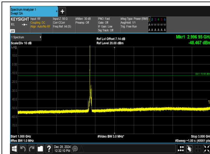
Band4-10MHz-16QAM-20350-1RB#0-1000~3000-PASS
