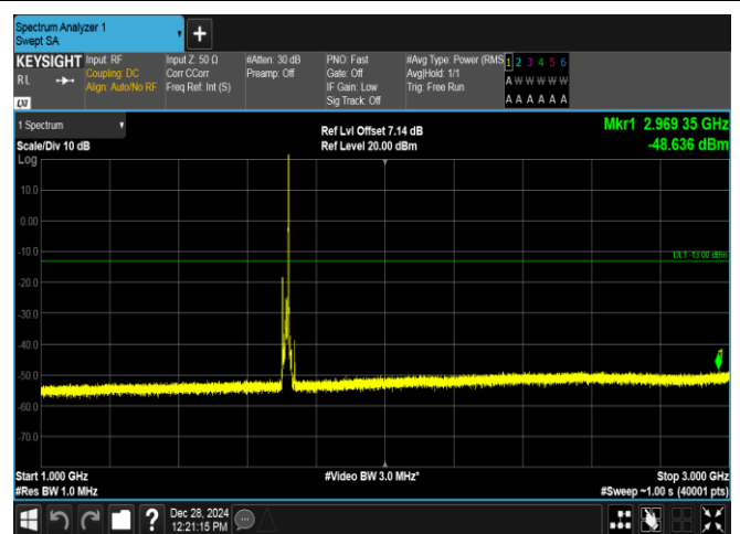
Band4-10MHz-16QAM-20000-1RB#49-1000~3000-PASS
