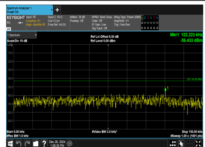
Band4-15MHz-QPSK-2025-1RB#74-0.009~0.15-PASS
