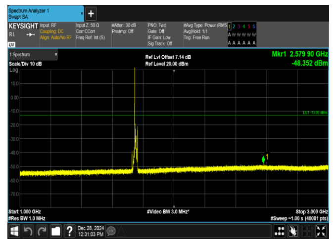
Band4-10MHz-QPSK-20350-1RB#0-1000~3000-PASS
