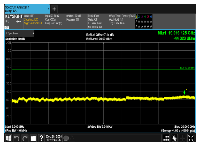
Band4-10MHz-16QAM-20000-50RB#0-3000~20000-PASS
