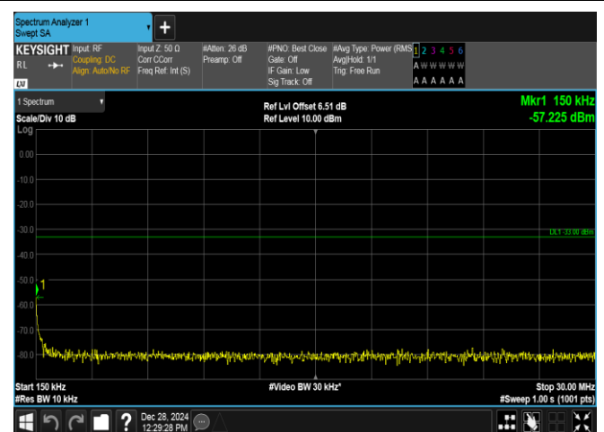
Band4-10MHz-16QAM-20175-50RB#0-0.15~30-PASS
