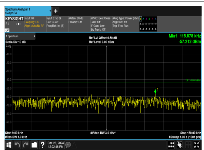
Band4-10MHz-16QAM-20000-50RB#0-0.009~0.15-PASS
