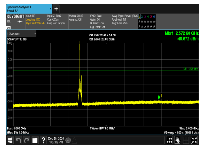
Band4-15MHz-QPSK-2025-1RB#0-1000~3000-PASS
