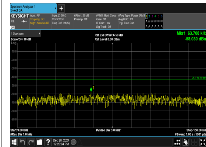
Band4-10MHz-QPSK-20175-1RB#49-0.009~0.15-PASS
