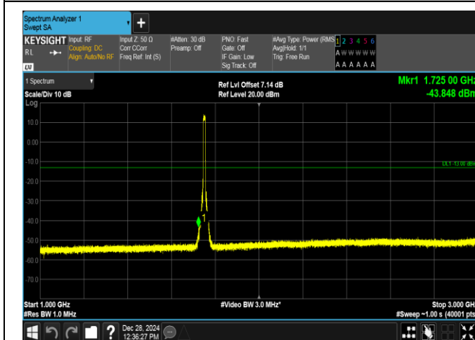
Band4-10MHz-16QAM-20350-50RB#0-1000~3000-PASS
