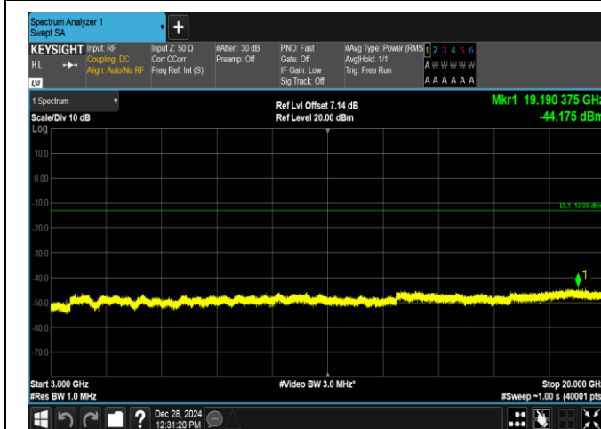
Band4-10MHz-QPSK-20350-1RB#0-3000~20000-PASS
