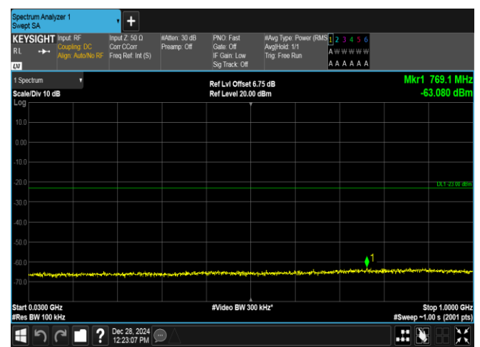
Band4-10MHz-16QAM-20000-50RB#0-30~1000-PASS
