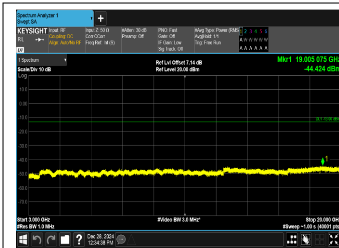
Band4-10MHz-16QAM-20350-1RB#49-3000~20000-PASS
