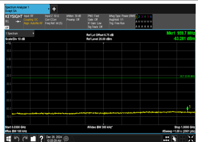
Band4-1.4MHz-16QAM-20393-1RB#0-30~1000-PASS
