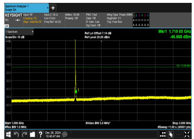
Band4-3MHz-QPSK-19965-1RB#0-1000~3000-PASS
