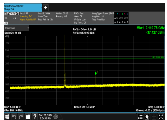
Band4-1.4MHz-16QAM-19957-1RB#5-1000~3000-PASS
