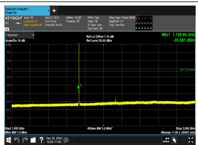
Band4-1.4MHz-16QAM-20175-6RB#0-1000~3000-PASS
