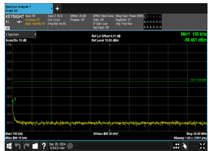
Band4-1.4MHz-16QAM-19957-1RB#5-0.15~30-PASS
