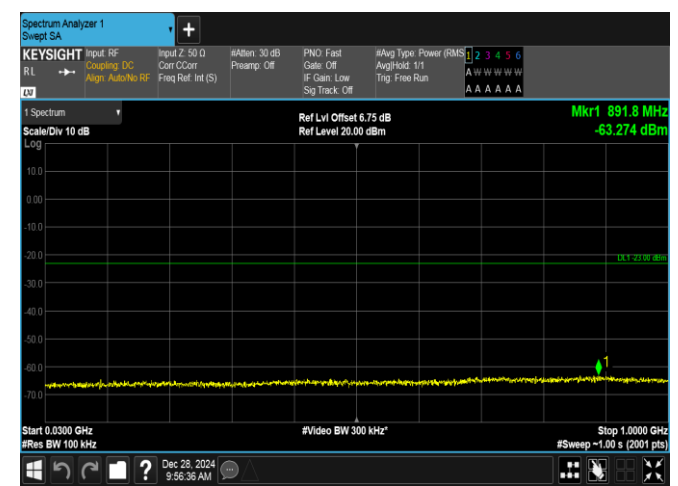
Band4-1.4MHz-16QAM-19957-6RB#0-30~1000-PASS
