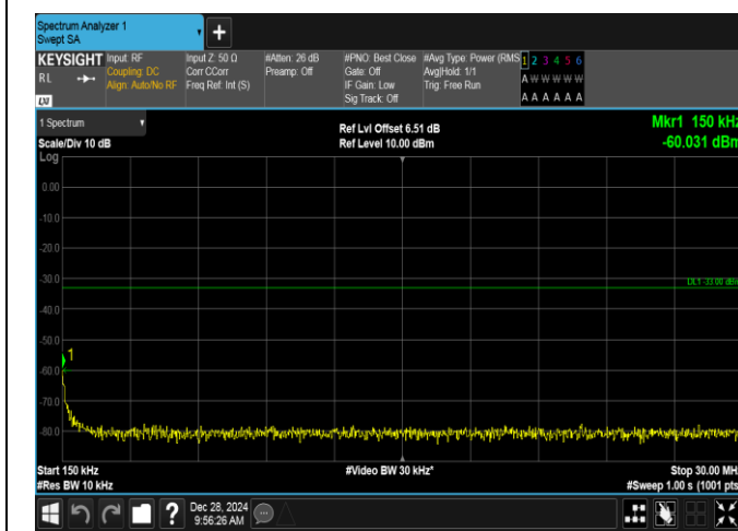
Band4-1.4MHz-16QAM-19957-6RB#0-0.15~30-PASS
