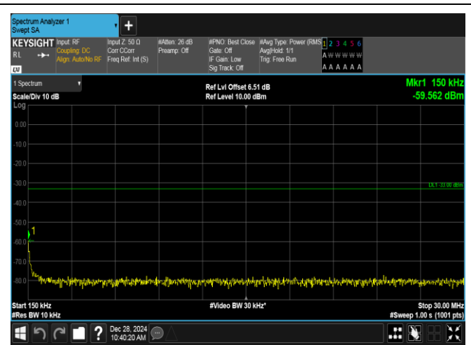
Band4-3MHz-QPSK-19965-1RB#0-0.15~30-PASS
