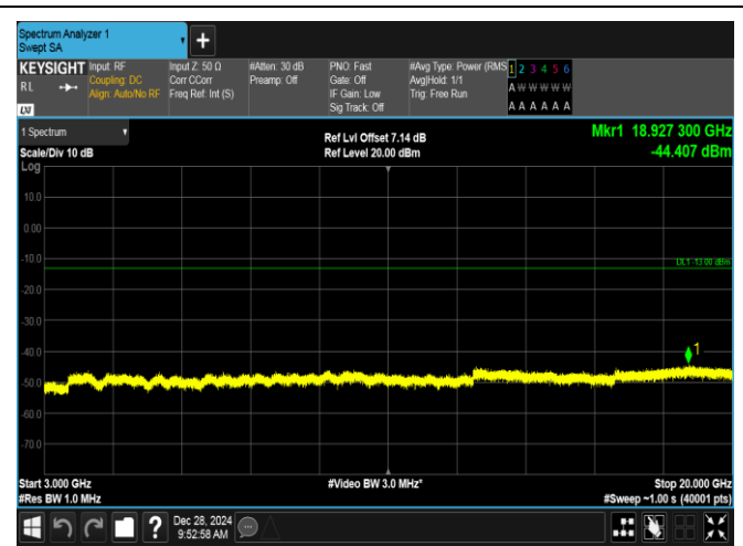
Band4-1.4MHz-16QAM-19957-1RB#0-3000~20000-PASS
