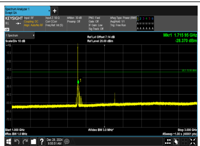
Band4-1.4MHz-QPSK-19957-6RB#0-1000~3000-PASS
