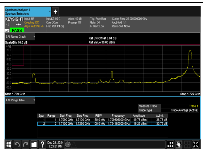
Band4-15MHz-QPSK-20025-1RB#74-PASS
