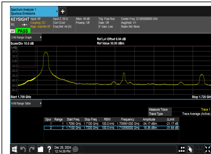
Band4-10MHz-16QAM-20000-1RB#0-PASS
