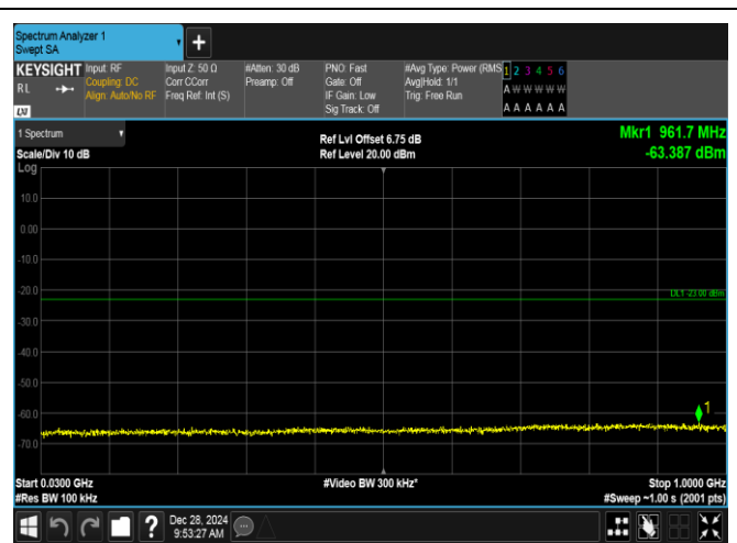
Band4-1.4MHz-QPSK-19957-1RB#5-30~1000-PASS
