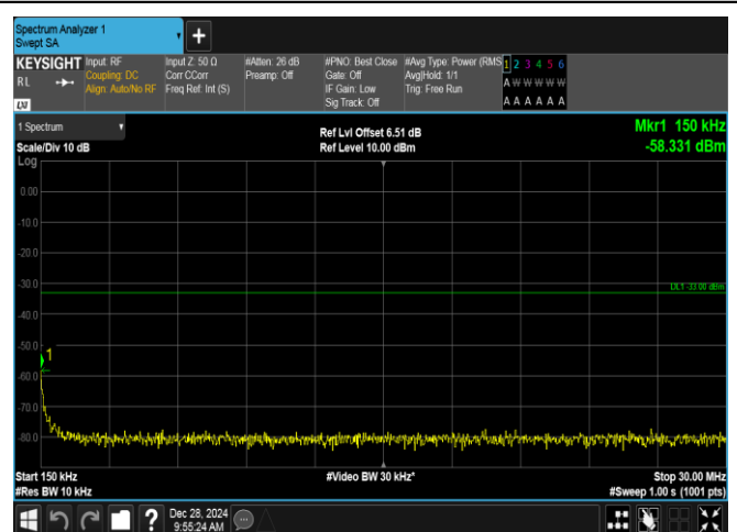
Band4-1.4MHz-QPSK-19957-6RB#0-0.15~30-PASS
