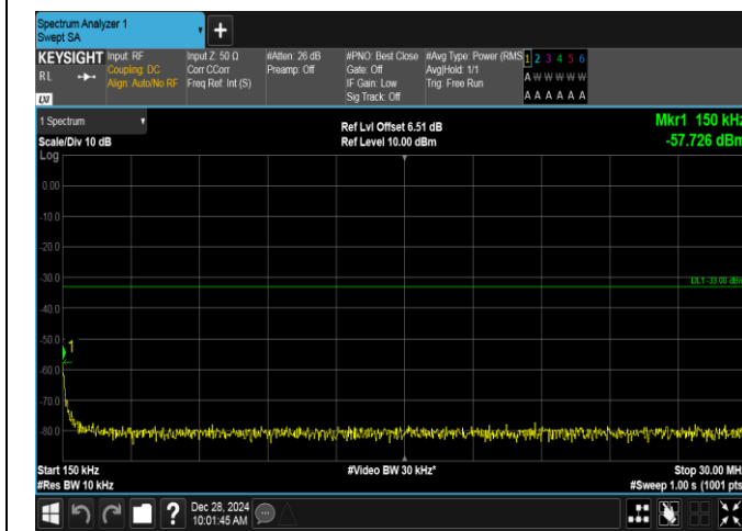
Band4-1.4MHz-QPSK-20175-6RB#0-0.15~30-PASS
