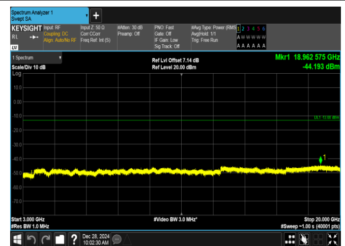
Band4-1.4MHz-QPSK-20175-6RB#0-3000~20000-PASS
