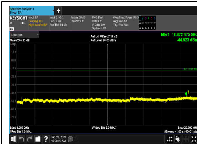
Band4-1.4MHz-QPSK-20175-1RB#5-3000~20000-PASS
