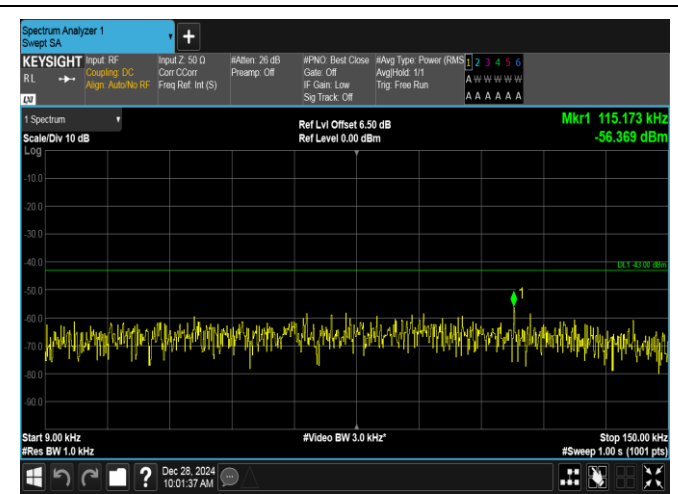
Band4-1.4MHz-QPSK-20175-6RB#0-0.009~0.15-PASS
