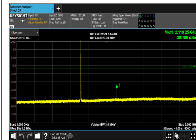
Band4-1.4MHz-QPSK-19957-1RB#5-1000~3000-PASS
