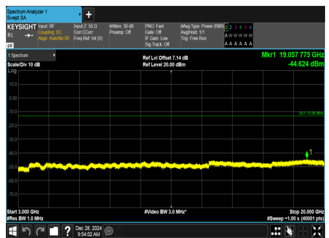
Band4-1.4MHz-QPSK-19957-1RB#5-3000~20000-PASS
