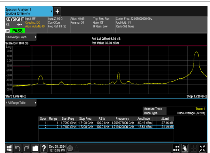
Band4-10MHz-16QAM-20000-1RB#49-PASS
