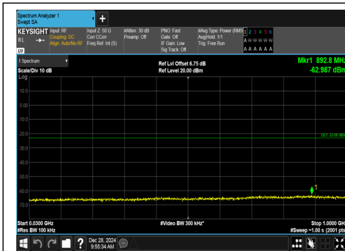
Band4-1.4MHz-QPSK-19957-6RB#0-30~1000-PASS
