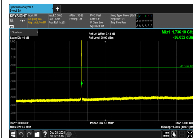
Band4-1.4MHz-QPSK-20175-6RB#0-1000~3000-PASS
