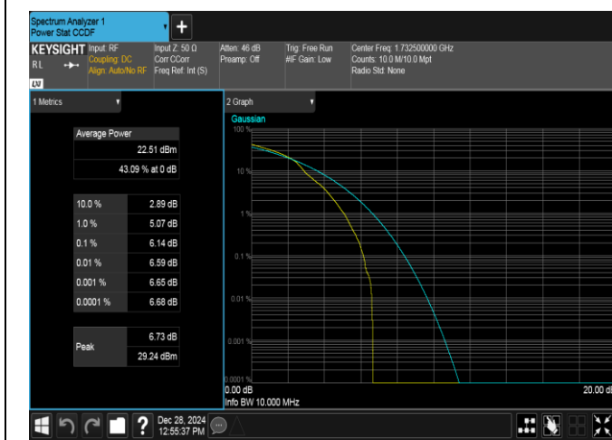
Band4-10MHz-16QAM-20175-1RB#0-PASS
