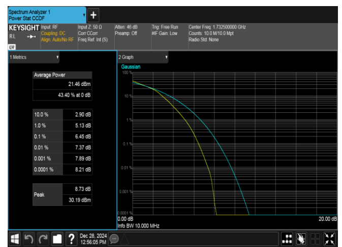
Band4-10MHz-16QAM-20175-50RB#0-PASS
