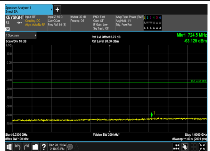
Band4-20MHz-16QAM-20300-1RB#0-30~1000-PASS
