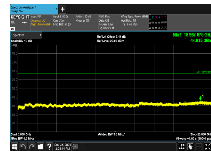
Band4-20MHz-16QAM-20175-100RB#0-3000~20000-PASS S
