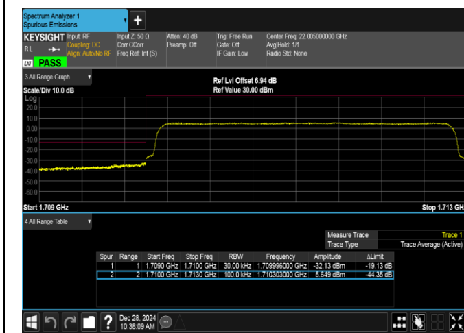
Band4-3MHz-QPSK-19965-15RB#0-PASS
