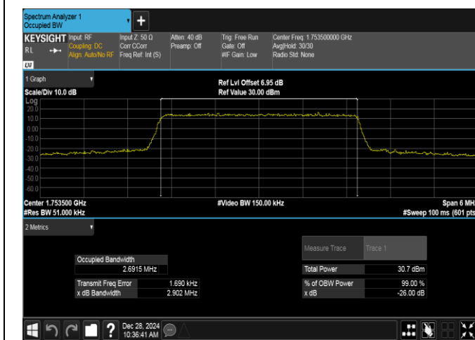
Band4-3MHz-QPSK-20385-15RB#0-PASS
