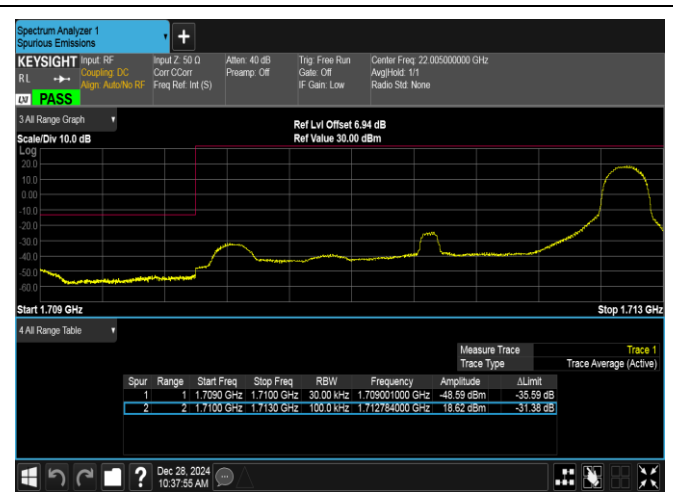
Band4-3MHz-16QAM-19965-1RB#14-PASS
