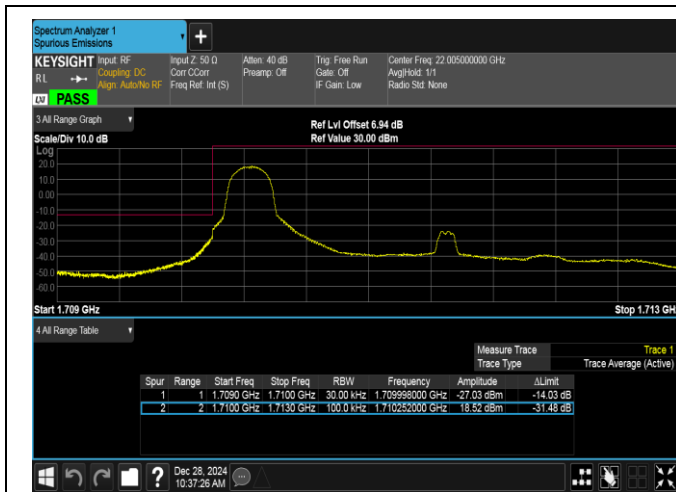
Band4-3MHz-16QAM-19965-1RB#0-PASS
