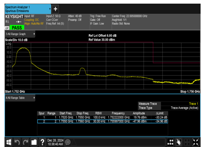
Band4-3MHz-QPSK-20385-1RB#0-PASS
