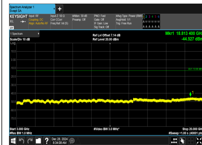
Band2-20MHz-QPSK-19100-100RB#0-3000~20000-PASS
