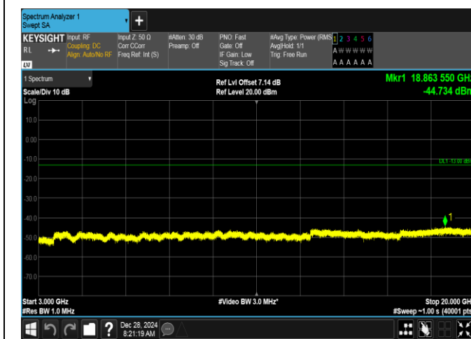
Band2-20MHz-QPSK-18700-100RB#0-3000~20000-PASS
