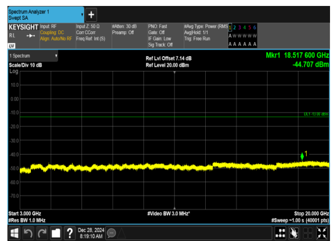
Band2-20MHz-QPSK-18700-1RB#99-3000~20000-PASS
