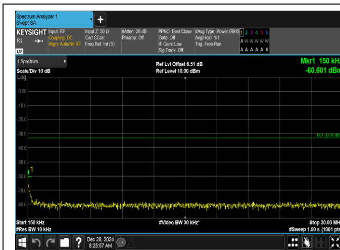
Band2-20MHz-16QAM-18900-1RB#99-0.15~30-PASS
