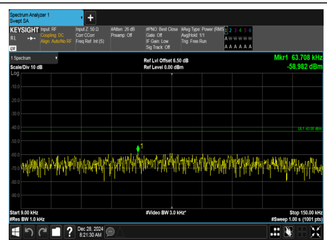
Band2-20MHz-16QAM-18700-100RB#0-0.009~0.15-PASS
