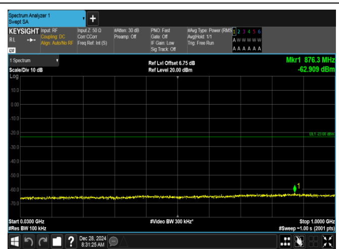
Band2-20MHz-QPSK-19100-1RB#99-30~1000-PASS
