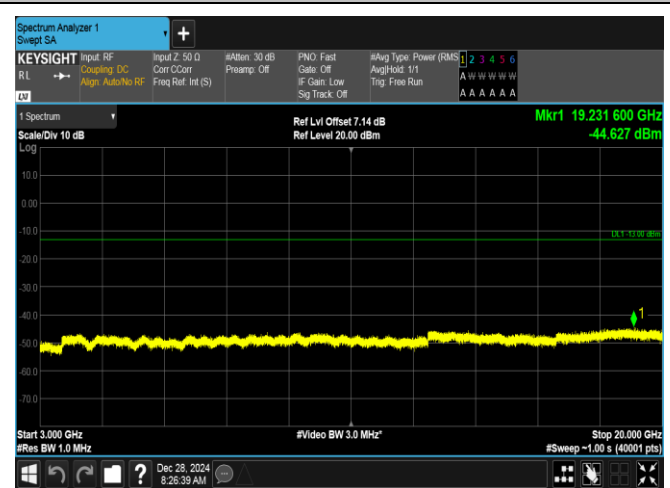
Band2-20MHz-16QAM-18900-1RB#99-3000~20000-PASS
