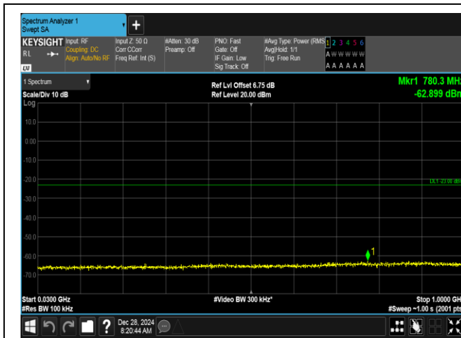
Band2-20MHz-QPSK-18700-100RB#0-30~1000-PASS
