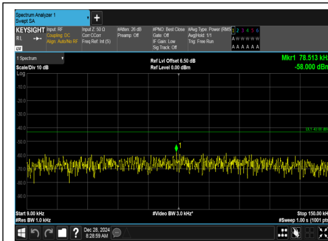
Band2-20MHz-QPSK-19100-1RB#0-0.009~0.15-PASS
