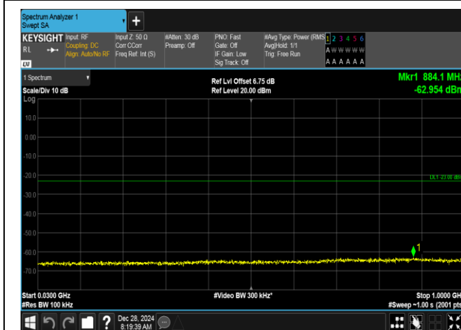
Band2-20MHz-16QAM-18700-1RB#99-30~1000-PASS
