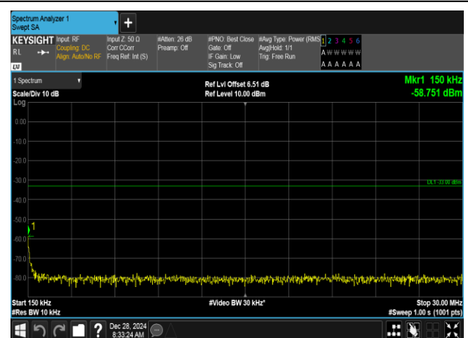
Band2-20MHz-QPSK-19100-100RB#0-0.15~30-PASS
