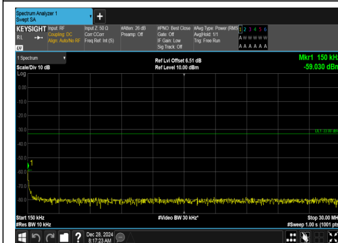
Band2-20MHz-16QAM-18700-1RB#0-0.15~30-PASS
