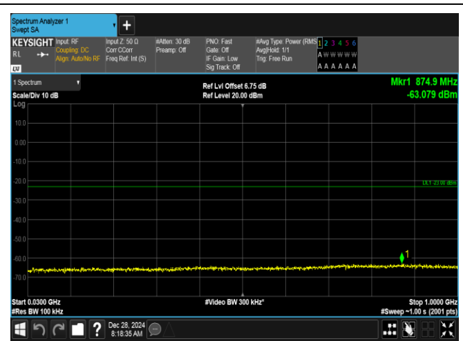
Band2-20MHz-QPSK-18700-1RB#99-30~1000-PASS
