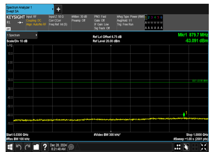
Band2-20MHz-16QAM-18700-100RB#0-30~1000-PASS
