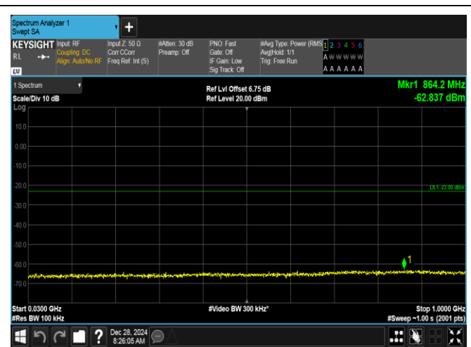
Band2-20MHz-16QAM-18900-1RB#99-30~1000-PASS
