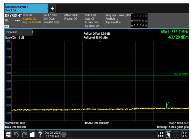
Band2-20MHz-QPSK-18900-100RB#0-30~1000-PASS
