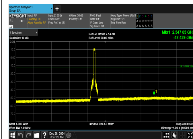
Band2-20MHz-QPSK-18900-100RB#0-1000~3000-PASS
