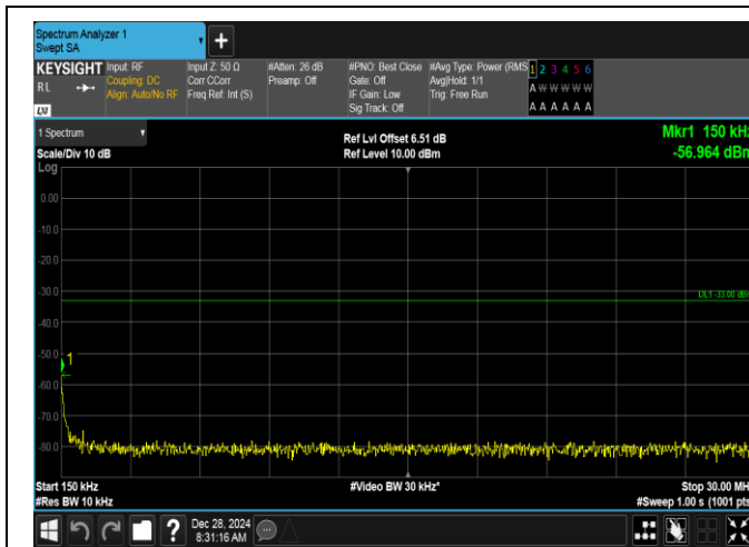
Band2-20MHz-QPSK-19100-1RB#99-0.15~30-PASS
