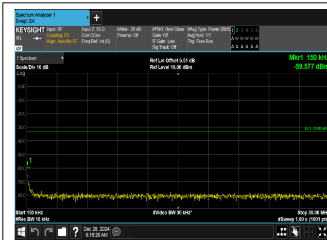
Band2-20MHz-QPSK-18700-1RB#99-0.15~30-PASS
