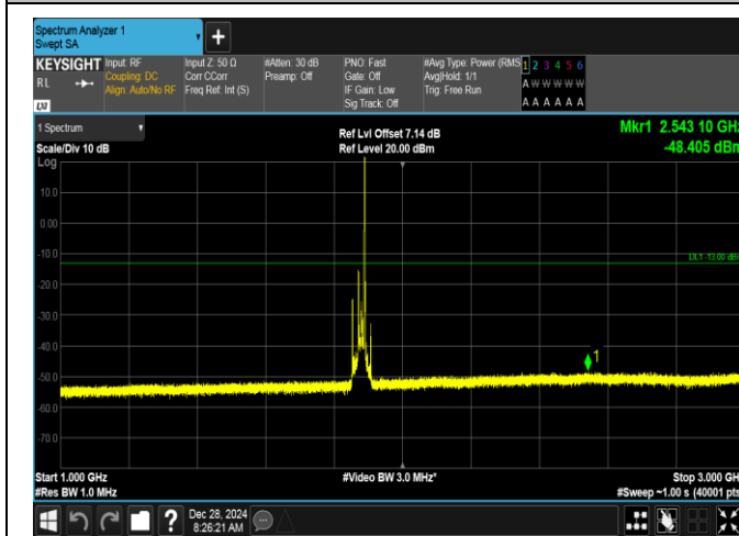
Band2-20MHz-16QAM-18900-1RB#99-1000~3000-PASS
