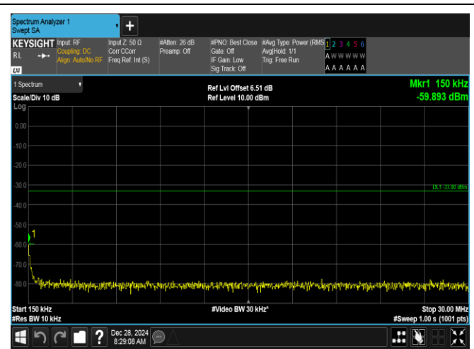
Band2-20MHz-QPSK-19100-1RB#0-0.15~30-PASS
