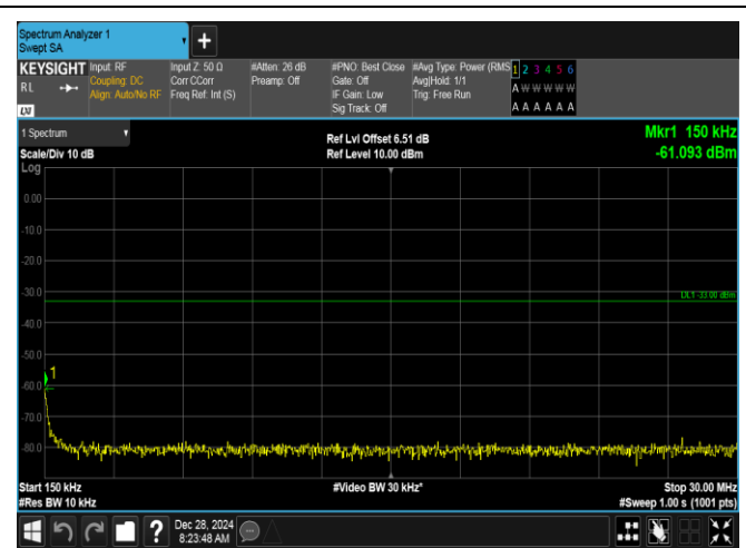
Band2-20MHz-16QAM-18900-1RB#0-0.15~30-PASS
