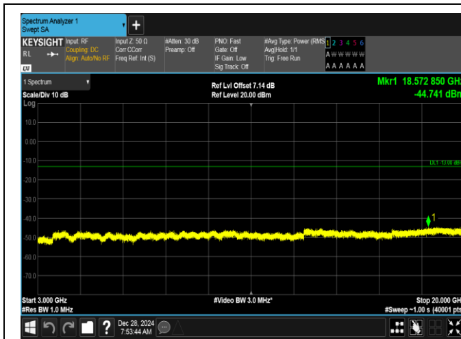
Band2-15MHz-16QAM-19125-1RB#74-3000~20000-PASS
