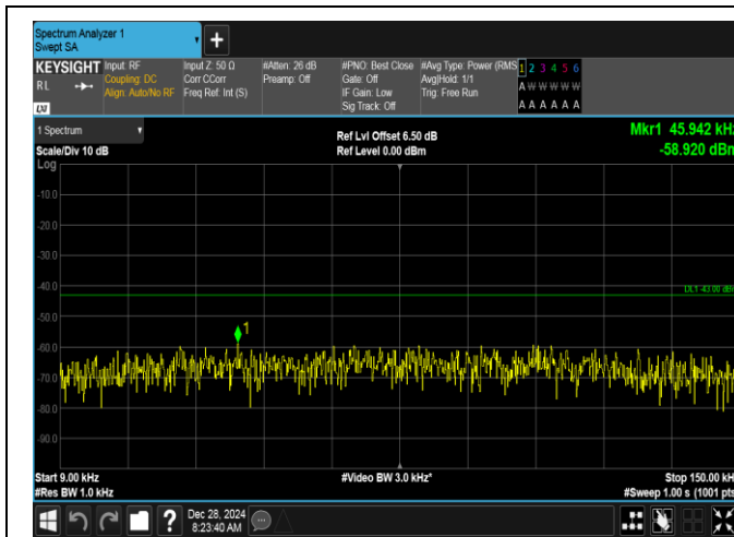
Band2-20MHz-16QAM-18900-1RB#0-0.009~0.15-PASS
