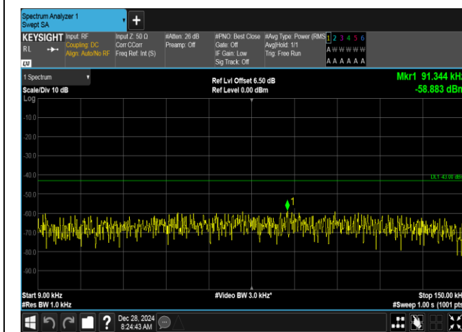
Band2-20MHz-QPSK-18900-1RB#99-0.009~0.15-PASS
