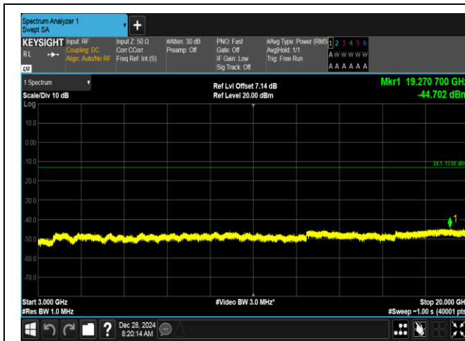
Band2-20MHz-16QAM-18700-1RB#99-3000~20000-PASS
