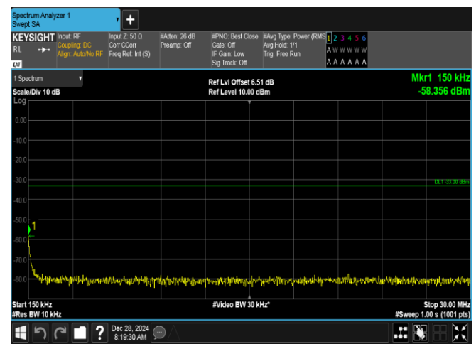
Band2-20MHz-16QAM-18700-1RB#99-0.15~30-PASS
