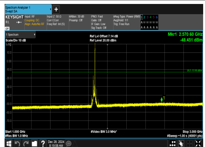
Band2-20MHz-16QAM-18700-1RB#99-1000~3000-PASS
