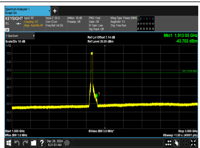
Band2-20MHz-QPSK-18700-100RB#0-1000~3000-PASS
