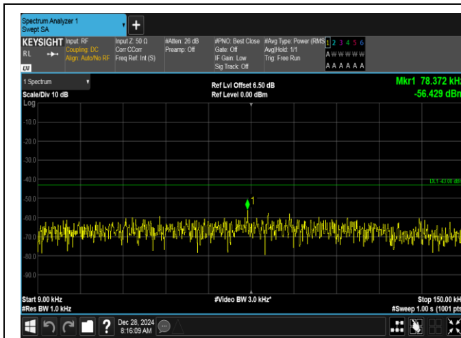
Band2-20MHz-QPSK-18700-1RB#0-0.009~0.15-PASS
