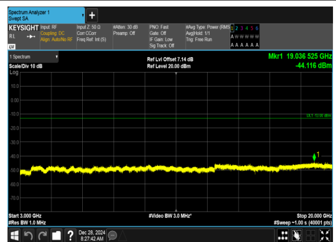
Band2-20MHz-QPSK-18900-100RB#0-3000~20000-PASS
