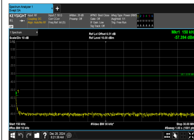
Band2-20MHz-16QAM-18700-100RB#0-0.15~30-PASS
