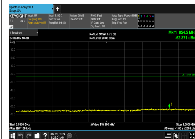
Band2-20MHz-QPSK-18900-1RB#99-30~1000-PASS
