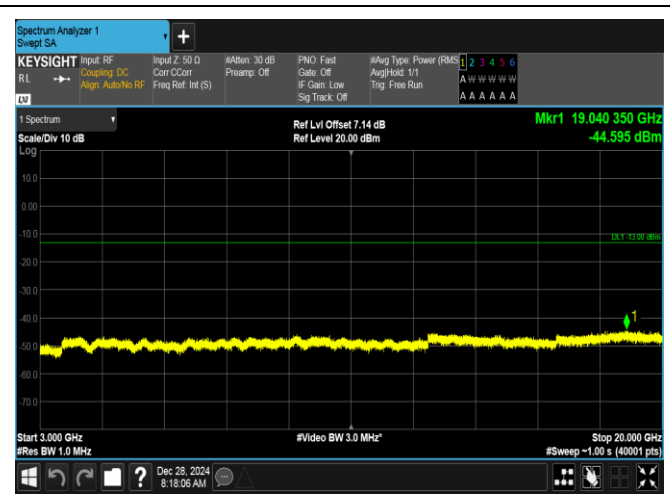
Band2-20MHz-16QAM-18700-1RB#0-3000~20000-PASS
