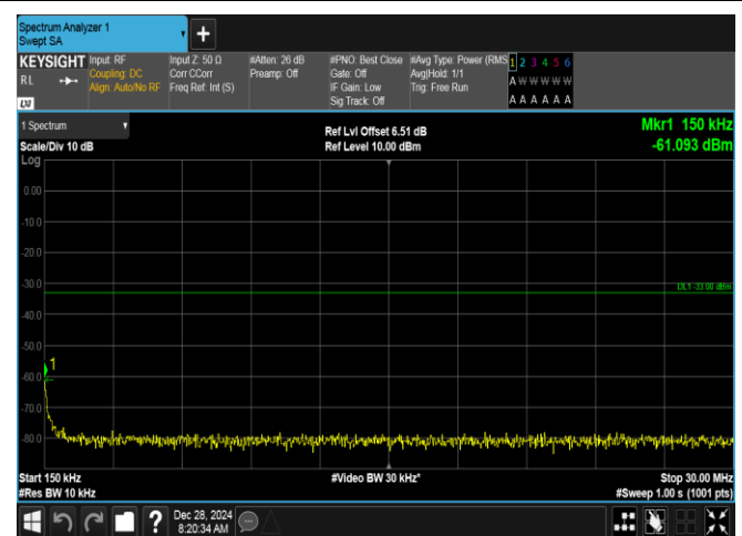
Band2-20MHz-QPSK-18700-100RB#0-0.15~30-PASS
