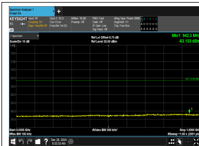
Band2-20MHz-QPSK-19100-100RB#0-30~1000-PASS
