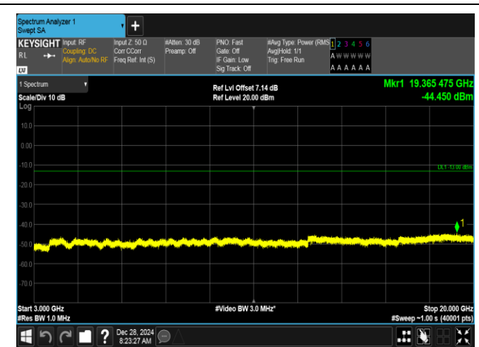
Band2-20MHz-QPSK-18900-1RB#0-3000~20000-PASS
