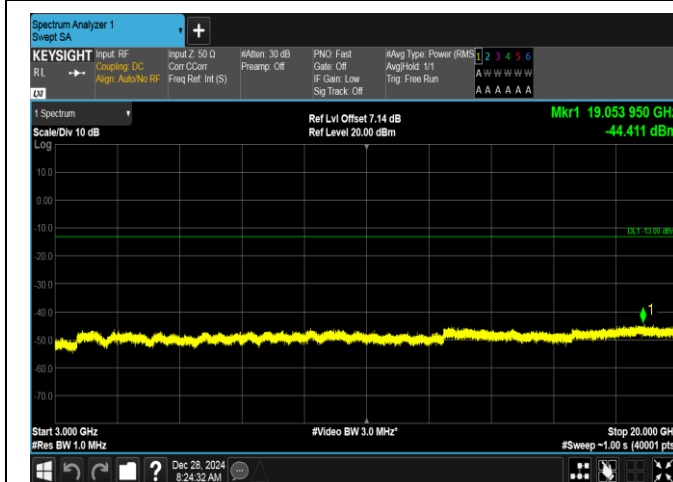
Band2-20MHz-16QAM-18900-1RB#0-3000~20000-PASS
