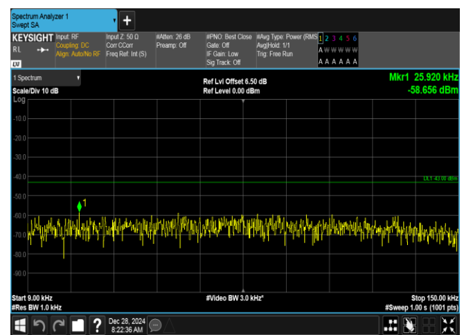
Band2-20MHz-QPSK-18900-1RB#0-0.009~0.15-PASS
