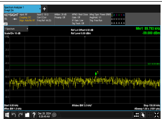
Band2-20MHz-QPSK-18900-100RB#0-0.009~0.15-PASS
