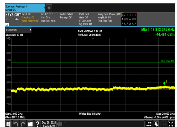
Band2-20MHz-16QAM-18700-100RB#0-3000~20000-PAS
