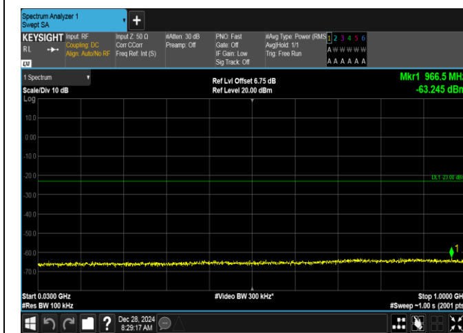
Band2-20MHz-QPSK-19100-1RB#0-30~1000-PASS
