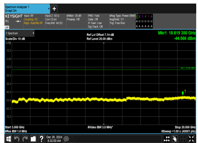
Band2-20MHz-QPSK-19100-1RB#99-3000~20000-PASS
