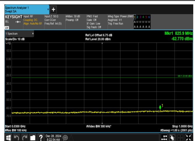
Band2-20MHz-QPSK-18900-1RB#0-30~1000-PASS
