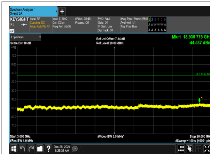
Band2-20MHz-QPSK-18900-1RB#99-3000~20000-PASS
