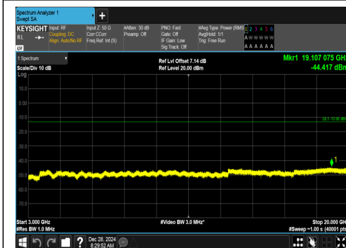
Band2-20MHz-QPSK-19100-1RB#0-3000~20000-PASS
