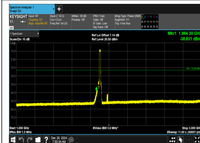
Band2-15MHz-16QAM-19125-75RB#0-1000~3000-PASS
