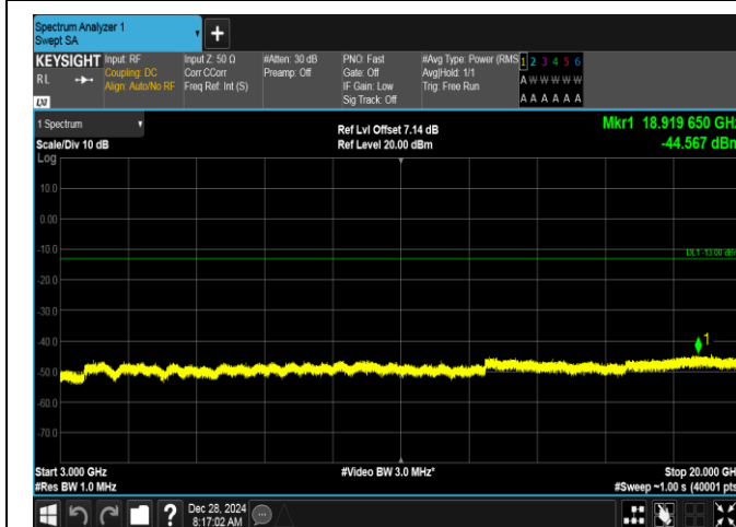
Band2-20MHz-QPSK-18700-1RB#0-3000~20000-PASS
