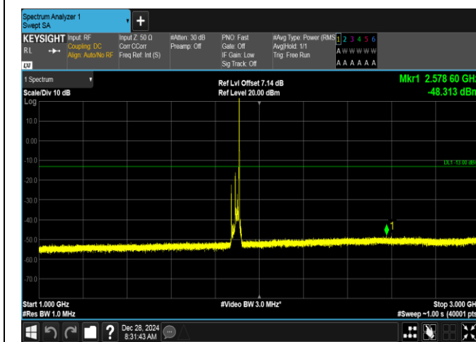
Band2-20MHz-QPSK-19100-1RB#99-1000~3000-PASS
