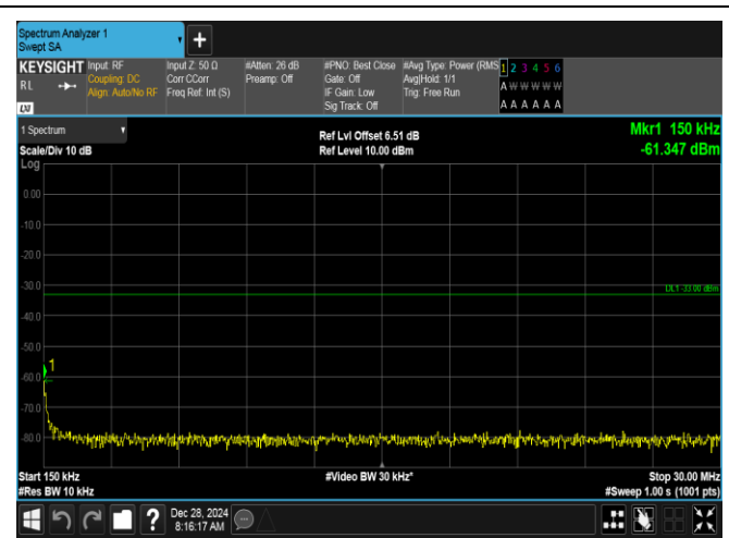
Band2-20MHz-QPSK-18700-1RB#0-0.15~30-PASS
