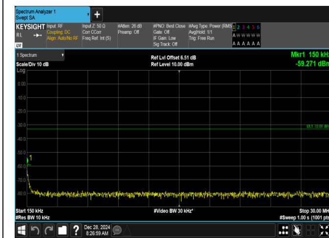
Band2-20MHz-QPSK-18900-100RB#0-0.15~30-PASS
