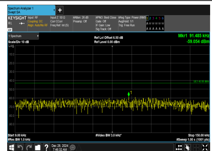
Band2-15MHz-16QAM-18900-1RB#74-0.009~0.15-PASS
