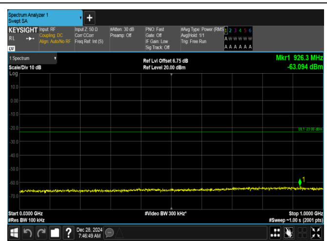
Band2-15MHz-16QAM-18900-1RB#74-30~1000-PASS
