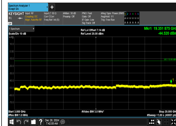
Band2-15MHz-QPSK-18675-75RB#0-3000~20000-PASS
