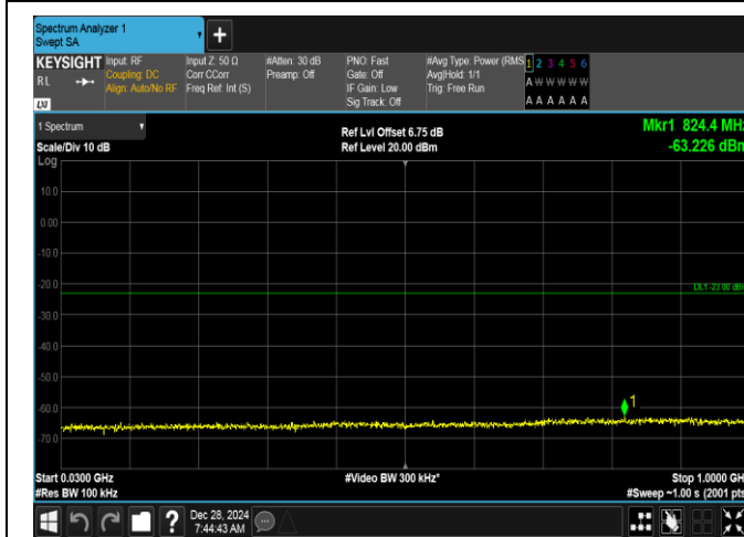
Band2-15MHz-16QAM-18900-1RB#0-30~1000-PASS
