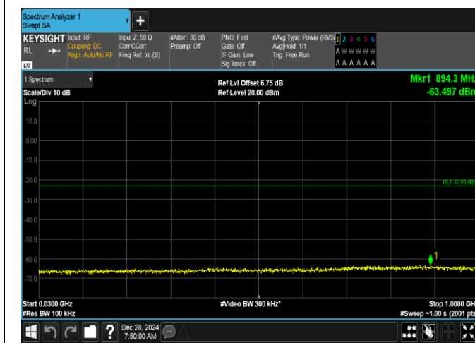
Band2-15MHz-QPSK-19125-1RB#0-30~1000-PASS
