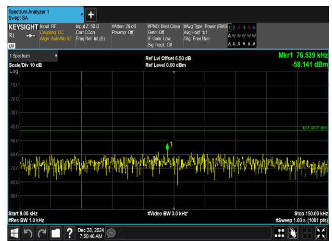
Band2-15MHz-16QAM-19125-1RB#0-0.009~0.15-PASS
