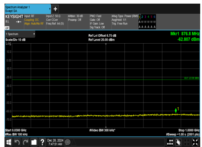
Band2-15MHz-QPSK-18900-75RB#0-30~1000-PASS
