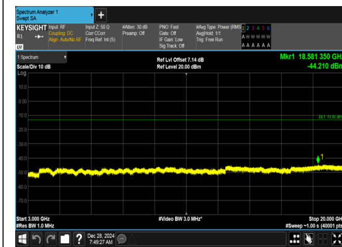
Band2-15MHz-16QAM-18900-75RB#0-3000~20000-PASS
