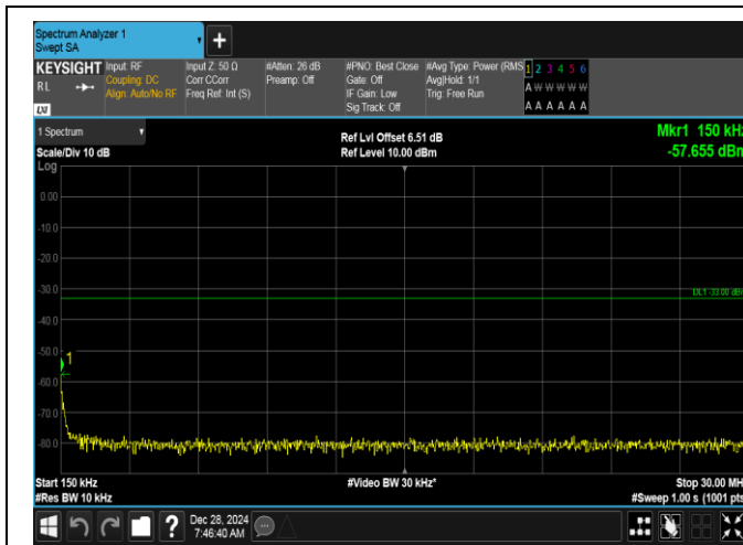
Band2-15MHz-16QAM-18900-1RB#74-0.15~30-PASS
