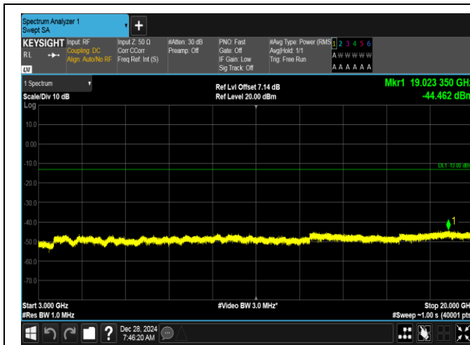
Band2-15MHz-QPSK-18900-1RB#74-3000~20000-PASS
