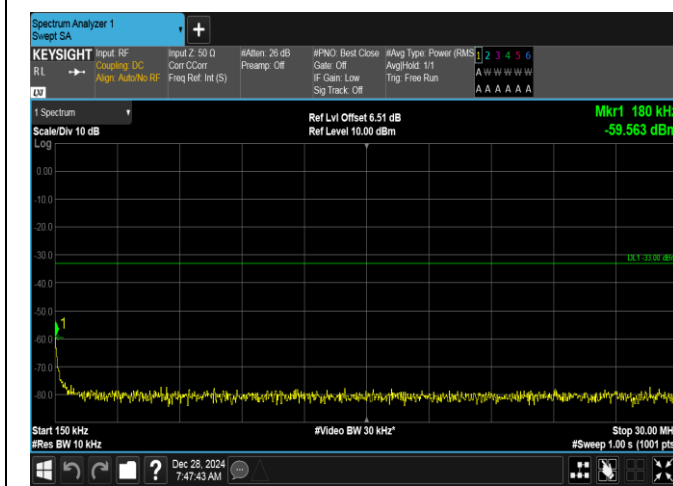
Band2-15MHz-QPSK-18900-75RB#0-0.15~30-PASS
