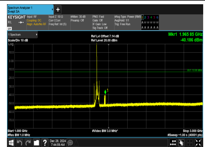
Band2-15MHz-16QAM-18900-1RB#0-1000~3000-PASS
