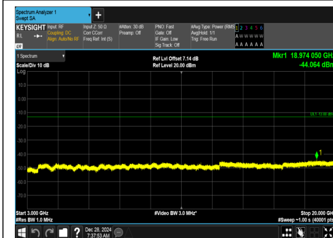
Band2-15MHz-QPSK-18675-1RB#0-3000~20000-PASS
