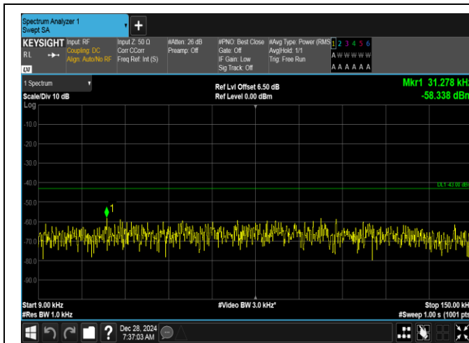
Band2-15MHz-QPSK-18675-1RB#0-0.009~0.15-PASS
