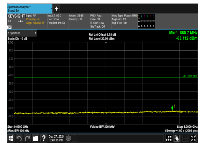
Band2-10MHz-16QAM-19150-50RB#0-30~1000-PASS
