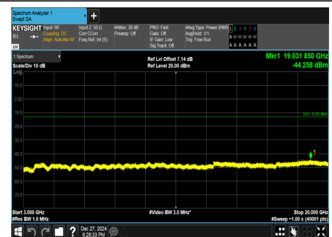
Band2-10MHz-16QAM-18650-50RB#0-3000~20000-PASS
