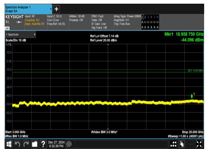
Band2-10MHz-16QAM-18900-1RB#49-3000~20000-PASS
