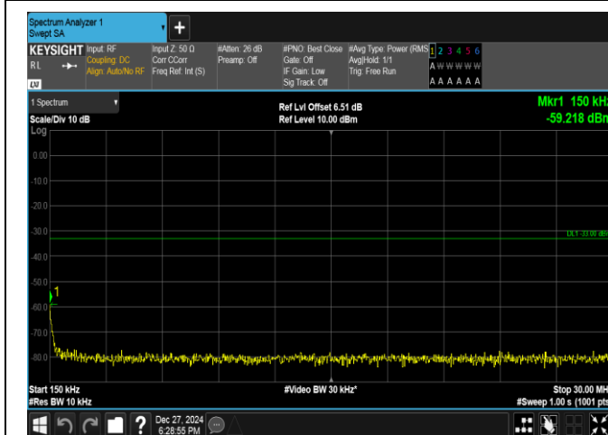
Band2-10MHz-QPSK-18900-1RB#0-0.15~30-PASS
