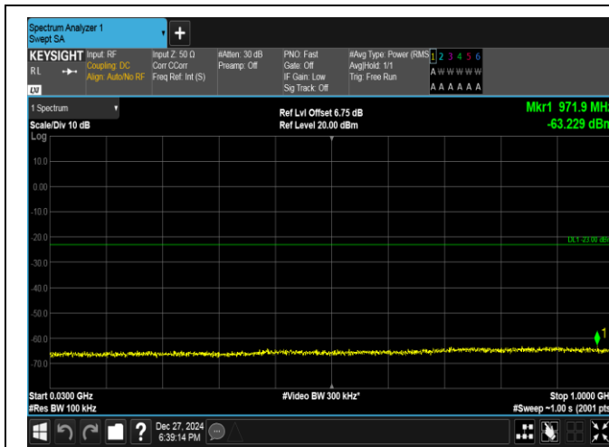
Band2-10MHz-QPSK-19150-50RB#0-30~1000-PASS
