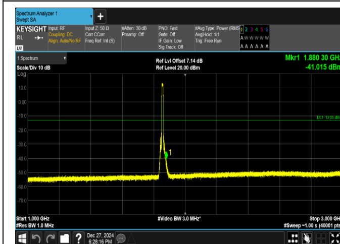
Band2-10MHz-16QAM-18650-50RB#0-1000~3000-PASS
