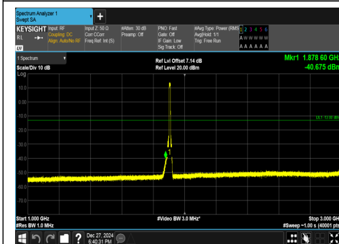
Band2-10MHz-16QAM-19150-50RB#0-1000~3000-PASS
