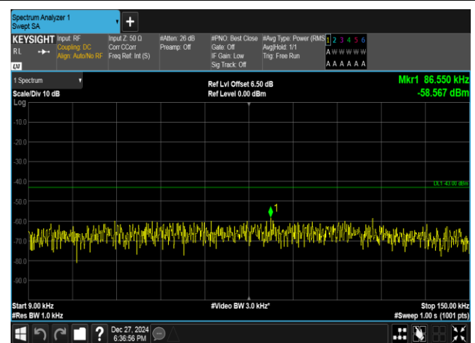
Band2-10MHz-QPSK-19150-1RB#49-0.009~0.15-PASS
