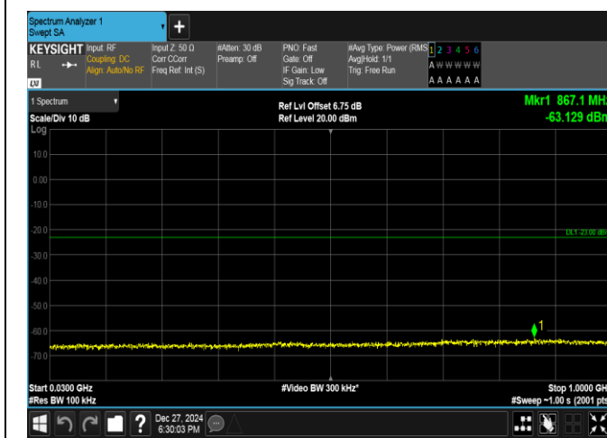
Band2-10MHz-16QAM-18900-1RB#0-30~1000-PASS
