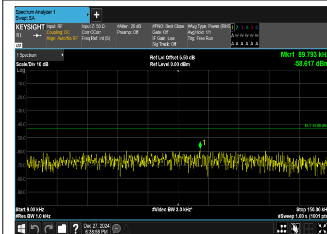
Band2-10MHz-QPSK-19150-50RB#0-0.009~0.15-PASS
