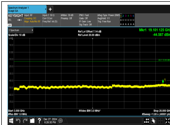
Band2-10MHz-16QAM-18650-1RB#49-3000~20000-PASS
