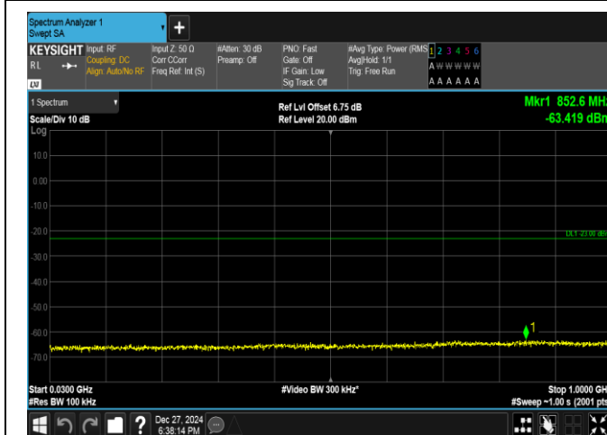
Band2-10MHz-16QAM-19150-1RB#49-30~1000-PASS
