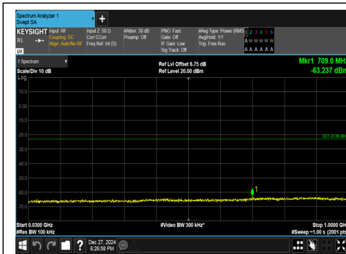
Band2-10MHz-QPSK-18650-50RB#0-30~1000-PASS
