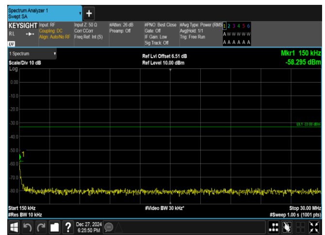
Band2-10MHz-16QAM-18650-1RB#49-0.15~30-PASS
