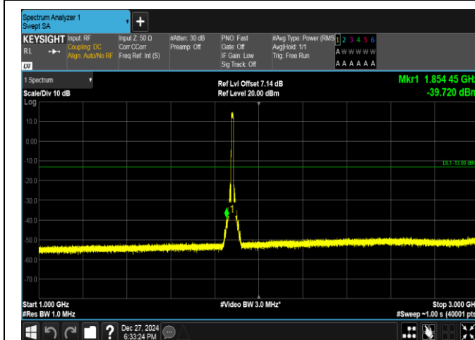
Band2-10MHz-QPSK-18900-50RB#0-1000~3000-PASS
