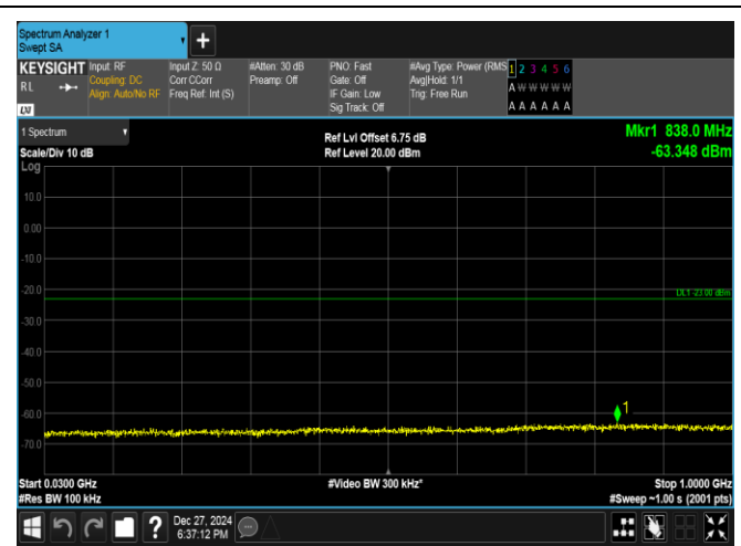
Band2-10MHz-QPSK-19150-1RB#49-30~1000-PASS
