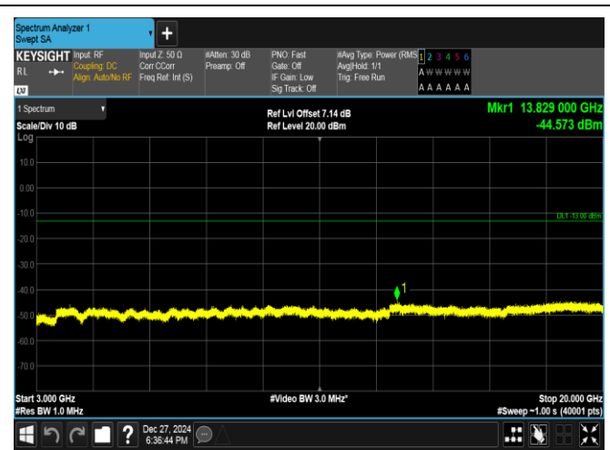
Band2-10MHz-16QAM-19150-1RB#0-3000~20000-PASS
