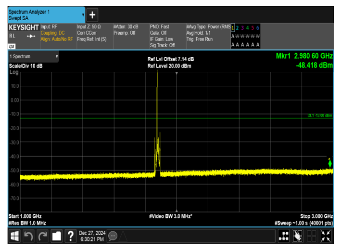
Band2-10MHz-16QAM-18900-1RB#0-1000~3000-PASS
