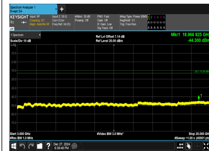
Band2-10MHz-QPSK-19150-50RB#0-3000~20000-PASS
