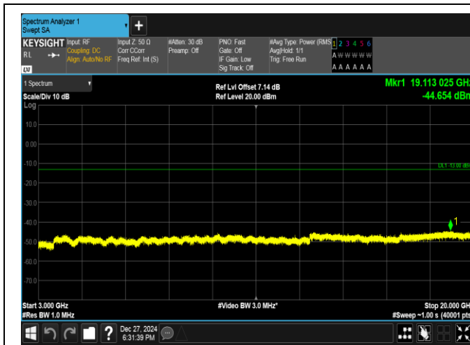
Band2-10MHz-QPSK-18900-1RB#49-3000~20000-PASS
