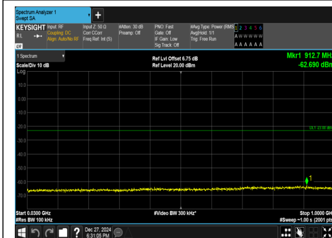
Band2-10MHz-QPSK-18900-1RB#49-30~1000-PASS
