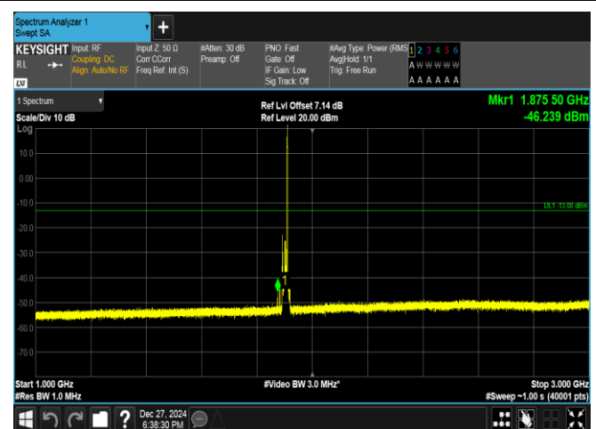
Band2-10MHz-16QAM-19150-1RB#49-1000~3000-PASS
