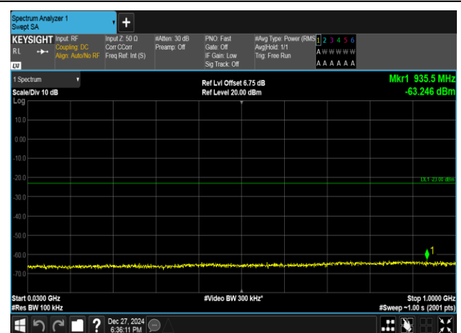
Band2-10MHz-16QAM-19150-1RB#0-30~1000-PASS
