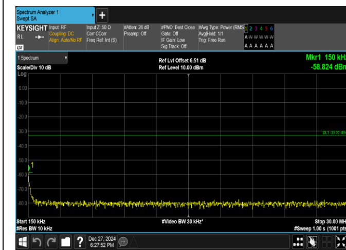
Band2-10MHz-16QAM-18650-50RB#0-0.15~30-PASS
