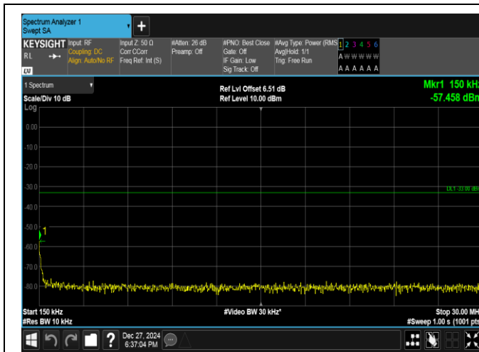
Band2-10MHz-QPSK-19150-1RB#49-0.15~30-PASS
