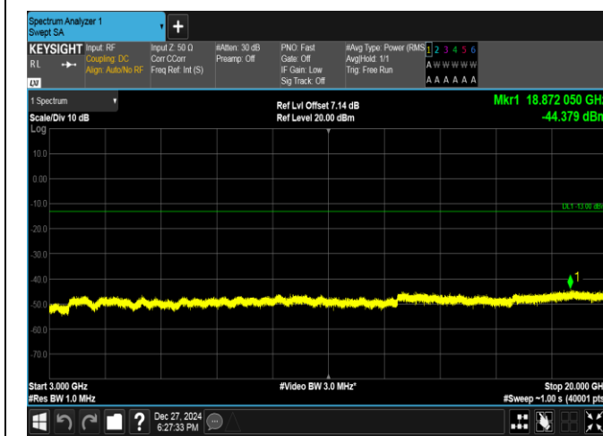
Band2-10MHz-QPSK-18650-50RB#0-3000~20000-PASS
