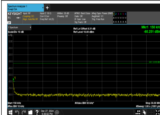
Band2-10MHz-16QAM-19150-1RB#0-0.15~30-PASS
