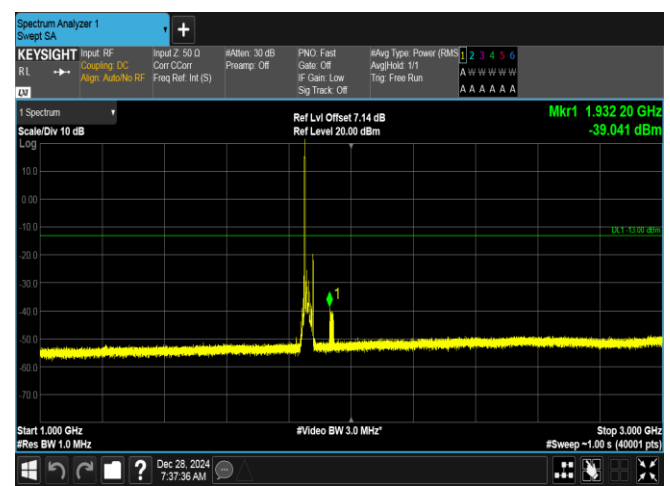
Band2-15MHz-QPSK-18675-1RB#0-1000~3000-PASS
