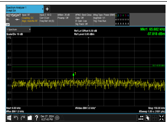
Band2-10MHz-16QAM-18650-50RB#0-0.009~0.15-PASS
