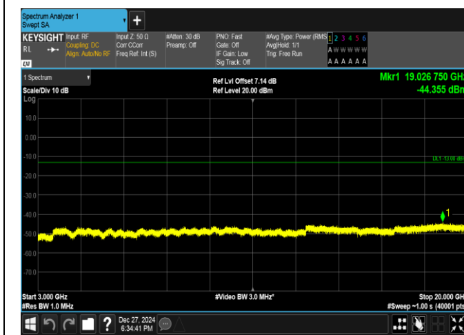
Band2-10MHz-16QAM-18900-50RB#0-3000~20000-PASS
