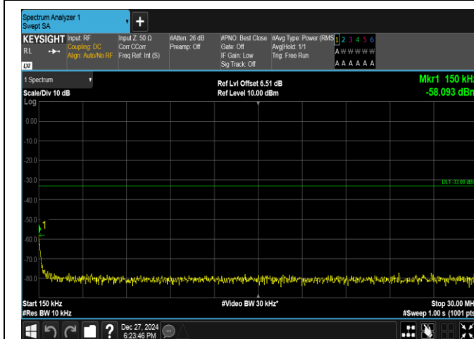
Band2-10MHz-16QAM-18650-1RB#0-0.15~30-PASS
