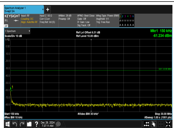
Band2-15MHz-QPSK-18675-1RB#0-0.15~30-PASS
