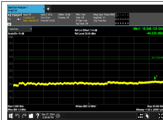
Band2-10MHz-16QAM-19150-1RB#49-3000~20000-PASS
