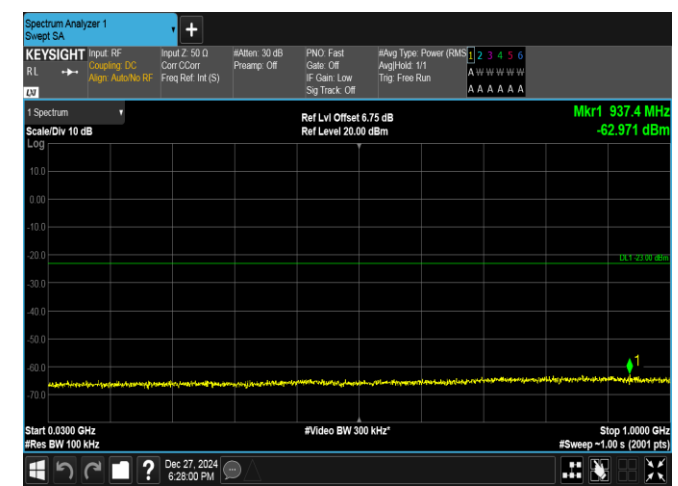
Band2-10MHz-16QAM-18650-50RB#0-30~1000-PASS
