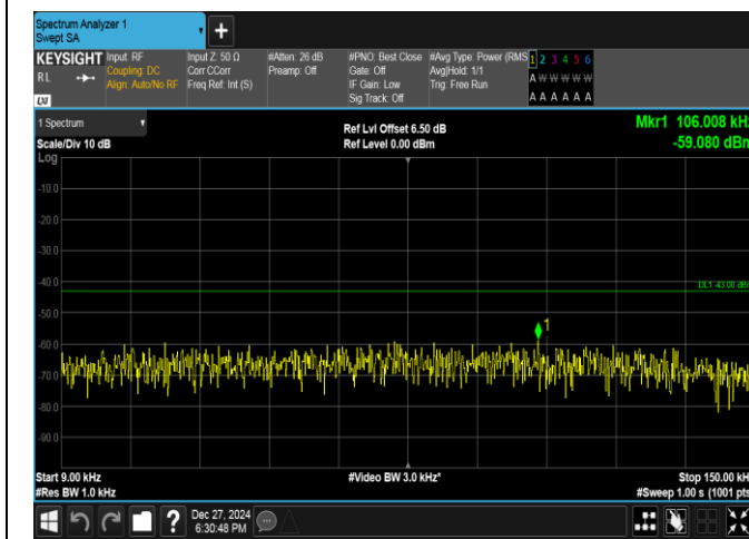
Band2-10MHz-QPSK-18900-1RB#49-0.009~0.15-PASS
