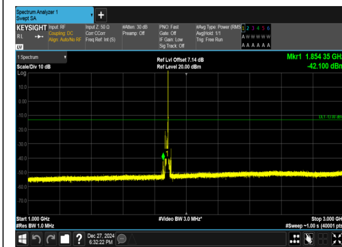
Band2-10MHz-16QAM-18900-1RB#49-1000~3000-PASS
