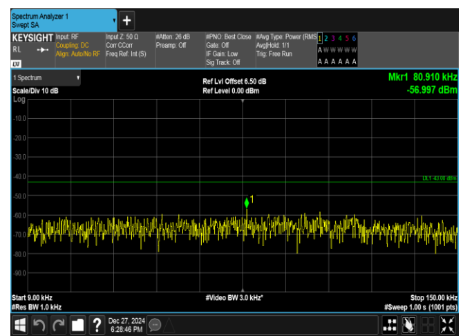
Band2-10MHz-QPSK-18900-1RB#0-0.009~0.15-PASS
