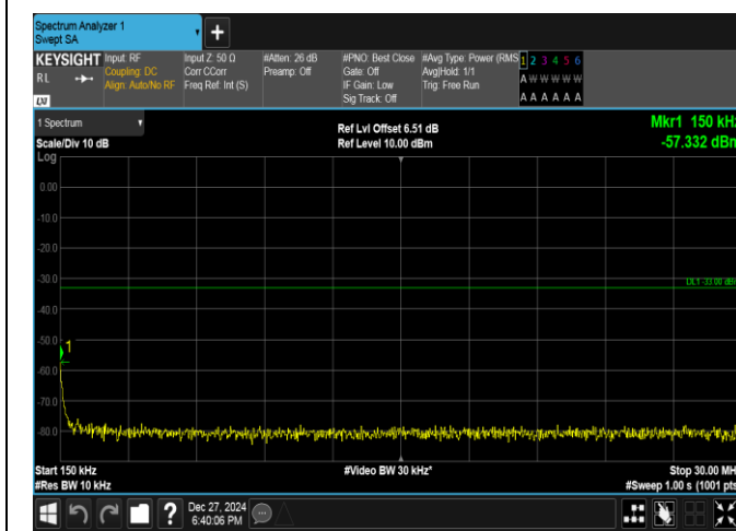
Band2-10MHz-16QAM-19150-50RB#0-0.15~30-PASS
