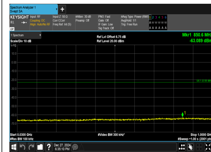
Band2-10MHz-QPSK-19150-1RB#0-30~1000-PASS
