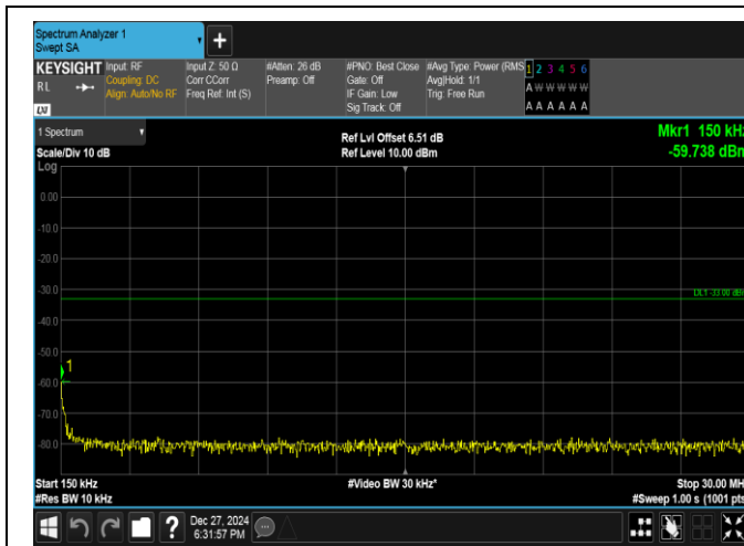
Band2-10MHz-16QAM-18900-1RB#49-0.15~30-PASS
