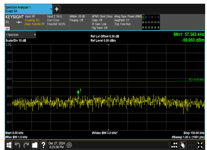
Band2-10MHz-16QAM-18650-1RB#0-0.009~0.15-PASS
