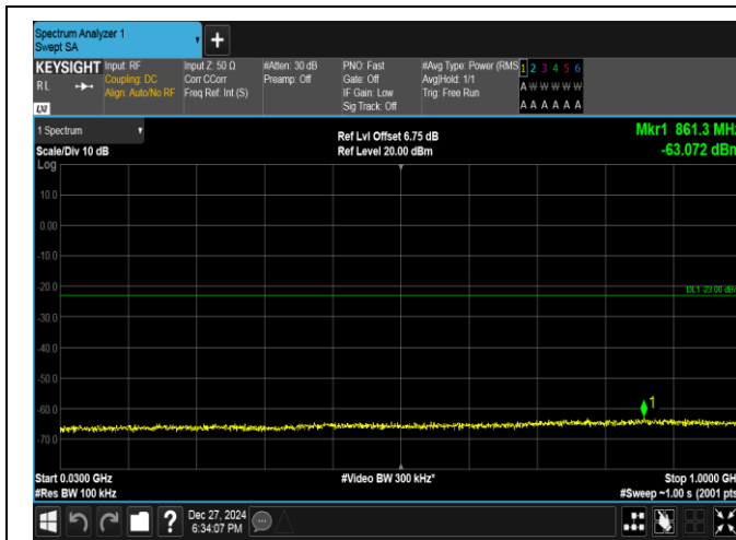
Band2-10MHz-16QAM-18900-50RB#0-30~1000-PASS
