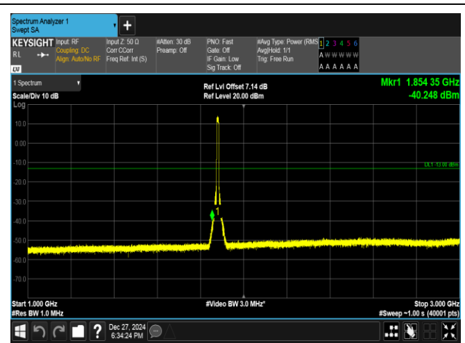
Band2-10MHz-16QAM-18900-50RB#0-1000~3000-PASS
