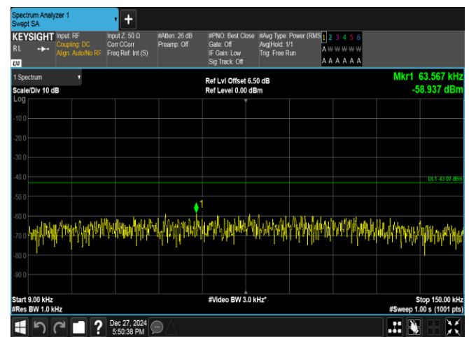
Band2-5MHz-16QAM-19175-1RB#0-0.009~0.15-PASS
