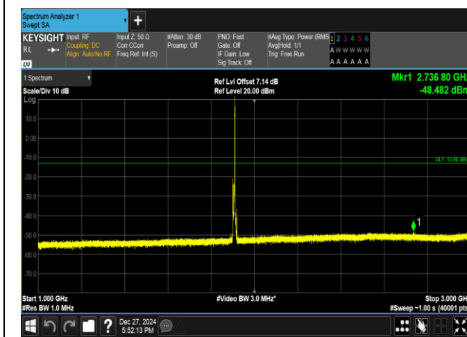
Band2-5MHz-QPSK-19175-1RB#24-1000~3000-PASS
