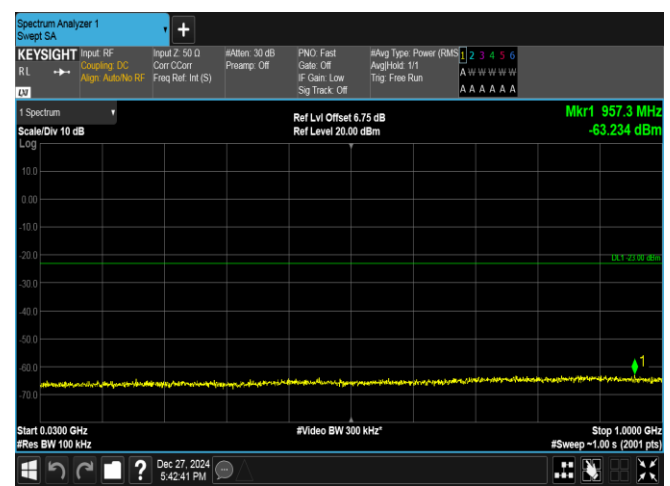
Band2-5MHz-16QAM-18625-25RB#0-30~1000-PASS
