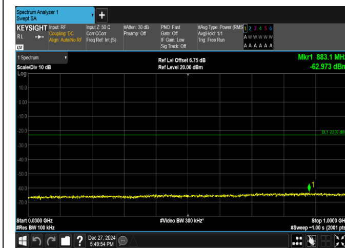
Band2-5MHz-QPSK-19175-1RB#0-30~1000-PASS
