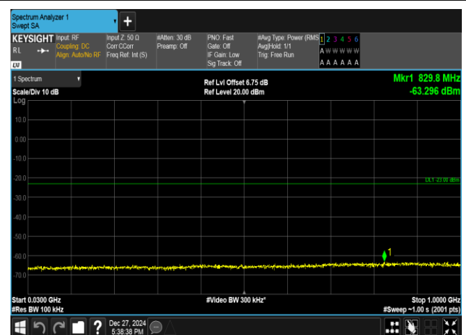
Band2-5MHz-16QAM-18625-1RB#0-30~1000-PASS
