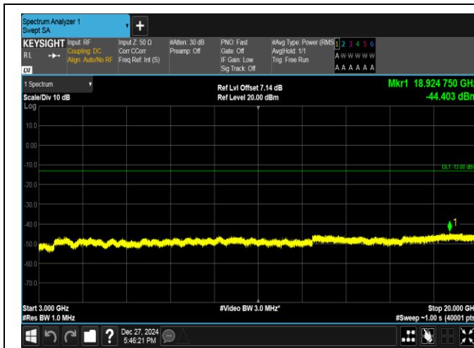
Band2-5MHz-QPSK-18900-1RB#24-3000~20000-PASS
