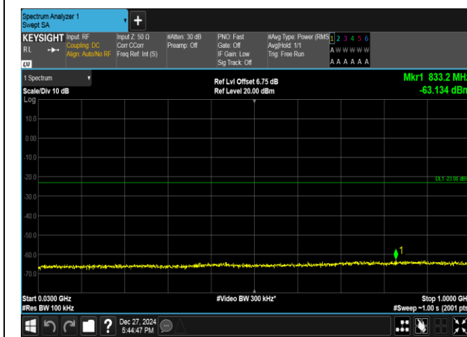
Band2-5MHz-16QAM-18900-1RB#0-30~1000-PASS
