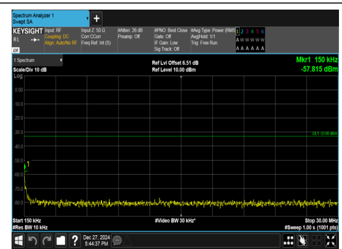
Band2-5MHz-16QAM-18900-1RB#0-0.15~30-PASS
