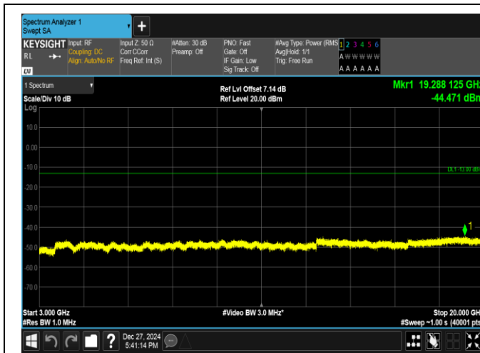
Band2-5MHz-16QAM-18625-1RB#24-3000~20000-PASS
