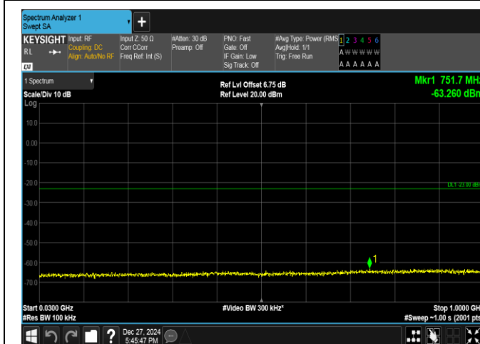
Band2-5MHz-QPSK-18900-1RB#24-30~1000-PASS
