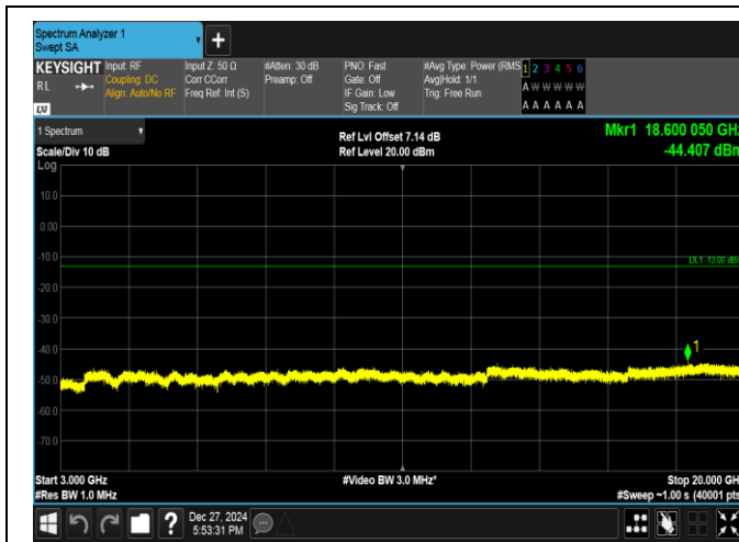
Band2-5MHz-16QAM-19175-1RB#24-3000~20000-PASS
