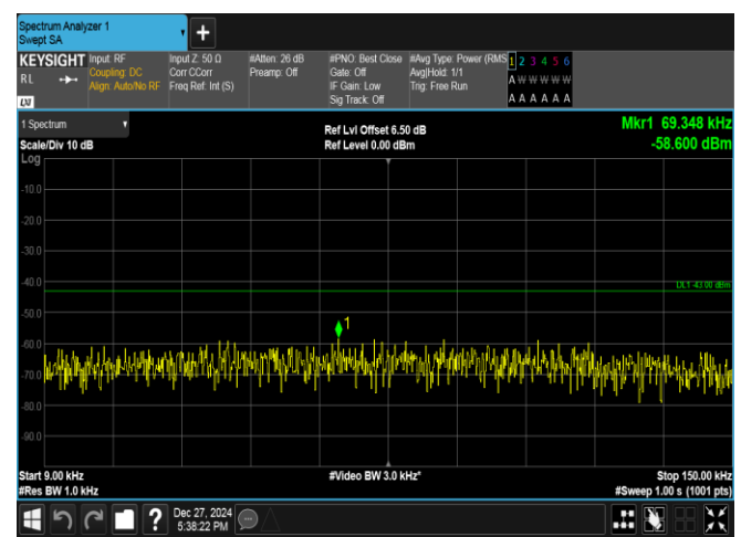
Band2-5MHz-16QAM-18625-1RB#0-0.009~0.15-PASS
