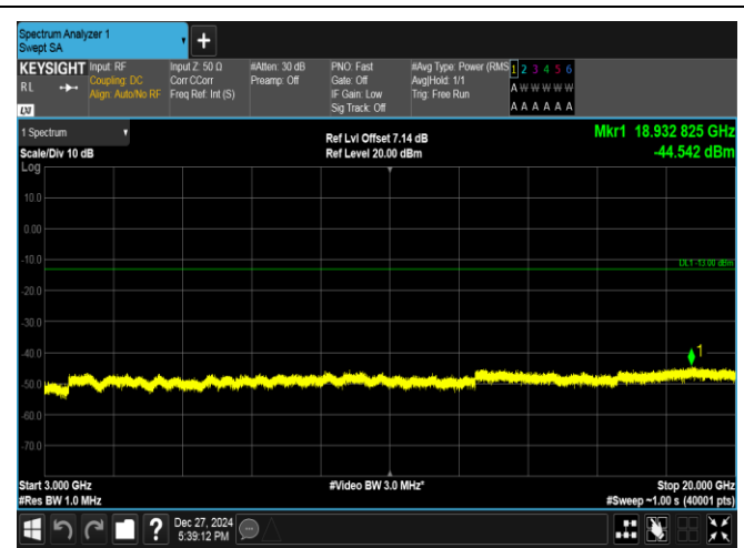
Band2-5MHz-16QAM-18625-1RB#0-3000~20000-PASS
