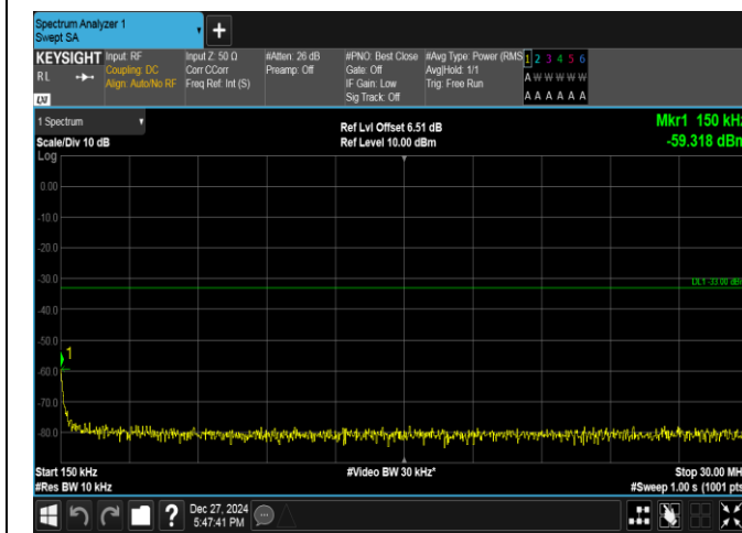
Band2-5MHz-QPSK-18900-25RB#0-0.15~30-PASS
