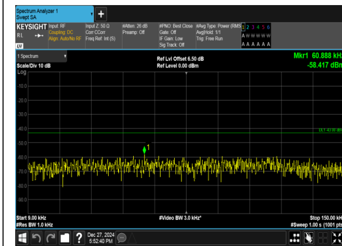
Band2-5MHz-16QAM-19175-1RB#24-0.009~0.15-PASS
