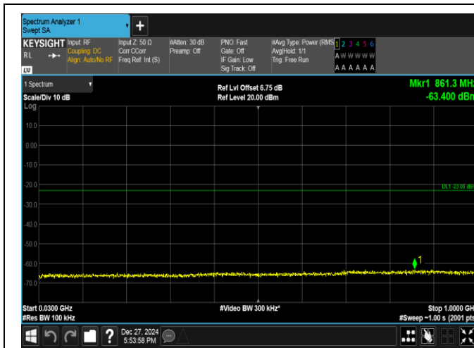
Band2-5MHz-QPSK-19175-25RB#0-30~1000-PASS
