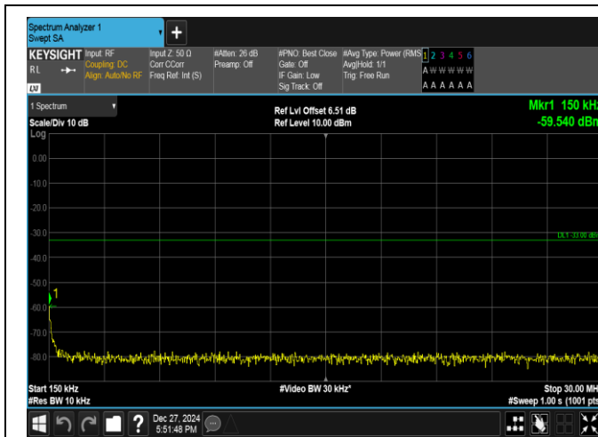
Band2-5MHz-QPSK-19175-1RB#24-0.15~30-PASS
