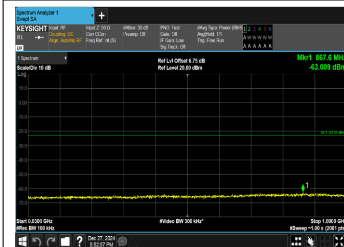
Band2-5MHz-16QAM-19175-1RB#24-30~1000-PASS
