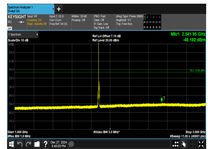
Band2-5MHz-16QAM-18900-1RB#0-1000~3000-PASS
