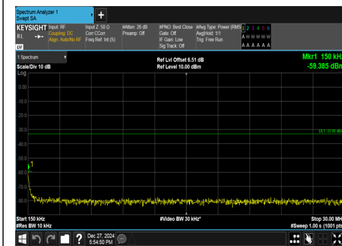
Band2-5MHz-16QAM-19175-25RB#0-0.15~30-PASS
