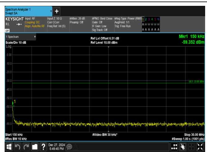
Band2-5MHz-QPSK-19175-1RB#0-0.15~30-PASS
