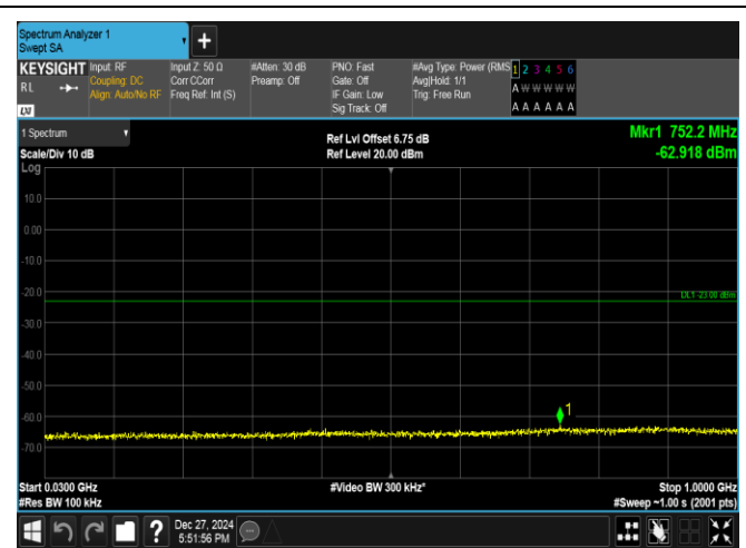
Band2-5MHz-QPSK-19175-1RB#24-30~1000-PASS
