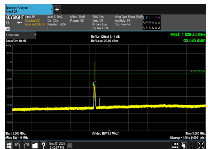
Band2-5MHz-16QAM-18625-1RB#24-1000~3000-PASS
