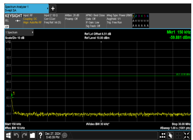
Band2-5MHz-QPSK-18900-1RB#24-0.15~30-PASS
