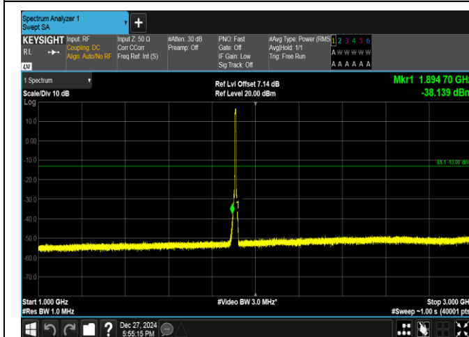
Band2-5MHz-16QAM-19175-25RB#0-1000~3000-PASS
