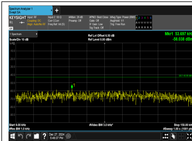
Band2-5MHz-QPSK-19175-1RB#0-0.009~0.15-PASS
