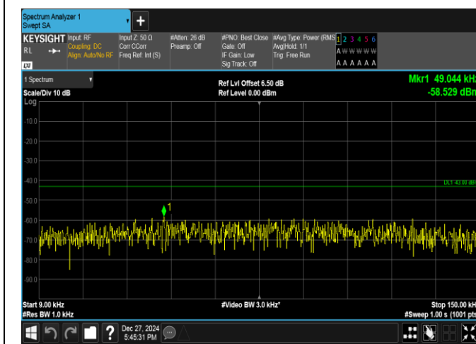
Band2-5MHz-QPSK-18900-1RB#24-0.009~0.15-PASS
