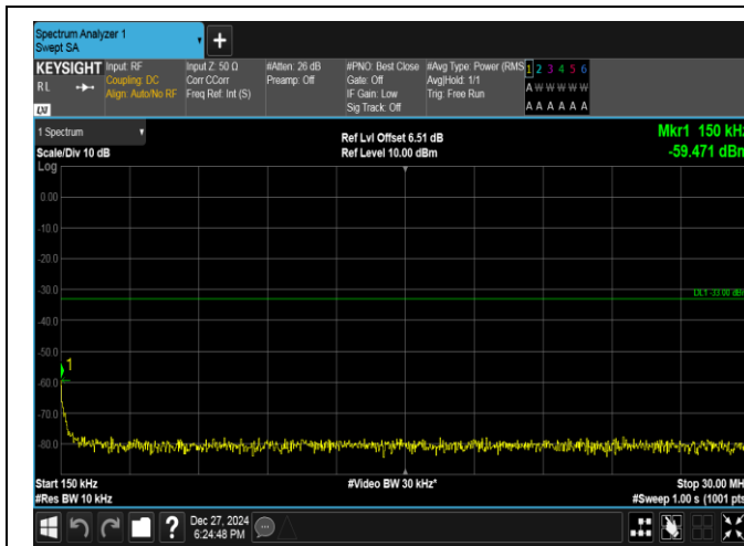
Band2-10MHz-QPSK-18650-1RB#49-0.15~30-PASS
