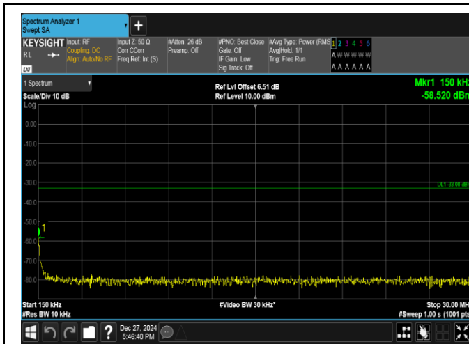
Band2-5MHz-16QAM-18900-1RB#24-0.15~30-PASS
