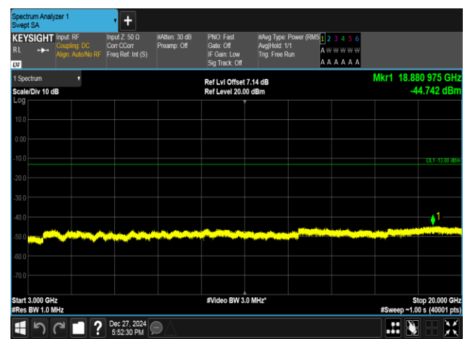
Band2-5MHz-QPSK-19175-1RB#24-3000~20000-PASS
