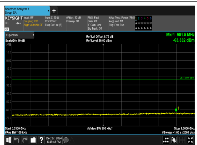
Band2-5MHz-16QAM-18900-1RB#24-30~1000-PASS
