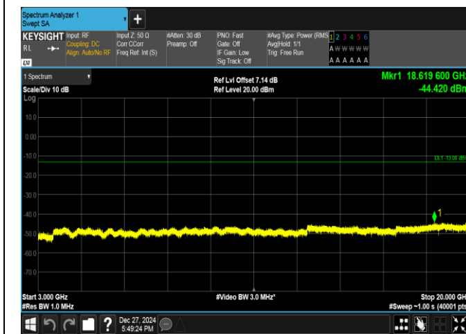
Band2-5MHz-16QAM-18900-25RB#0-3000~20000-PASS
