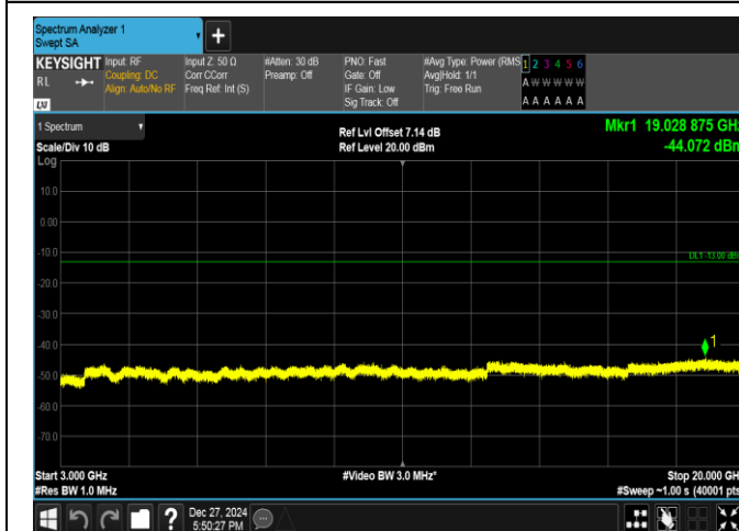
Band2-5MHz-QPSK-19175-1RB#0-3000~20000-PASS
