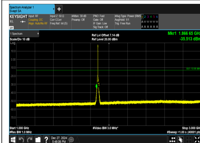
Band2-5MHz-QPSK-18900-25RB#0-1000~3000-PASS
