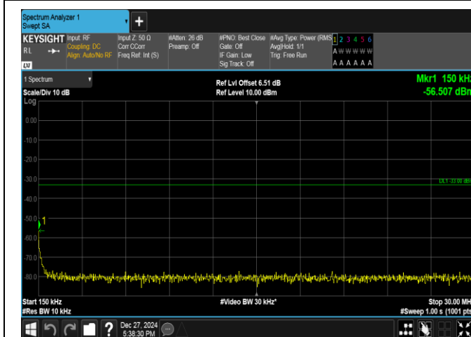
Band2-5MHz-16QAM-18625-1RB#0-0.15~30-PASS
