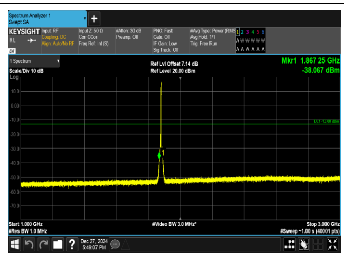
Band2-5MHz-16QAM-18900-25RB#0-1000~3000-PASS
