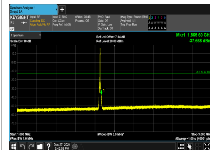
Band2-5MHz-16QAM-18625-25RB#0-1000~3000-PASS
