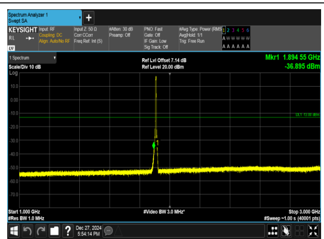
Band2-5MHz-QPSK-19175-25RB#0-1000~3000-PASS
