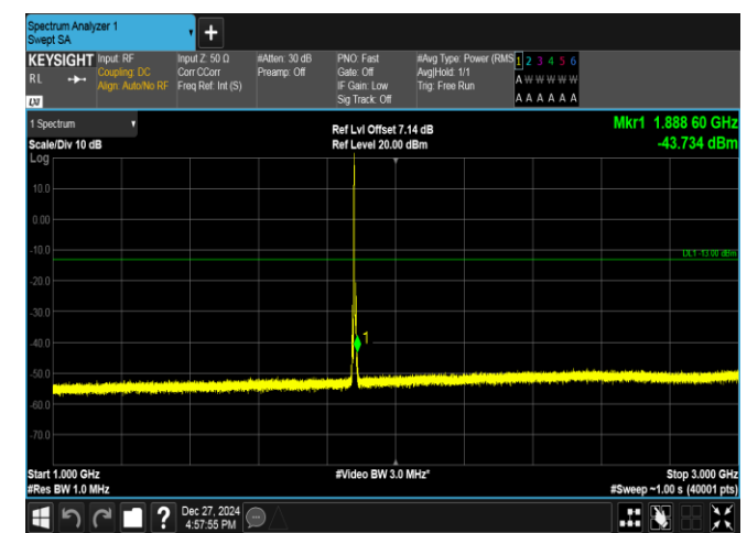
Band2-3MHz-16QAM-18900-1RB#0-1000~3000-PASS
