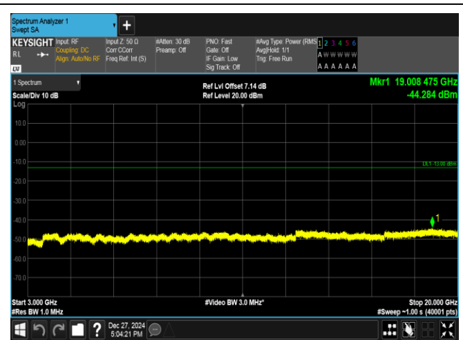
Band2-3MHz-16QAM-19185-1RB#0-3000~20000-PASS
