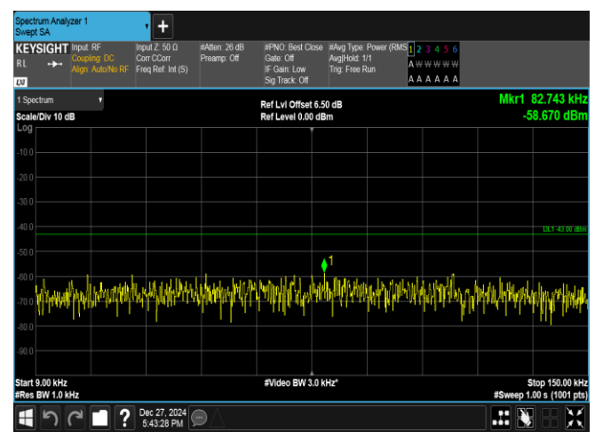
Band2-5MHz-QPSK-18900-1RB#0-0.009~0.15-PASS
