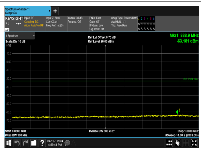
Band2-3MHz-16QAM-18900-1RB#14-30~1000-PASS
