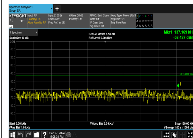
Band2-3MHz-QPSK-19185-15RB#0-0.009~0.15-PASS
