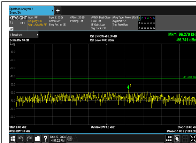
Band2-3MHz-16QAM-18900-1RB#0-0.009~0.15-PASS
