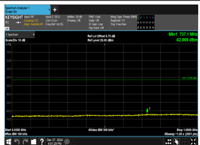
Band2-3MHz-16QAM-18615-1RB#0-30~1000-PASS
