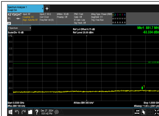
Band2-3MHz-16QAM-18900-15RB#0-30~1000-PASS
