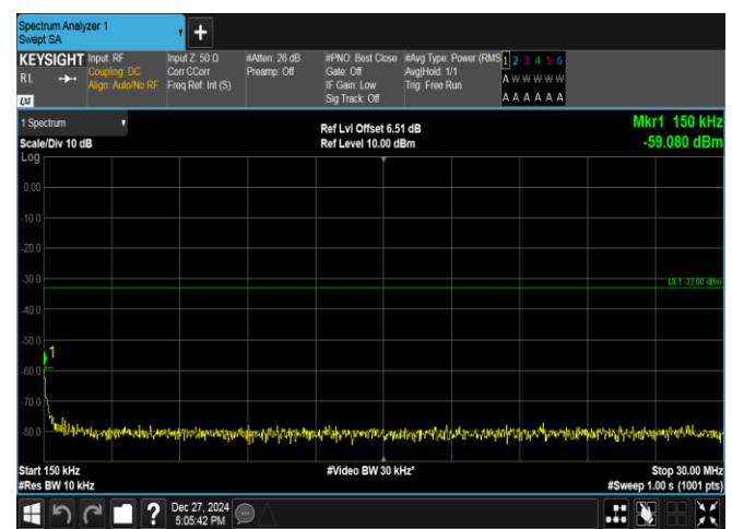
Band2-3MHz-16QAM-19185-1RB#14-0.15~30-PASS
