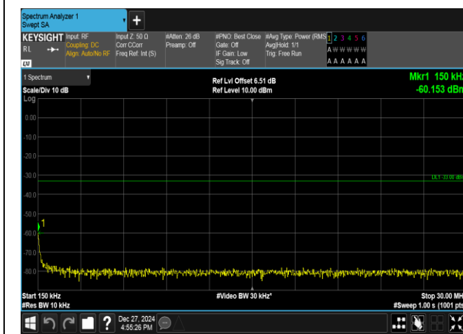
Band2-3MHz-16QAM-18615-15RB#0-0.15~30-PASS
