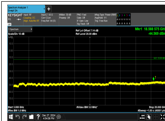
Band2-3MHz-16QAM-18615-1RB#14-3000~20000-PASS
