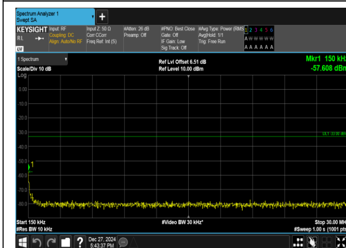
Band2-5MHz-QPSK-18900-1RB#0-0.15~30-PASS
