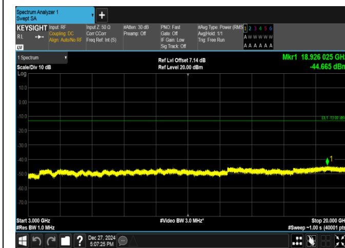
Band2-3MHz-QPSK-19185-15RB#0-3000~20000-PASS
