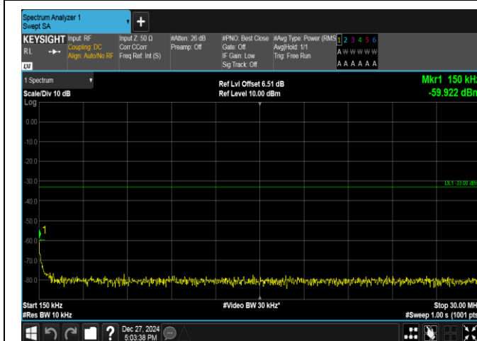
Band2-3MHz-16QAM-19185-1RB#0-0.15~30-PASS
