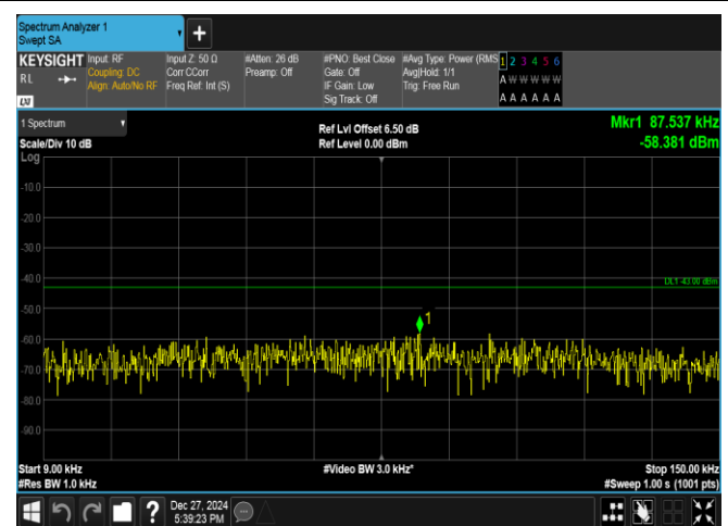
Band2-5MHz-QPSK-18625-1RB#24-0.009~0.15-PASS
