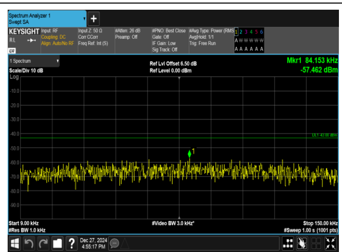
Band2-3MHz-16QAM-18615-15RB#0-0.009~0.15-PASS
