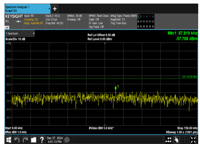
Band2-3MHz-16QAM-18615-1RB#0-0.009~0.15-PASS
