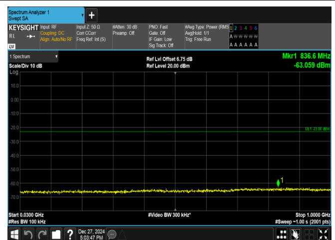
Band2-3MHz-16QAM-19185-1RB#0-30~1000-PASS
