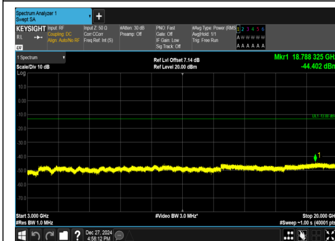
Band2-3MHz-16QAM-18900-1RB#0-3000~20000-PASS
