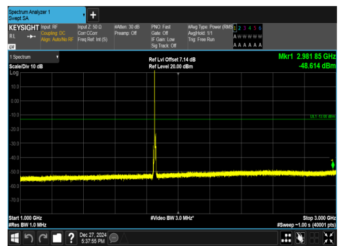
Band2-5MHz-QPSK-18625-1RB#0-1000~3000-PASS
