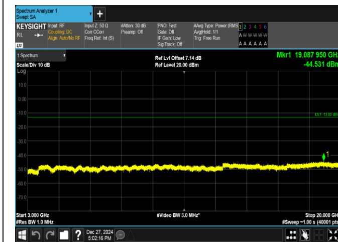
Band2-3MHz-16QAM-18900-15RB#0-3000~20000-PASS
