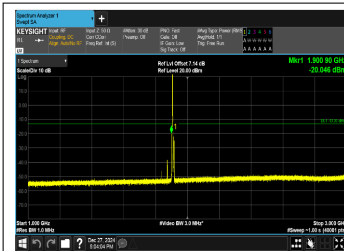
Band2-3MHz-16QAM-19185-1RB#0-1000~3000-PASS
