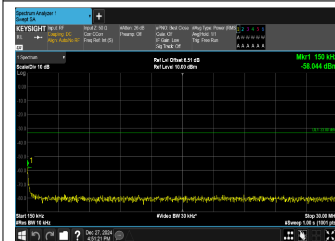
Band2-3MHz-16QAM-18615-1RB#0-0.15~30-PASS
