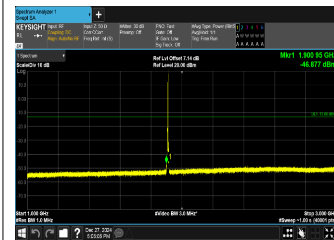
Band2-3MHz-QPSK-19185-1RB#14-1000~3000-PASS
