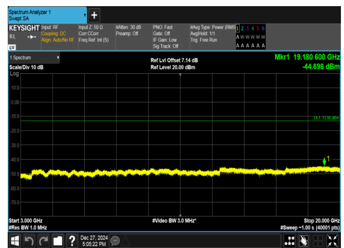
Band2-3MHz-QPSK-19185-1RB#14-3000~20000-PASS
