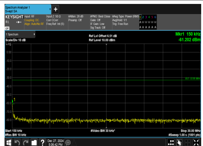
Band2-3MHz-QPSK-19185-15RB#0-0.15~30-PASS
