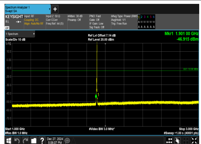
Band2-3MHz-16QAM-19185-1RB#14-1000~3000-PASS
