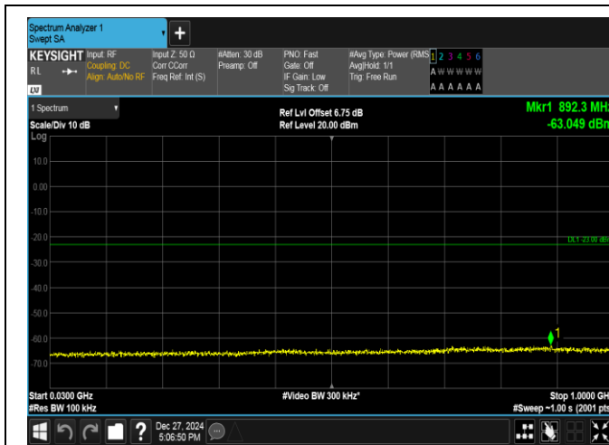
Band2-3MHz-QPSK-19185-15RB#0-30~1000-PASS
