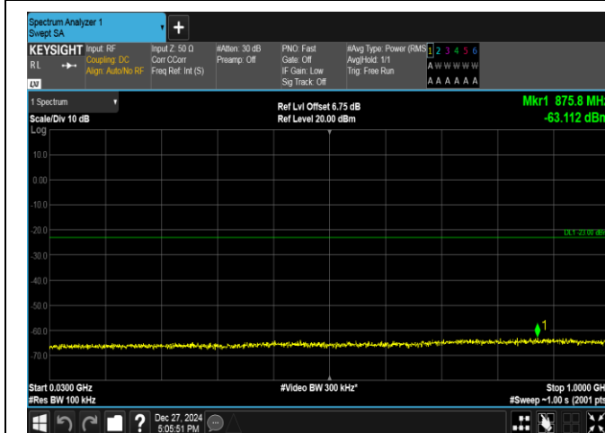
Band2-3MHz-16QAM-19185-1RB#14-30~1000-PASS
