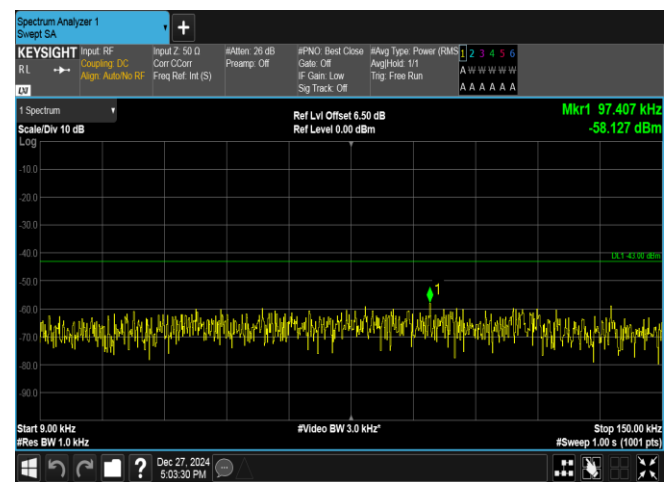
Band2-3MHz-16QAM-19185-1RB#0-0.009~0.15-PASS
