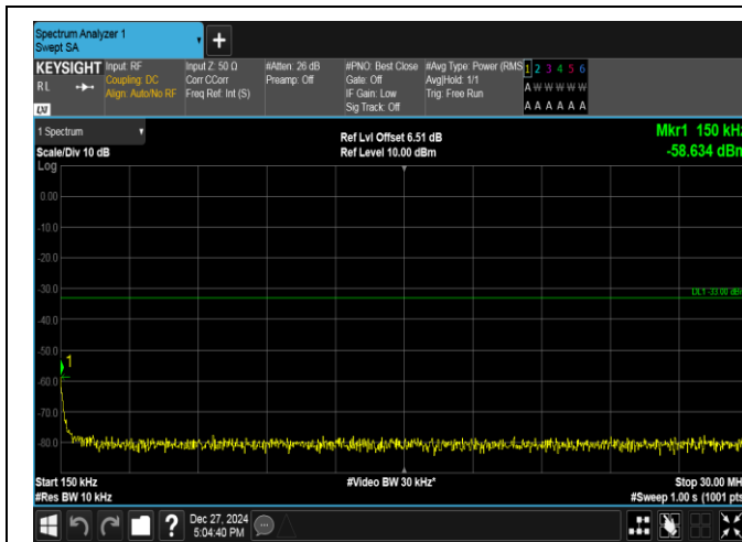
Band2-3MHz-QPSK-19185-1RB#14-0.15~30-PASS
