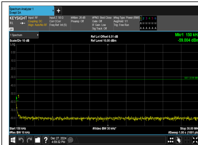
Band2-3MHz-16QAM-18900-1RB#14-0.15~30-PASS
