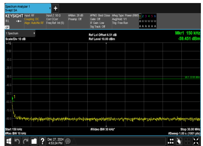
Band2-3MHz-16QAM-18615-1RB#14-0.15~30-PASS
