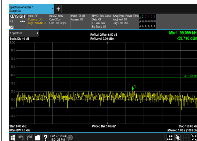
Band2-3MHz-16QAM-18900-15RB#0-0.009~0.15-PASS
