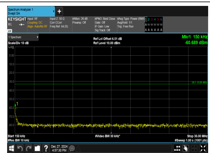
Band2-3MHz-16QAM-18900-1RB#0-0.15~30-PASS
