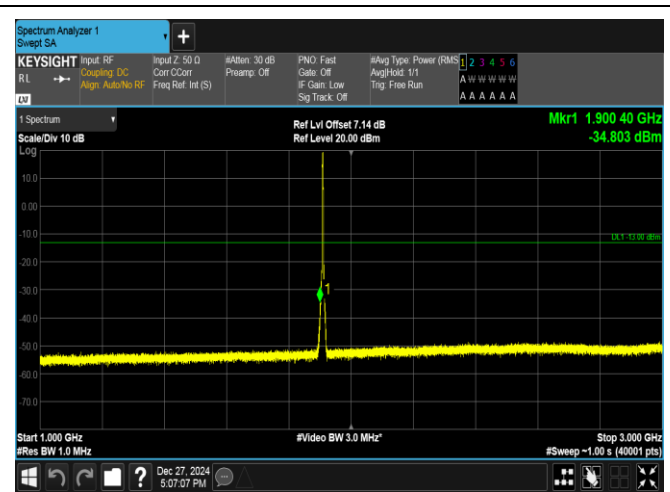
Band2-3MHz-QPSK-19185-15RB#0-1000~3000-PASS
