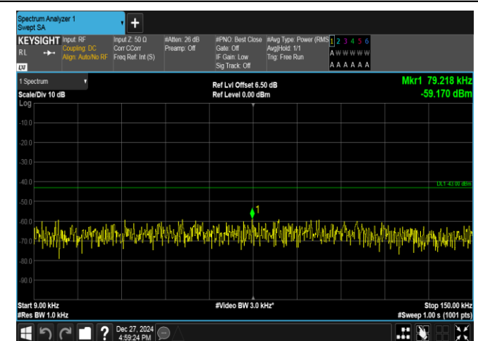
Band2-3MHz-16QAM-18900-1RB#14-0.009~0.15-PASS
