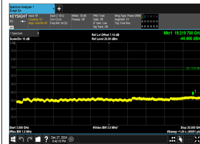
Band2-5MHz-QPSK-18625-25RB#0-3000~20000-PASS
