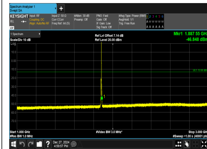
Band2-3MHz-16QAM-18900-1RB#14-1000~3000-PASS
