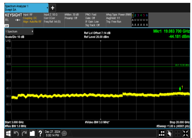
Band2-3MHz-16QAM-18900-1RB#14-3000~20000-PASS
