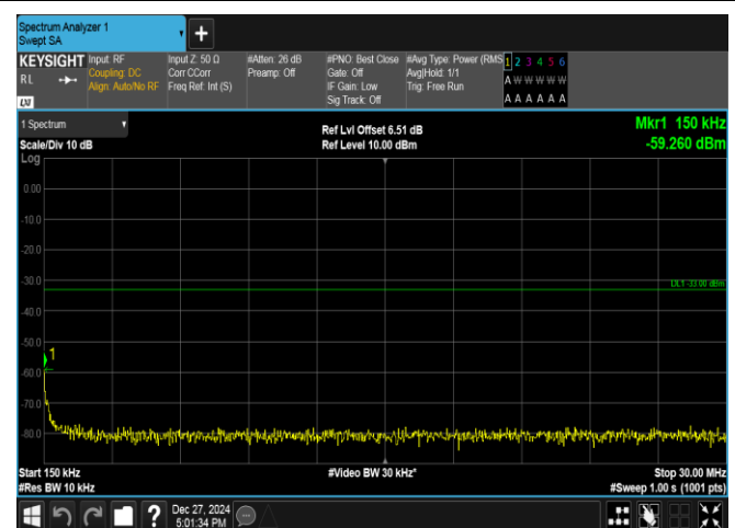
Band2-3MHz-16QAM-18900-15RB#0-0.15~30-PASS
