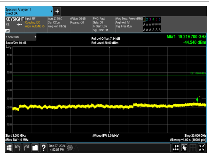
Band2-3MHz-16QAM-18615-1RB#0-3000~20000-PASS
