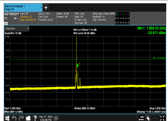
Band2-3MHz-16QAM-18615-1RB#14-1000~3000-PASS
