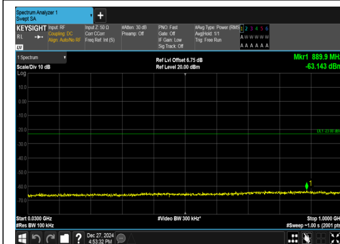
Band2-3MHz-16QAM-18615-1RB#14-30~1000-PASS
