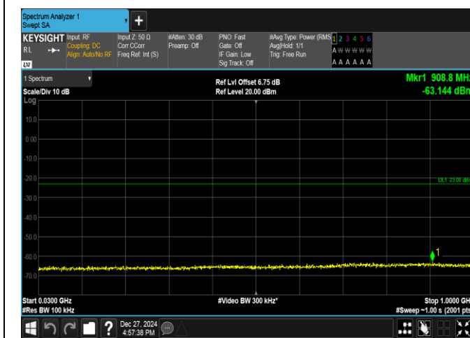
Band2-3MHz-16QAM-18900-1RB#0-30~1000-PASS
