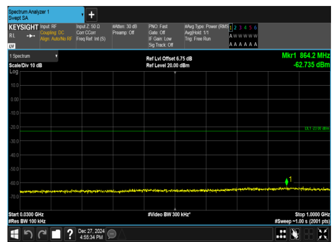
Band2-3MHz-16QAM-18615-15RB#0-30~1000-PASS
