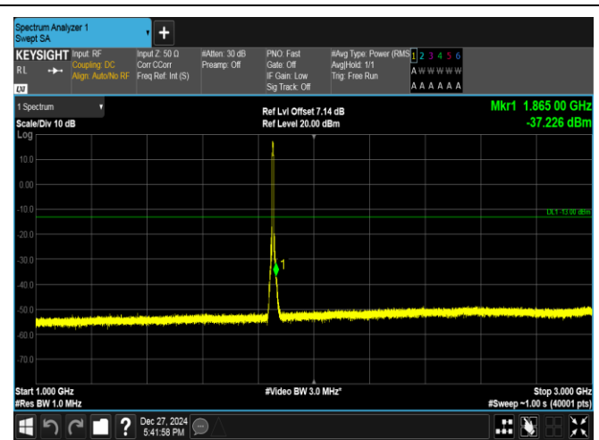
Band2-5MHz-QPSK-18625-25RB#0-1000~3000-PASS
