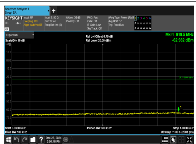
Band2-3MHz-QPSK-19185-1RB#14-30~1000-PASS
