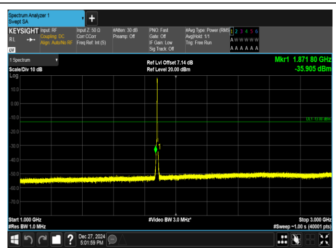
Band2-3MHz-16QAM-18900-15RB#0-1000~3000-PASS
