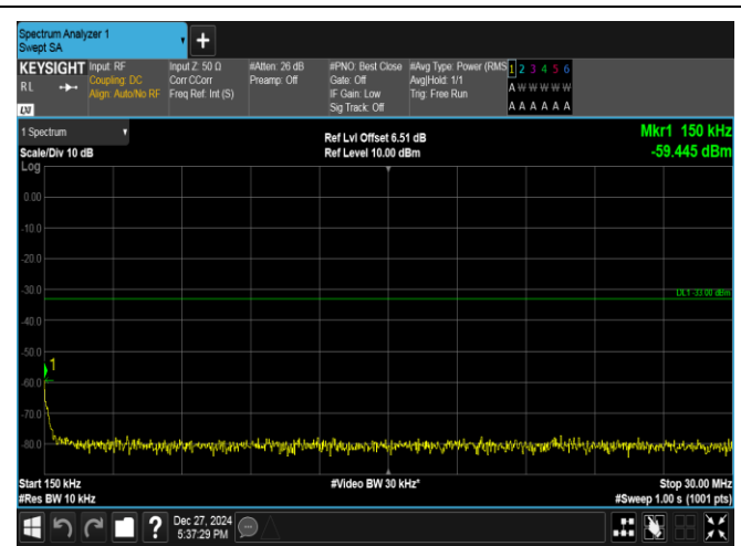
Band2-5MHz-QPSK-18625-1RB#0-0.15~30-PASS
