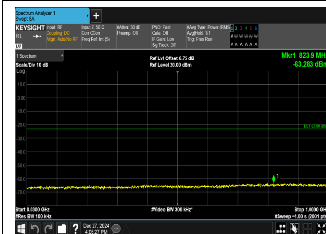
Band2-1.4MHz-16QAM-18607-1RB#5-30~1000-PASS
