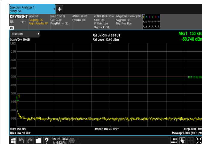
Band2-1.4MHz-16QAM-19193-1RB#0-0.15~30-PASS
