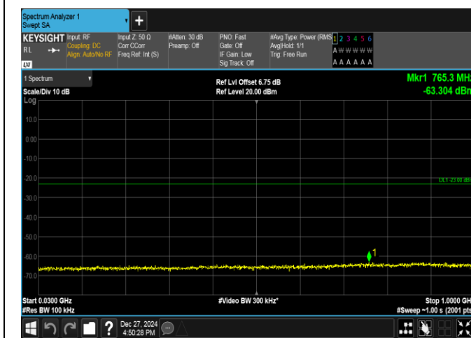
Band2-3MHz-QPSK-18615-1RB#0-30~1000-PASS
