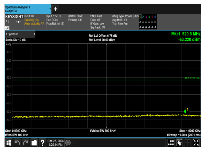
Band2-1.4MHz-16QAM-19193-6RB#0-30~1000-PASS
