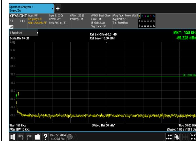
Band2-1.4MHz-16QAM-19193-6RB#0-0.15~30-PASS
