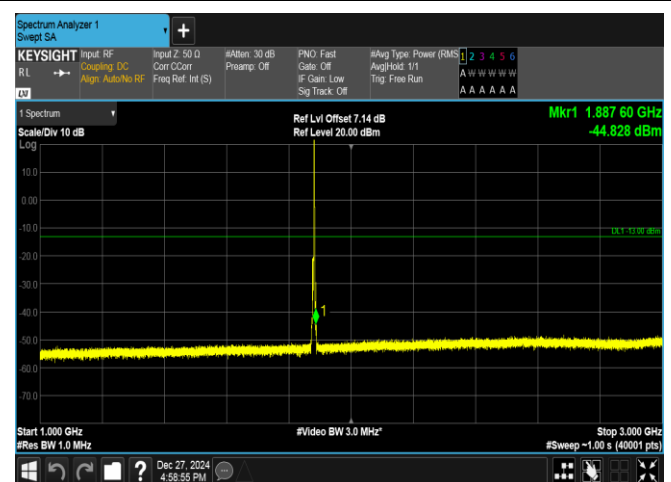
Band2-3MHz-QPSK-18900-1RB#14-1000~3000-PASS
