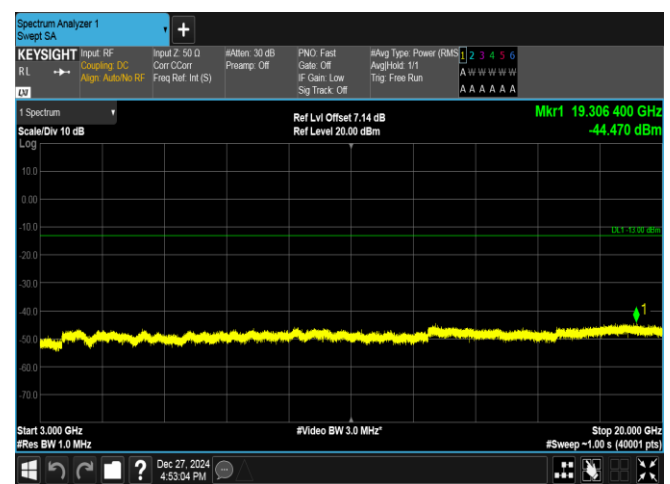
Band2-3MHz-QPSK-18615-1RB#14-3000~20000-PASS
