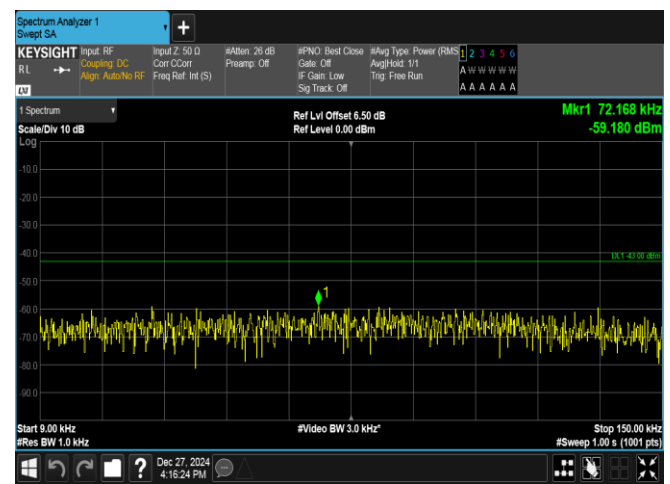
Band2-1.4MHz-16QAM-19193-1RB#0-0.009~0.15-PASS
