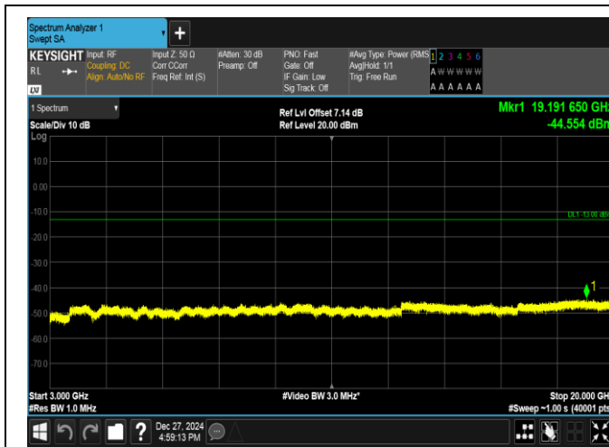
Band2-3MHz-QPSK-18900-1RB#14-3000~20000-PASS
