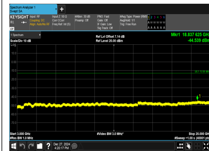
Band2-1.4MHz-QPSK-19193-6RB#0-3000~20000-PASS
