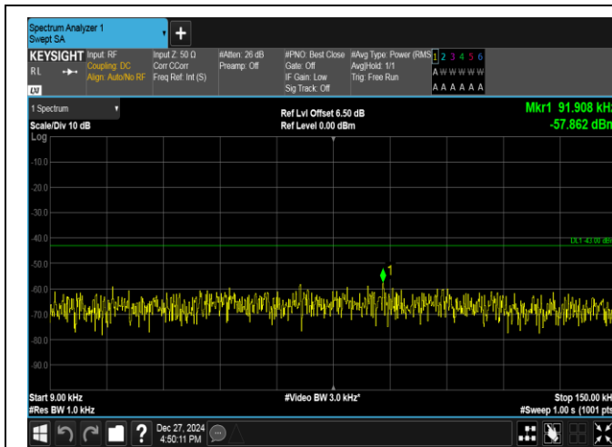
Band2-3MHz-QPSK-18615-1RB#0-0.009~0.15-PASS
