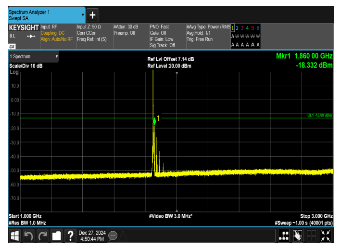
Band2-3MHz-QPSK-18615-1RB#0-1000~3000-PASS
