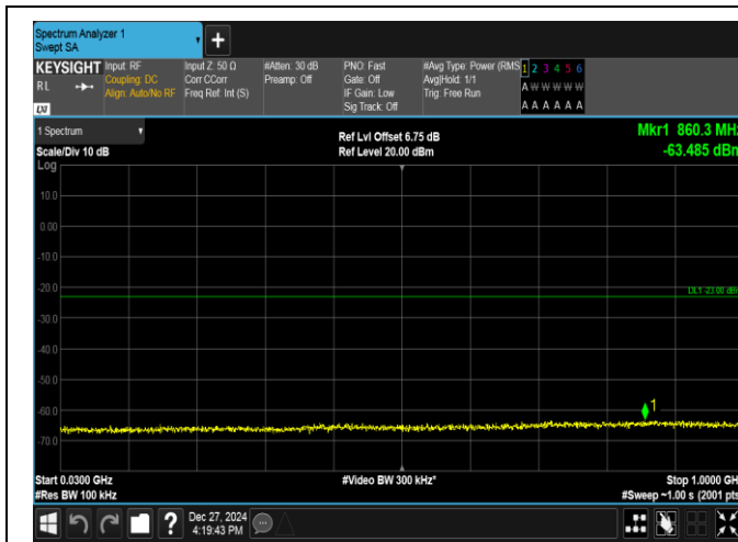
Band2-1.4MHz-QPSK-19193-6RB#0-30~1000-PASS
