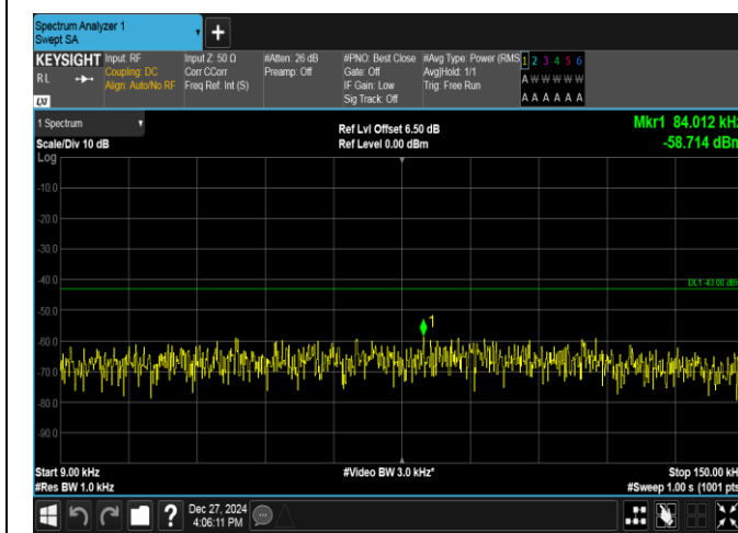
Band2-1.4MHz-16QAM-18607-1RB#5-0.009~0.15-PASS
