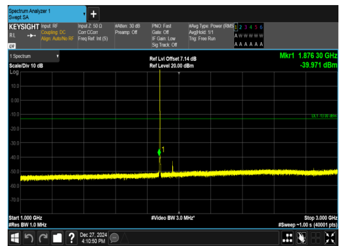
Band2-1.4MHz-16QAM-18900-1RB#0-1000~3000-PASS
