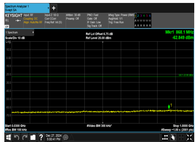
Band2-3MHz-QPSK-18900-15RB#0-30~1000-PASS
