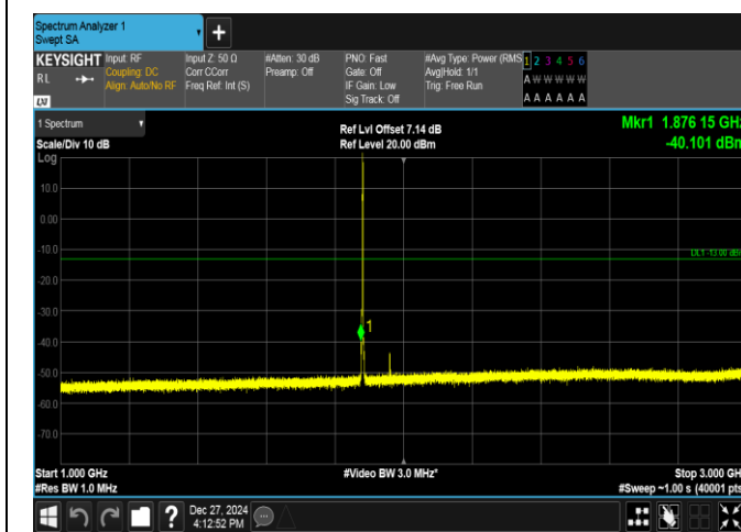
Band2-1.4MHz-16QAM-18900-1RB#5-1000~3000-PASS
