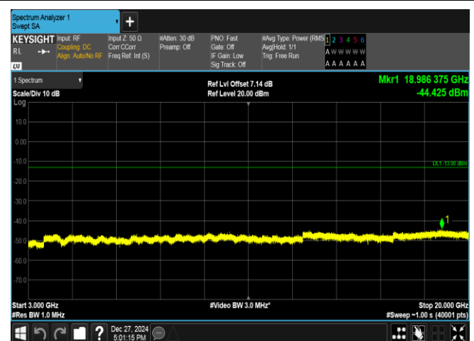
Band2-3MHz-QPSK-18900-15RB#0-3000~20000-PASS
