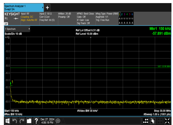
Band2-1.4MHz-16QAM-18607-1RB#5-0.15~30-PASS
