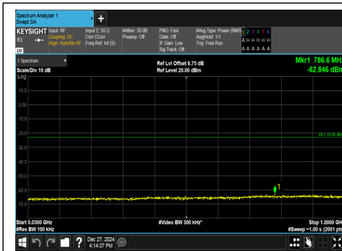
Band2-1.4MHz-16QAM-18900-6RB#0-30~1000-PASS
