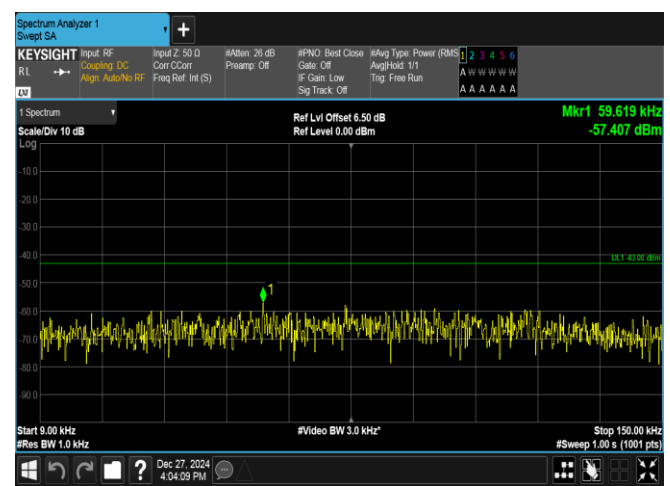
Band2-1.4MHz-16QAM-18607-1RB#0-0.009~0.15-PASS
