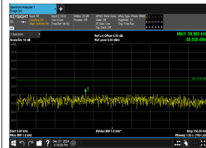
Band2-1.4MHz-16QAM-19193-1RB#5-0.009~0.15-PASS
