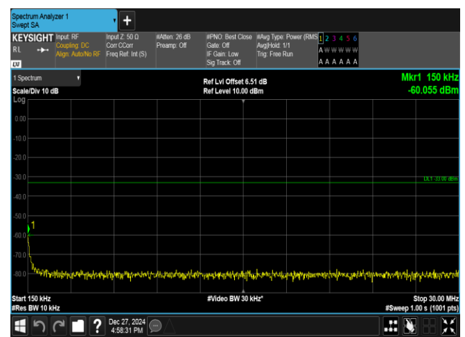
Band2-3MHz-QPSK-18900-1RB#14-0.15~30-PASS
