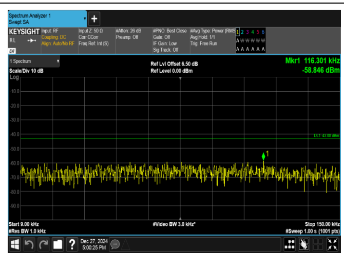
Band2-3MHz-QPSK-18900-15RB#0-0.009~0.15-PASS
