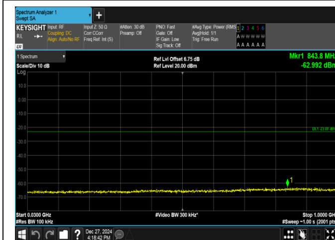
Band2-1.4MHz-16QAM-19193-1RB#5-30~1000-PASS
