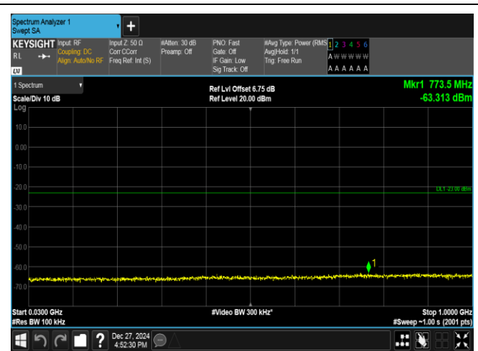
Band2-3MHz-QPSK-18615-1RB#14-30~1000-PASS
