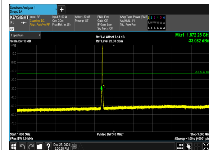
Band2-3MHz-QPSK-18900-15RB#0-1000~3000-PASS
