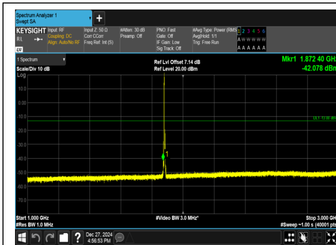
Band2-3MHz-QPSK-18900-1RB#0-1000~3000-PASS
