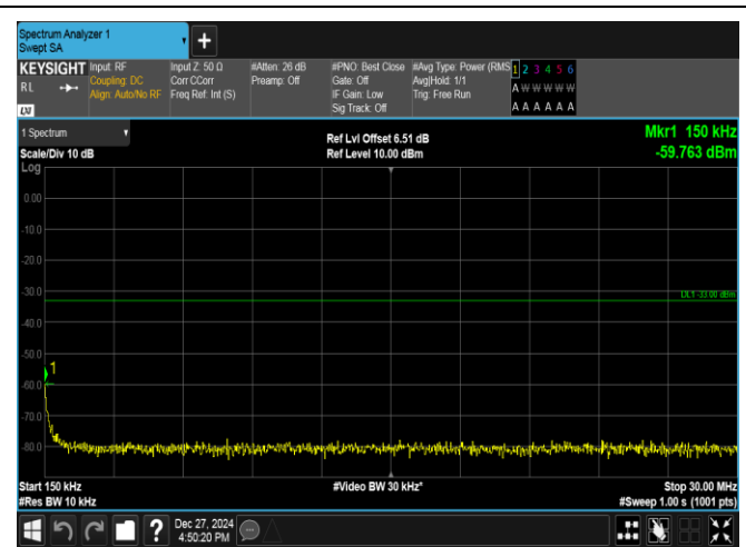
Band2-3MHz-QPSK-18615-1RB#0-0.15~30-PASS
