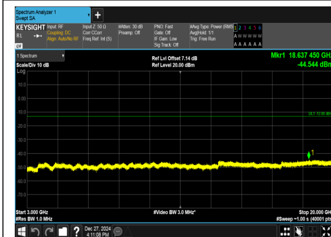
Band2-1.4MHz-16QAM-18900-1RB#0-3000~20000-PASS
