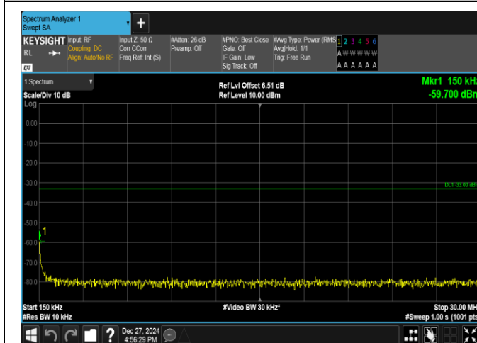
Band2-3MHz-QPSK-18900-1RB#0-0.15~30-PASS
