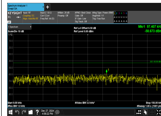
Band2-3MHz-QPSK-18900-1RB#14-0.009~0.15-PASS
