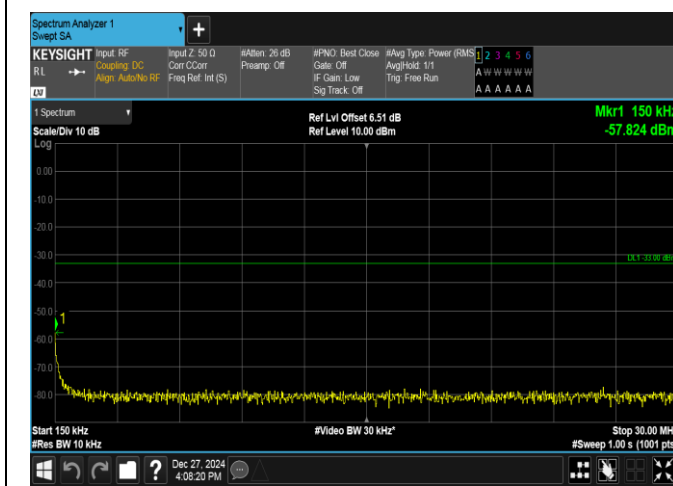
Band2-1.4MHz-16QAM-18607-6RB#0-0.15~30-PASS
