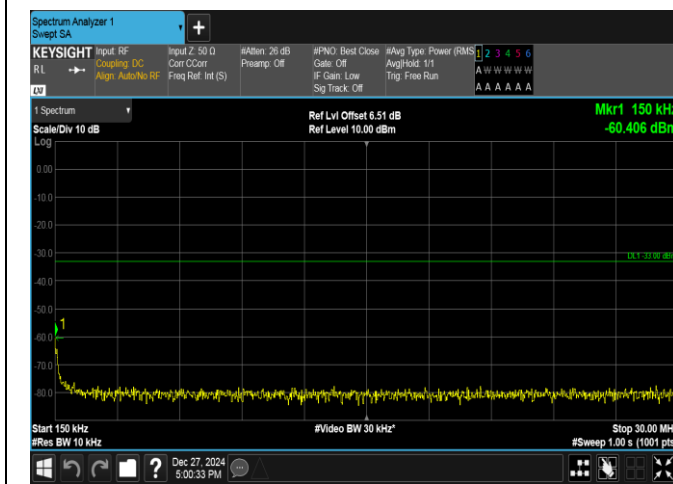
Band2-3MHz-QPSK-18900-15RB#0-0.15~30-PASS
