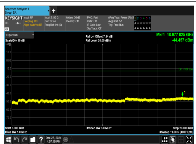
Band2-3MHz-QPSK-18900-1RB#0-3000~20000-PASS
