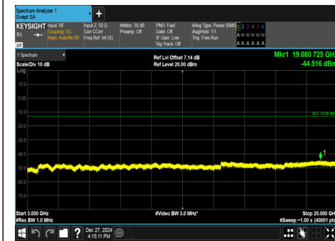
Band2-1.4MHz-16QAM-18900-6RB#0-3000~20000-PASS
