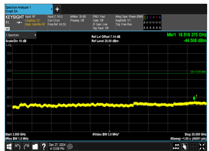
Band2-1.4MHz-16QAM-18900-1RB#5-3000~20000-PASS
