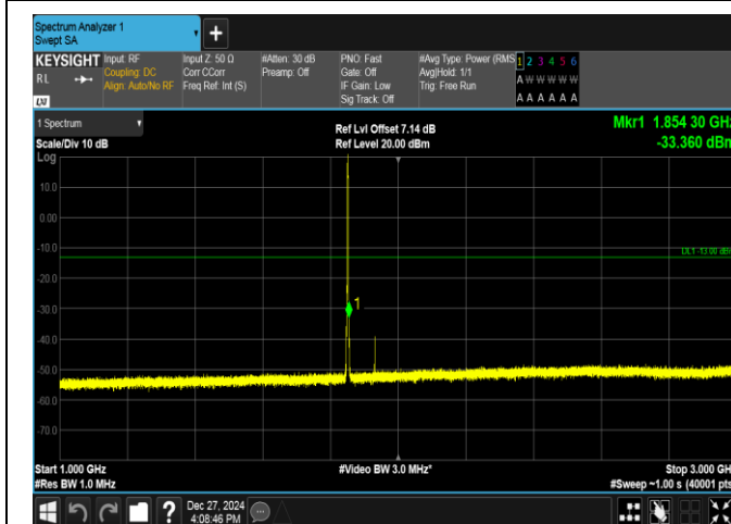
Band2-1.4MHz-16QAM-18607-6RB#0-1000~3000-PASS
