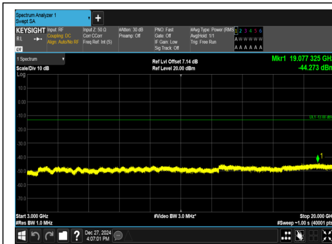
Band2-1.4MHz-16QAM-18607-1RB#5-3000~20000-PASS
