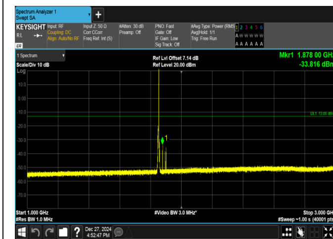
Band2-3MHz-QPSK-18615-1RB#14-1000~3000-PASS
