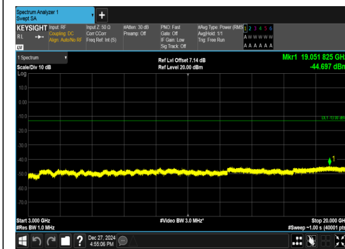
Band2-3MHz-QPSK-18615-15RB#0-3000~20000-PASS
