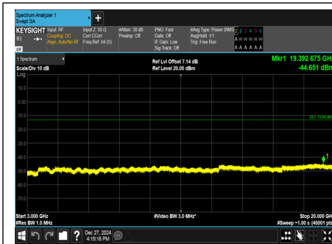
Band2-1.4MHz-16QAM-19193-1RB#5-3000~20000-PASS
