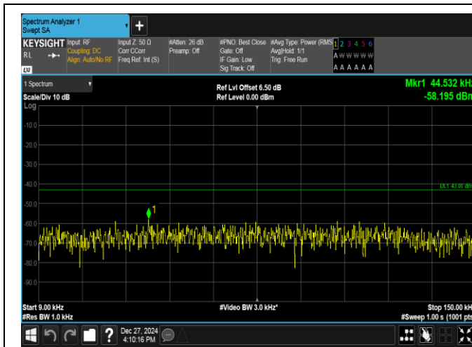
Band2-1.4MHz-16QAM-18900-1RB#0-0.009~0.15-PASS
