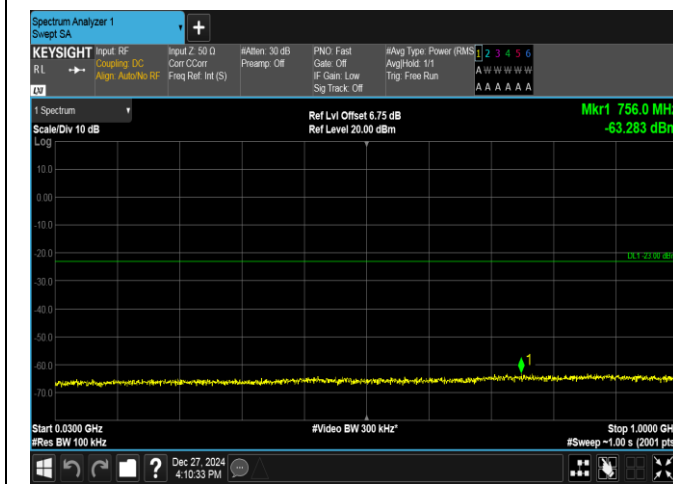
Band2-1.4MHz-16QAM-18900-1RB#0-30~1000-PASS
