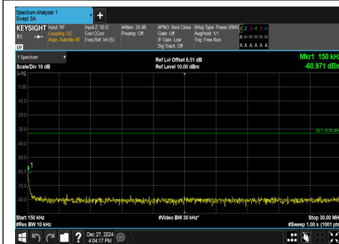
Band2-1.4MHz-16QAM-18607-1RB#0-0.15~30-PASS
