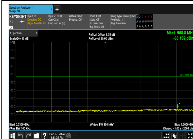
Band2-1.4MHz-QPSK-18900-1RB#5-30~1000-PASS
