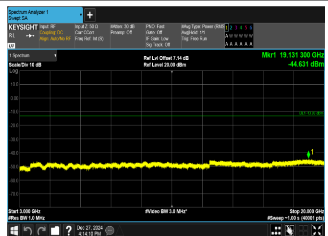
Band2-1.4MHz-QPSK-18900-6RB#0-3000~20000-PASS
