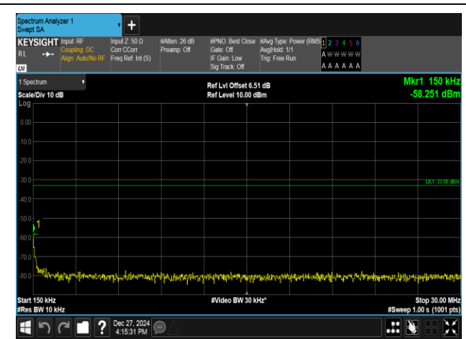
Band2-1.4MHz-QPSK-19193-1RB#0-0.15~30-PASS
