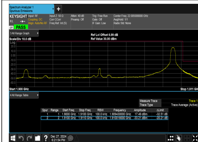
Band2-10MHz-16QAM-19150-1RB#49-PASS
