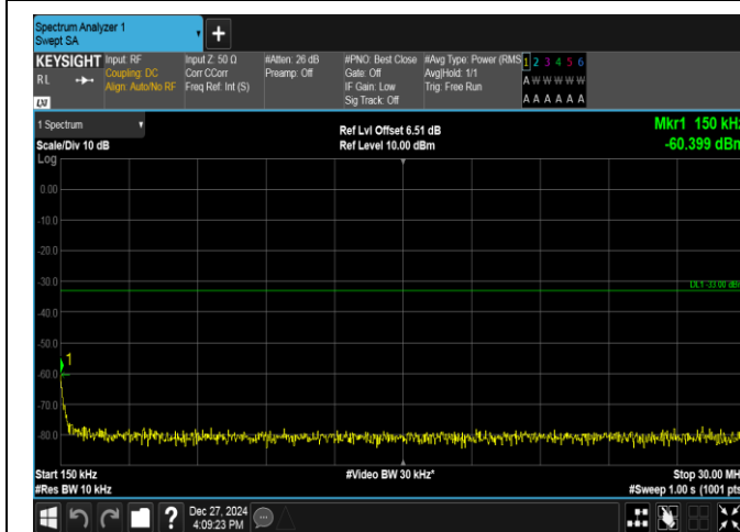
Band2-1.4MHz-QPSK-18900-1RB#0-0.15~30-PASS
