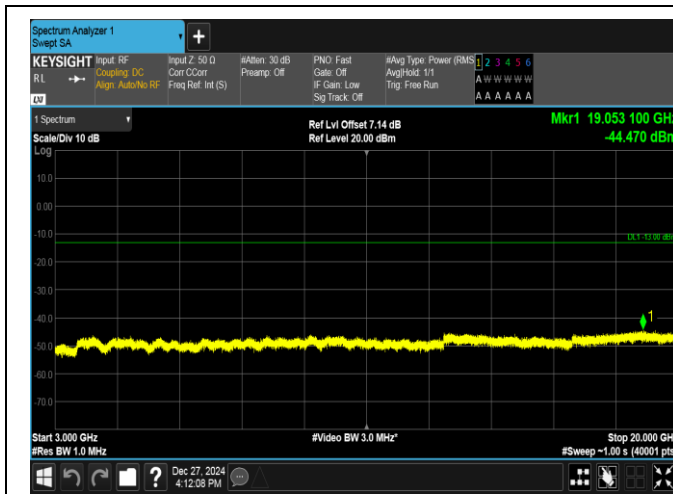
Band2-1.4MHz-QPSK-18900-1RB#5-3000~20000-PASS
