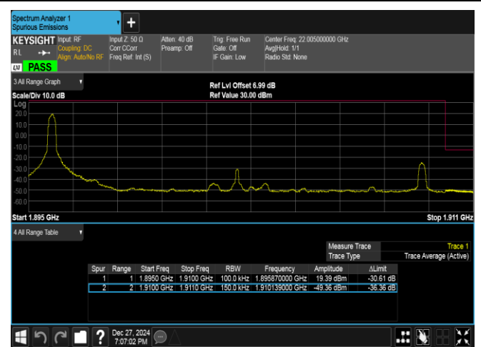
Band2-15MHz-QPSK-19125-1RB#0-PASS
