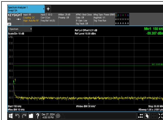
Band2-1.4MHz-QPSK-18607-1RB#5-0.15~30-PASS
