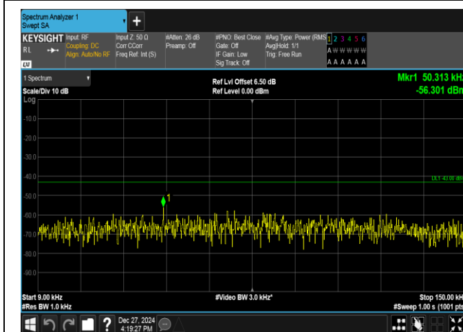
Band2-1.4MHz-QPSK-19193-6RB#0-0.009~0.15-PASS
