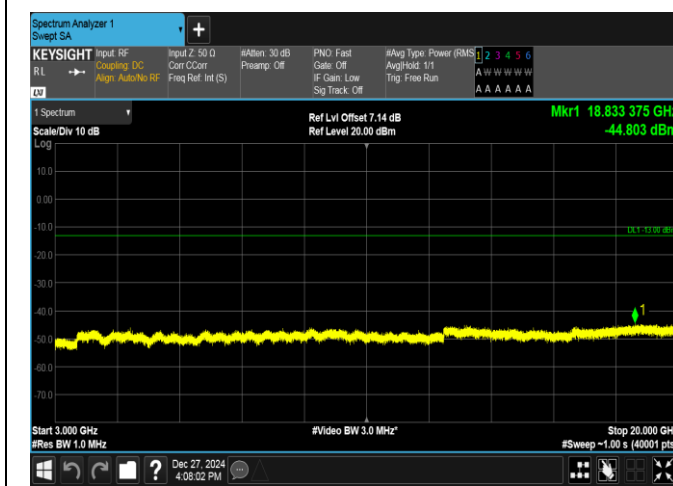
Band2-1.4MHz-QPSK-18607-6RB#0-3000~20000-PASS
