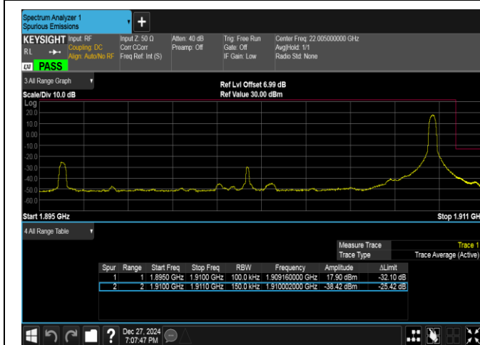
Band2-15MHz-16QAM-19125-1RB#74-PASS
