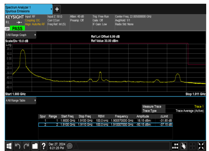
Band2-10MHz-16QAM-19150-1RB#0-PASS
