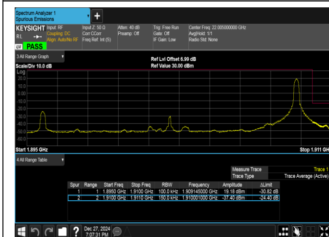
Band2-15MHz-QPSK-19125-1RB#74-PASS
