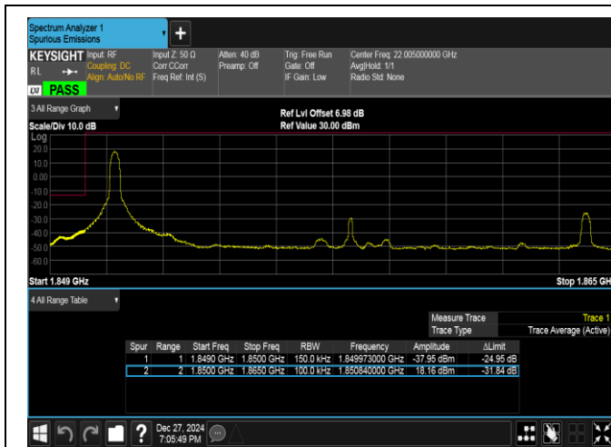
Band2-15MHz-16QAM-18675-1RB#0-PASS
