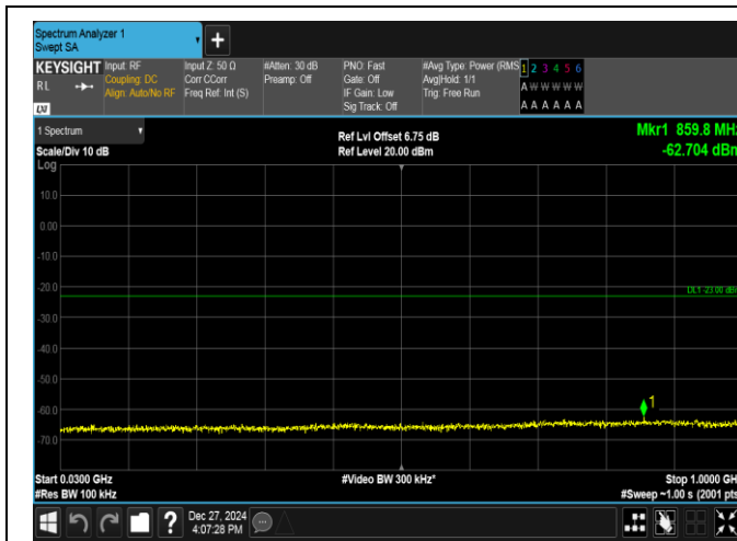
Band2-1.4MHz-QPSK-18607-6RB#0-30~1000-PASS
