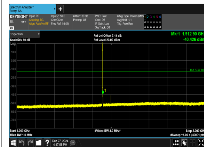
Band2-1.4MHz-QPSK-19193-1RB#5-1000~3000-PASS
