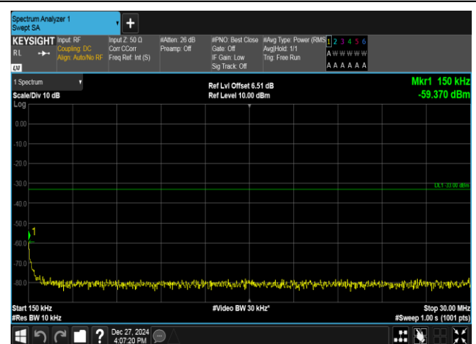
Band2-1.4MHz-QPSK-18607-6RB#0-0.15~30-PASS
