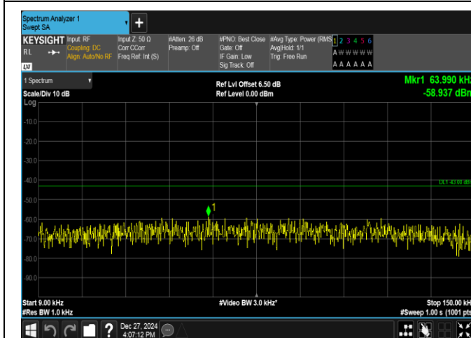
Band2-1.4MHz-QPSK-18607-6RB#0-0.009~0.15-PASS
