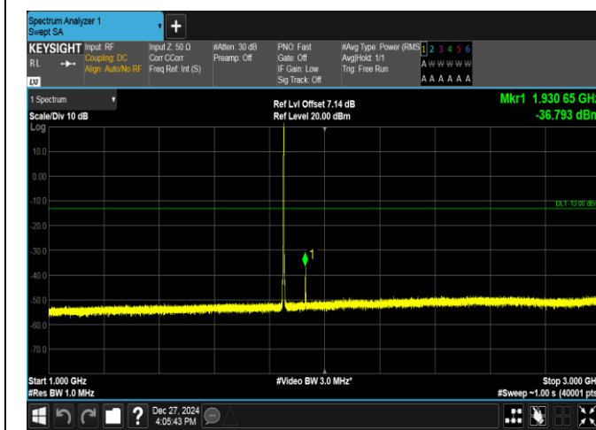
Band2-1.4MHz-QPSK-18607-1RB#5-1000~3000-PASS
