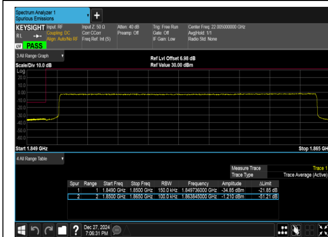
Band2-15MHz-QPSK-18675-75RB#0-PASS
