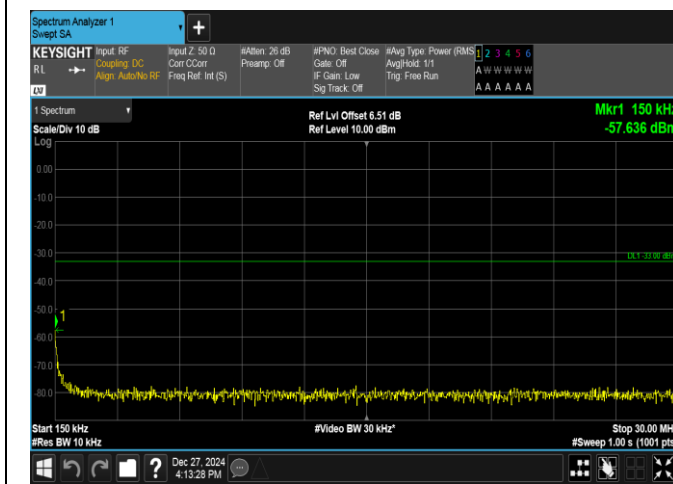
Band2-1.4MHz-QPSK-18900-6RB#0-0.15~30-PASS
