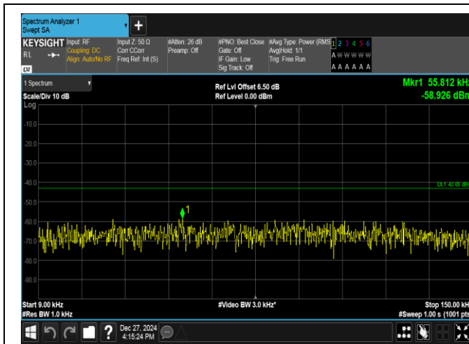
Band2-1.4MHz-QPSK-19193-1RB#0-0.009~0.15-PASS
