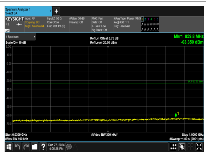
Band2-1.4MHz-QPSK-18607-1RB#5-30~1000-PASS
