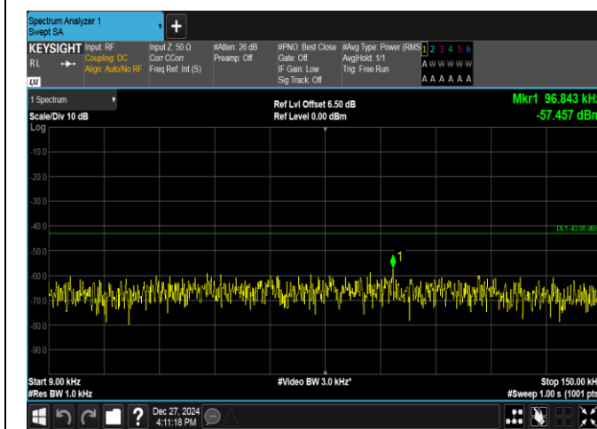
Band2-1.4MHz-QPSK-18900-1RB#5-0.009~0.15-PASS
