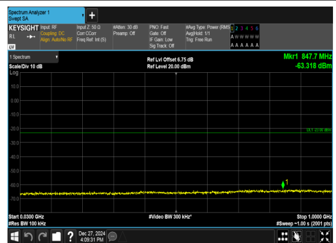
Band2-1.4MHz-QPSK-18900-1RB#0-30~1000-PASS
