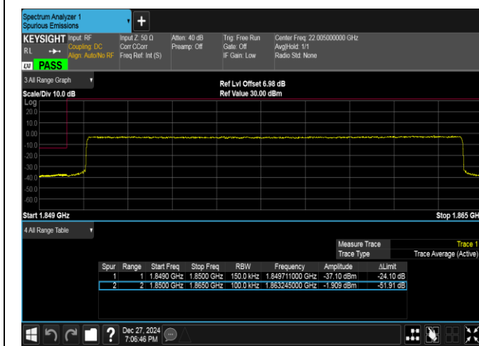
Band2-15MHz-16QAM-18675-75RB#0-PASS
