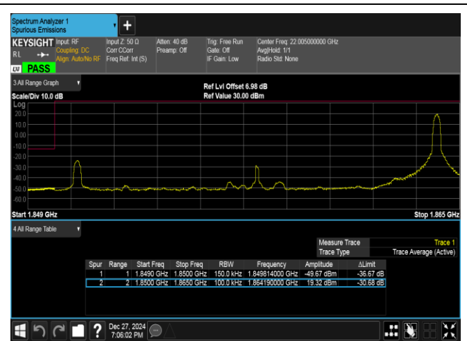
Band2-15MHz-QPSK-18675-1RB#74-PASS
