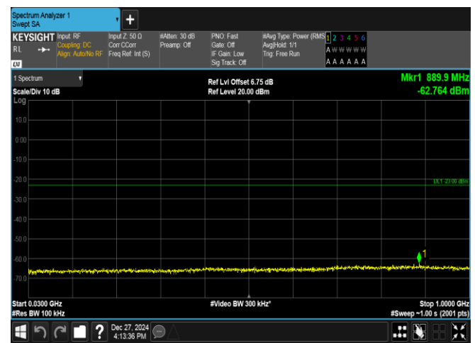
Band2-1.4MHz-QPSK-18900-6RB#0-30~1000-PASS
