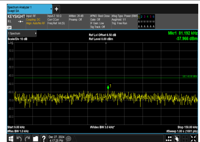
Band2-1.4MHz-QPSK-19193-1RB#5-0.009~0.15-PASS
