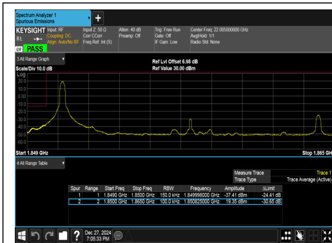
Band2-15MHz-QPSK-18675-1RB#0-PASS
