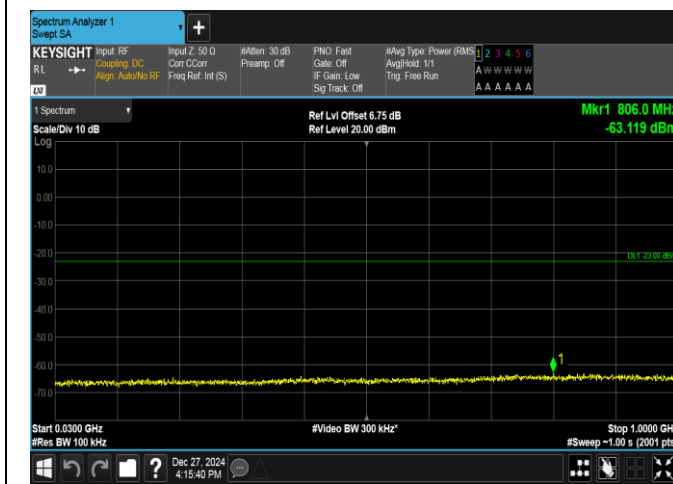
Band2-1.4MHz-QPSK-19193-1RB#0-30~1000-PASS
