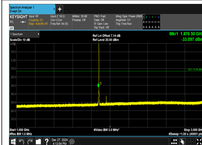
Band2-1.4MHz-QPSK-18900-6RB#0-1000~3000-PASS
