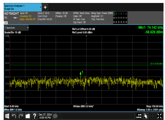
Band2-1.4MHz-QPSK-18900-1RB#0-0.009~0.15-PASS
