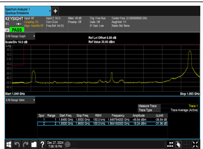
Band2-15MHz-16QAM-18675-1RB#74-PASS
