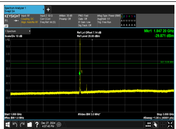
Band2-1.4MHz-QPSK-18607-6RB#0-1000~3000-PASS
