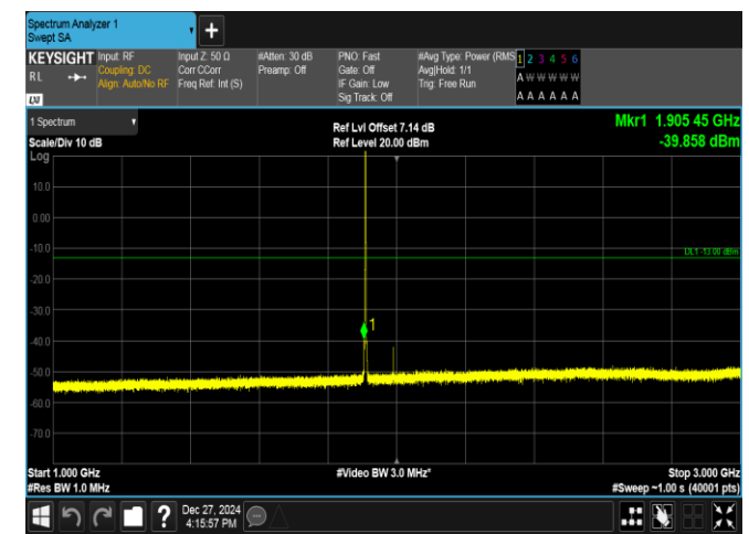
Band2-1.4MHz-QPSK-19193-1RB#0-1000~3000-PASS
