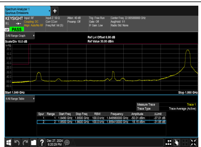
Band2-10MHz-16QAM-18650-1RB#49-PASS
