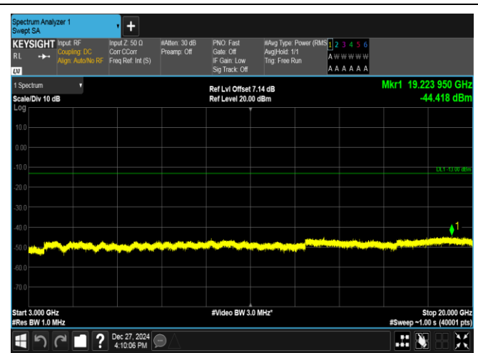
Band2-1.4MHz-QPSK-18900-1RB#0-3000~20000-PASS
