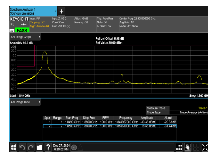
Band2-10MHz-16QAM-18650-1RB#0-PASS
