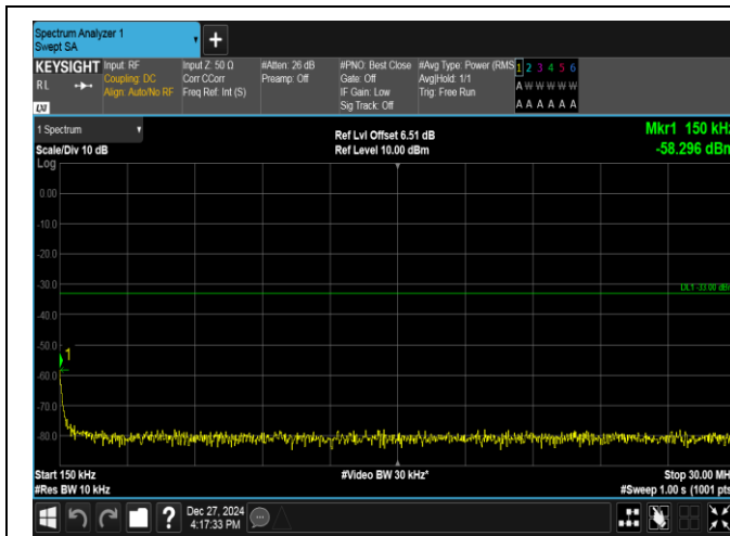
Band2-1.4MHz-QPSK-19193-1RB#5-0.15~30-PASS
