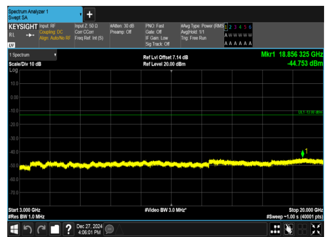
Band2-1.4MHz-QPSK-18607-1RB#5-3000~20000-PASS
