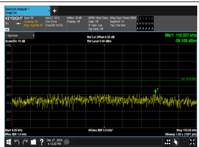
Band2-1.4MHz-QPSK-18900-6RB#0-0.009~0.15-PASS
