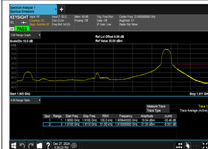
Band2-5MHz-QPSK-19175-1RB#24-PASS
