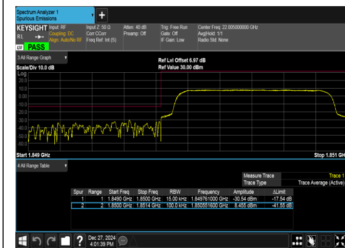
Band2-1.4MHz-16QAM-18607-6RB#0-PASS
