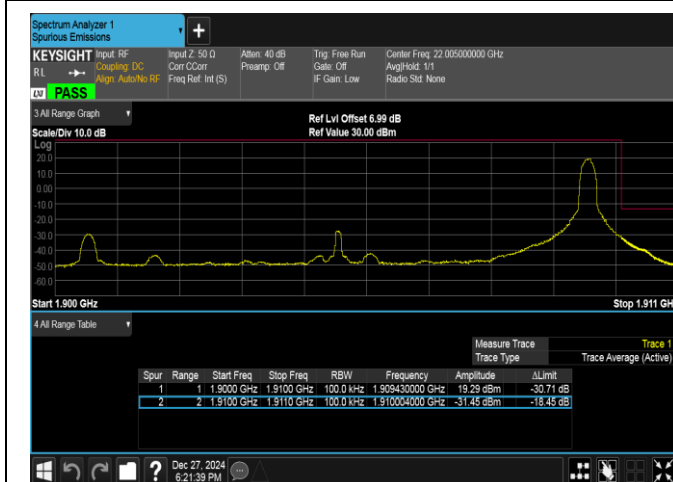
Band2-10MHz-QPSK-19150-1RB#49-PASS
