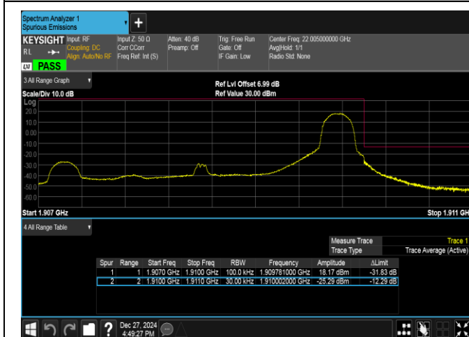
Band2-3MHz-16QAM-19185-1RB#14-PASS
