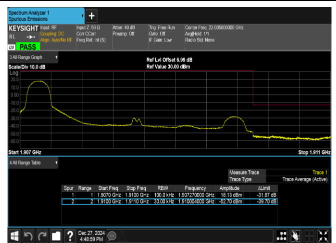
Band2-3MHz-16QAM-19185-1RB#0-PASS
