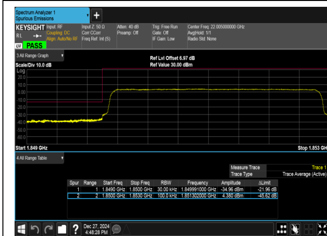
Band2-3MHz-16QAM-18615-15RB#0-PASS
