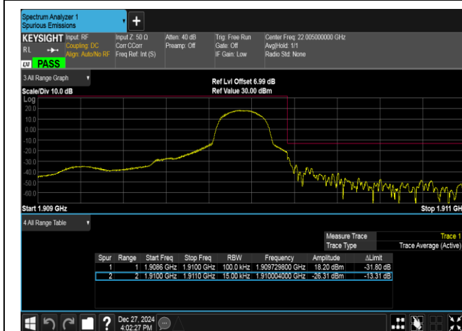
Band2-1.4MHz-16QAM-19193-1RB#5-PASS
