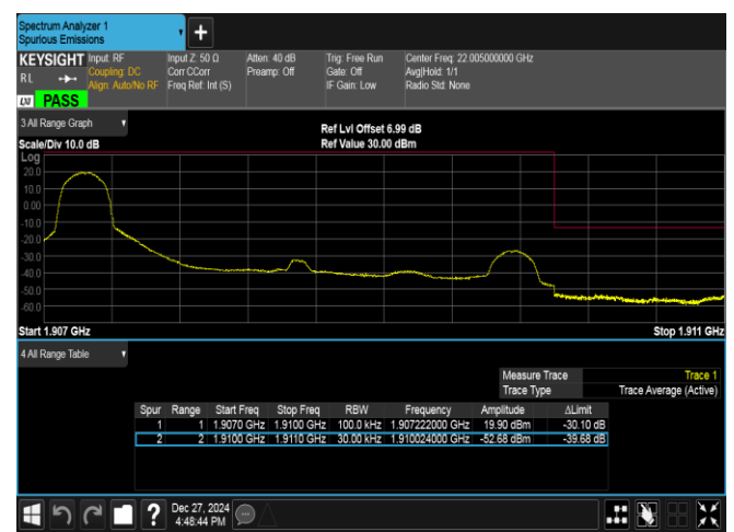
Band2-3MHz-QPSK-19185-1RB#0-PASS
