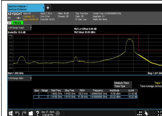
Band2-5MHz-16QAM-19175-1RB#24-PASS
