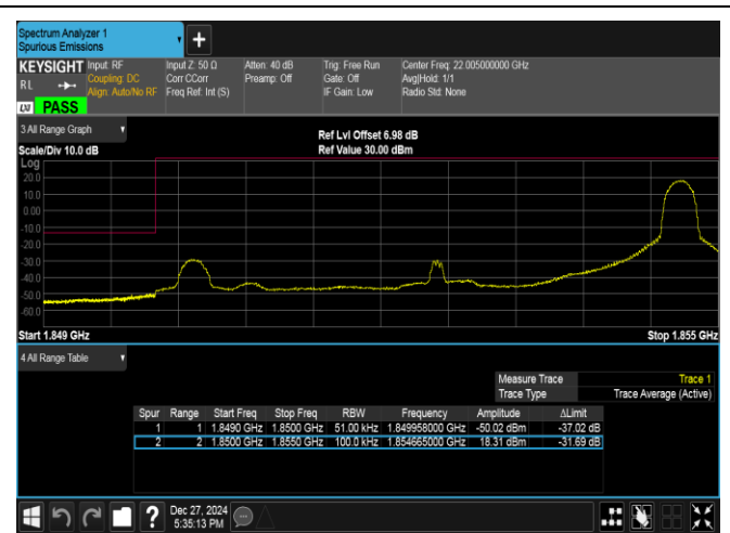
Band2-5MHz-16QAM-18625-1RB#24-PASS
