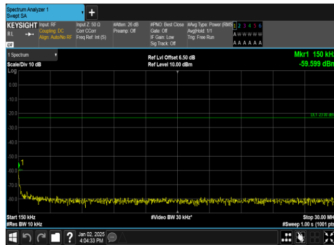
Band5-4233-2-0.15~30MHz-PASS
