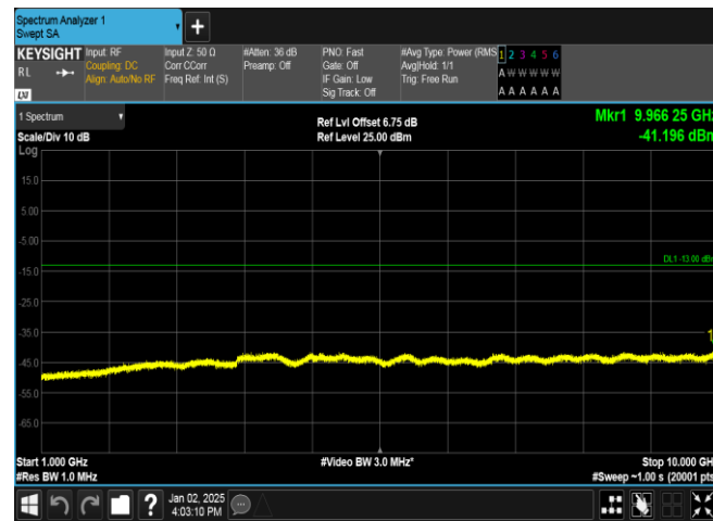
Band5-4182-2-1000~10000MHz-PASS
