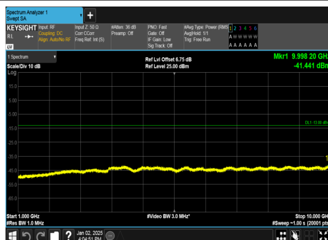
Band5-4233-2-1000~10000MHz-PASS
