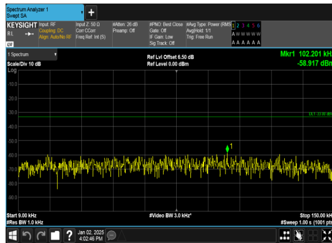
Band5-4182-2-0.009~0.15MHz-PASS
