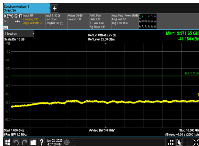
Band5-4182-3-1000~10000MHz-PASS
