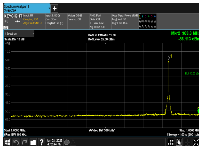
Band5-4182-4-30~1000MHz-PASS
