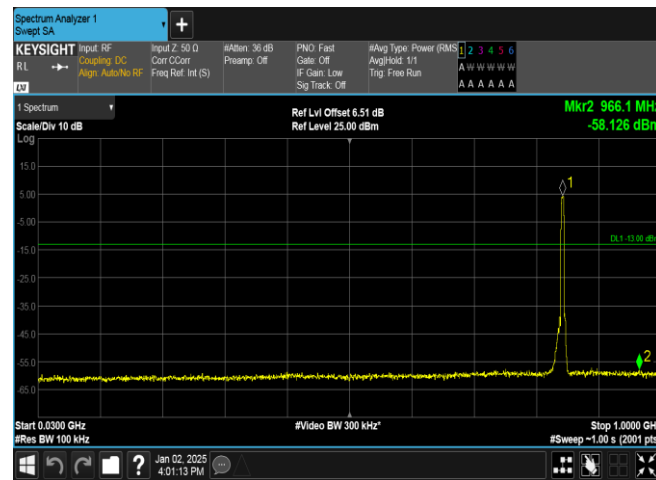
Band5-4233-1-30~1000MHz-PASS
