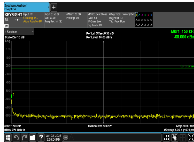
Band5-4182-1-0.15~30MHz-PASS
