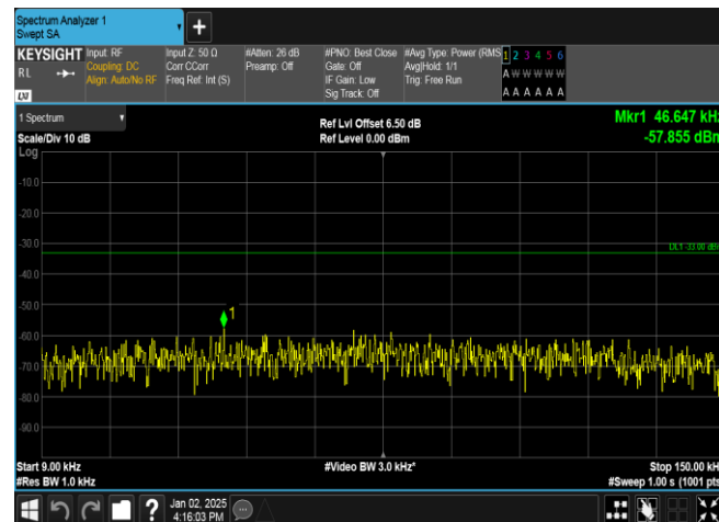
Band5-4182-5-0.009~0.15MHz-PASS
