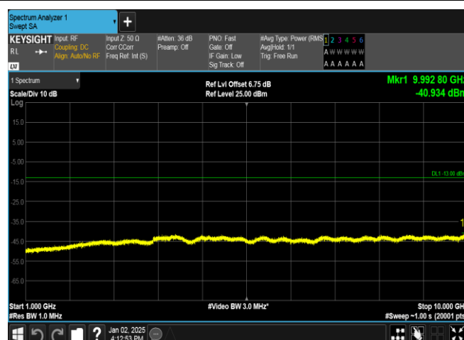
Band5-4182-4-1000~10000MHz-PASS
