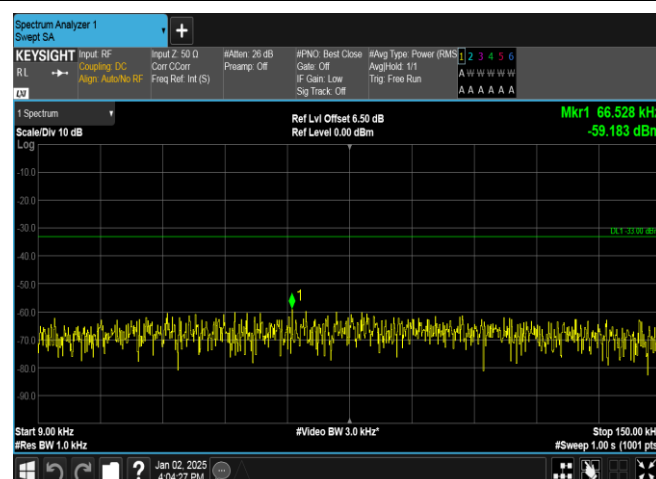
Band5-4233-2-0.009~0.15MHz-PASS
