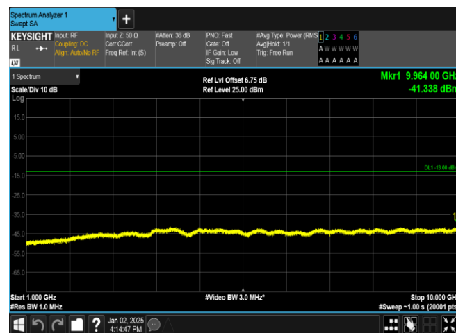
Band5-4233-4-1000~10000MHz-PASS
