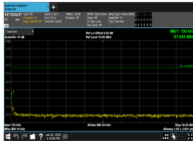
Band5-4233-5-0.15~30MHz-PASS
