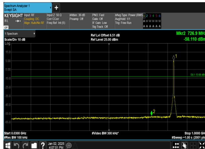
Band5-4182-3-30~1000MHz-PASS
