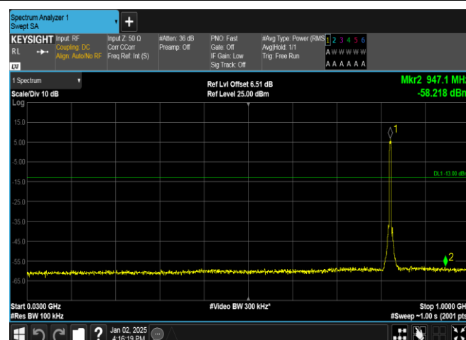
Band5-4182-5-30~1000MHz-PASS
