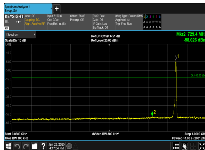
Band5-4233-5-30~1000MHz-PASS
