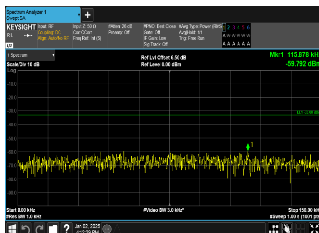
Band5-4182-4-0.009~0.15MHz-PASS
