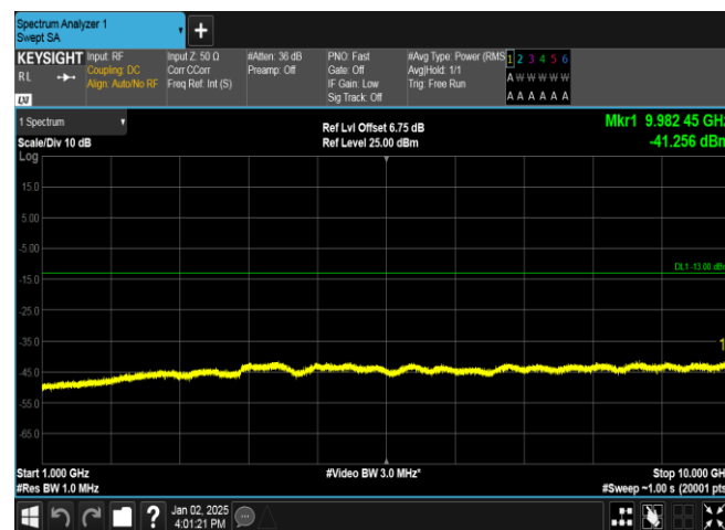
Band5-4233-1-1000~10000MHz-PASS
