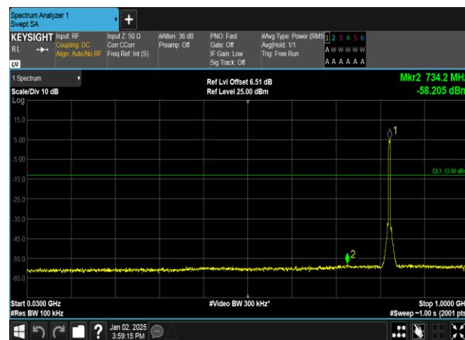
Band5-4182-1-30~1000MHz-PASS
