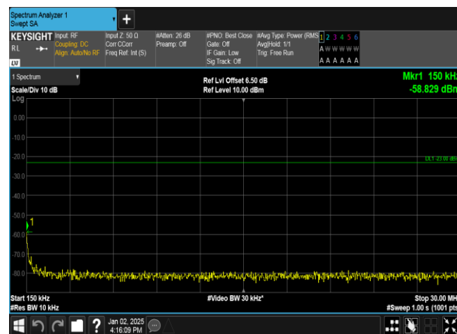
Band5-4182-5-0.15~30MHz-PASS
