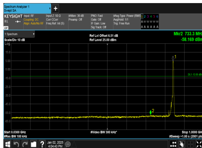
Band5-4233-2-30~1000MHz-PASS
