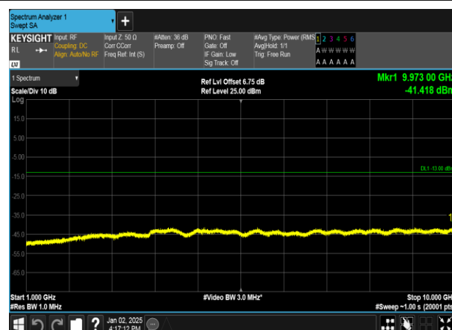
Band5-4233-5-1000~10000MHz-PASS
