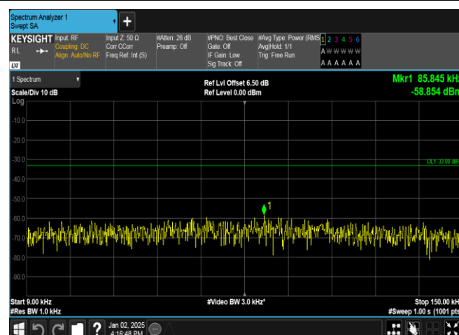
Band5-4233-5-0.009~0.15MHz-PASS
