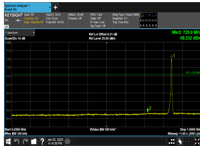
Band5-4233-4-30~1000MHz-PASS
