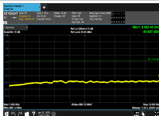
Band5-4182-1-1000~10000MHz-PASS
