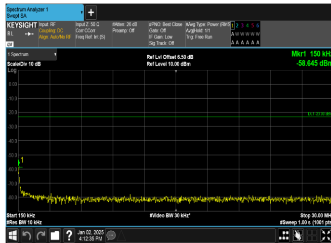
Band5-4182-4-0.15~30MHz-PASS
