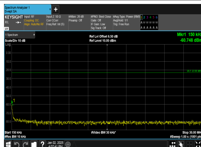
Band5-4182-3-0.15~30MHz-PASS
