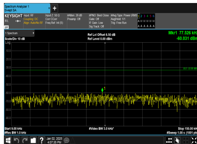
Band5-4182-3-0.009~0.15MHz-PASS
