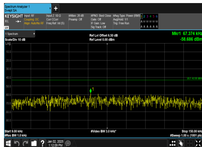
Band4-1312-2-0.009~0.15MHz-PASS
