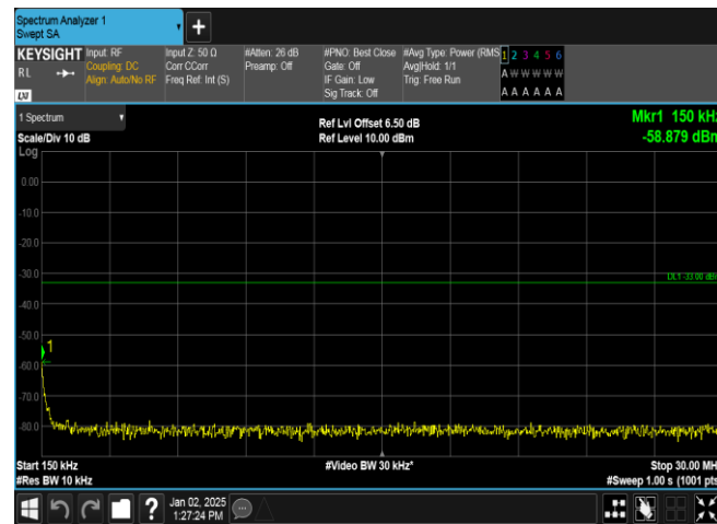
Band4-1413-5-0.15~30MHz-PASS
