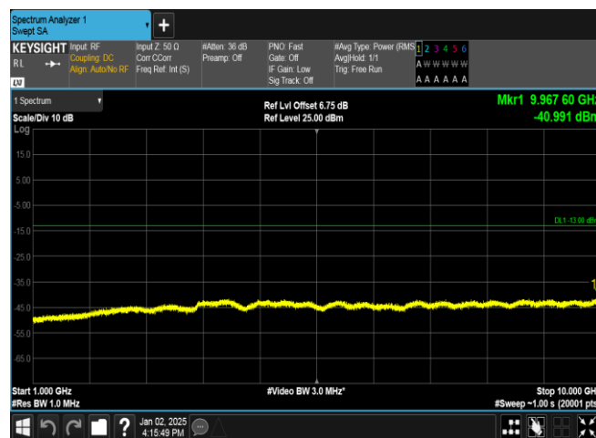
Band5-4132-5-1000~10000MHz-PASS
