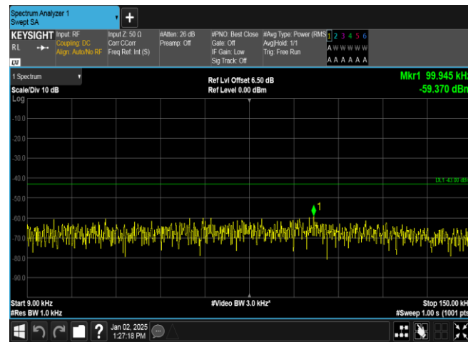
Band4-1413-5-0.009~0.15MHz-PASS
