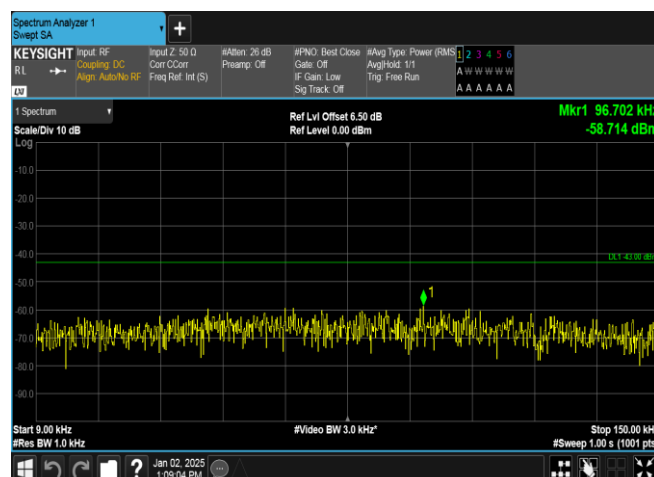
Band4-1413-1-0.009~0.15MHz-PASS
