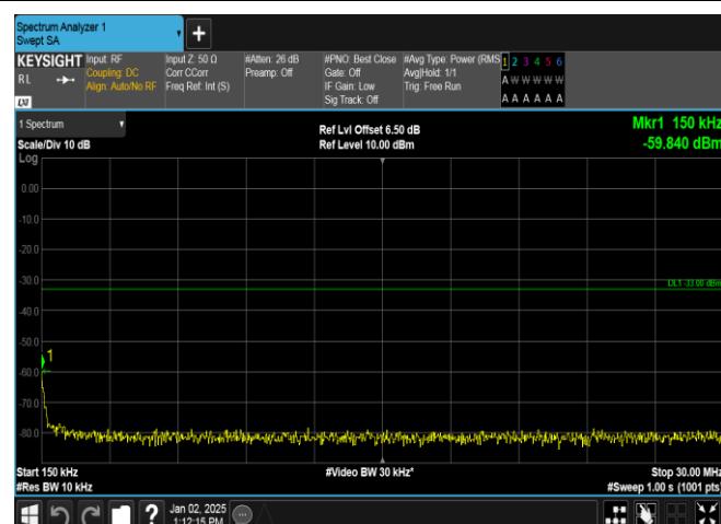
Band4-1312-2-0.15~30MHz-PASS
