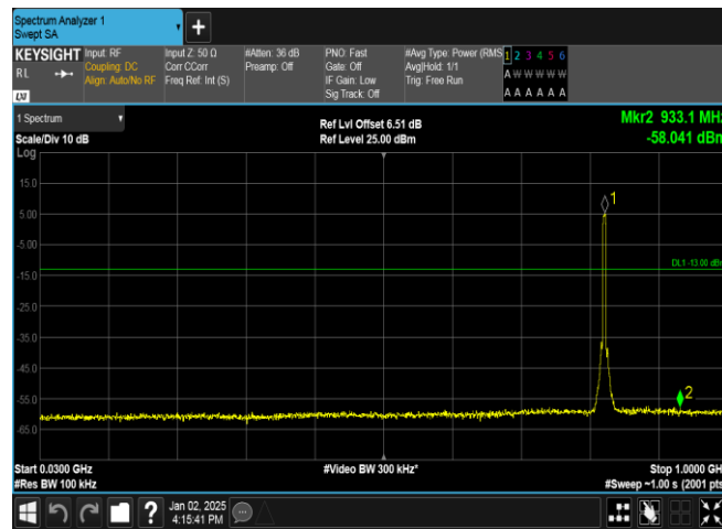
Band5-4132-5-30~1000MHz-PASS
