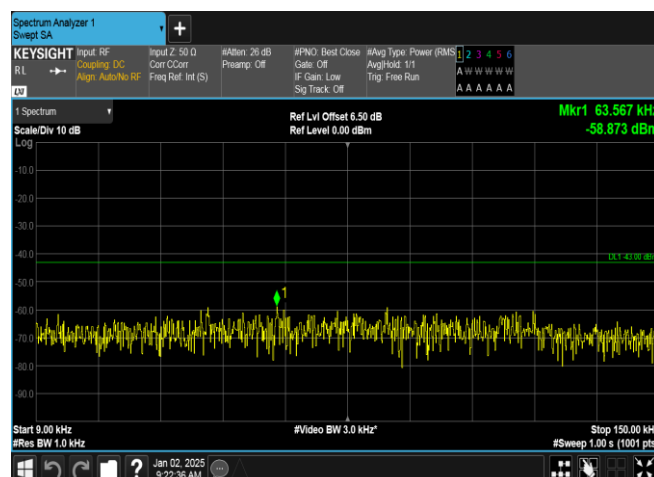
Band2-9400-4-0.009~0.15MHz-PASS
