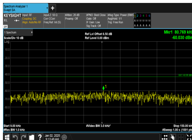
Band2-9400-2-0.009~0.15MHz-PASS
