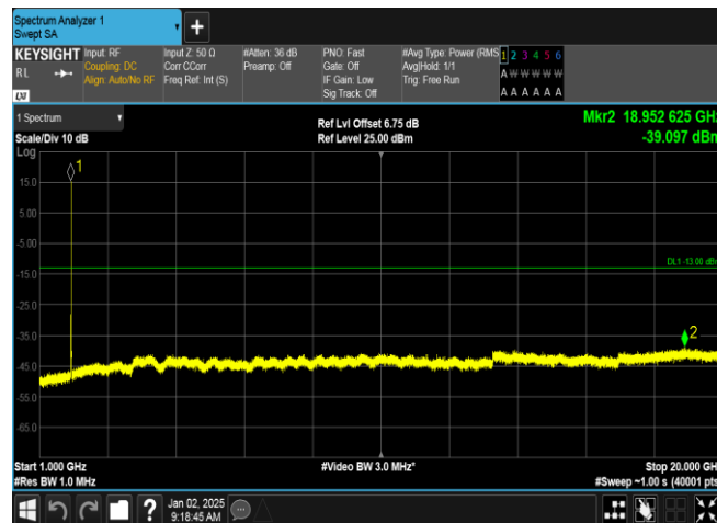
Band2-9400-3-1000~20000MHz-PASS
