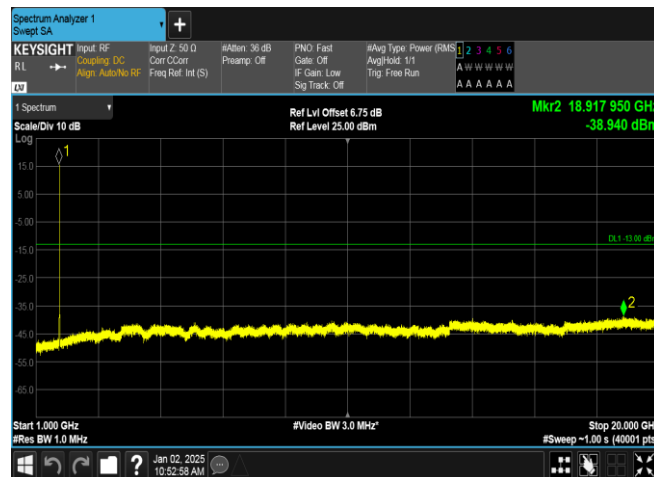
Band4-1312-2-1000~20000MHz-PASS
