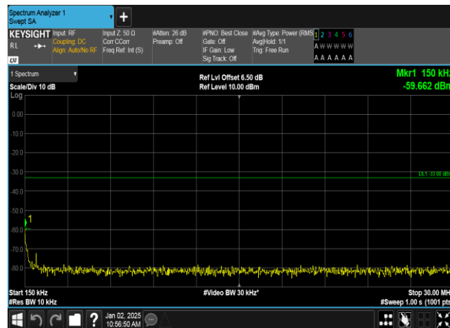
Band4-1312-4-0.15~30MHz-PASS
