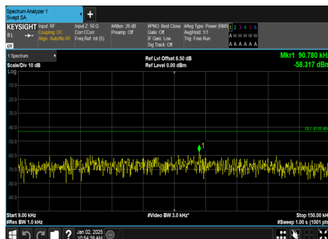
Band4-1312-3-0.009~0.15MHz-PASS
