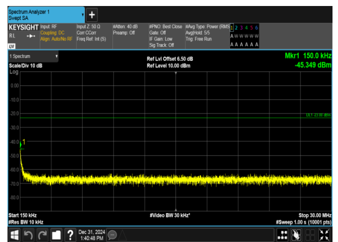
EGPRS850-251-8-0.15~30MHz-PASS
