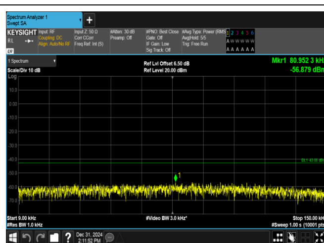
GPRS1900-512-0-0.009~0.15MHz-PASS
