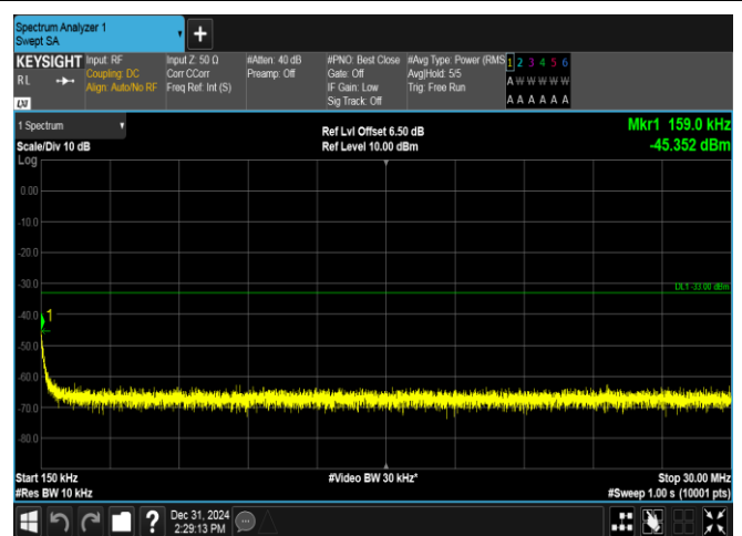
EGPRS1900-512-2-0.15~30MHz-PASS
