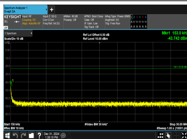
EGPRS850-128-8-0.15~30MHz-PASS
