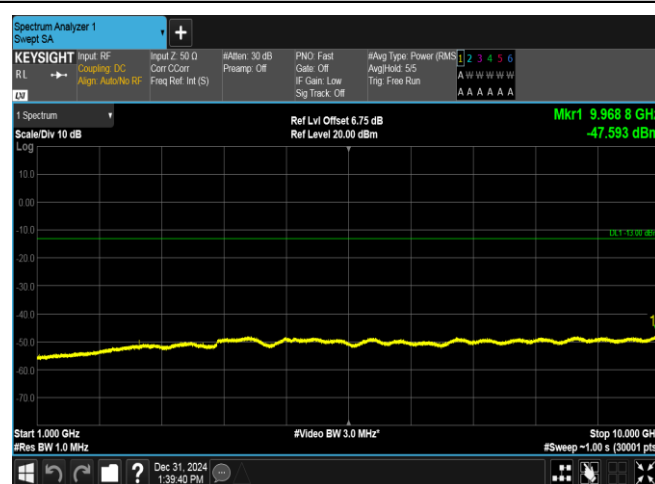
EGPRS850-128-8-1000~10000MHz-PASS
