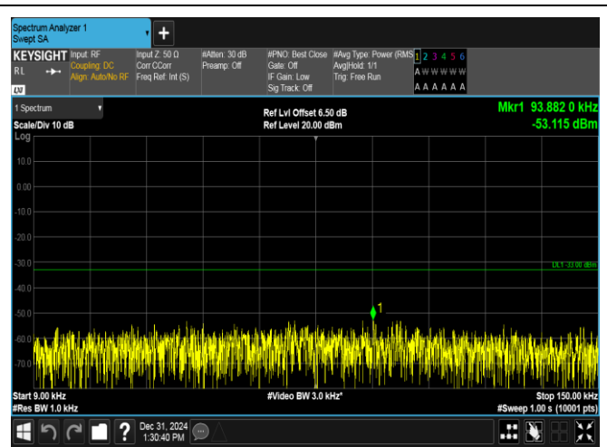
GPRS850-190-5-0.009~0.15MHz-PASS
