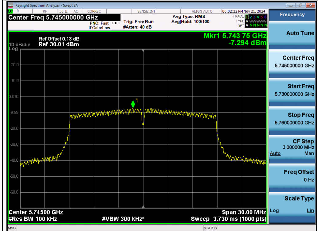
Test_Graph_802.11n20_ANT1_5745_MCS0_PSD
