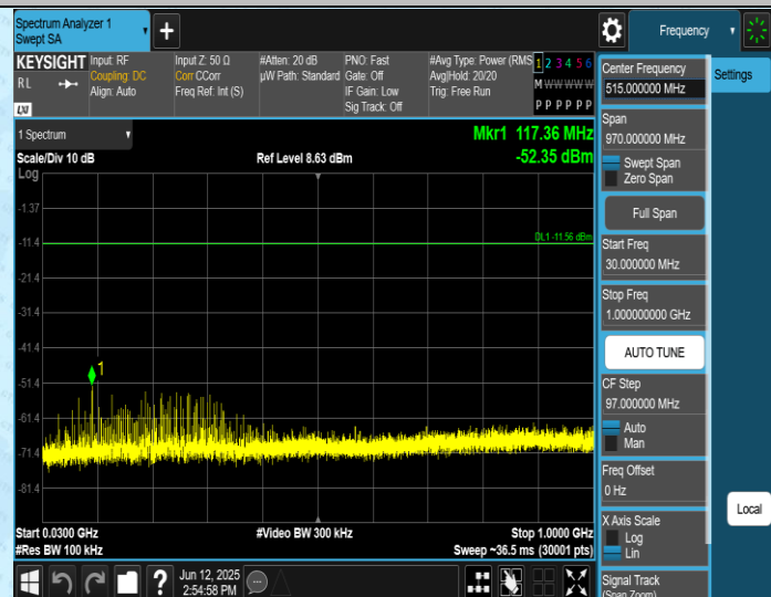
TX-Ant1-2475-30~1000-PASS
