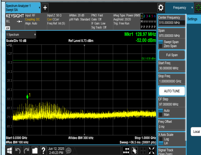
TX-Ant1-2440-30~1000-PASS
