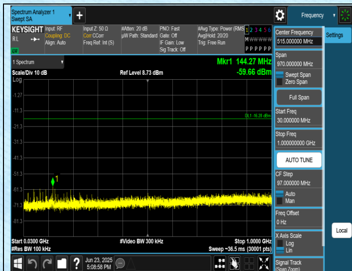
TX-Ant1-2440-30~1000-PASS
