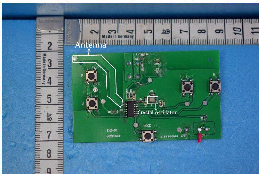
Internal view of EUT
